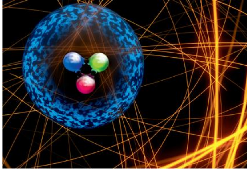
Quarks The concept of quarks is a vital element of our theories of fundamental physics even though individual quarks cannot be observed.
