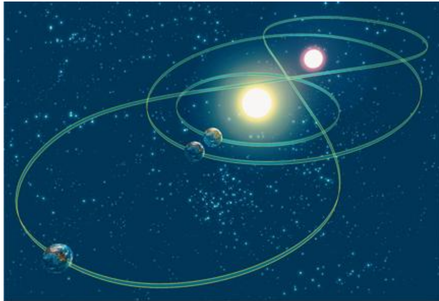
Binary Orbits Planets that orbit binary star systems will probably have inhospitable weather, in some seasons too hot for life, in others, too cold.
