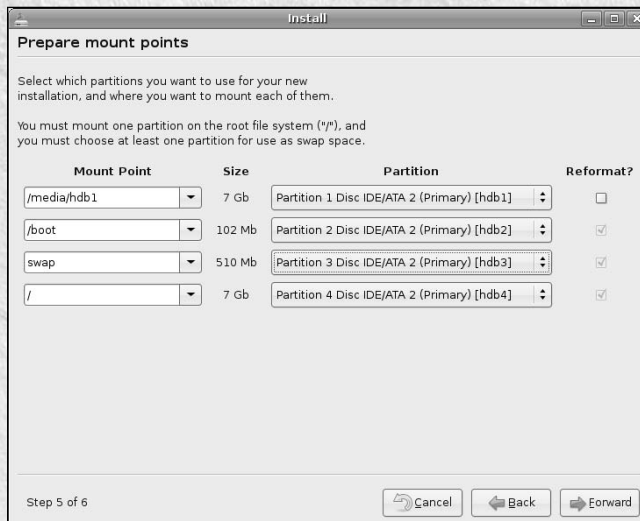
Identifying partition mount points during manual partitioning
