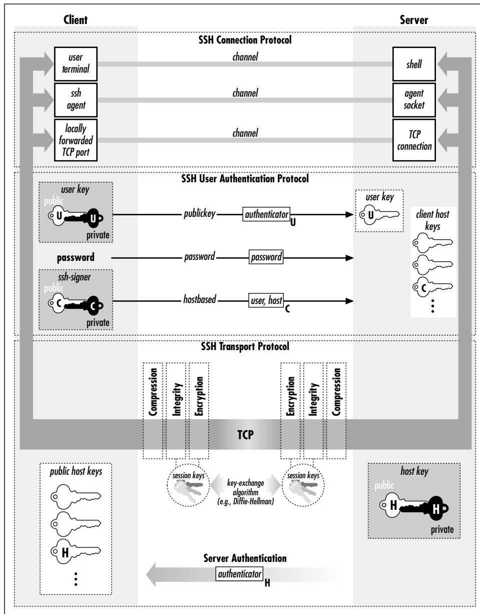
Figure 3-4. SSH-2 architecture
