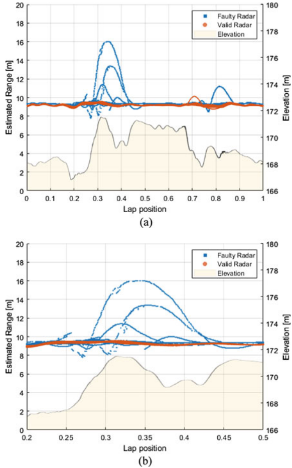
Fig. 10 a Headway perceived by the CACC system for valid and faulty radar; b Range estimate in region of interest for truck T13 in a 4 T 100' platoon with and without radar faults
