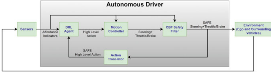
Fig. 29 Training architecture
