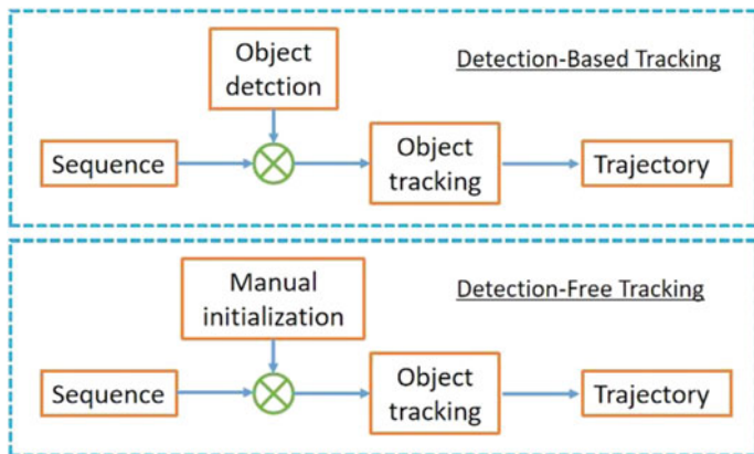
Fig. 32 Detection-based tracking and detection-free tracking
