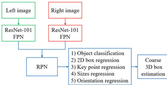
Fig. 7 The overall flowchart of Stereo RCNN (SRCNN)
