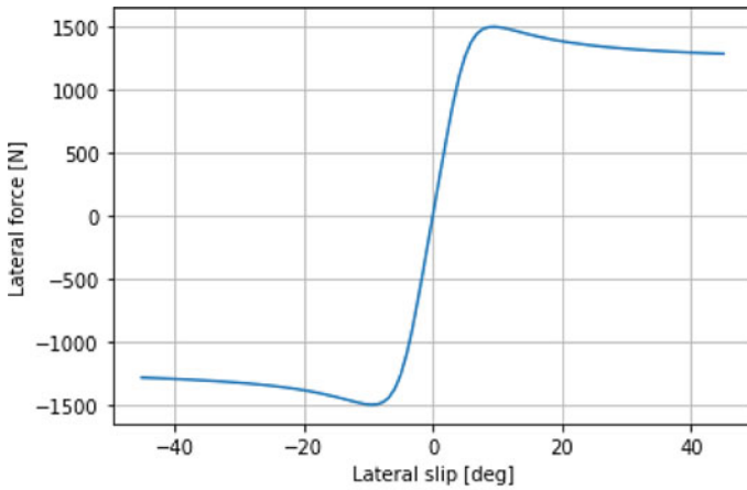
(a) Lateral Tire Curve
