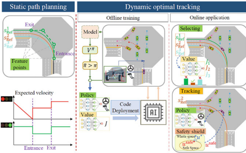
Fig. 2 Illustration of the integrated decision and control framework
