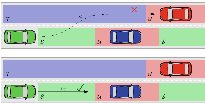
Fig. 11 Exemplary visualization of safe ( S ), temporary safe ( T ) and unsafe ( U ) sets of states including an unsafe action a and a safe action a_c . For simplicity only temporal sets of states are shown
