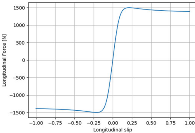
(b) Longitudinal Tire Curve
