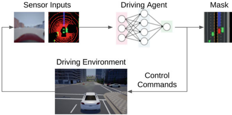
Fig. 9 The interpretable end-to-end autonomous driving agent
