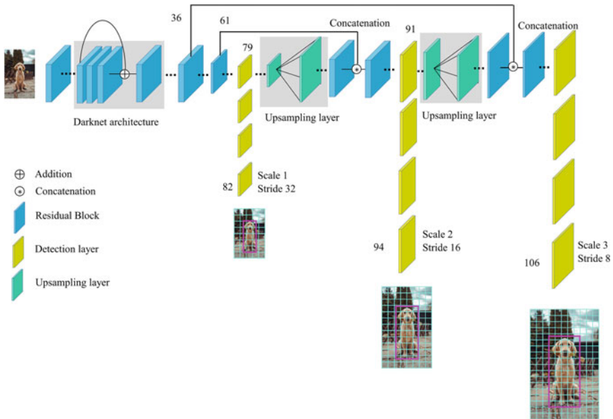
Fig. 24 The architecture of YOLO v3 network
