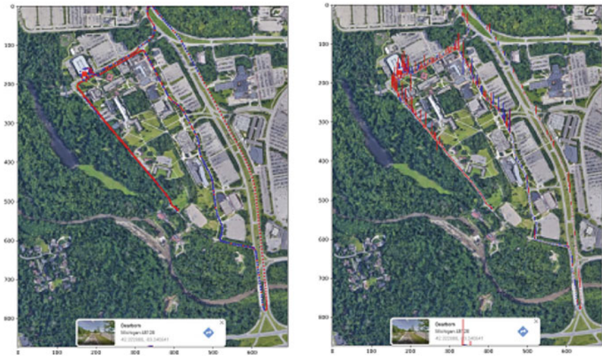
Fig. 5 The illustration of the best beam varying with positions (left) and gain of beamforming when comparing omnidirectional antenna
