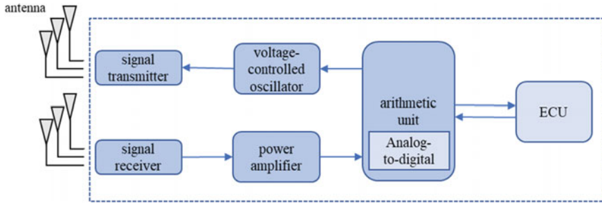
Fig. 8 Schematic diagram of the basic working principle of MWR
