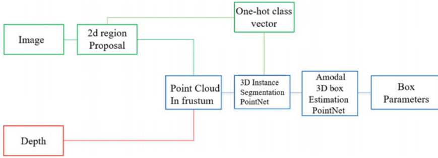
Fig. 2 The network structure of Frustum PointNets (F-PointNet)
