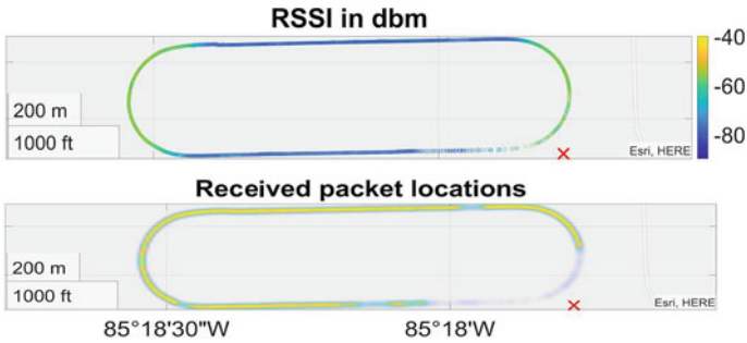
Fig. 32 RSSI and received packet reception density graphs. Interference source marked with a red cross
