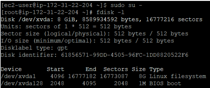
Figure 2.2 – Check the Linux instance disk storage
