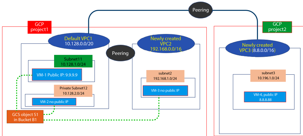
Figure 11.10 – GCP diagram
