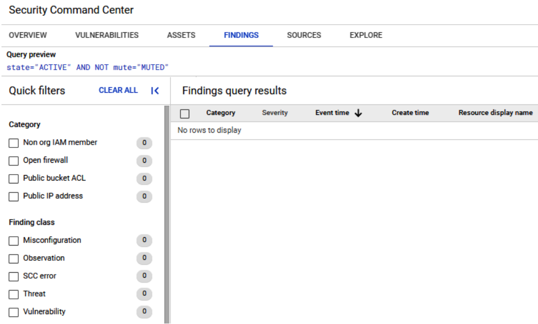
Figure 11.3 – SCC findings
