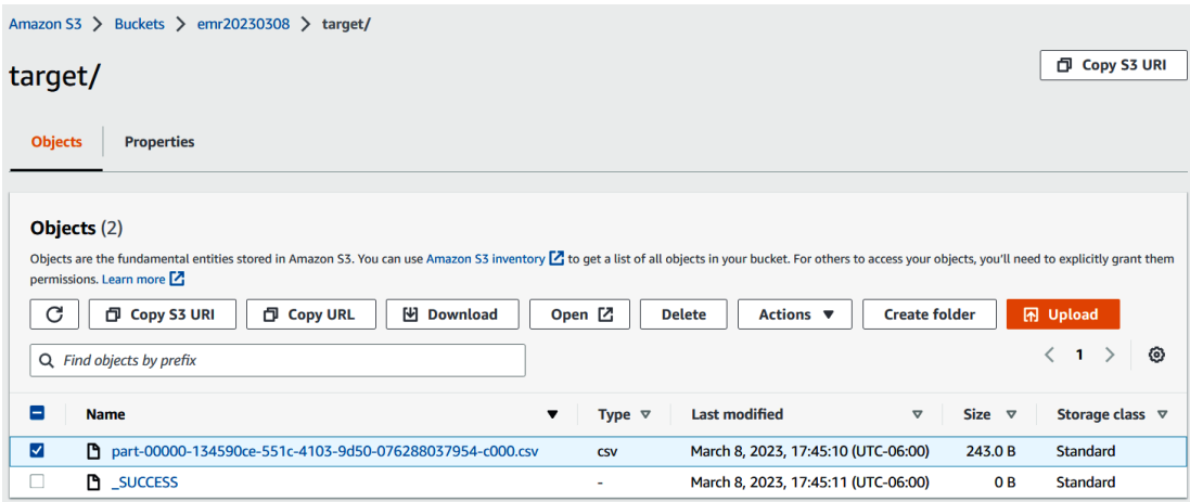
Figure 5.33 – Spark step target folder
