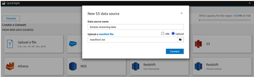
Figure 5.19 – Generate dataset
