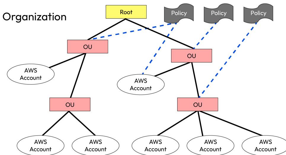
Figure 7.6 – AWS Organizations
