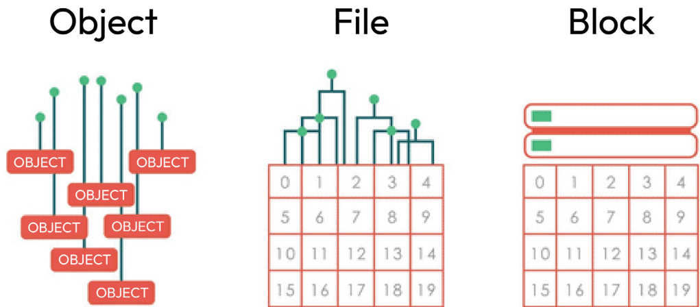
Figure 2.1 – Object storage, filesystem, and block storage
