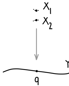
FIGURE 28.3. “Formal neighborhoods” of X_1 and X_2 in the proof of Zariski’s Connectedness Lemma 28.4.1
