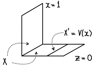
FIGURE 9.6. Order matters in a regular sequence (in the “non-local” situation), for unsurprising reasons
