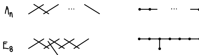
FIGURE 22.2. The exceptional divisors for resolutions of some ADE surface singularities, and their corresponding dual graphs (see Remark 22.4.5)
