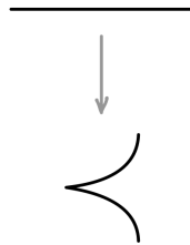
FIGURE 10.5. Normalization of a cusp
