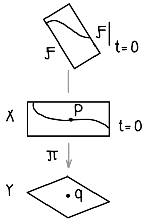
FIGURE 24.4. The (sufficient) slicing criterion for flatness on the source, Theorem 24.6.9
