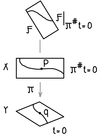
FIGURE 24.3. The (necessary and sufficient) slicing criterion for flatness on the target, Theorem 24.6.6
