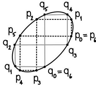
FIGURE 19.9. Exercise 19.10.L (with 17 replaced by 3)
