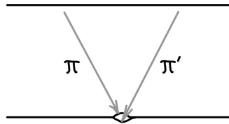
FIGURE 11.4. Two different maps to a nonseparated scheme agreeing on a dense open set (see Exercise 11.3.D)
