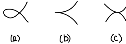
FIGURE 13.3. Plane curve singularities
