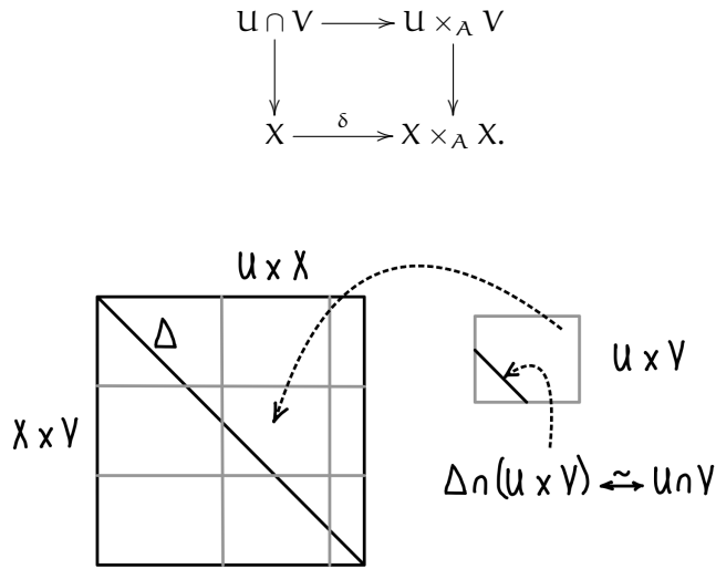
FIGURE 11.3. \Delta \cap (U \times V) \cong U \cap V (Exercise 11.2.M)
