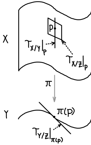
FIGURE 21.2. The geometry behind the cotangent exact sequence
