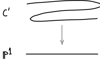
FIGURE 16.3. Constructing a projective regular model of a curve C over k via a finite cover of \mathbb{P}^1
