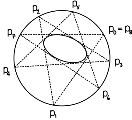
FIGURE 19.8. Poncelet's Porism 19.10.8
