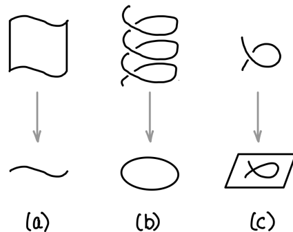
FIGURE 24.6. Sketches of notions from differential geometry: (a) maps “locally on the source a smooth fibration”, (b) local isomorphisms, and (c) immersions. (In algebraic geometry: (a) smooth morphisms, (b) étale morphisms, and (c) unramified morphisms.)
