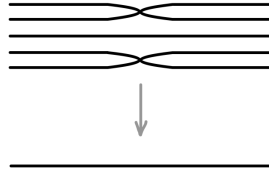
FIGURE 21.4. An example where the branch divisor appears with multiplicity 2 (see Exercise 21.4.C)
