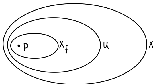
FIGURE 16.2. Visual aid for the proof of Theorem 16.2.2
