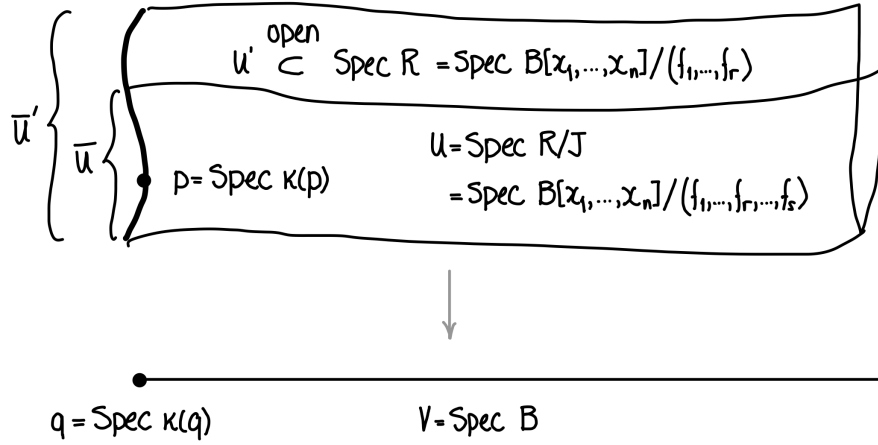
FIGURE 24.8. Geometry behind part of the proof of Theorem 24.8.8
