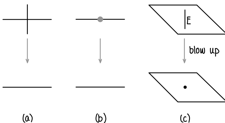
FIGURE 24.2. Morphisms that are not flat (Exercise 24.1.L)
