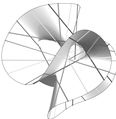
FIGURE 27.1. The twenty-seven lines on the Clebsch cubic surface (from Greg Egan)
