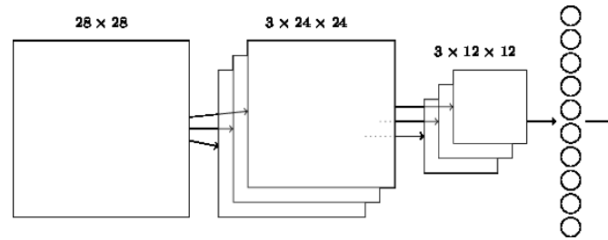
Figure 9.18: A simple CNN of three feature maps, to classify MNIST digits.
