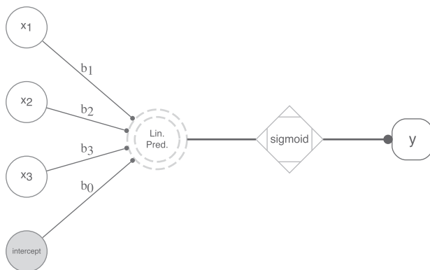
Figure 16.2: Logistic Regression Model
