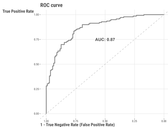
Figure 4.2: ROC curve and AUC value.
