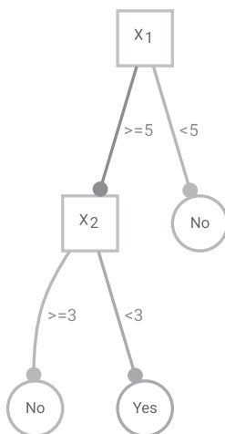
Figure 11.2: Simple classification tree.
