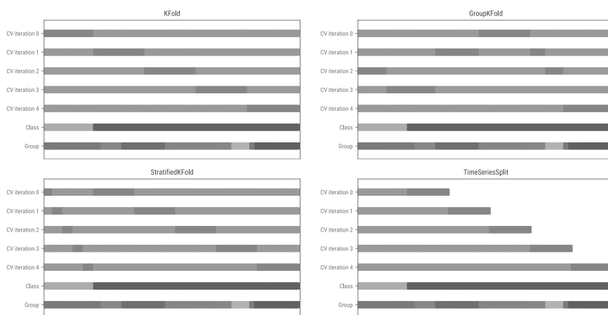
Figure 10.6: Comparison of cross-validation strategies.
