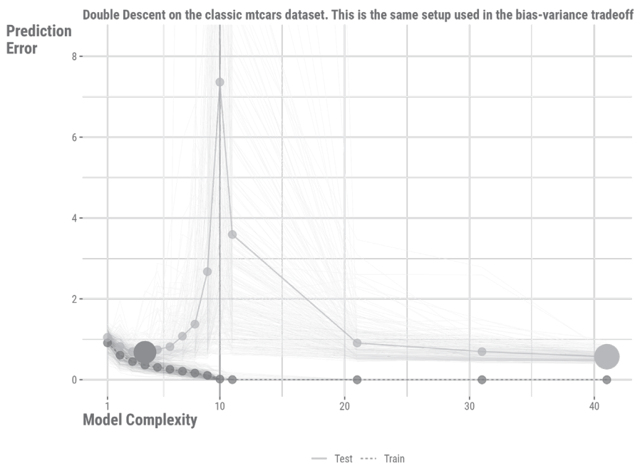
Figure 10.2: Double descent on the classic mtcars dataset.
