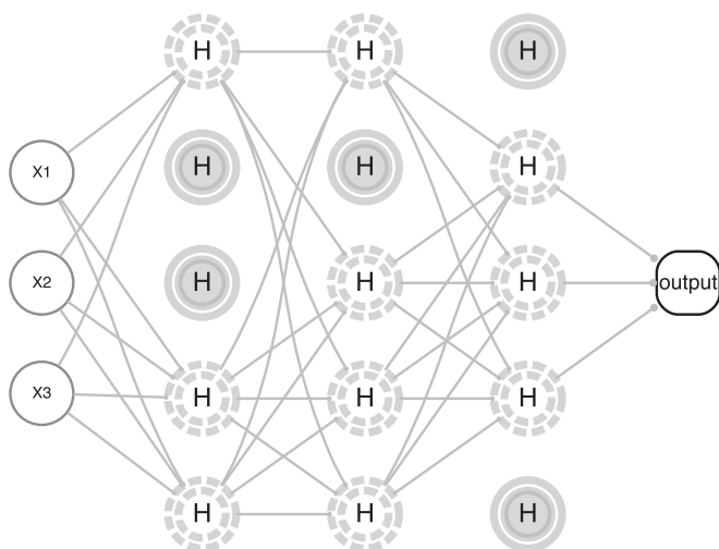
Figure 10.4: Neural network with dropout.
