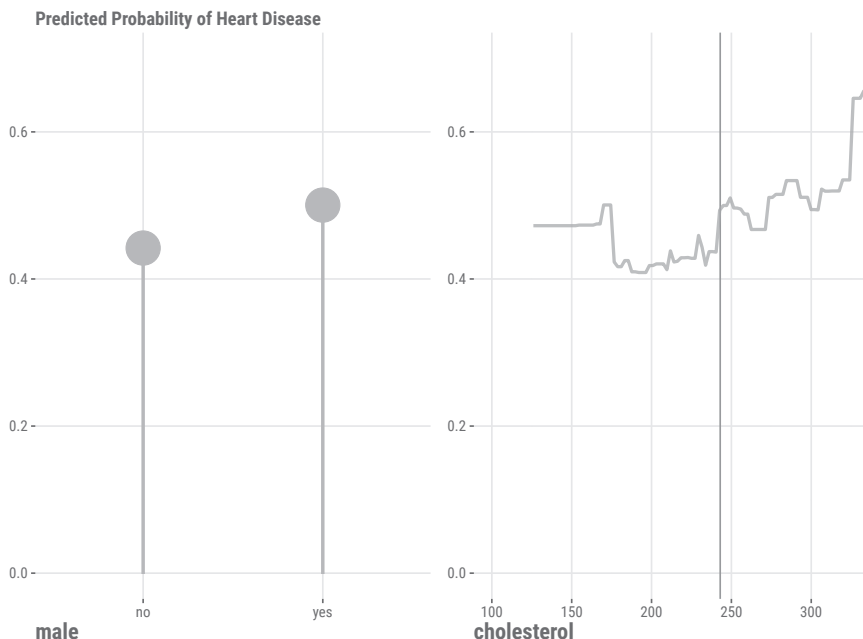
Figure 11.8: Partial dependence plot for cholesterol.
