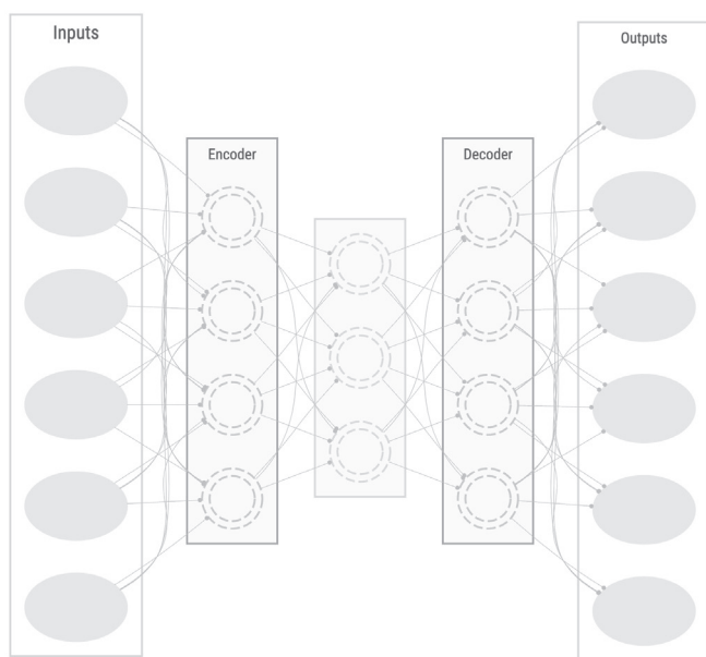
Figure 12.3: Conceptual diagram of an autoencoder.
