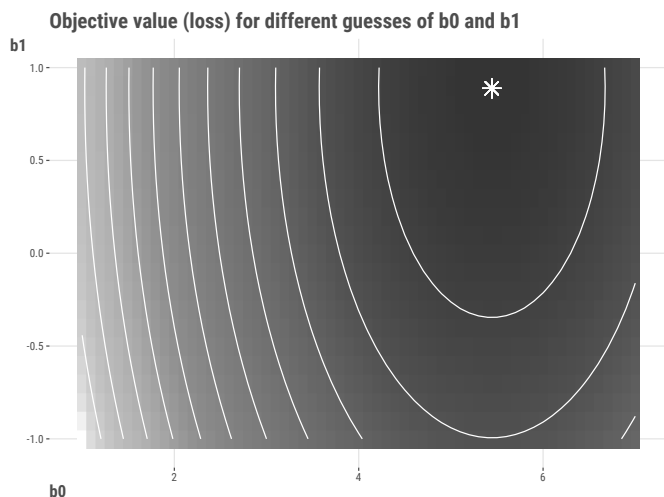
Figure 6.2: Results of parameter search.
