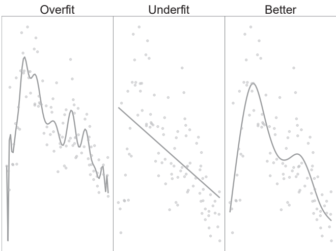
Figure 10.3: Overfitting and underfitting.
