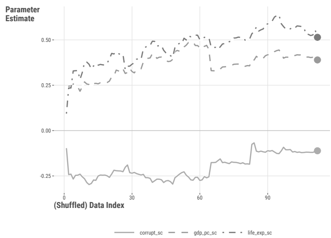
Figure 6.8: Stochastic gradient descent path.
