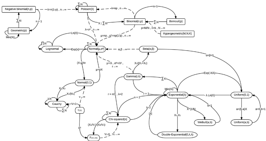
Figure 6.3: Relationships among some probability distributions.
