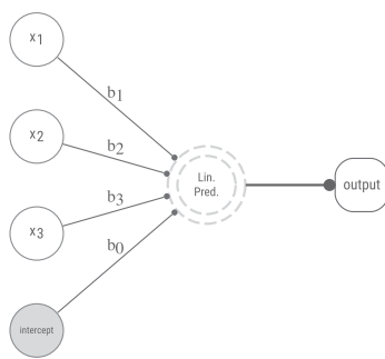
Figure 3.2: Linear regression as a graphical model.
