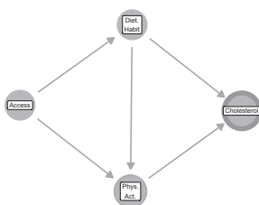
Figure 13.4: Causal DAG.
