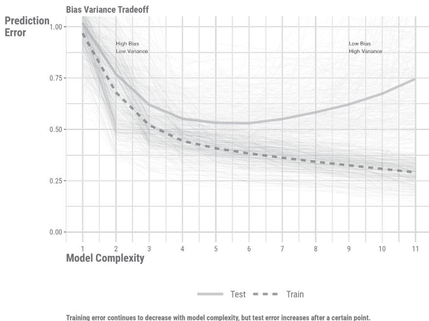
Figure 10.1: Bias-variance tradeoff.
