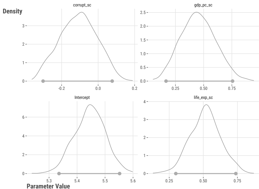
Figure 7.1: Bootstrap distributions of parameter estimates.
