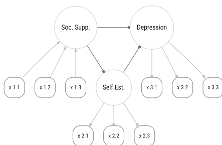
Figure 13.5: SEM with latent and observed variables.
