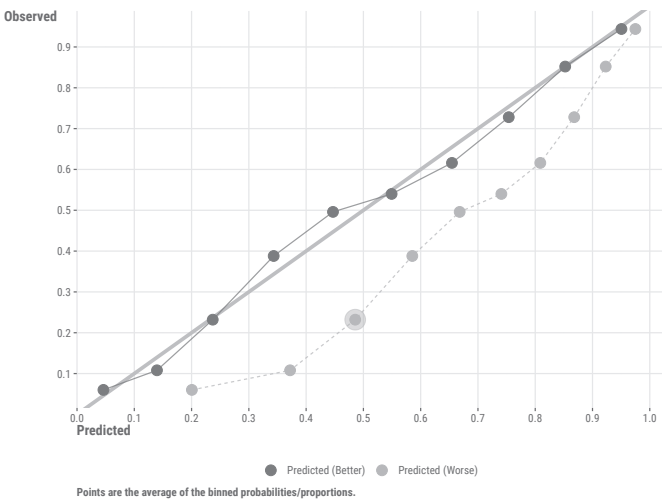
Figure 14.5: Calibration plot.
