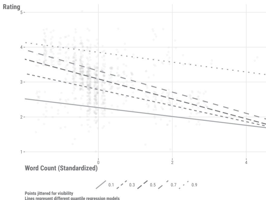
Figure 9.13: Quantile regression lines.
