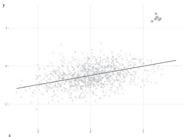
Figure 9.11: Linear relationship with extreme scores.
