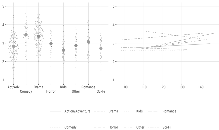
Left Plot: Group Means by Genre Right Plot: Length Slopes by Genre
