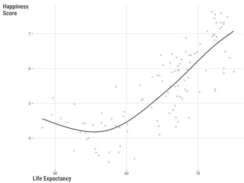
Figure 9.8: Curvilinear relationship.
