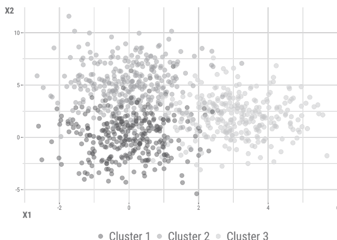
Figure 12.1: Two variables with three overlapping clusters.
