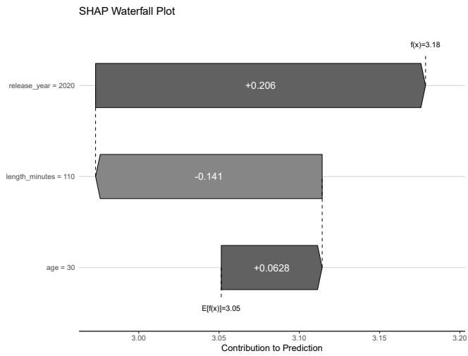
Figure 5.2: SHAP waterfall plot.
