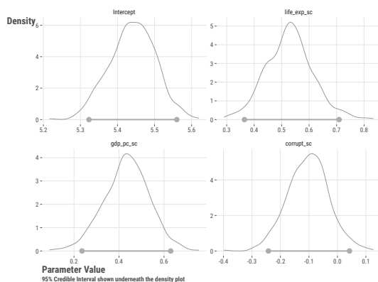
Figure 7.3: Posterior distribution of parameters.
