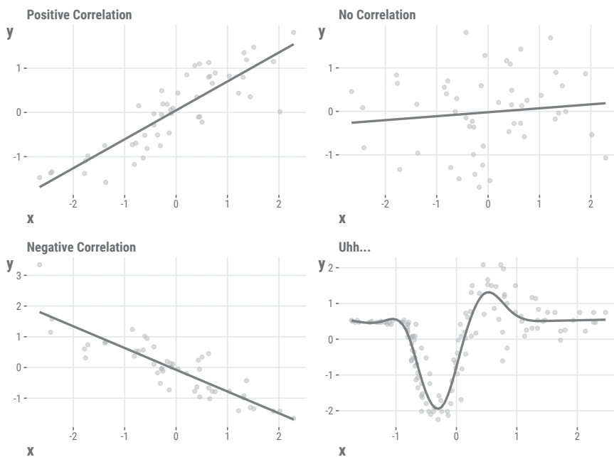
Figure 2.1: Correlation.
