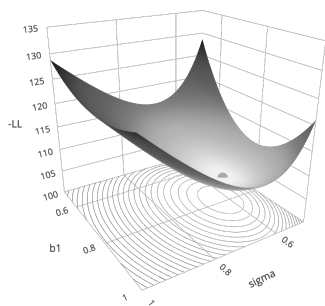
Figure 6.5: Likelihood surface for two parameters.
