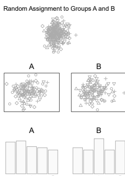
Figure 13.2: Random assignment.
