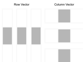
Figure B.2: Row and column vectors.
