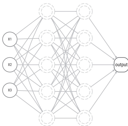
Figure 11.3: Neural network.
