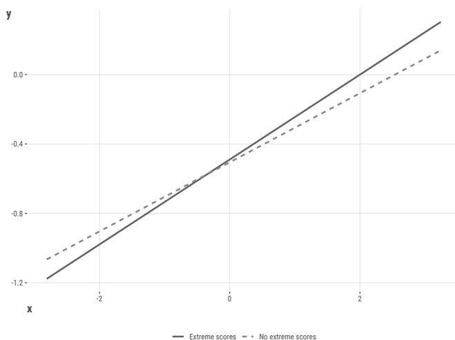
Figure 9.12: Linear relationships with and without extreme scores.
