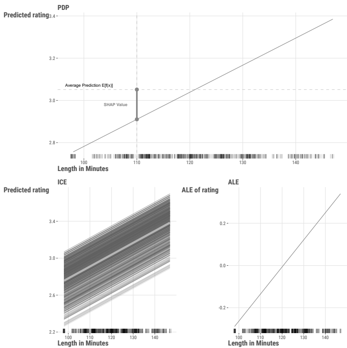
Figure 5.3: PDP, ICE, and ALE plots.
