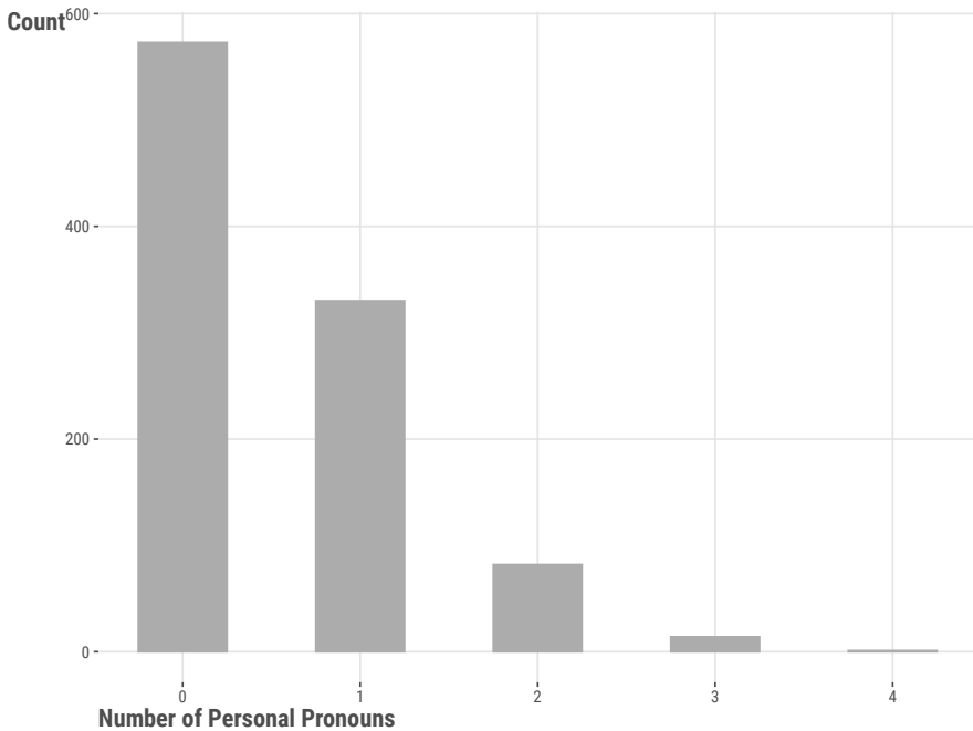
Figure 8.6: Distribution of personal pronouns seen across reviews.
