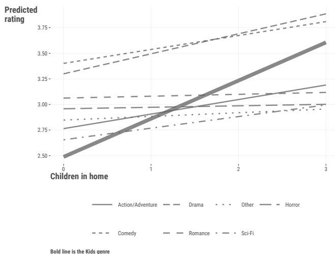
Figure 9.1: Interaction plot.
