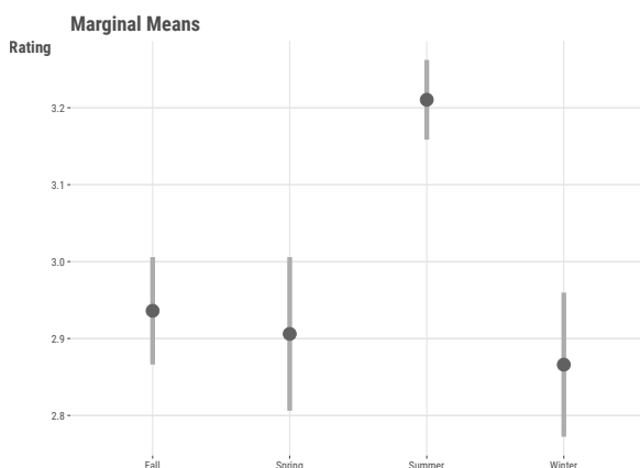
Figure 3.6: Marginal effects of season on rating
