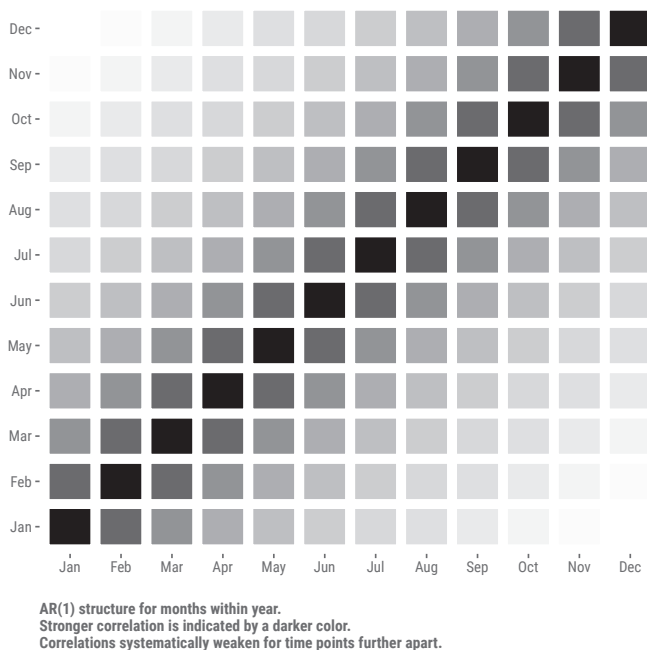
Figure 14.10: AR (1) covariance structure visualized.
