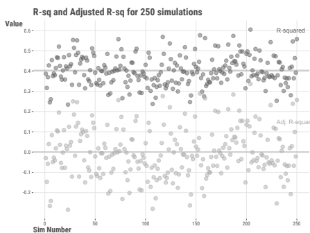
Figure 15.1: The problem of R^2 .
