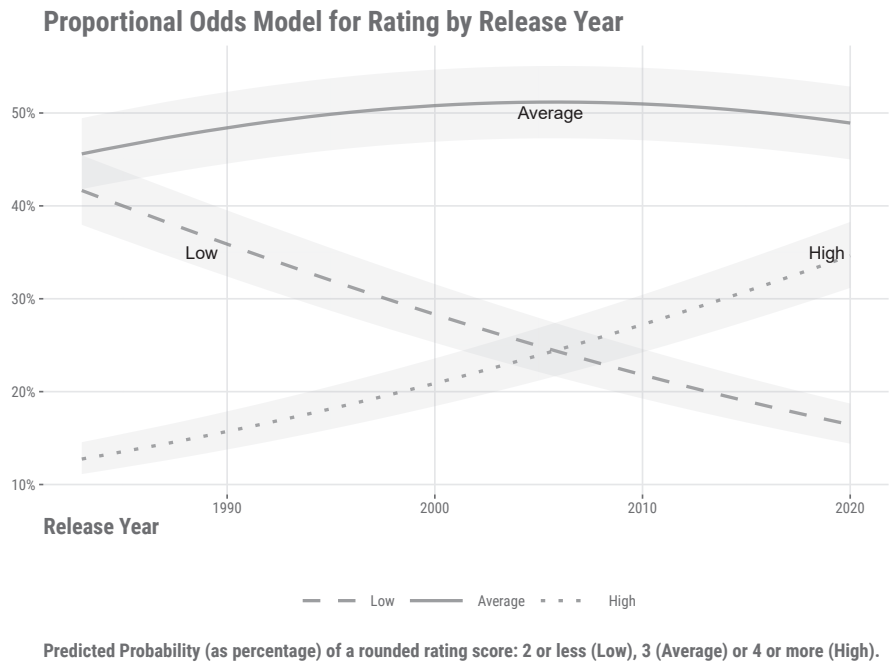
Figure 14.3: Proportional odds model for rating by release year.
