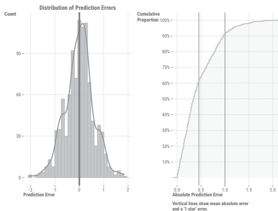
Figure 3.4: Distribution of prediction errors.
