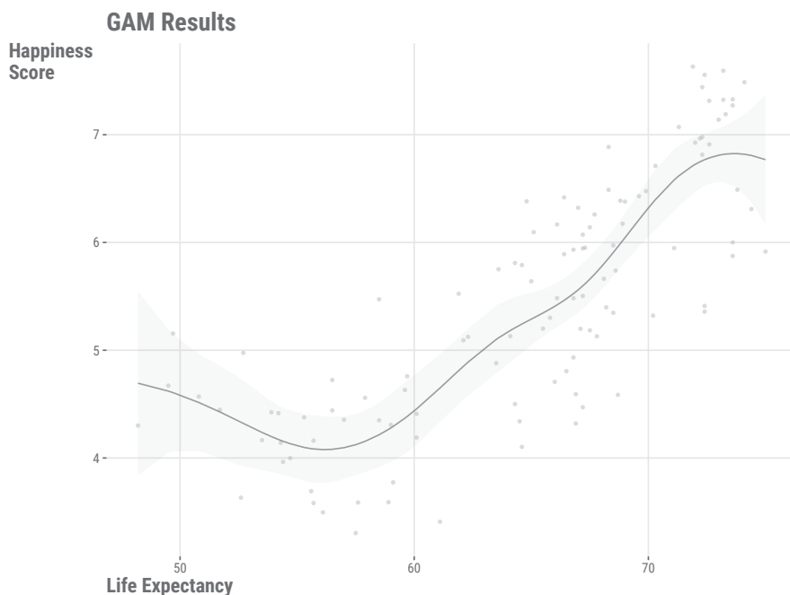
Figure 9.9: Visualizing a GAM.
