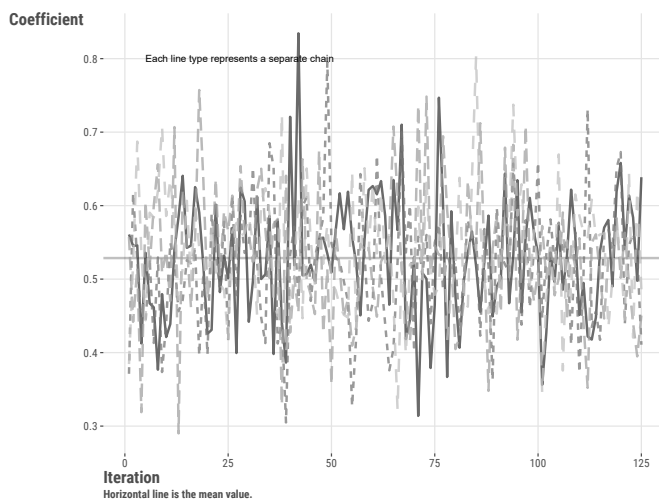
Figure 7.4: Bayesian chains for life expectancy coefficient.
