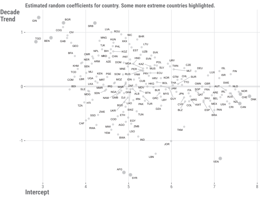
Figure 9.6: Random effects for a mixed model.
