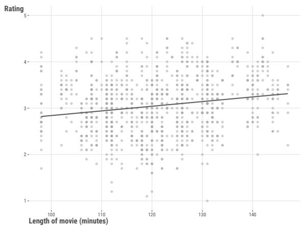
Figure 9.2: Linear relationship between length of movie and rating.
