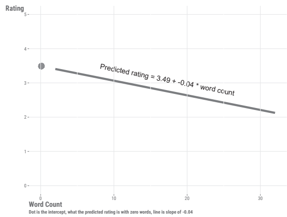
Figure 3.1: Linear regression of rating vs. word count
