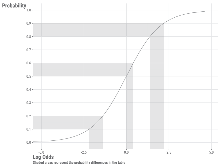
Figure 8.3: Comparison of probability and odds differences.
