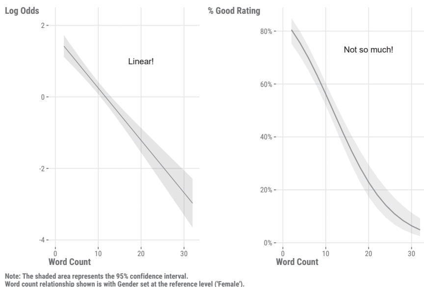
Figure 8.4: Model predictions for word count feature.
