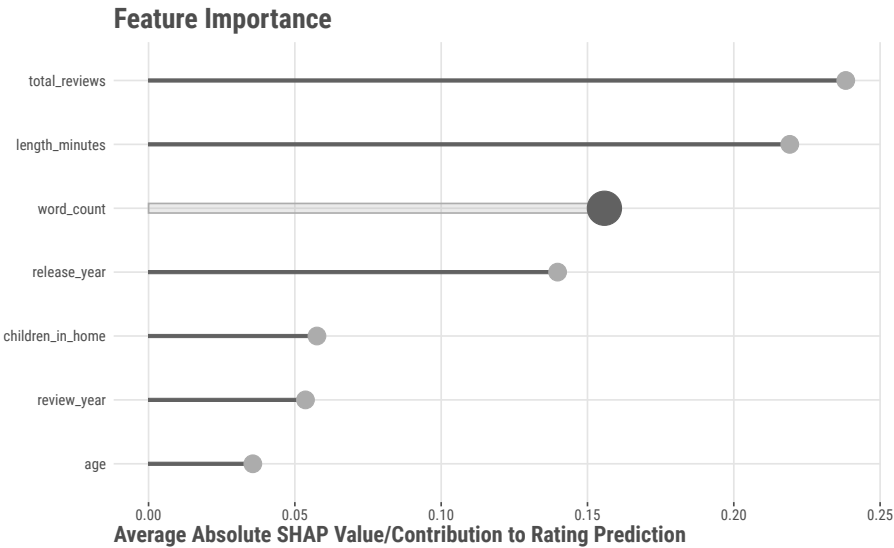
Figure 5.5: SHAP importance.
