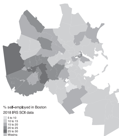
Figure 12.6: Spatial Demographic Data (code available from Kyle Walker)
