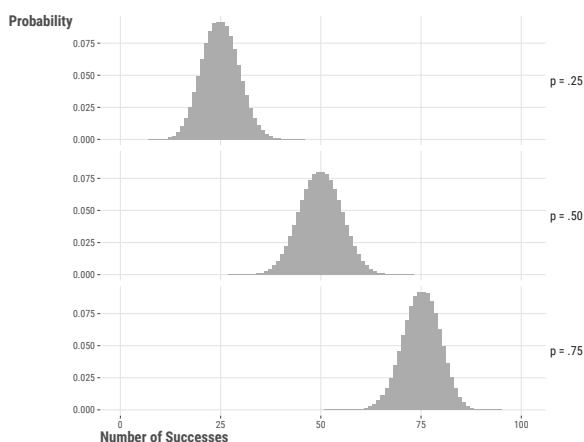
Figure 8.1: Binomial distributions for different probabilities.
