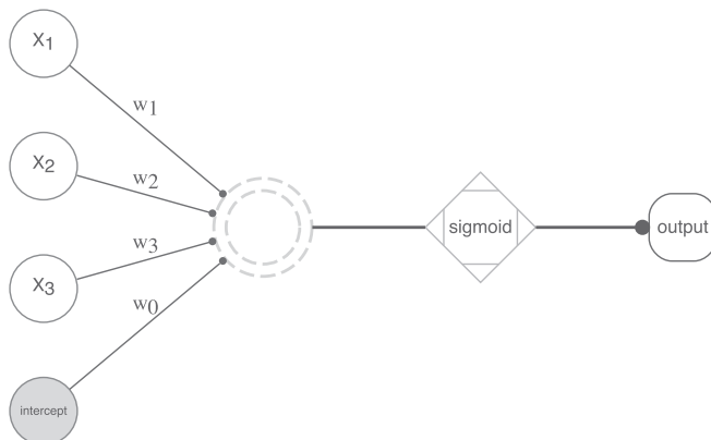
Figure 3.7: Linear model with transformation can be a logistic regression
