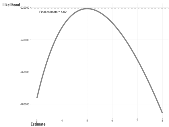
Figure 6.4: Likelihood function for one parameter.
