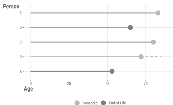
Figure 14.6: Censoring for time until death.
