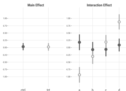
Figure 15.3: Main effect vs. interaction.
