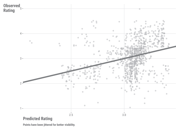
Figure 3.3: Predicted vs. observed ratings.
