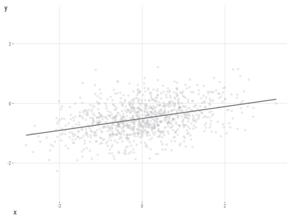
Figure 9.10: Linear relationship without extreme scores.
