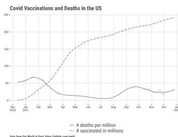
Figure 13.3: Covid vaccinations and deaths in the US.
