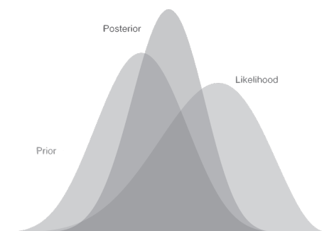
Figure 7.2: Prior, likelihood, and posterior distributions.
