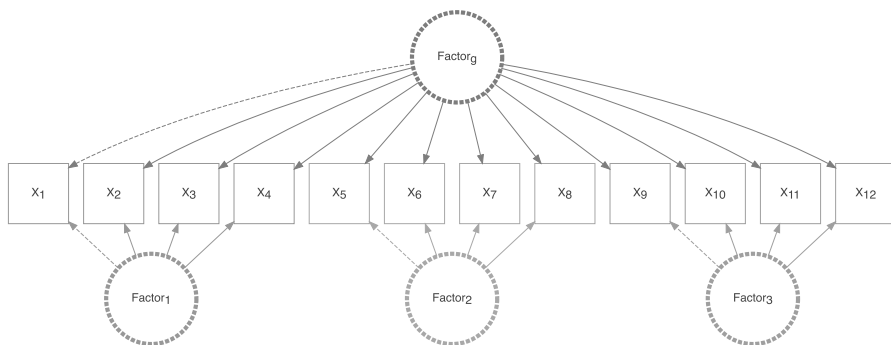
Figure 14.12: Latent variable model (bifactor).
