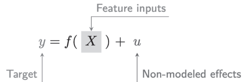
Figure 2.2: Generic model.
