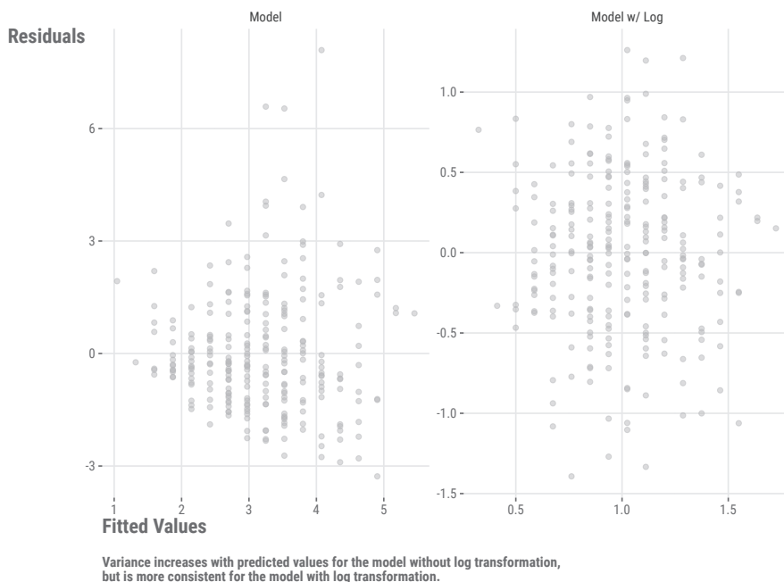
Figure 14.1: Log transformation and heteroscedasticity.
