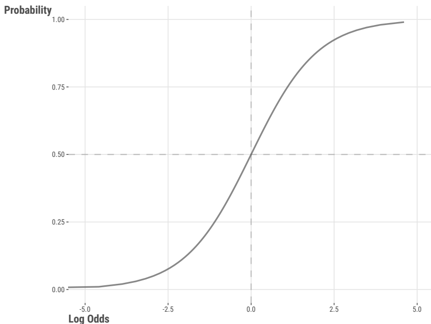
Figure 8.2: Log-odds and probability values.
