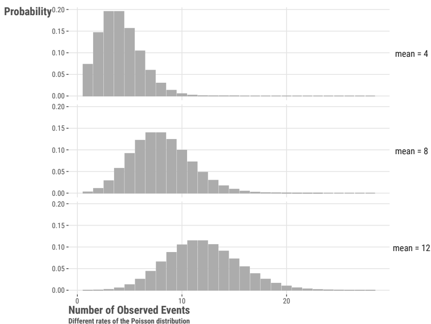
Figure 8.5: Poisson distributions for different rates.
