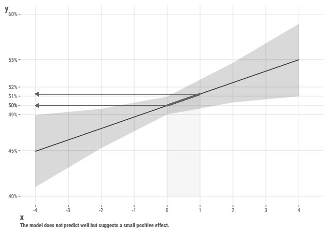
Figure 13.1: Results from a hypothetical causal model.
