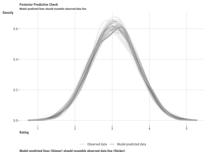
Figure 4.6: Bayesian posterior predictive check for a regression model.
