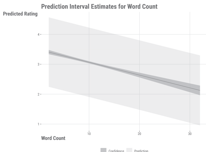
Figure 3.5: Prediction and confidence intervals compared.
