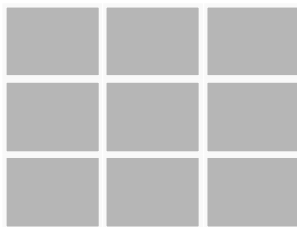
Figure B.3: Matrix.
