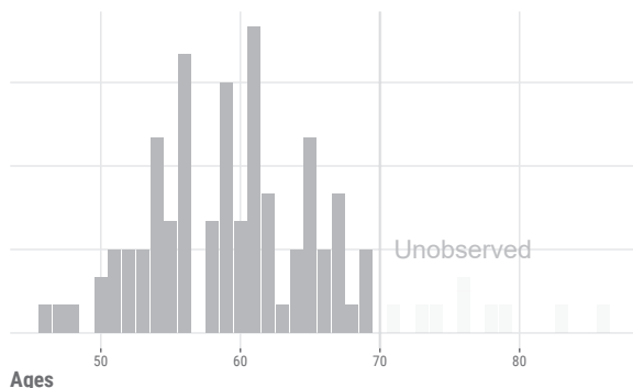
Figure 14.7: Truncation.
