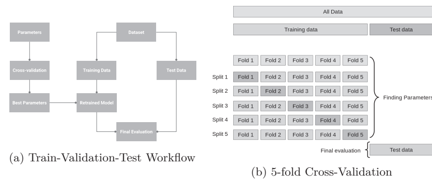
Figure 10.7: A tuning workflow.
