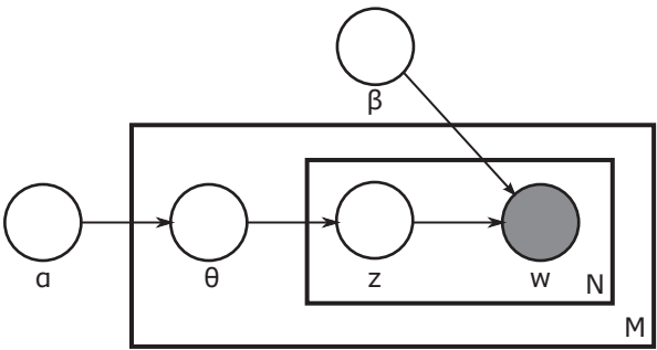
Figure 16.3: Plate Notation for Latent Dirichlet Allocation
