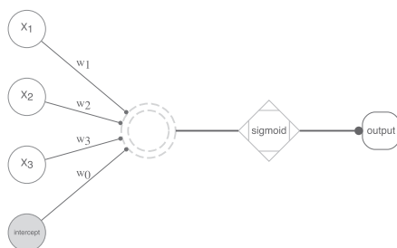
Figure 11.6: Logistic regression as a neural network with a single hidden layer with one node, and sigmoid activation
