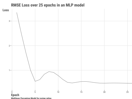
Figure 4.4: MSE loss over 25 epochs in an MLP model.
