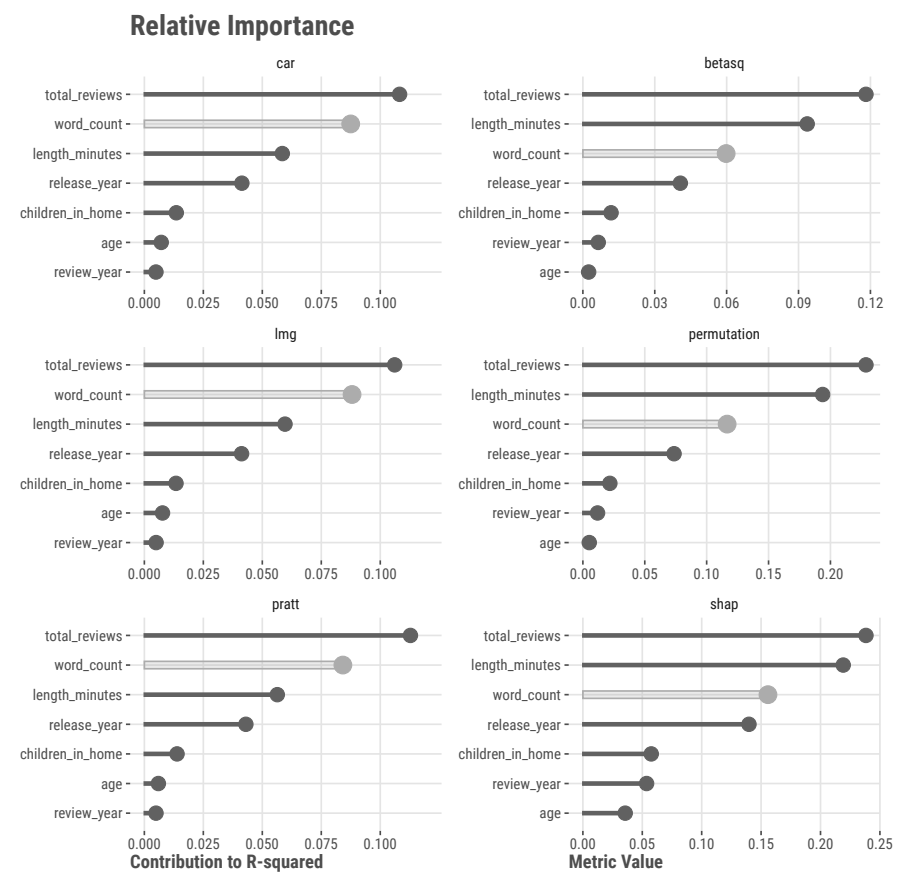
Figure 5.6: Feature importance by various methods.
