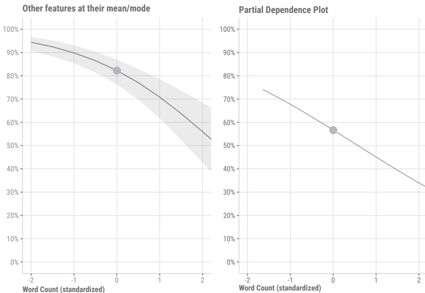
Figure 5.1: Marginal effect at the mean vs. partial dependence plot.
