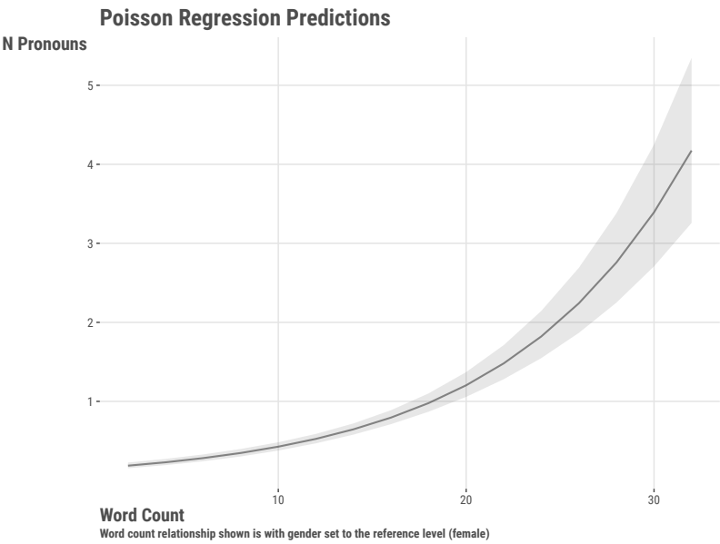
Figure 8.7: Poisson model predictions for word count feature.
