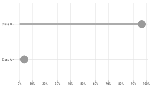
Figure 14.4: Class imbalance.
