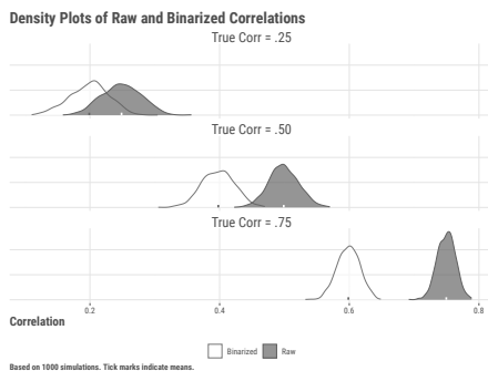
Figure 15.2: Density plots of raw and binarized correlations.
