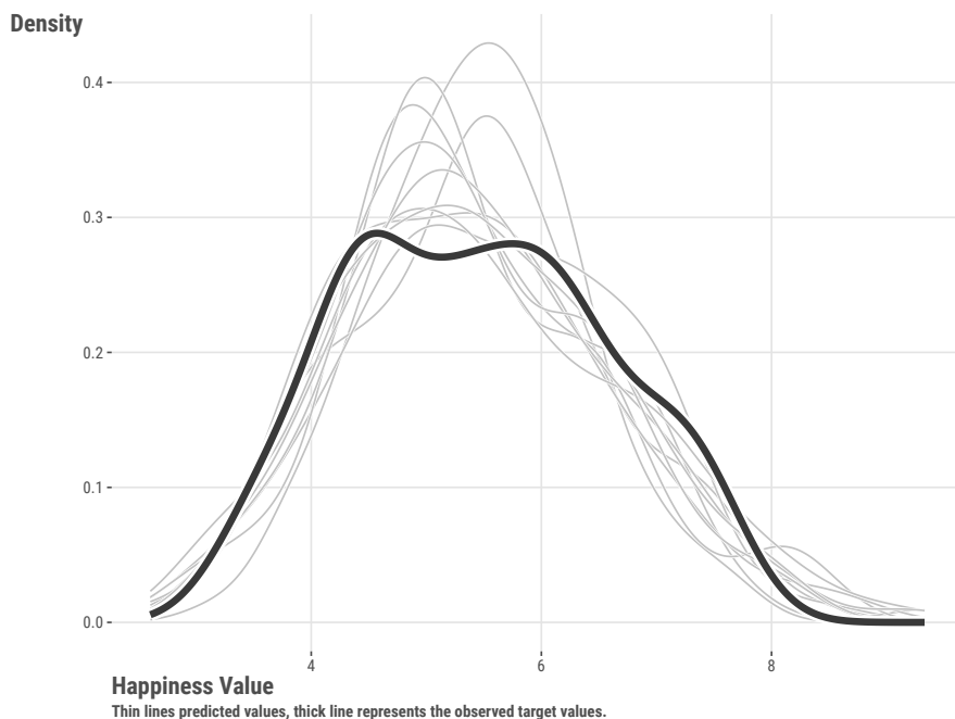
Figure 7.5: Posterior predictive distribution of happiness values.
