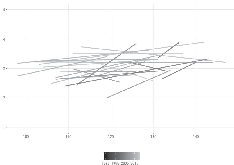
Figure 9.4: Release year effects on length and rating.
