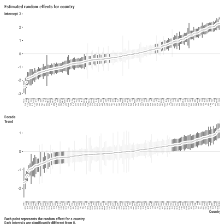
Figure 9.5: Estimated random effects.
