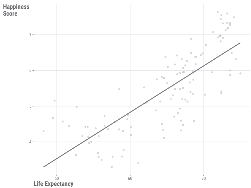
Figure 9.7: Standard linear relationship.
