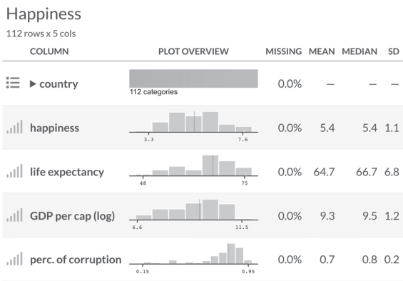
Figure 6.1: World happiness data summary.
