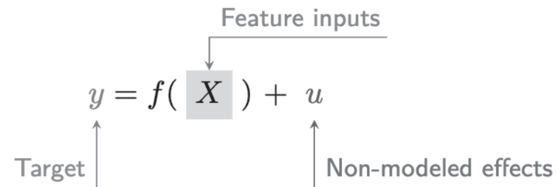
Figure 16.1: Generic model.
