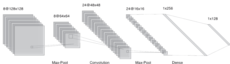
Figure 12.8: Convolutional neural network LeNet 4 .
