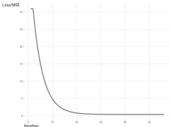
Figure 6.7: Loss with gradient descent.
