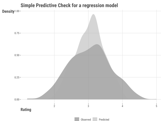
Figure 4.5: Predictive check for a regression model.
