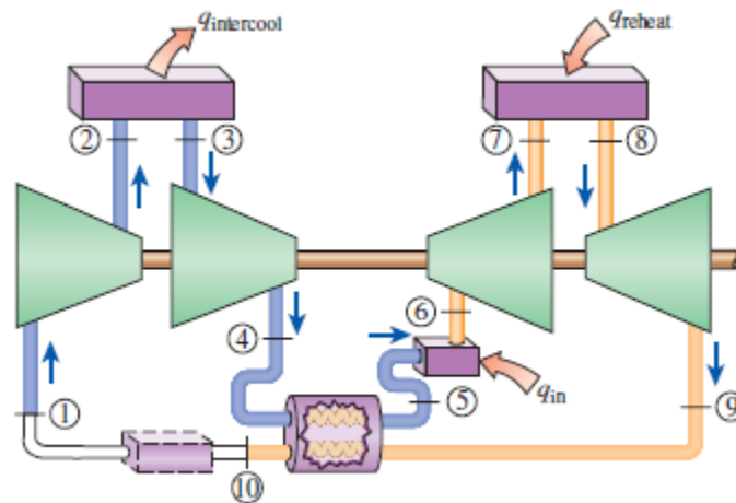
FIGURE P10-130E
