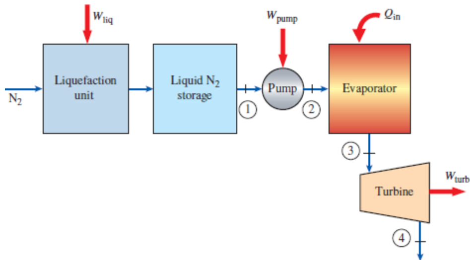
FIGURE P5-191
