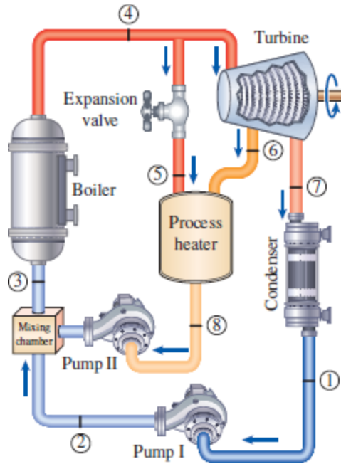
A cogeneration plant with adjustable loads.
