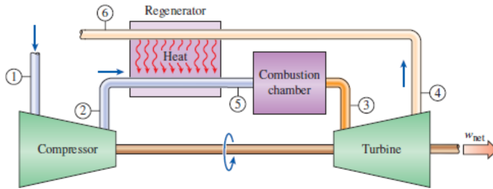
FIGURE 10-40
