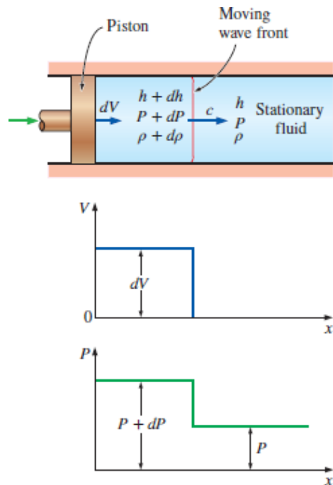
Propagation of a small pressure wave along a duct.
