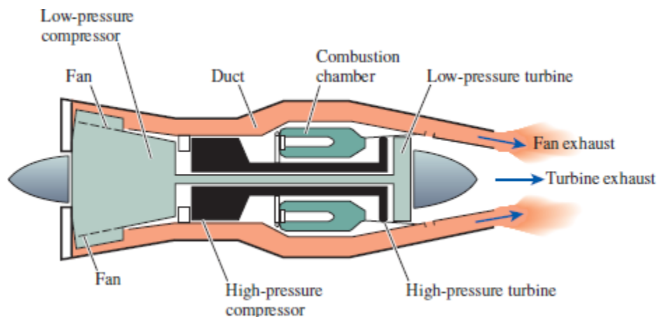
FIGURE 10-54 A modern jet engine used to power Boeing 777 aircraft. This
