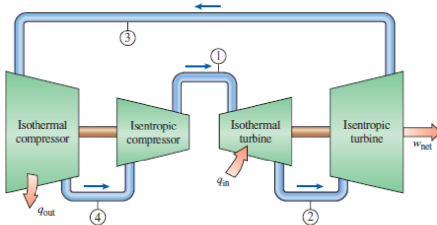
FIGURE 10-6 A steady-flow Carnot engine.
