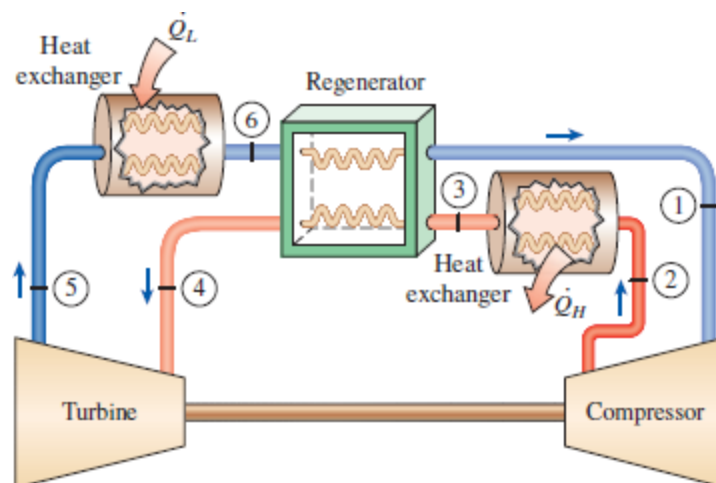
FIGURE P12-125
