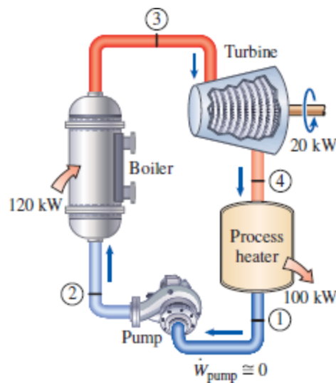
An ideal cogeneration plant.
