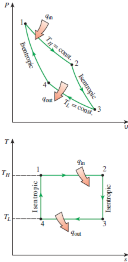
FIGURE 10-6 A steady-flow Carnot engine.
