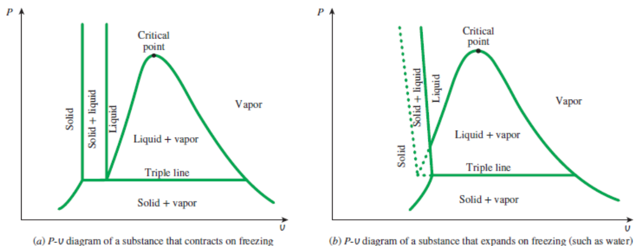
FIGURE 3-19 P - v diagrams of different substances.
