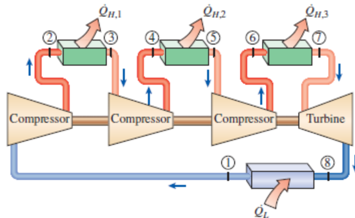
FIGURE P12-126
