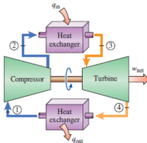
A closed-cycle gas-turbine engine.
