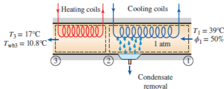
FIGURE P15-87
