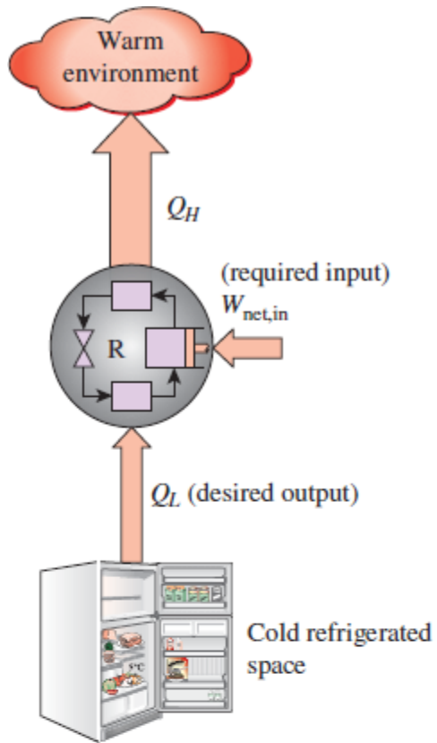
(a) Refrigerator
