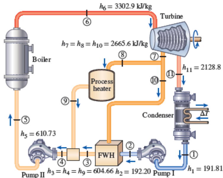
FIGURE P11-129
