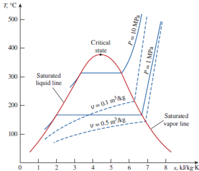
FIGURE 7-11 T-s diagram for water.
