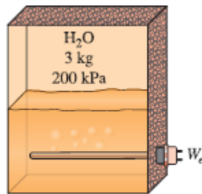
FIGURE P7-36
