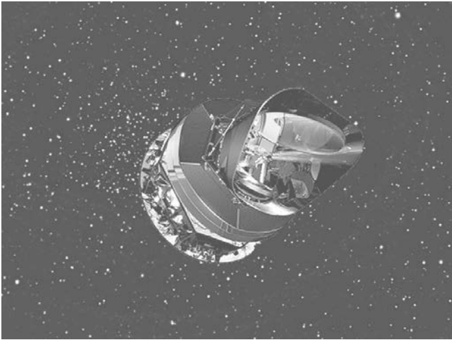
Figure 9.2 The Planck satellite.
