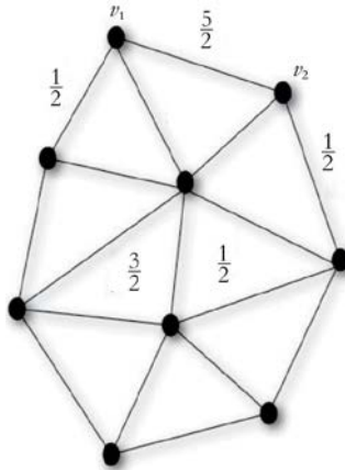
Figure 6.4 A spin network
