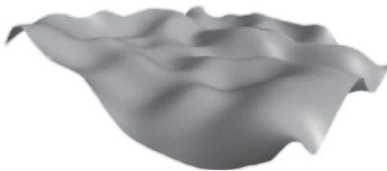
Figure 3.7 A curved (bidimensional) surface.
