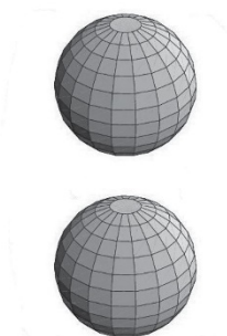
Figure 3.12 A 3-sphere can be represented as two balls joined together.
