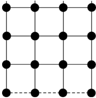
Figure 7.6 A grid approximating physical spacetime.
