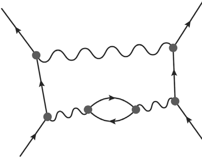
Figure 7.5 A Feynman diagram.
