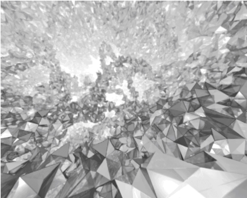
Figure 13.1 An intuitive representation of quantum gravity.
