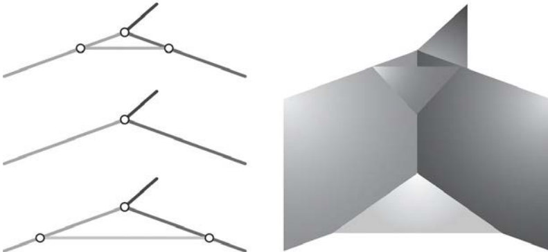
Figure 7.2 An evolving spin-network: three nodes combine into a single node, and then separate again. On the right, the spinfoam representing this process.
