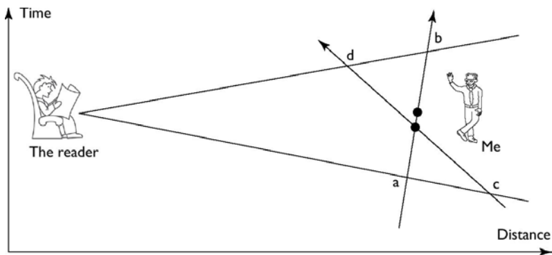
Figure 3.3 The relativity of simultaneity.
