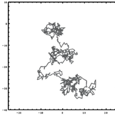
Figure 1.4 Typical Brownian motion.
