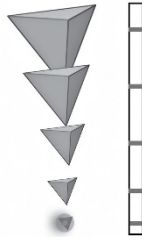
Figure 6.2 The spectrum of the volume: the volumes of a regular tetrahedron that are possible in nature are limited in number. The smallest, at the bottom, is the smallest volume in existence.
