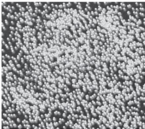
Figure 4.5 Light is a wave on a field, but it has also a granular structure.
