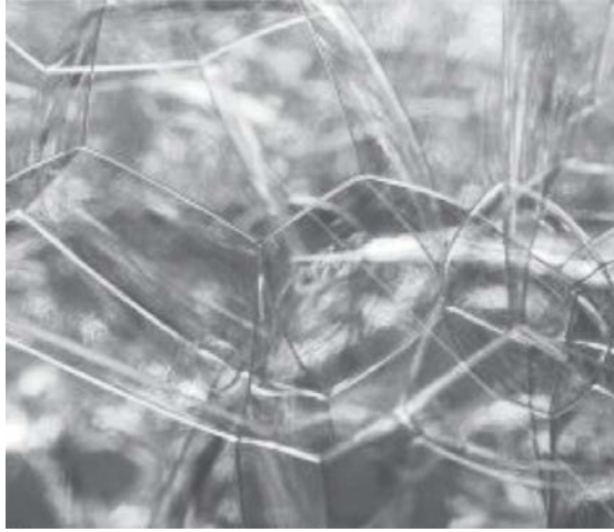
Figure 7.3 The foam of soap bubbles.
