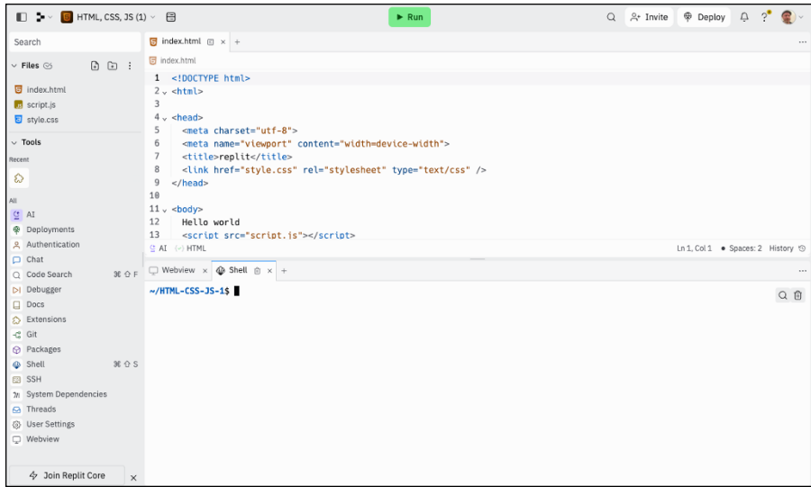
FIGURE 3-15: Rearranging panes.
