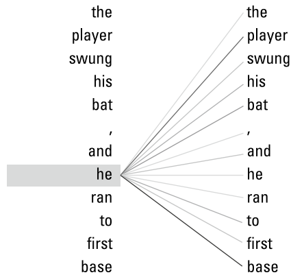
FIGURE 2-8: Visualizing self-attention.
