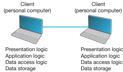
FIGURE 2.7 Peer-to-peer architecture
