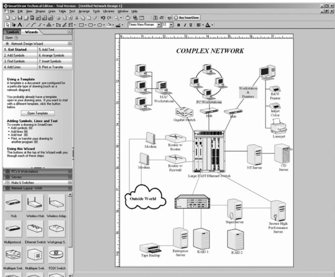
FIGURE 11.17 SmartDraw software
