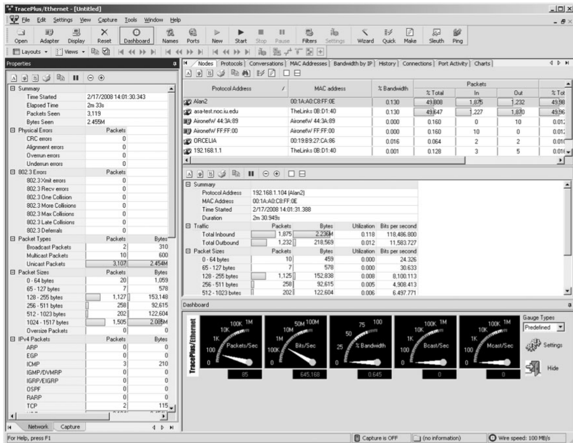
FIGURE 6.13 Trace plus
