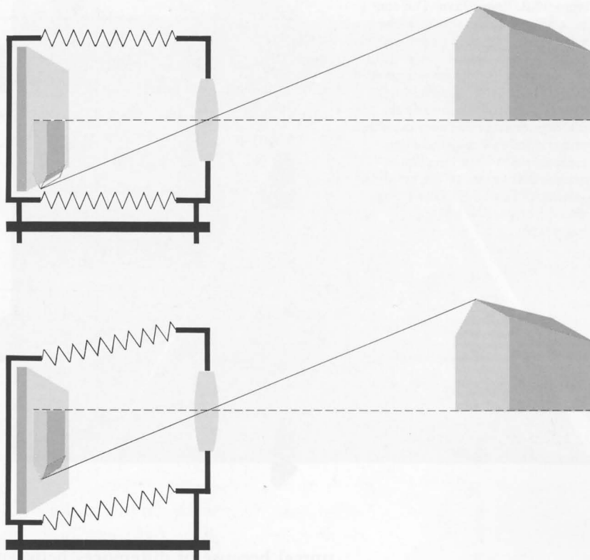
Figure 10-2. Effect of rising front. The rising front adjustment can be used to alter the position of the image within the borders, while keeping the lensboard and film plane parallel. The drawing shows the image of a subject repositioned through this lens shift. Since the subject is rectangular, tilting the camera to include the top of the structure would cause convergence; if the camera back is kept vertical and the rising front adjustment used, no convergence will occur. The same principle applies (in reverse) with the falling back, if available, and to the use of the sliding front and back. However, the rising front and sliding front move the lens, and the relationship of near and far subjects will change.
