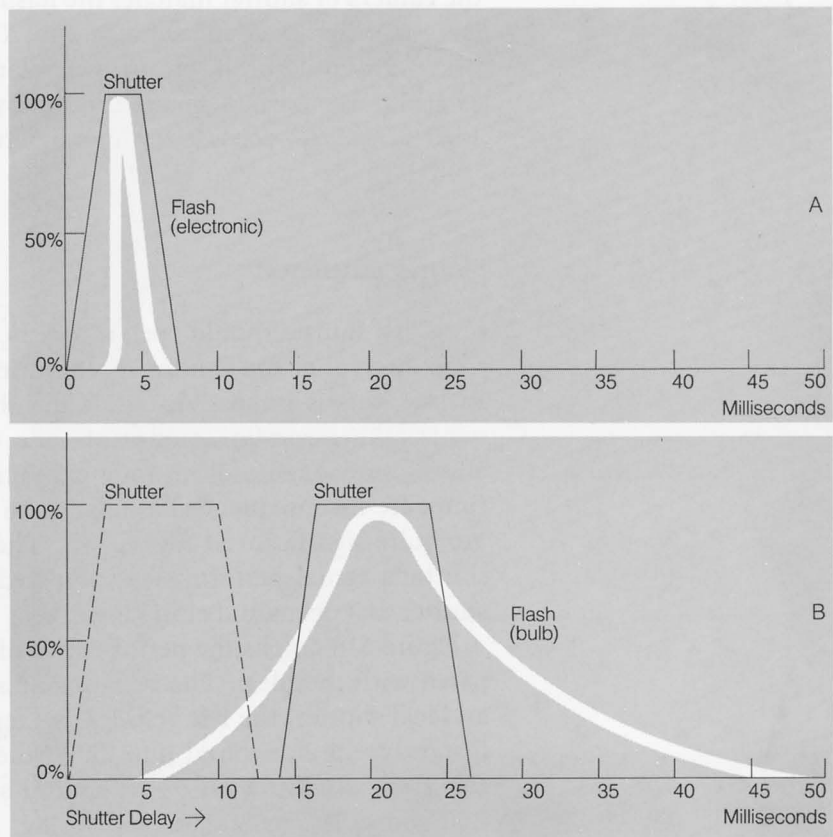
Figure 6-7. Flash synchronization.
