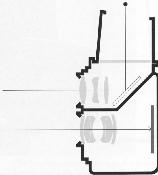
Figure 3-3. Twin-lens reflex camera, cross section. Separate lenses of identical focal length are used to form the viewing and picture-making images. The two lenses are contained in a single focusing mount so that, when the viewing lens focuses the subject on the ground glass, the primary lens focuses it at the film plane. The image seen on the ground glass is reversed left-to-right because of the mirror. As the viewing lens is a few inches above the taking lens, parallax is unavoidable.
