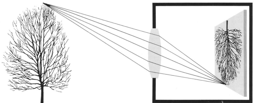
Figure 5-2. Image formation by a simple lens. Light from a subject point falling on any part of the lens surface is focused at a single point behind the lens, and the total image is the accumulation of all such points. By comparing this illustration with Figure 1-2, the effect of replacing a pinhole with a lens can be seen. The lens “gathers” light over its entire surface, producing a much brighter image, and it focuses the light to produce a sharper image than the pinhole.
