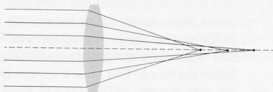
Figure 5-24. Spherical aberration.
