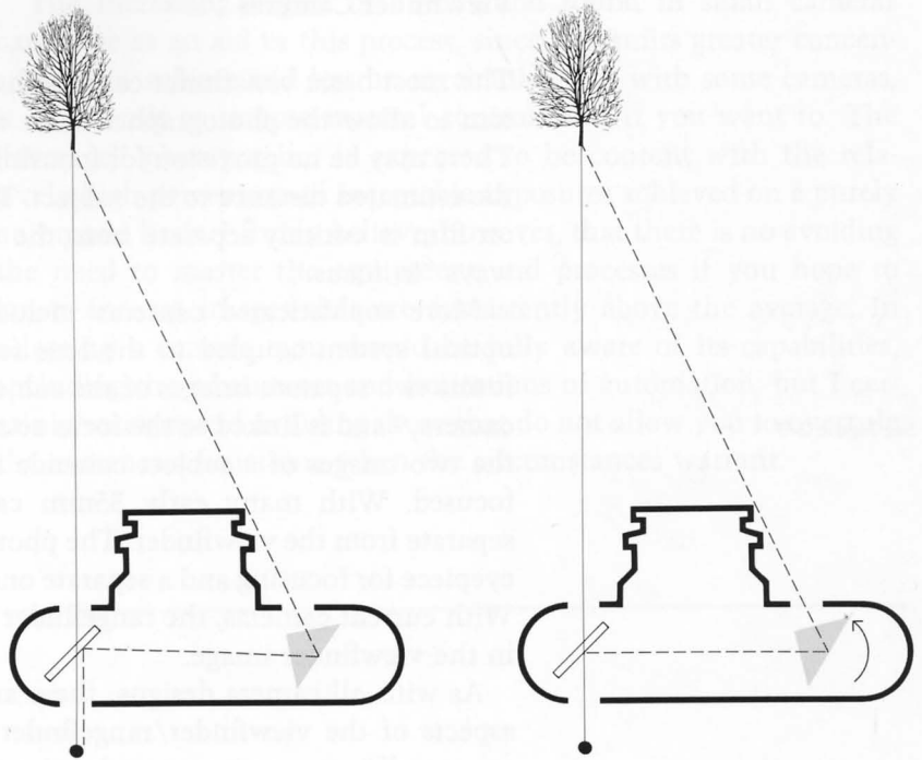
Figure 2-3. Rangefinder optical system. The viewfinder image, seen through the window at the left end of the camera, includes a small superimposed rangefinder area controlled by the prism at the right. The prism is coupled with the lens focus setting and rotates in such a way that the image it forms comes into alignment with the primary viewing image when the focus is correct. The structure may differ with different makes, but the principle remains the same. The greater the distance between the rangefinder windows (sometimes referred to as the rangefinder base length), the more accurate the system is likely to be.
