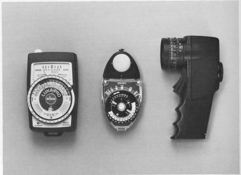
Figure 11-2. Exposure meters. The three general types of exposure meter are, from left, the general-purpose reflected light meter, the incident light meter, and the spot meter.
