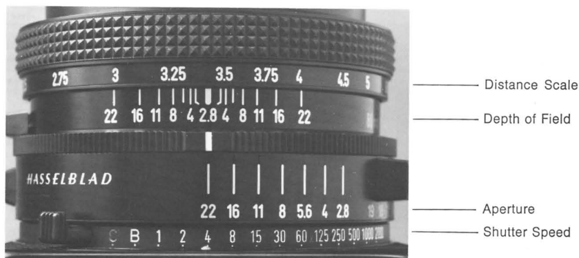
Figure 5-7. Depth-of-field scale. The top row of numbers is the distance scale, and immediately below it is the depth of field scale. The aperture numbers appear in pairs on either side of the mark indicating optimum focus. Numbers on the distance scale that lie between the pair corresponding to the aperture chosen are within the depth of field region; the image is acceptably sharp within these limits. In this case, the optimum focus is at about 3.4 feet, and depth of field extends from 3 feet to 4 feet at f/22 .
