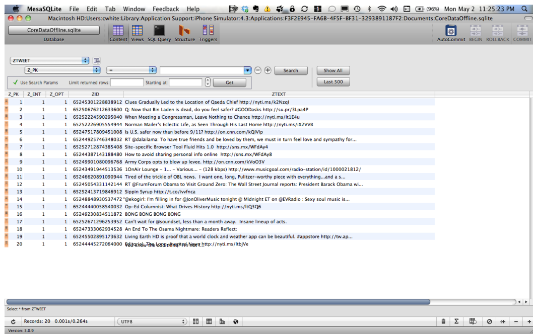
Figure 10–11. The Core Data SQLite database
