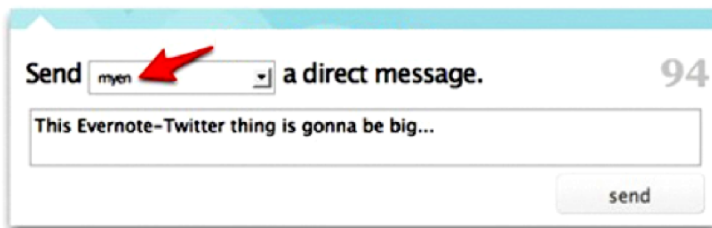
Figure 11–3. Tweeting @MyEN
