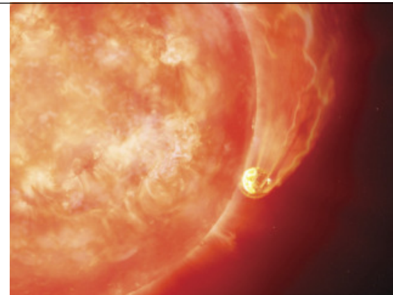
▲ Astronomers have observed the first compelling evidence of an aging Sun-like star engulfing an exoplanet.
