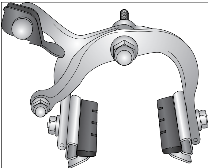
Figure 8-3: Center- mount brakes.
