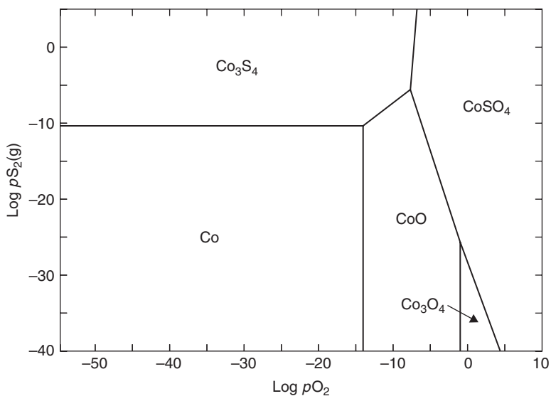
FIGURE 15.7 Stability diagram of the Co-S-O system at 870°C.
