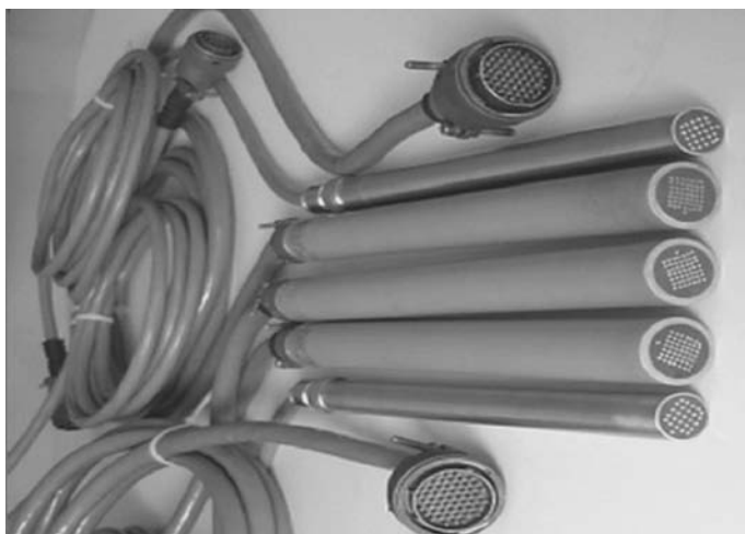
FIGURE 5.39 Typical CMAS probes used for real-time corrosion monitoring. (Courtesy of Corr Instruments, LLC)
