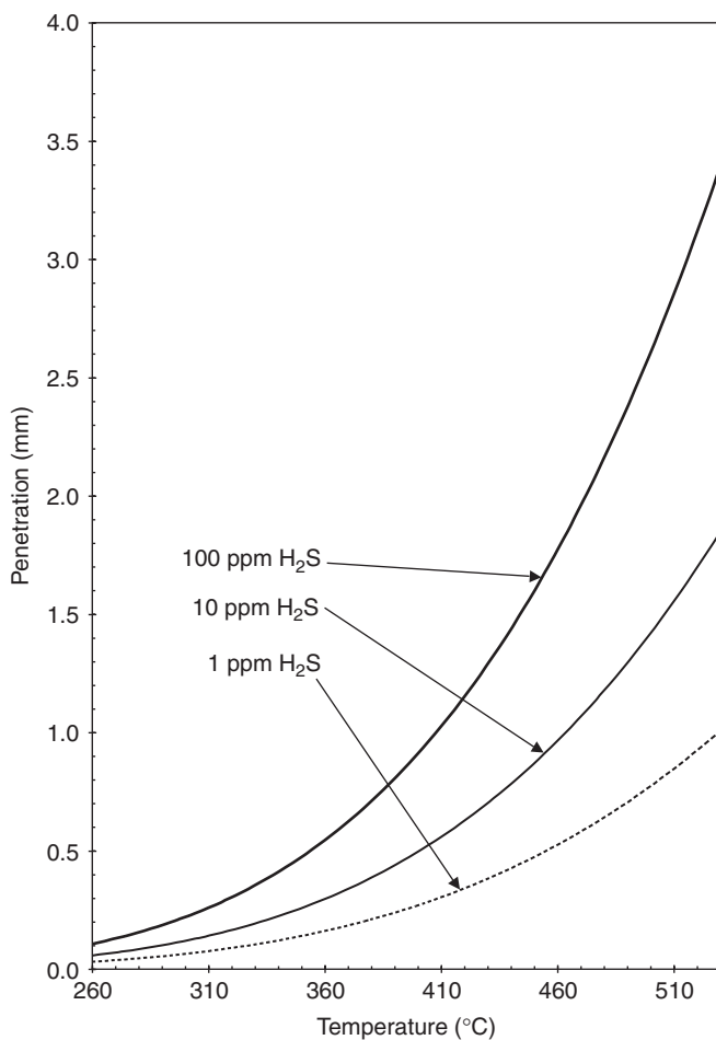
FIGURE 15.23 Effect of temperature upon sulfidation corrosion of S41000 after one year in \text{H}_2\text{-H}_2\text{S} gases at 34 atm.
