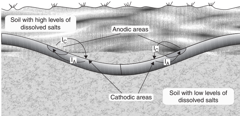
FIGURE 13.9 DC ( I_C ) and ( I_A ) flow, respectively, through earth from anodic area to cathodic area and through the pipe steel from cathodic area back to anodic area to complete the circuit. The anodic area, where current leaves the steel to enter the surrounding earth is where corrosion occurs.
