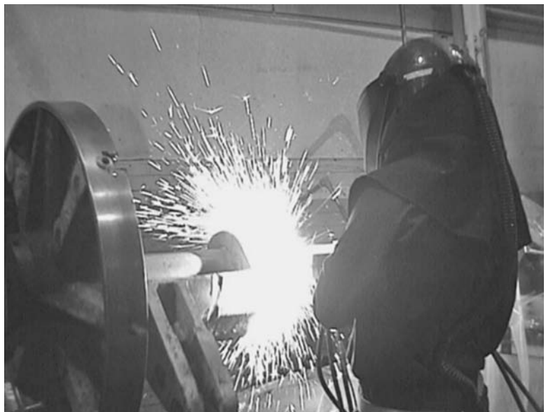
FIGURE 14.14 Arc-spraying process. (Courtesy of M. Gariepy, WEIR Engineering Services, Montreal, Canada)
