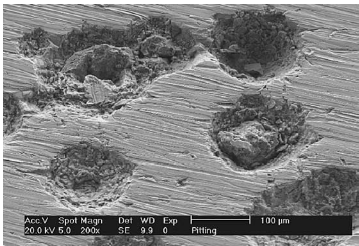
FIGURE 5.36 Scanning electron microscope image of a sensor element surface after exposure at the base of the scrubbing tower clearly showing corrosion pits.
