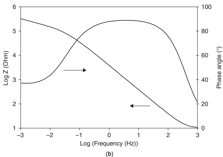
FIGURE 5.27 (a) Complex plane and (b) Bode plots of simulated data corresponding to model circuit in Fig. 5.25(b) where R_s = 10 \, \Omega , R_p = 100 \, \text{k}\Omega , C_{dl} = 40 \, \mu\text{F} and the exponent n of the Warburg component = 0.4.
