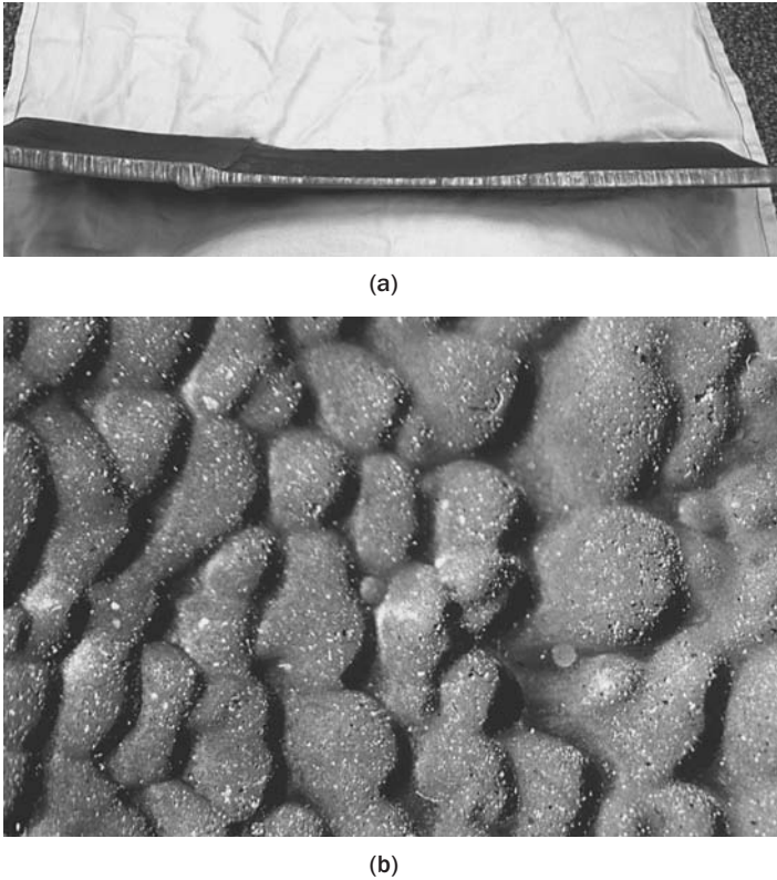
FIGURE 6.37 Pipe wall thinning (a) and corrosion patterns (b) caused by flow accelerated corrosion (FAC) inside a steam line. (Courtesy of Russ Green, TMI)
