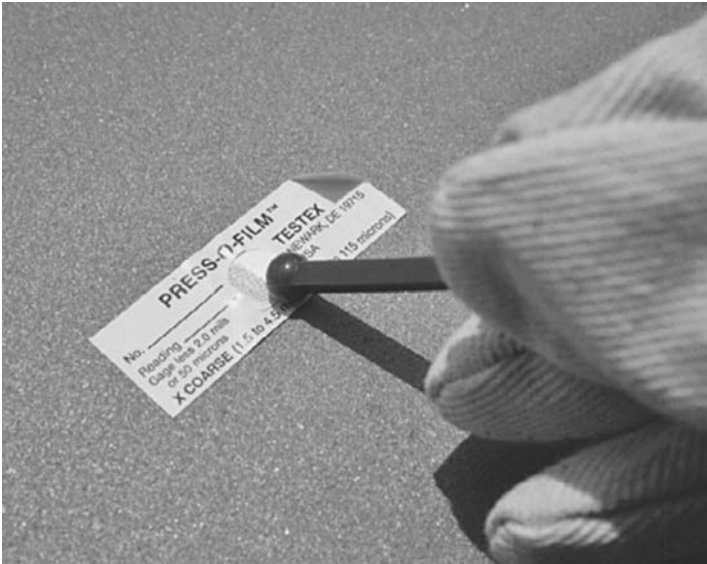
FIGURE 14.23 Burnishing Testex Press-O-Film replica tape. (Courtesy of KTA-Tator, Inc.)
