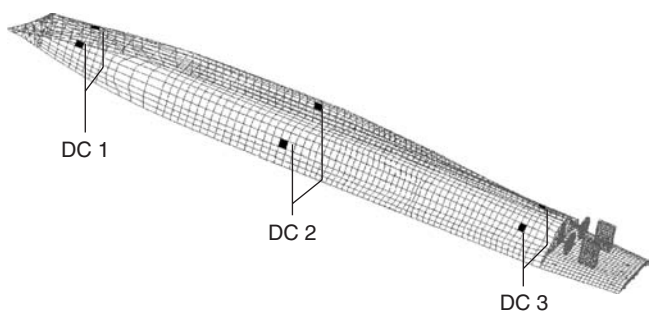
FIGURE 13.42 BE meshed ship hull with ICCP anode positions and power supplies. (Courtesy of Robert A. Adey, Computational Mechanics BEASY)
