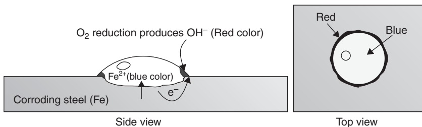
FIGURE 7.40 Ferroxyl drop experiment on a steel plate.
