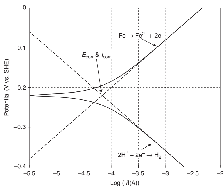
FIGURE 5.14 Polarization behavior of carbon steel in a deaerated solution maintained at 25°C and a pH of zero.
