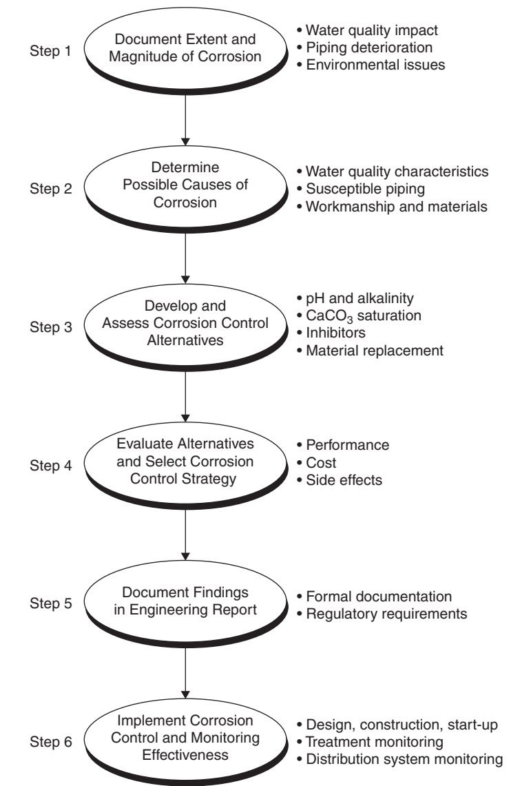
FIGURE 8.2 Corrosion control program implementation flowchart.
