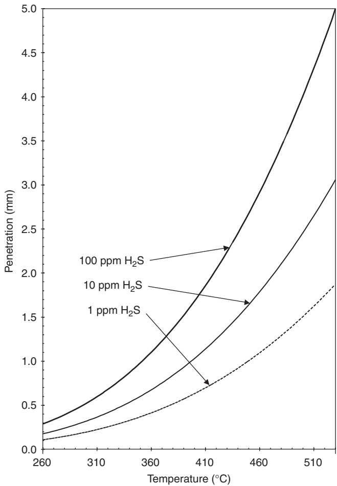
FIGURE 15.22 Effect of temperature upon sulfidation corrosion of 9 Cr 1 Mo after one year in H 2 -H 2 S gases at 34 atma.
