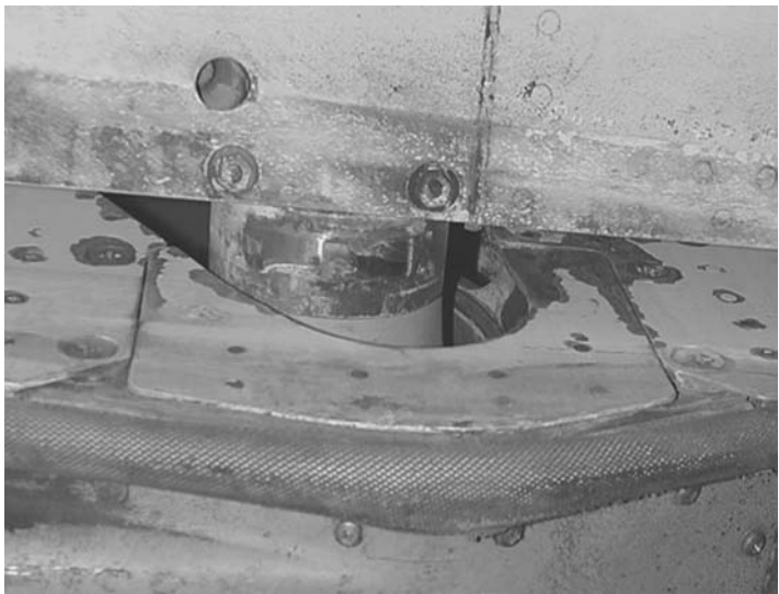
FIGURE 6.50 Fretting corrosion at the interface of two highly loaded surfaces which are not designed to move against each other. (Courtesy of Pacific Corrosion Control Corp)
