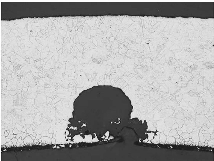
FIGURE 6.17 Stainless-steel cavernous pits formed on S30400 stainless steel following an intergranular corrosion attack. (Courtesy of Russ Green, TMI)
