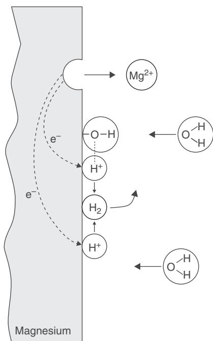
FIGURE 3.4 Electrochemical reactions occurring during the corrosion of magnesium in neutral water.
