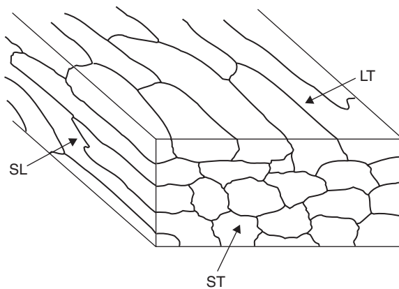
FIGURE 11.6 Schematic representation of the anisotropic grain structure of wrought aluminum alloys.
