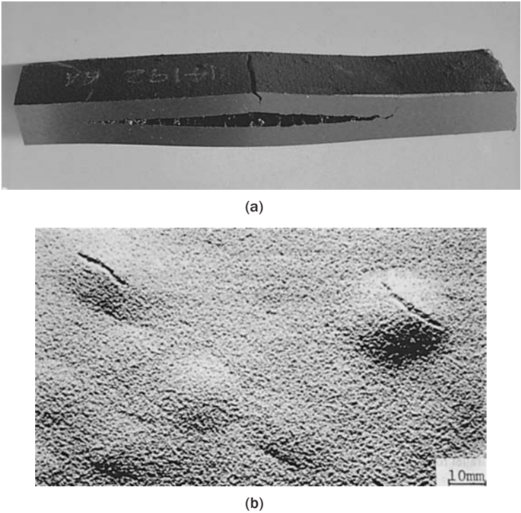
FIGURE 6.36 (a) Hydrogen induced cracking with mid-wall cracks running parallel to the pipeline wall; (b) Surface blisters may also contain cracks. (Courtesy of MACAW's Pipeline Defects , published by Yellow Pencil Marketing Co.)
