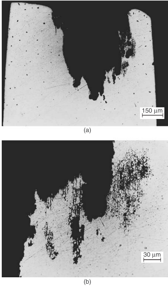
FIGURE 6.16 Photomicrograph of a section through an edge of the 8090-T851 panel immersed in seawater during four months; (a) at 64 \times and (b) at 320 \times to illustrate the intergranular nature of the corrosion attack.
