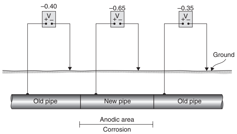
FIGURE 7.37 Schematic showing a differential corrosion cell created by replacement of a section of pipe.
