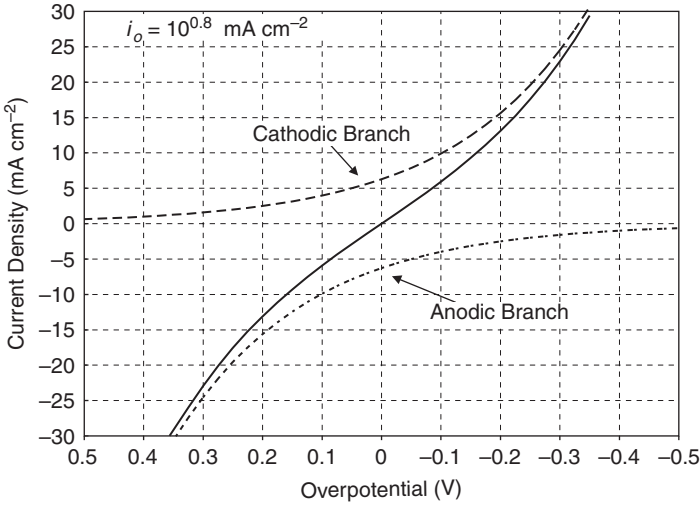
FIGURE 5.2 Current versus overpotential polarization plot of the ferric/ferrous ion reaction on palladium showing both the anodic and cathodic branches of the resultant current behavior.
