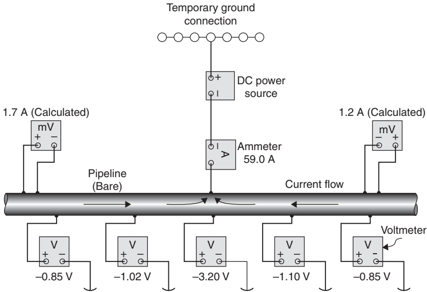
FIGURE 13.33 Evaluation of current requirement for CP.
