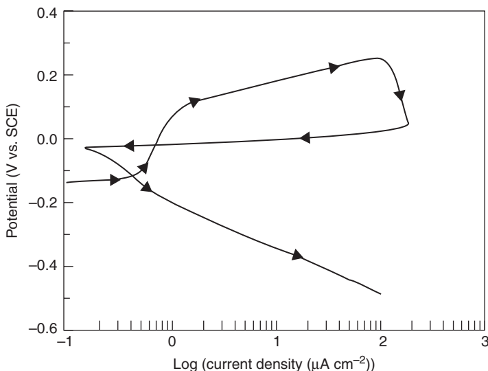
FIGURE 5.19 Polarization scan for S31600 steel in 50 percent aminotrimethylene phosphonic acid after one day of exposure (the arrow indicates scanning direction).
