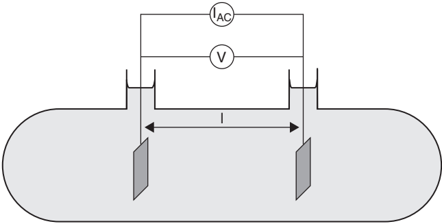
FIGURE 5.7 Schematic of a conductivity cell containing an electrolyte and two inert electrodes of surface A parallel to each other and separated by distance \ell .
