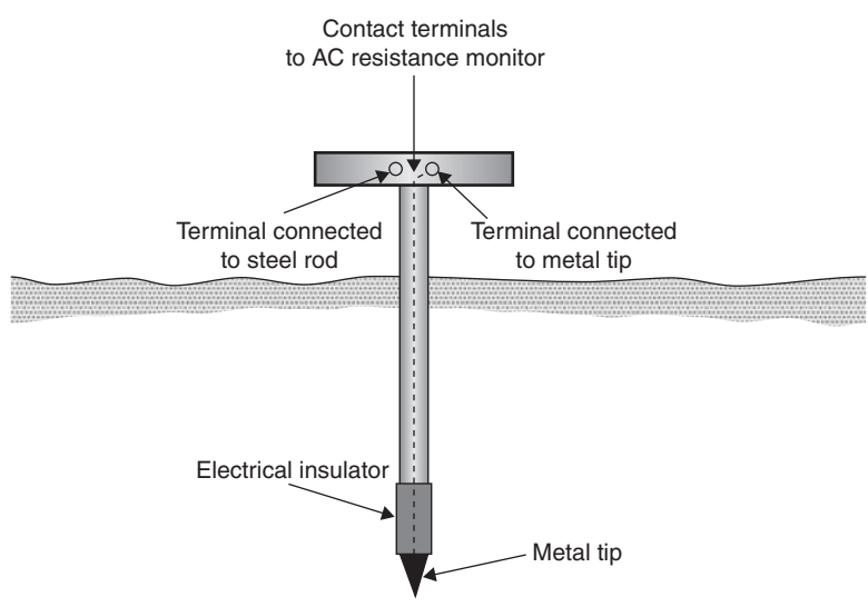
FIGURE 5.12 Soil rod method for soil resistivity measurements.
