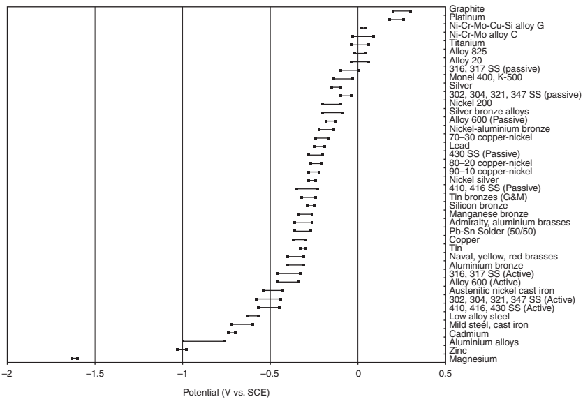
FIGURE 7.18 Galvanic series for slow-moving seawater.
