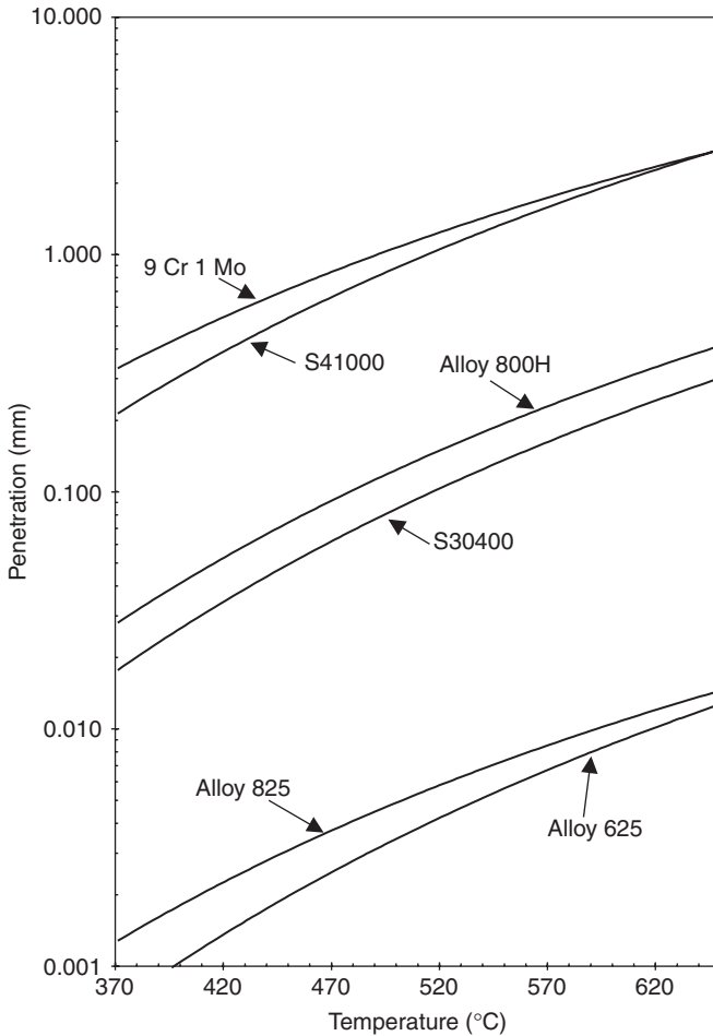
FIGURE 15.25 Effect of temperature upon sulfidation corrosion after one year in \text{H}_2 - \text{H}_2\text{S} gases containing 1 percent vol \text{H}_2\text{S} at 34 atm.
