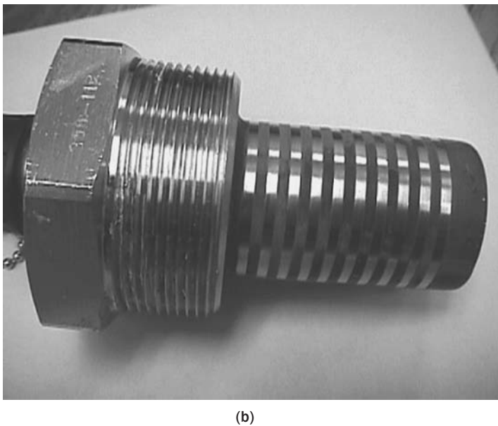
FIGURE 10.13 (a) Schematic and (b) picture of the BioGEORGE MIC detection probe. (Courtesy of George Licina, Structural Integrity Associates, Inc)
