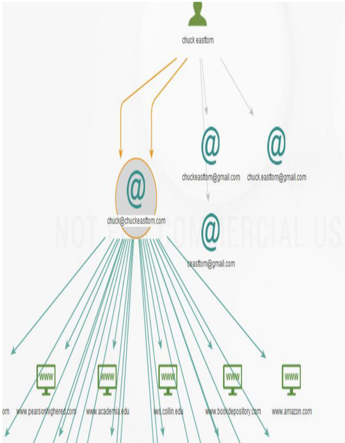
Figure 13.10 Maltego Graph
