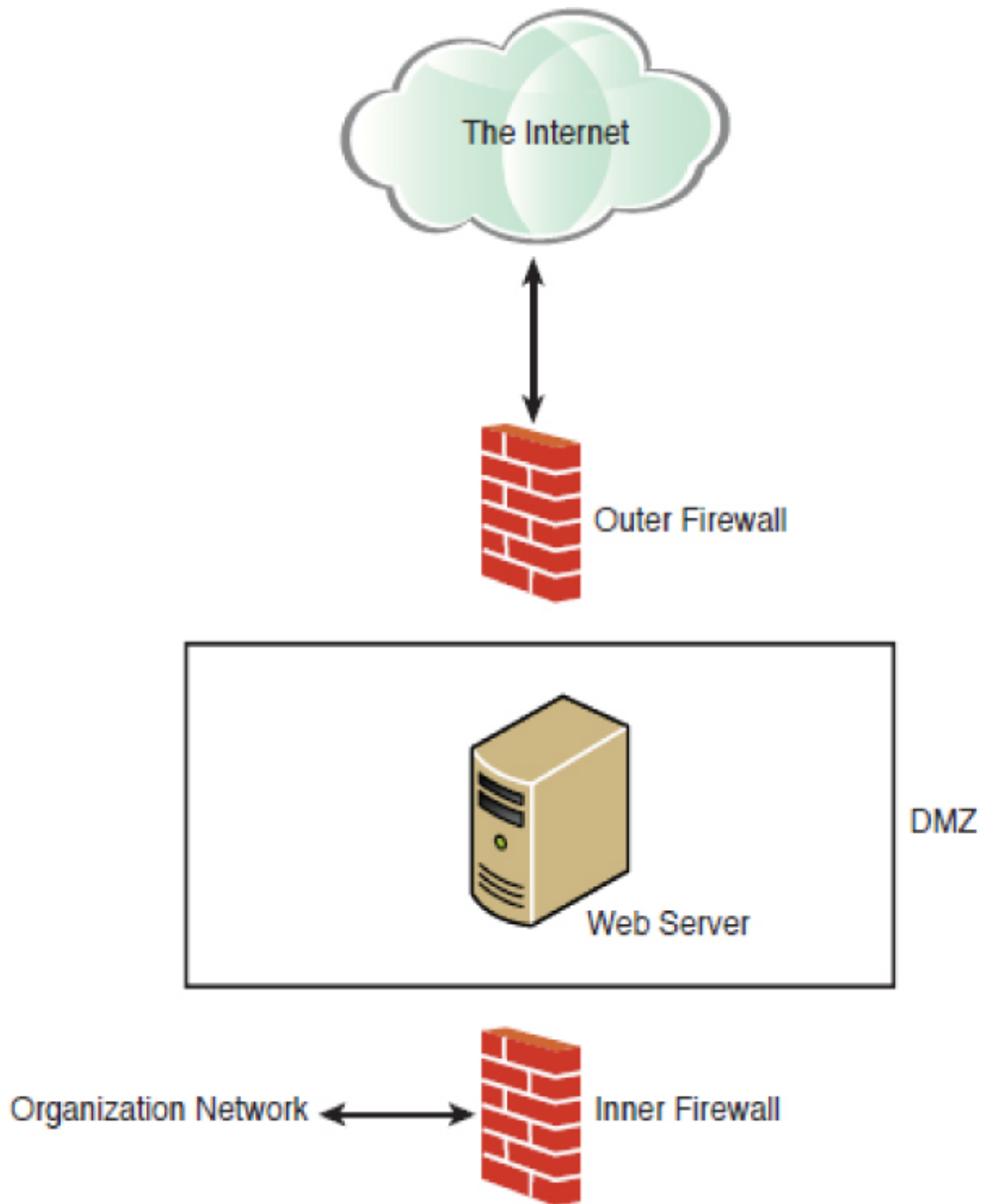
Figure 11.3 DMZ.
