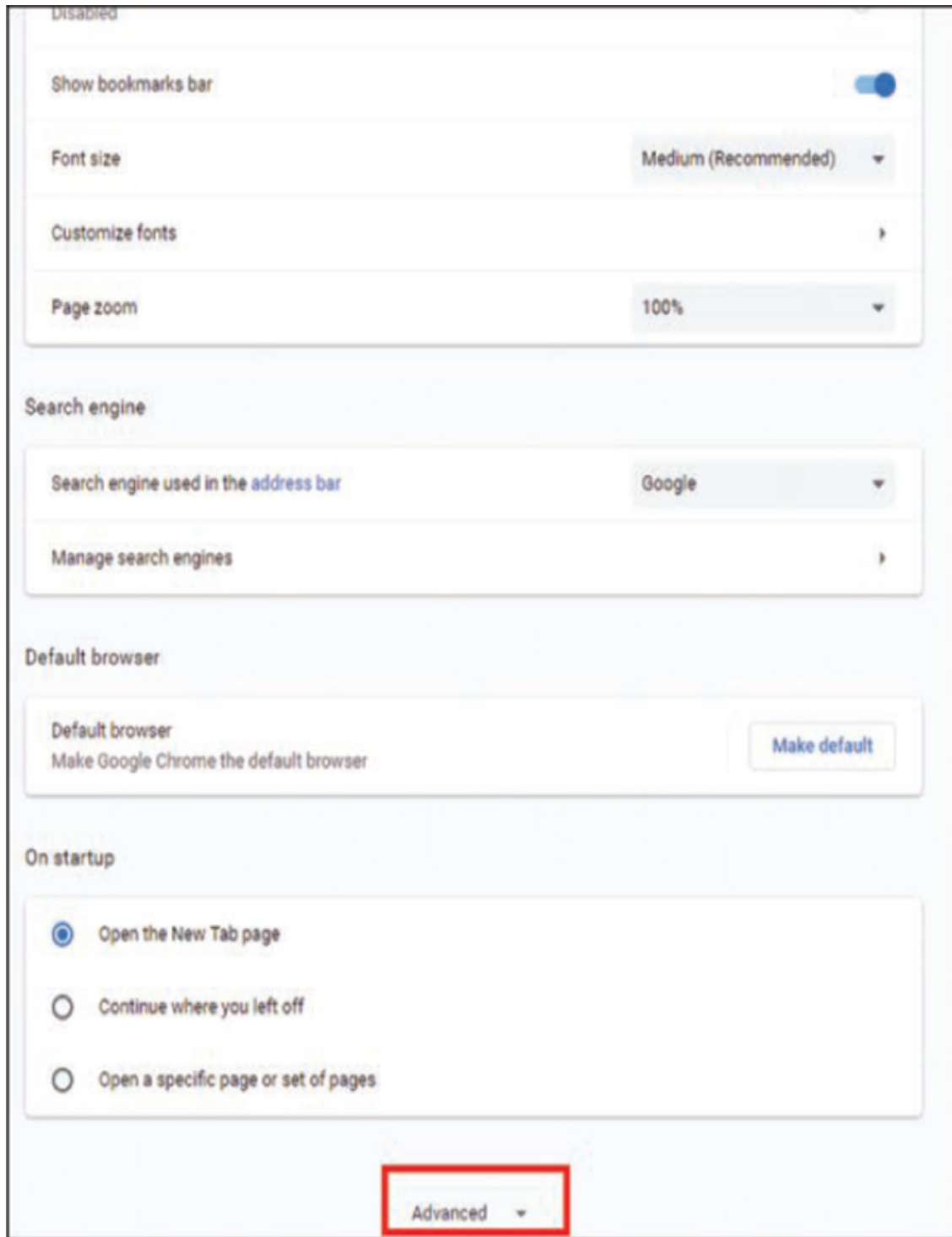
Figure 3.5 Chrome settings.
