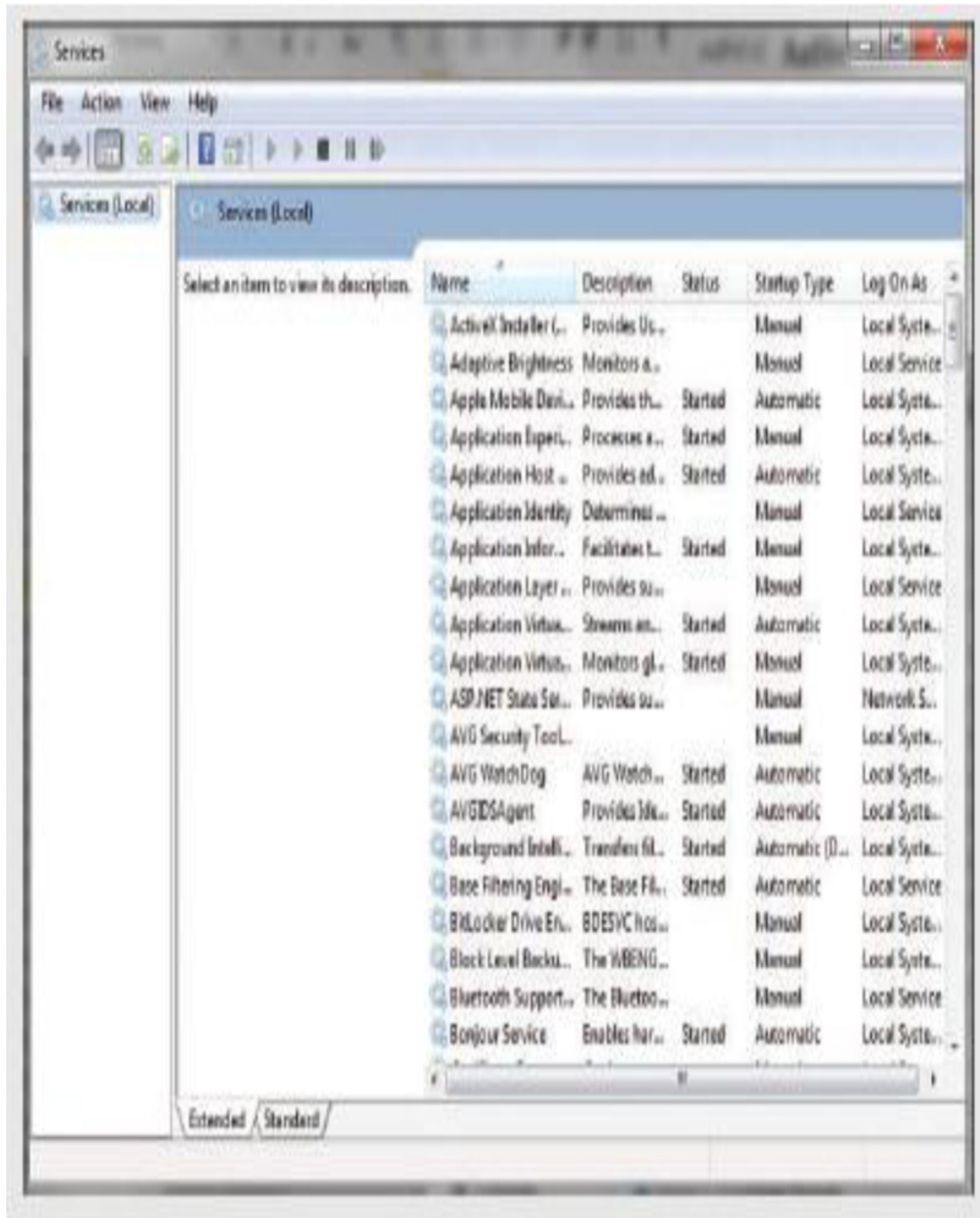
Figure 11.1 Services.
