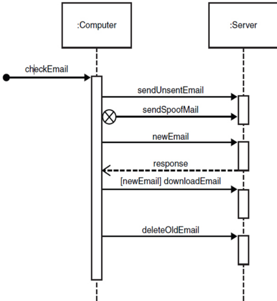
Figure 15.14 Modified sequence diagram.
