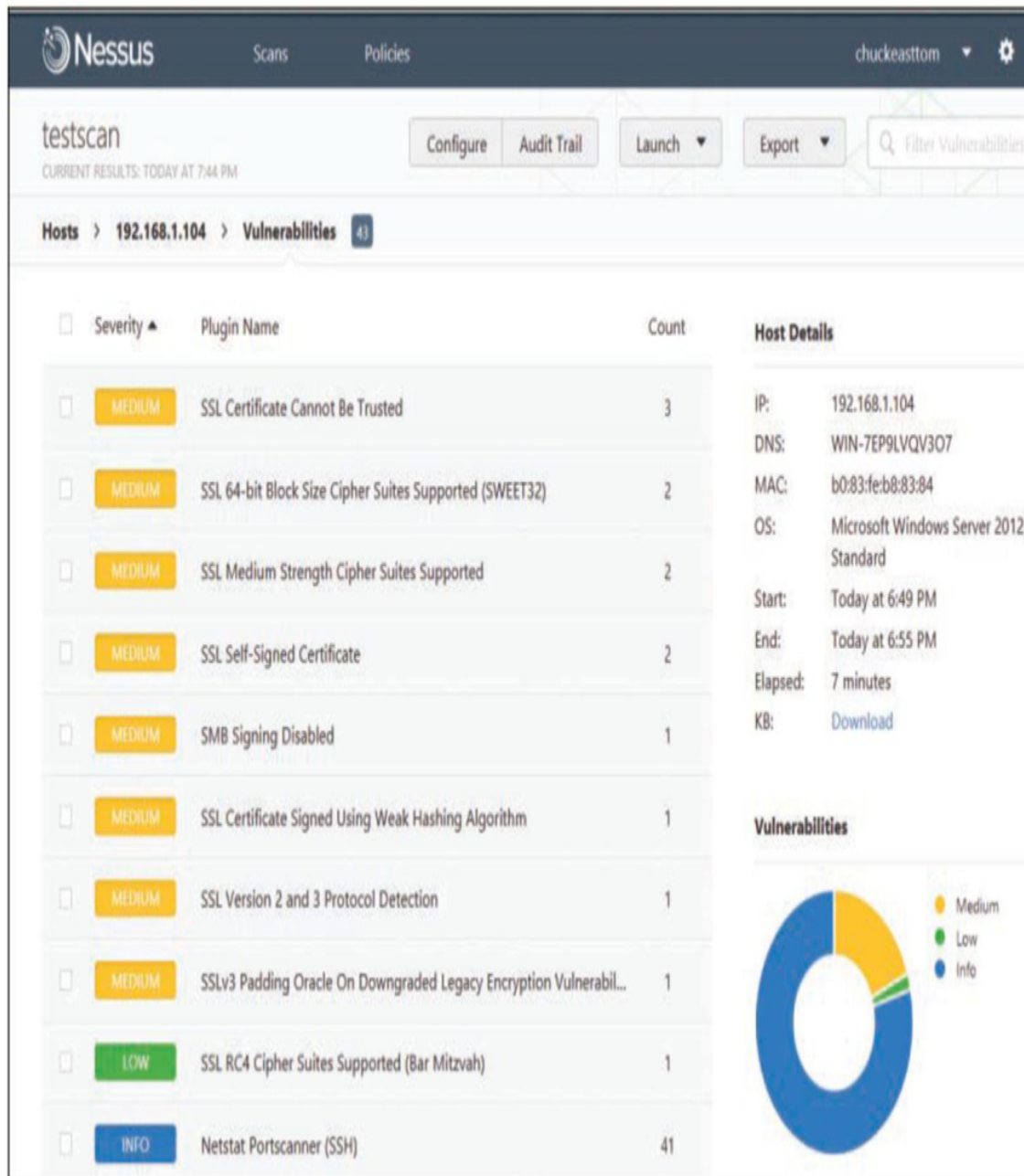
Figure 11.8 Drilling down into Nessus results.
