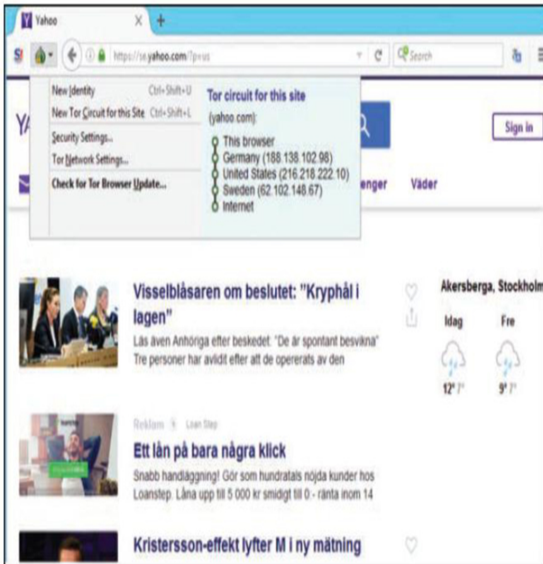
Figure 6.11 Yahoo through TOR.
