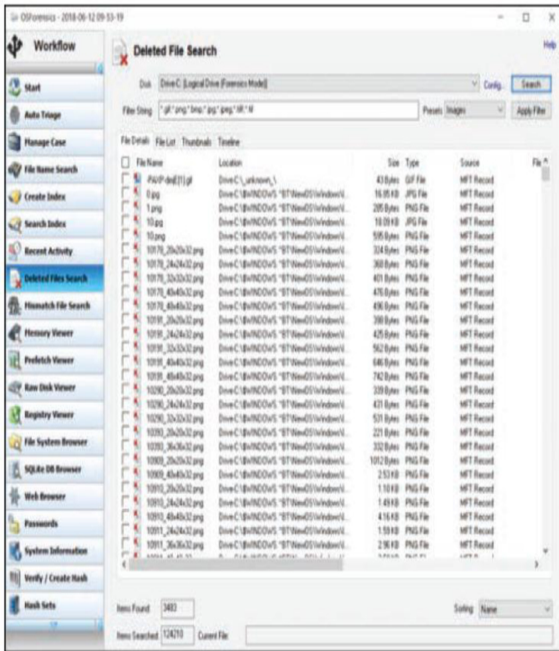
Figure 14.11 OSForensics Deleted File Search Option.
