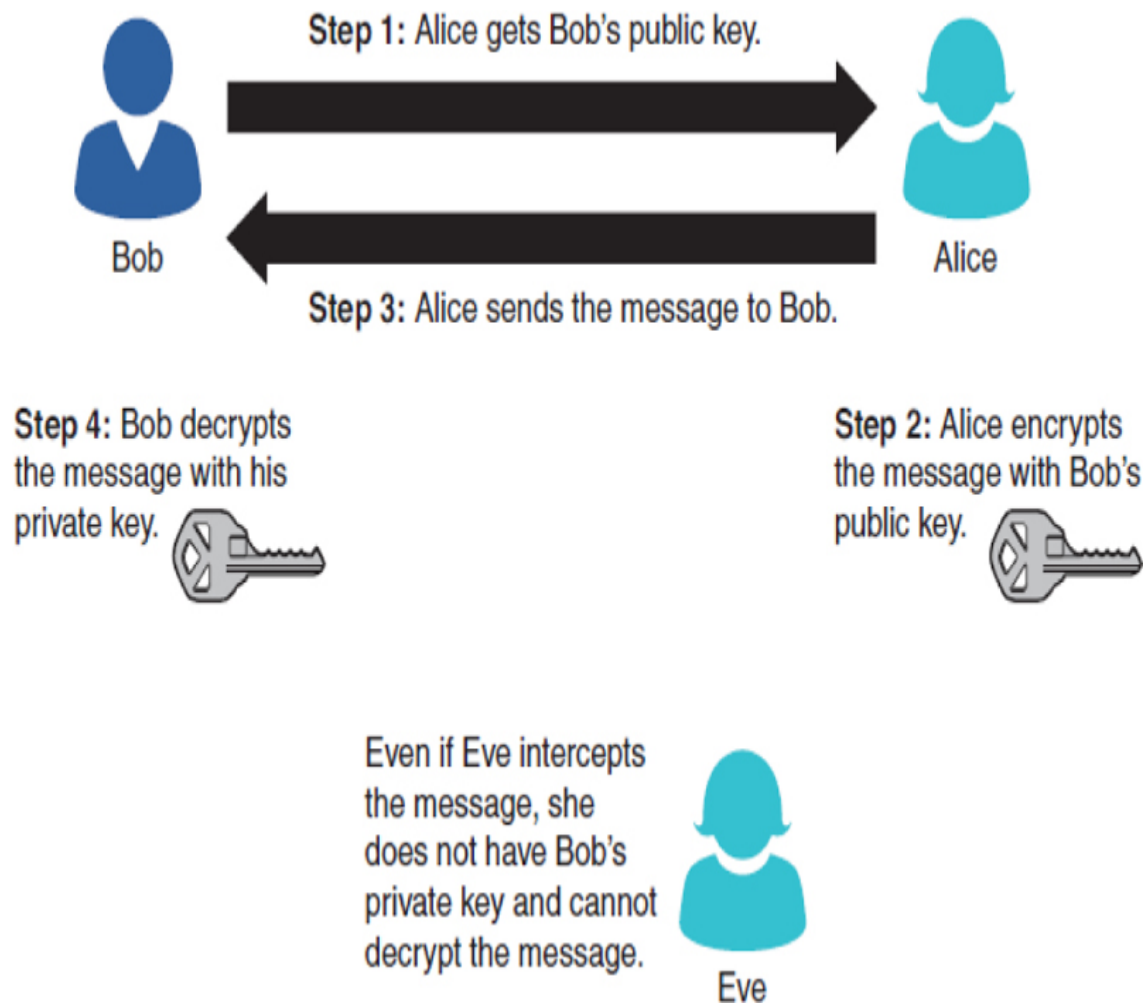
Figure 8.6 Public key cryptography.
