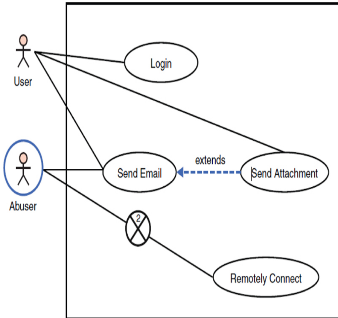
Figure 15.11 Specific misuse-case example.
