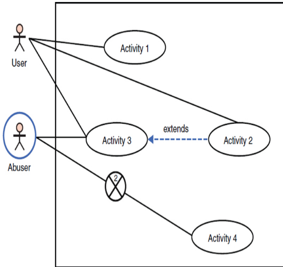
Figure 15.10 Another misuse-case example.
