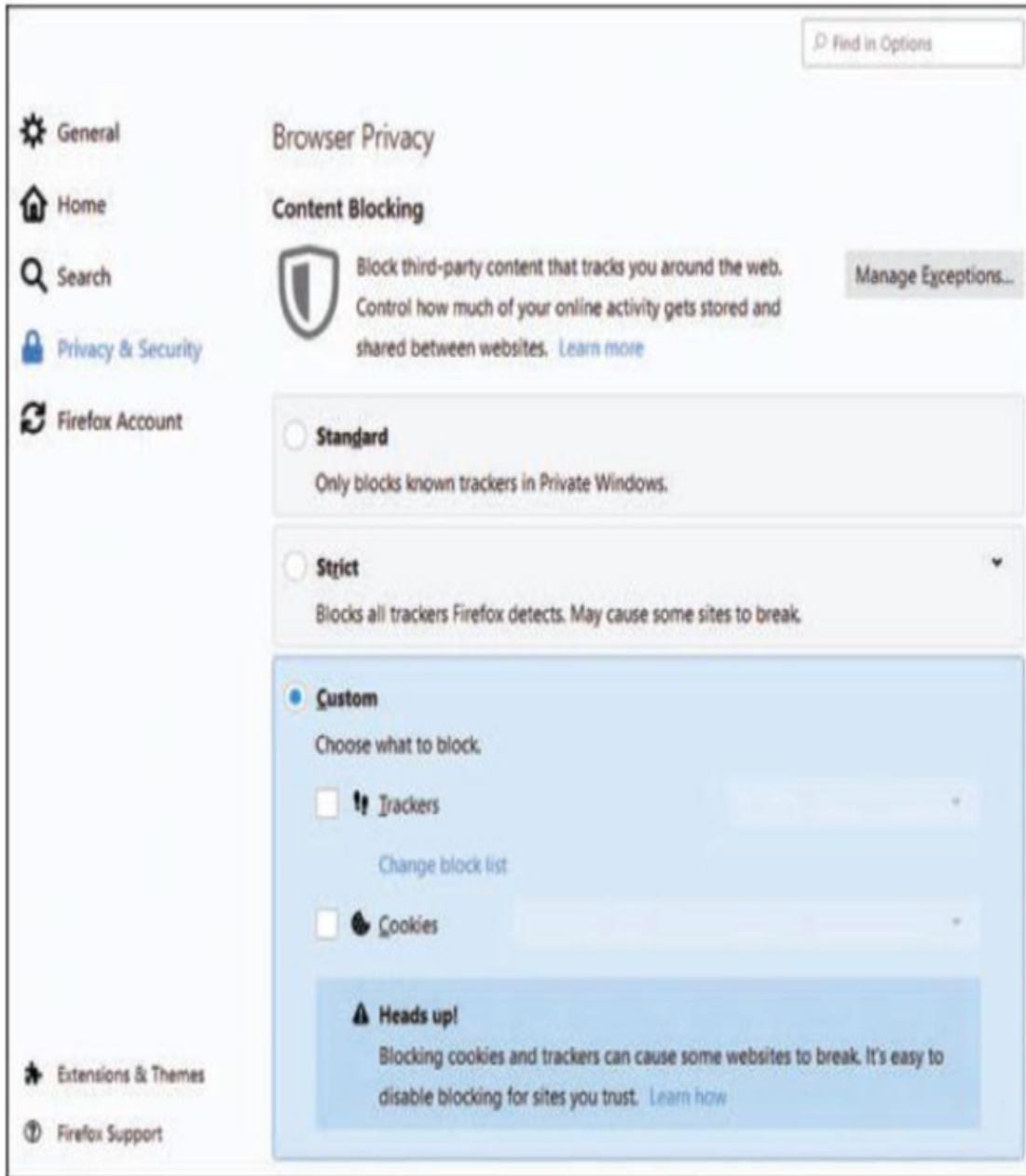
Figure 3.4 Firefox privacy.
