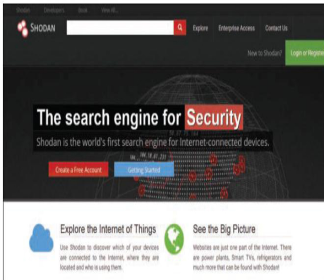
Figure 11.11 Shodan.io .
