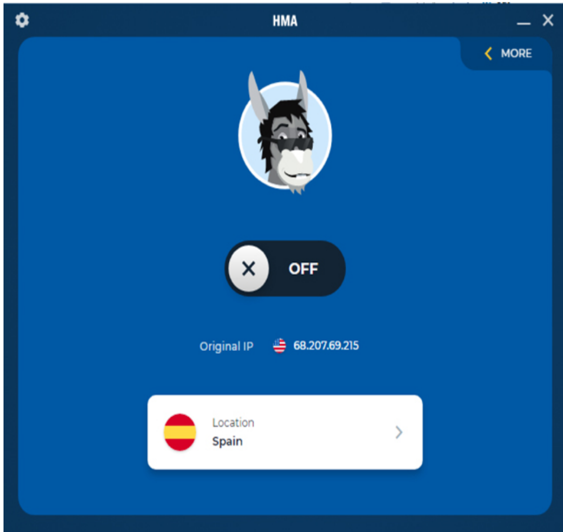
Figure 3.6 HMA
