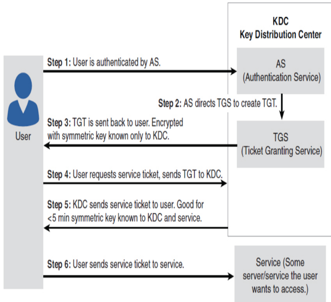
Figure 9.9 Kerberos.
