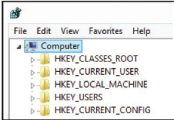
Figure 14.16 Windows Registry.
