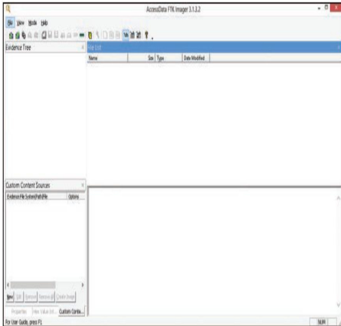
Figure 14.1 FTK Imager.
