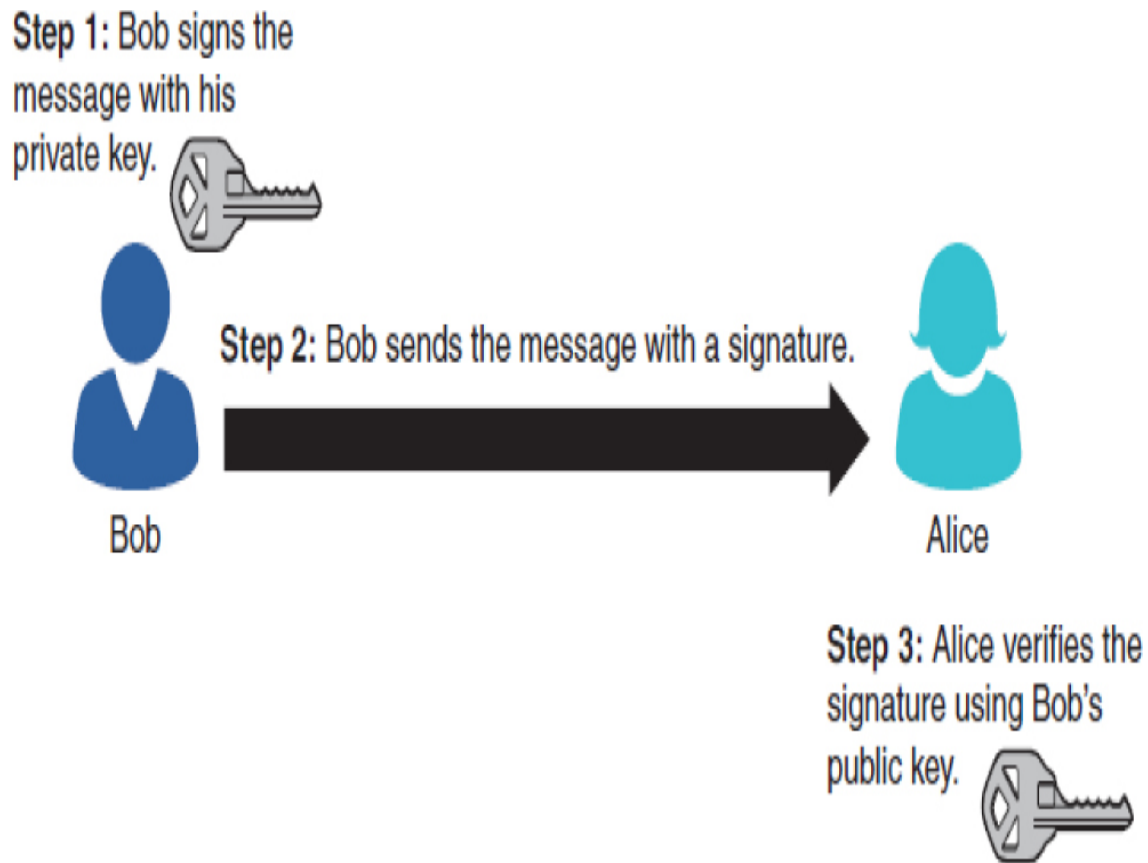
Figure 8.8 Digital signatures.
