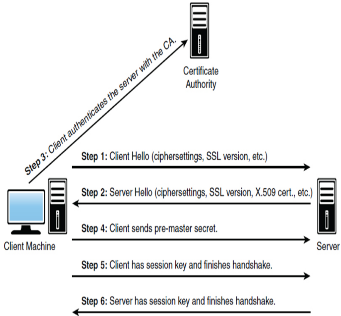
Figure 9.10 SSL/TLS .
