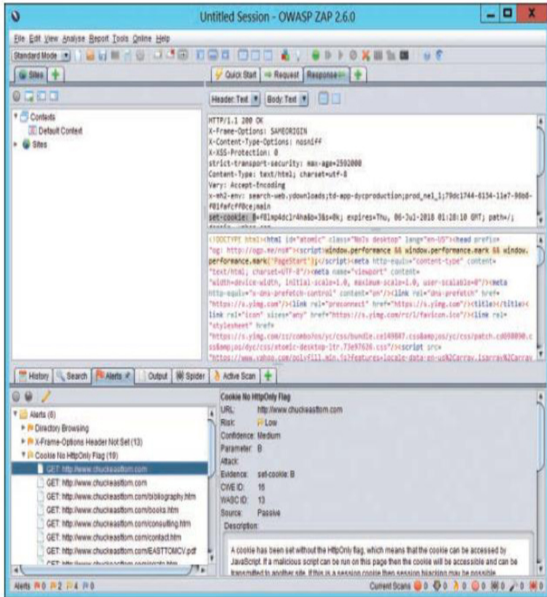
Figure 11.10 OWASP ZAP results.
