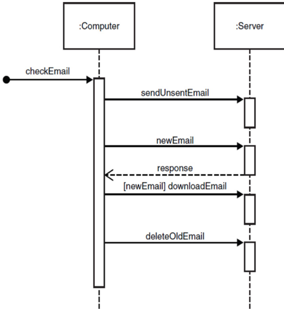
Figure 15.12 UML/SysML sequence diagram.
