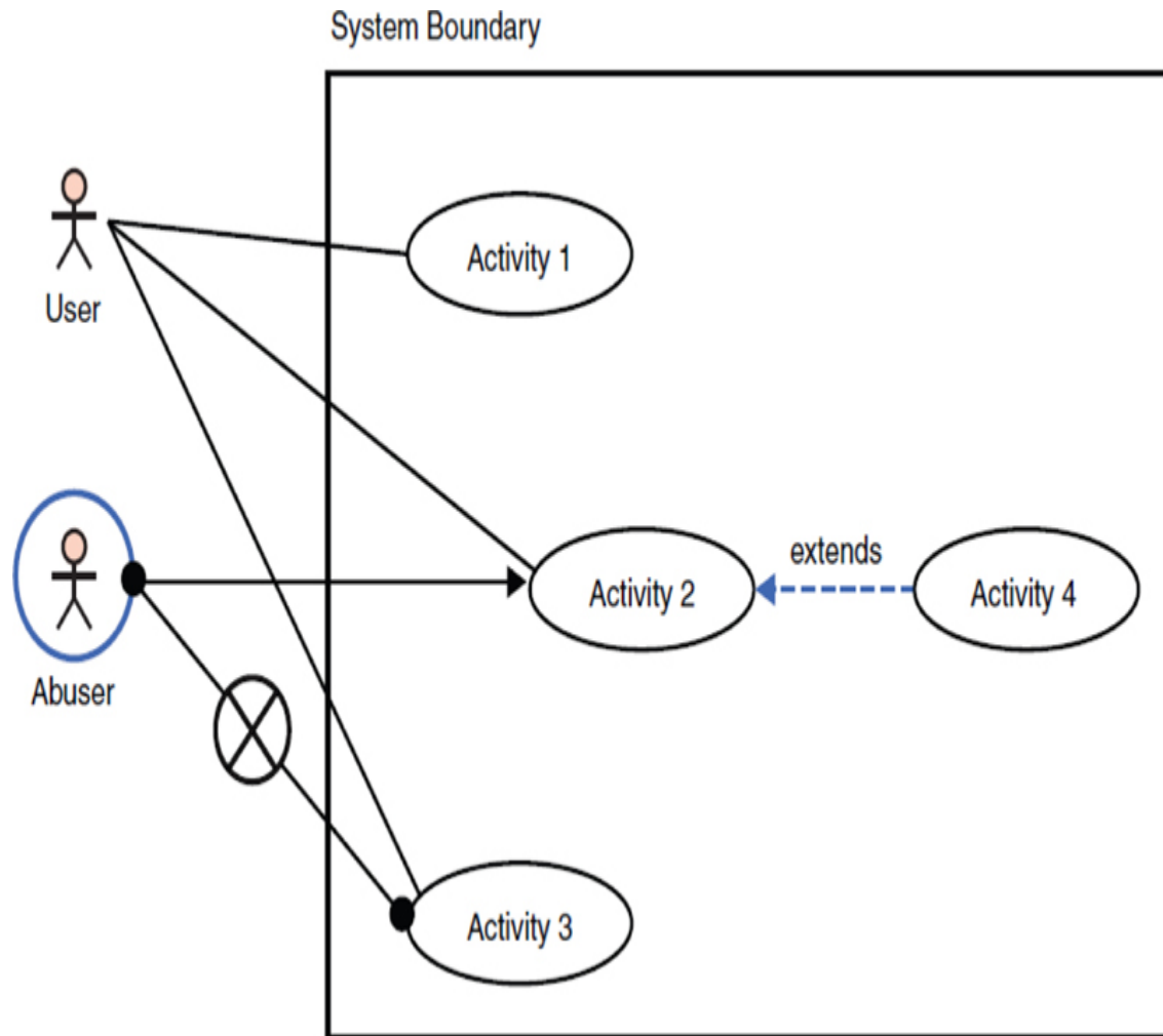
Figure 15.9 Misuse-case diagram example.
