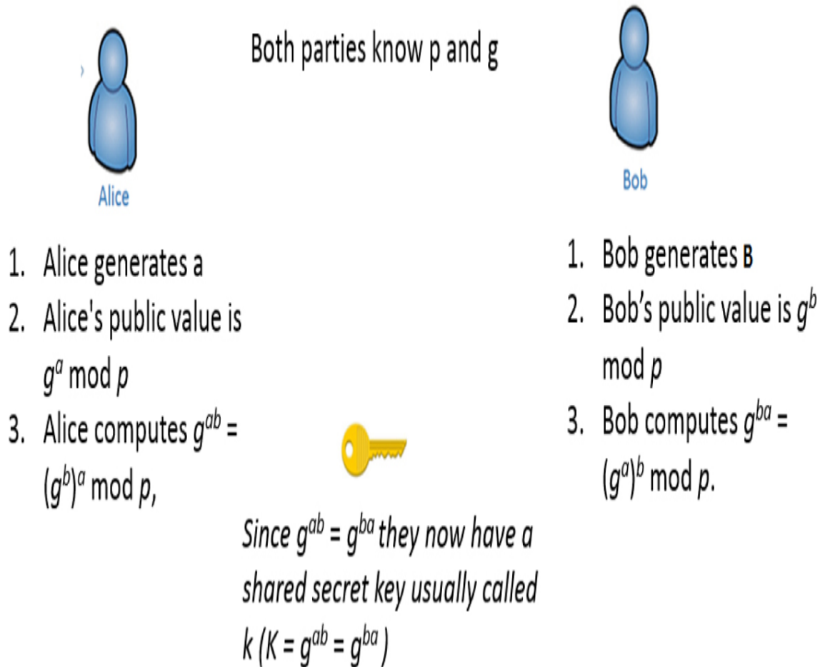
Figure 8-7 Diffie Hellman
