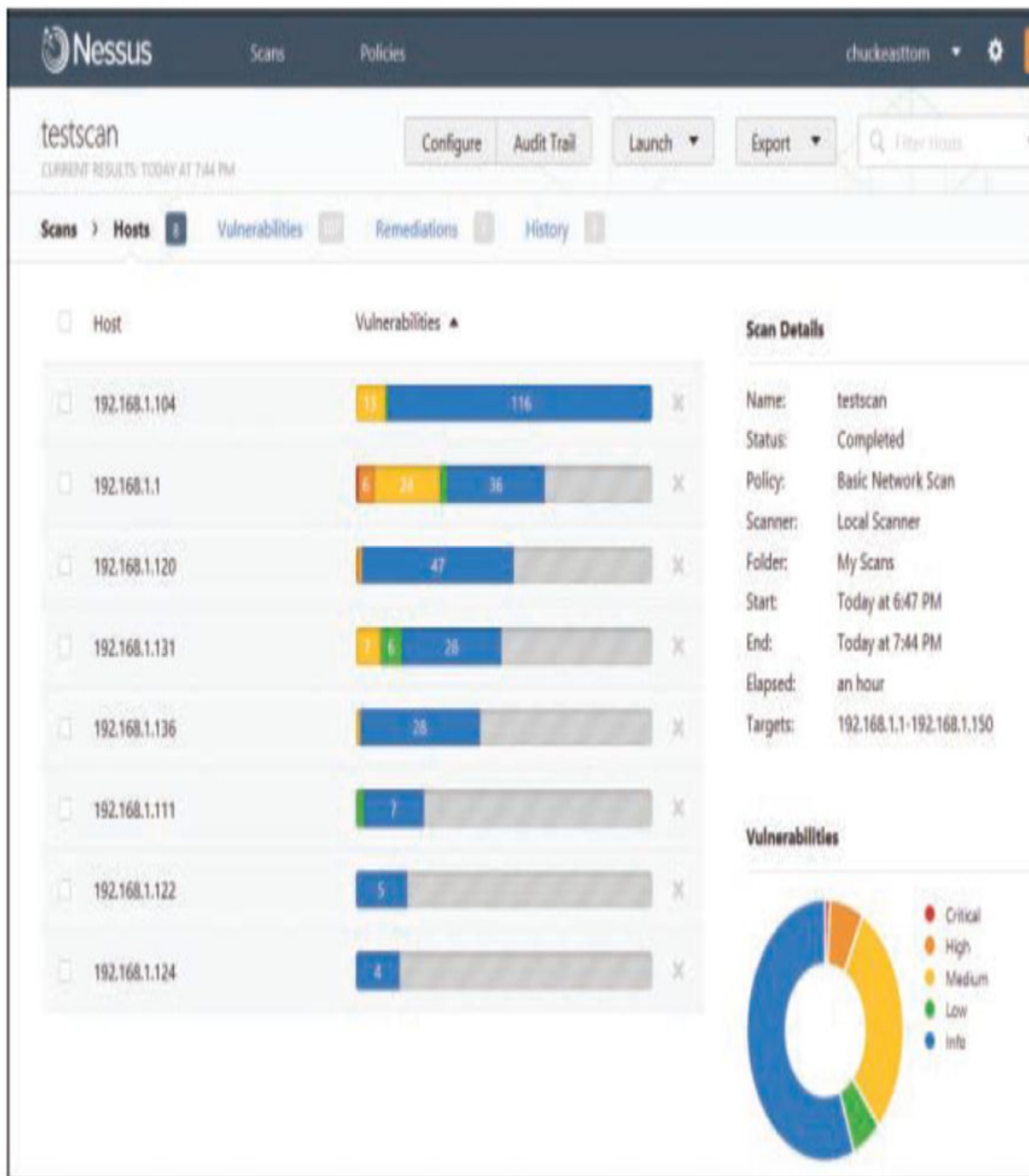
Figure 11.7 Nessus results.
