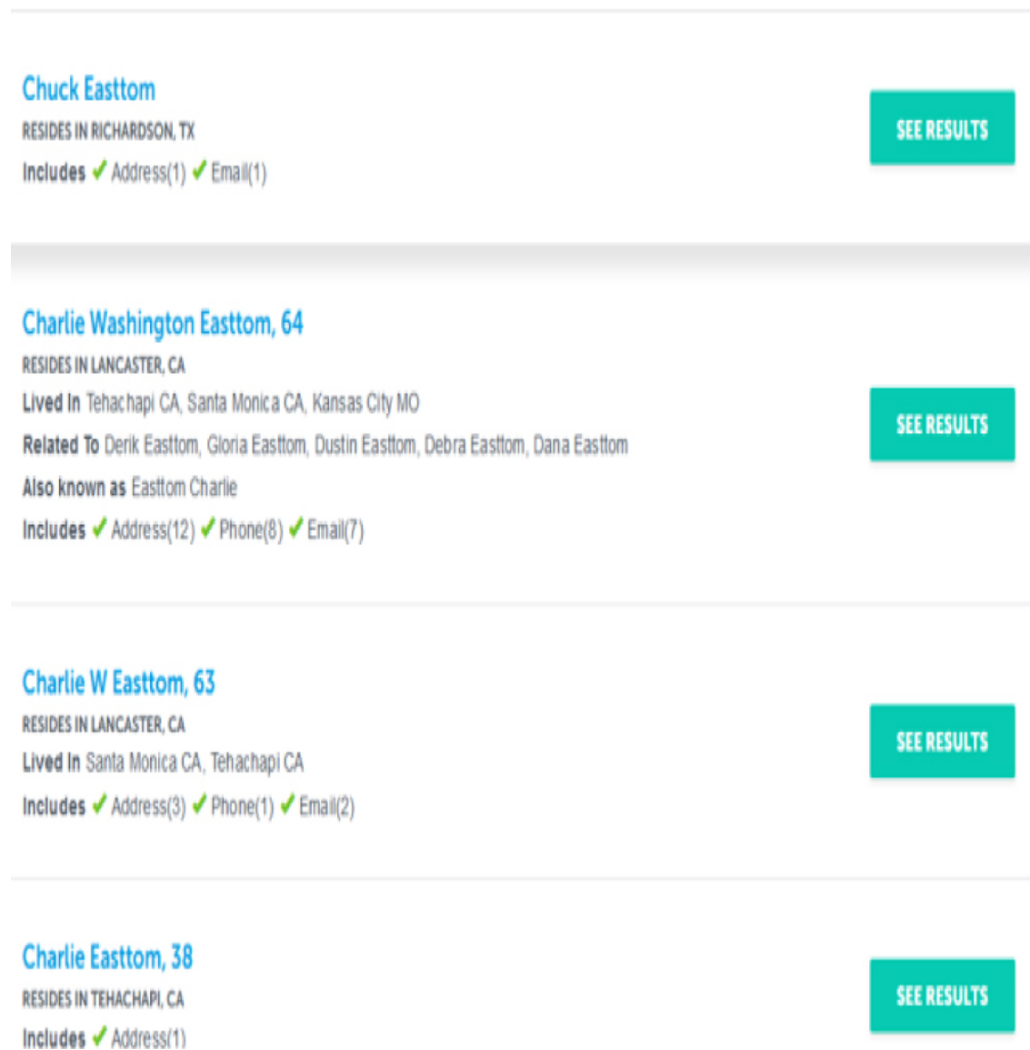
Figure 13.2 Search options.
