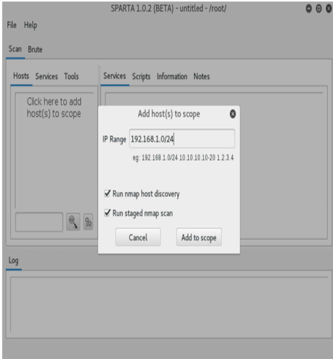
Figure 11.16 Sparta step 2
