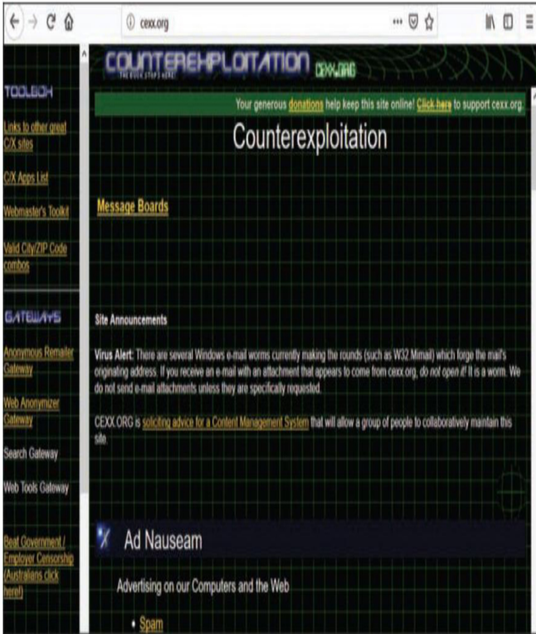
Figure 5.2 Counterexploitation website.
