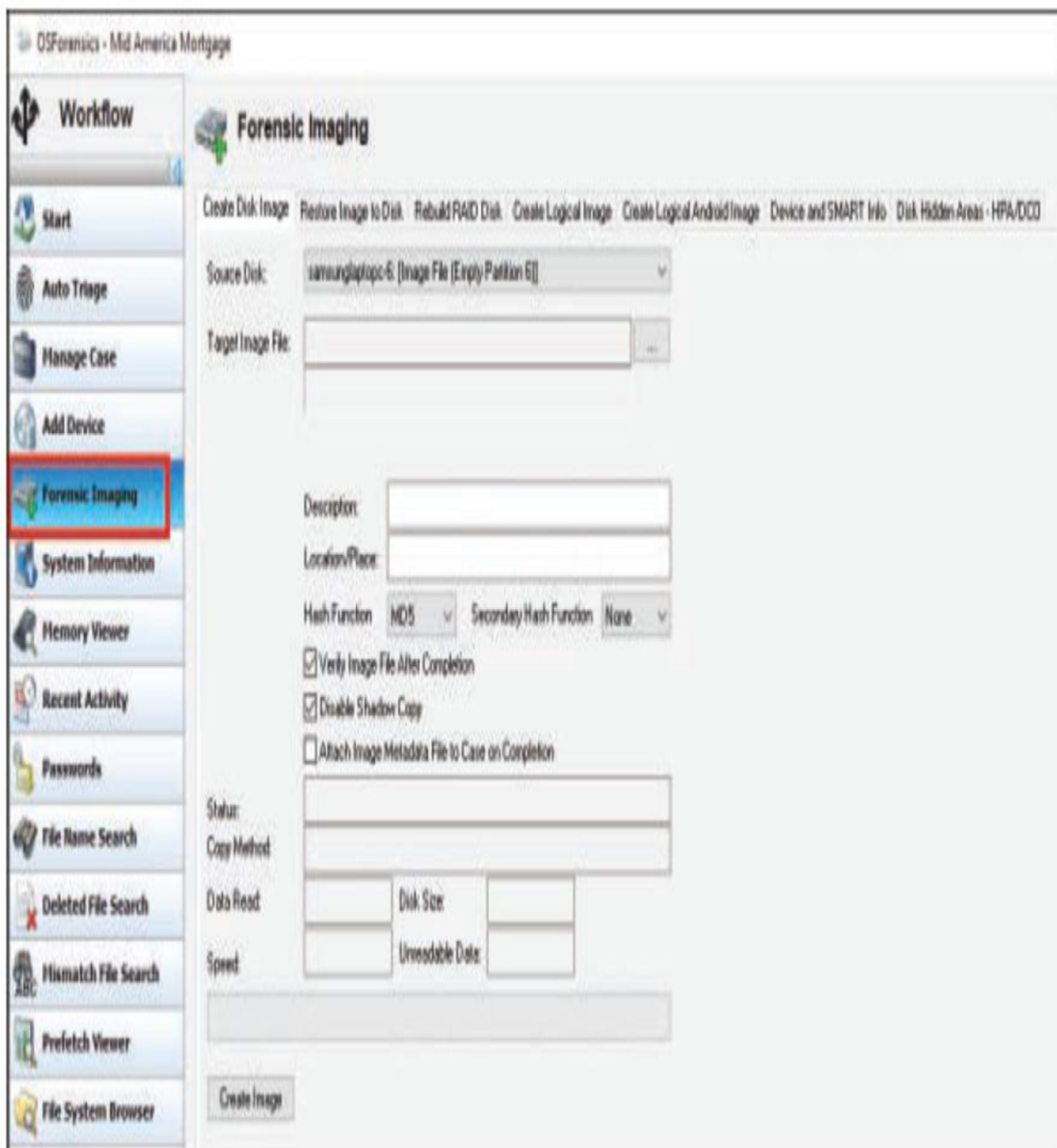
Figure 14.6 OSForensics Imaging.
