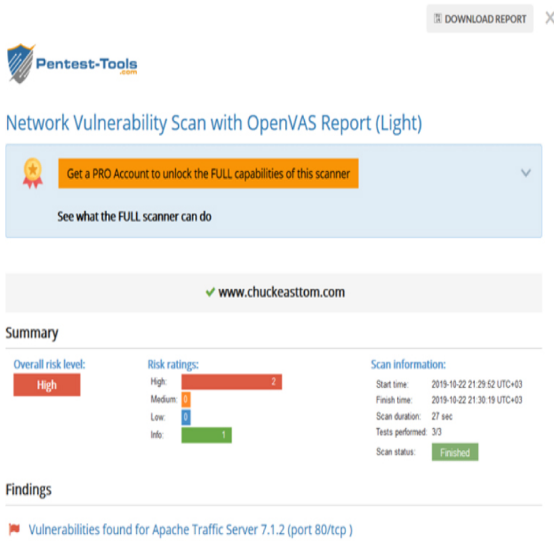
Figure 11.19 OpenVAS Results
