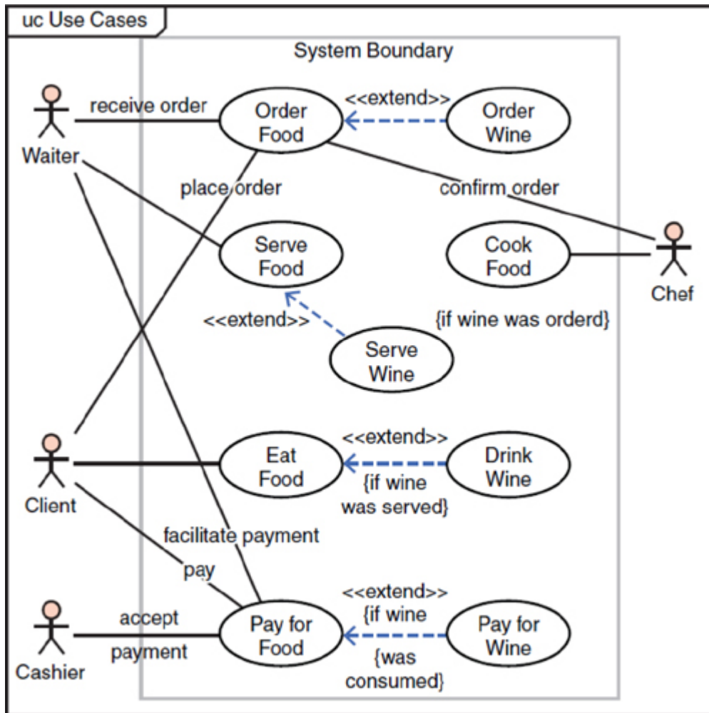
Figure 15.7 Typical use-case diagram.
