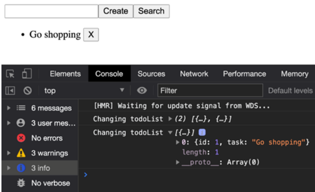
Figure 8.21: Changing to-do list data
