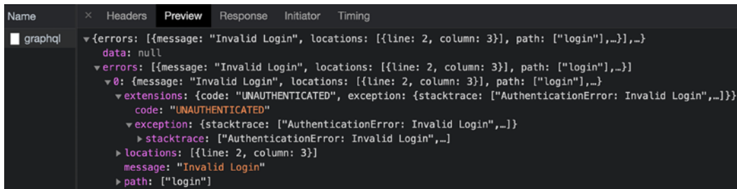
Figure 13.33: Invalid login
