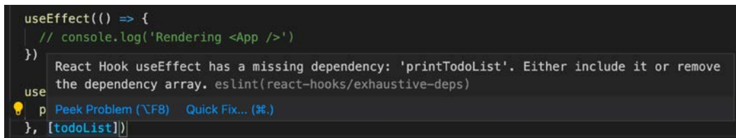
Figure 8.19: react-hooks/exhaustive-deps
