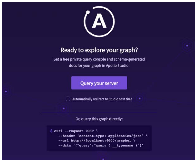
Figure 14.12: GraphQL Explorer
