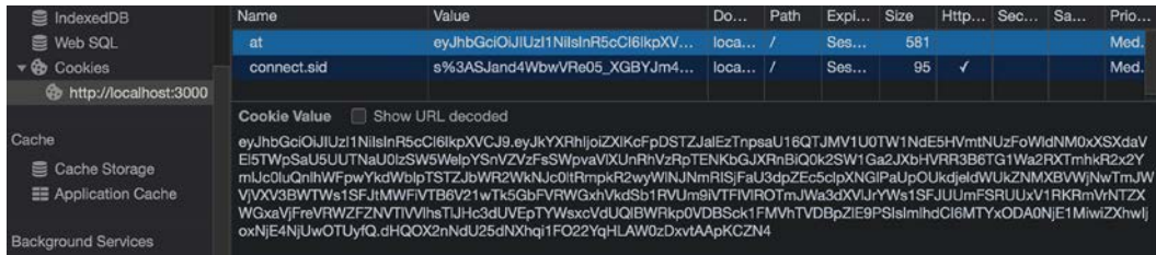
Figure 13.37: Cookies
