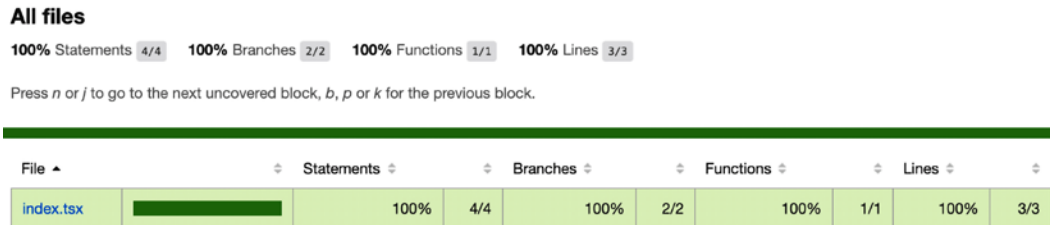
Figure 16.4: lcov-report
