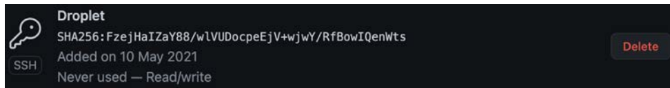
Figure 17.14: SSH
