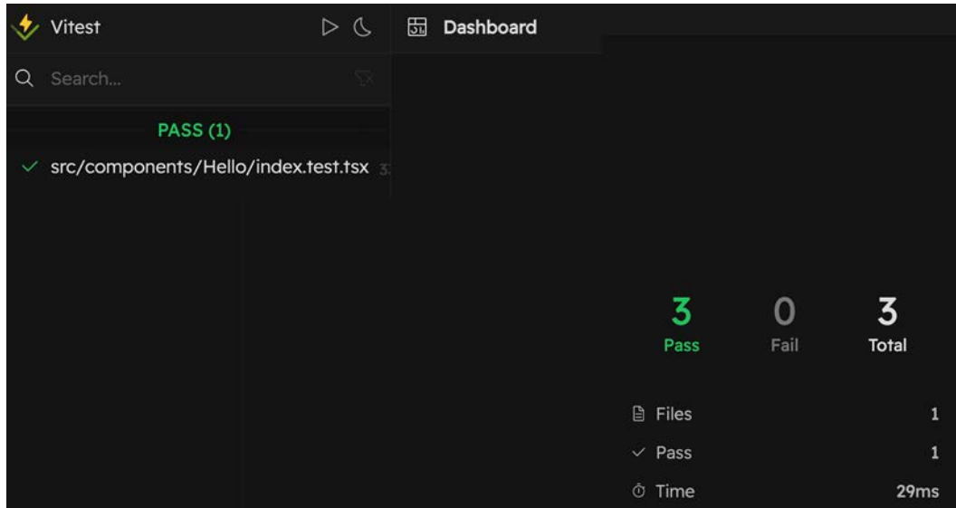
Figure 16.9: Vitest UI
