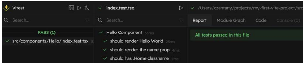
Figure 16.10 – Report
