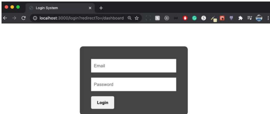
Figure 13.30: Login page
