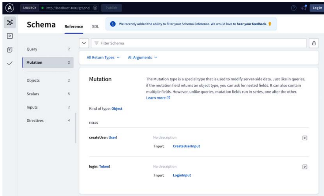
Figure 13.7: Schema
