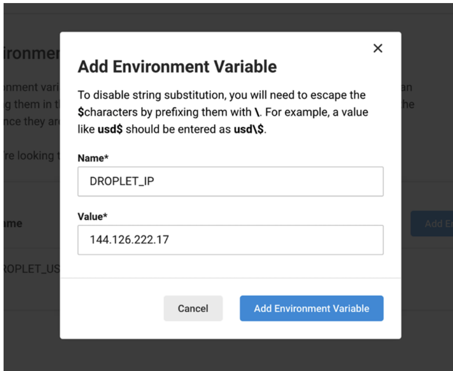
Figure 17.36: DROPLET_IP
