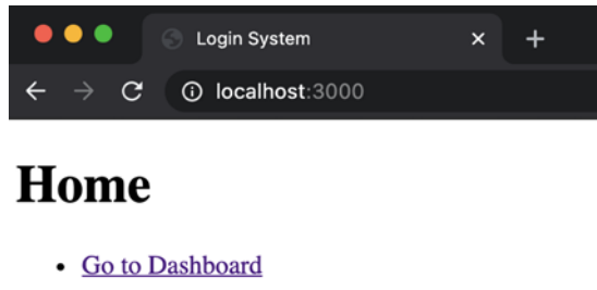
Figure 13.29: Home page
