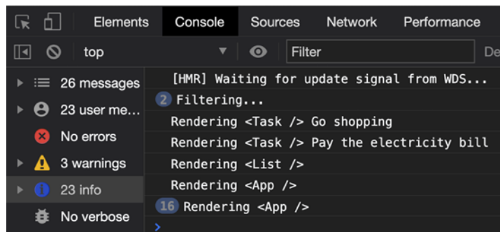
Figure 8.16: Improving performance
