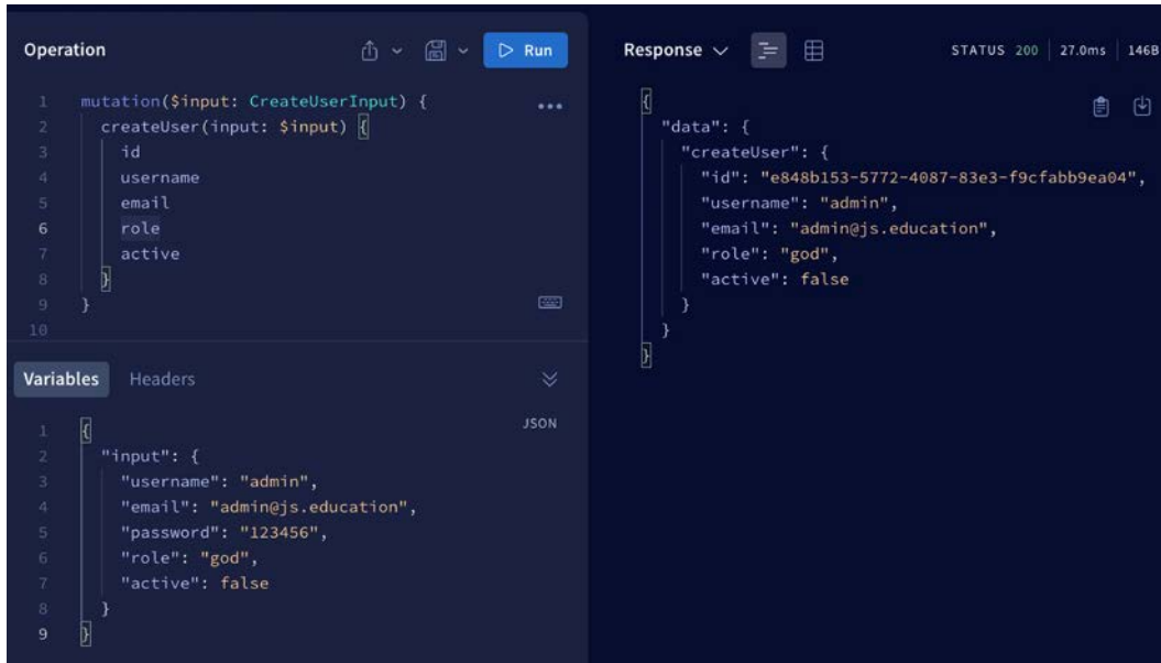
Figure 13.9: CreateUser mutation
