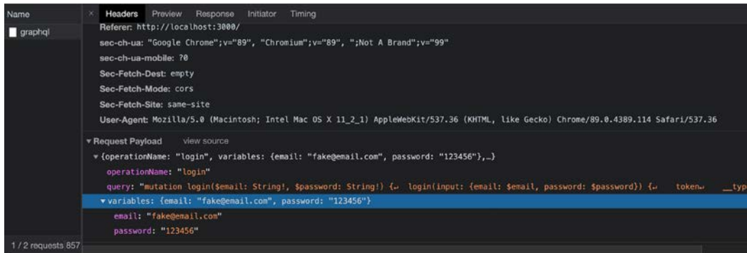
Figure 13.32: GraphQL request
