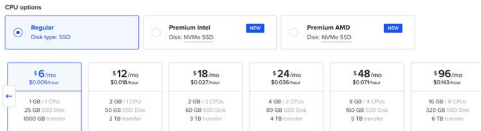
Figure 17.6: CPU options
