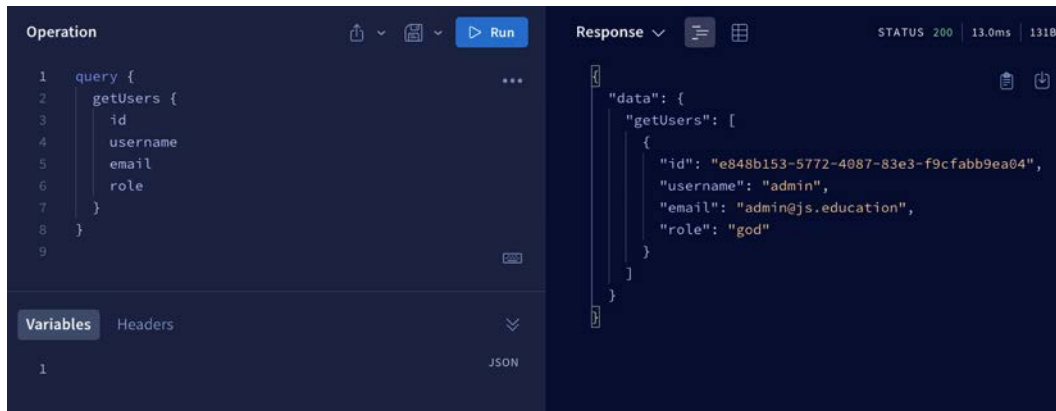
Figure 13.10: getUsers query
