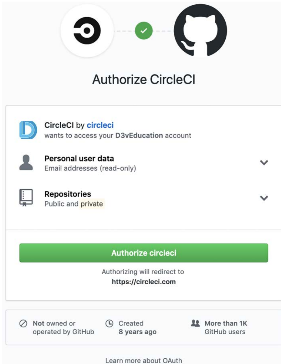
Figure 17.31: Authorize CircleCI
