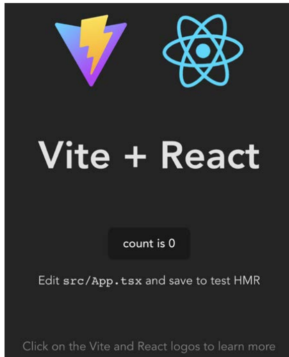
Figure 16.7: Vite app
