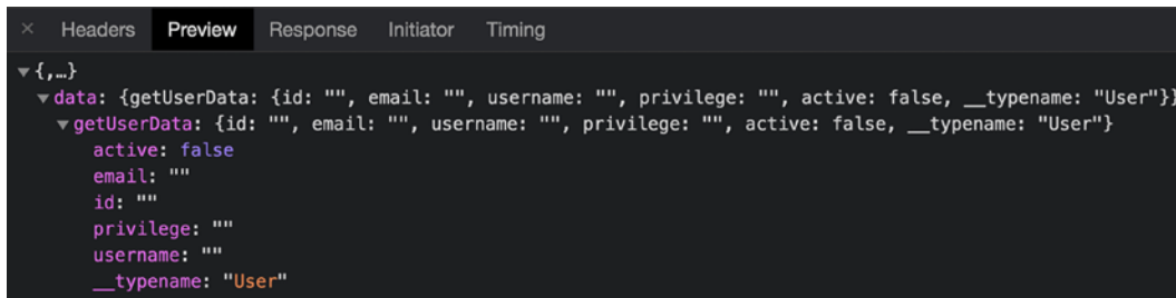
Figure 13.39: Empty data
