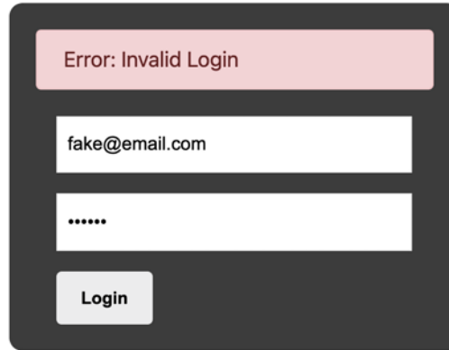
Figure 13.31: Invalid login
