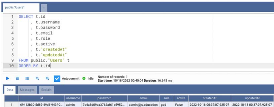
Figure 13.11: Database query
