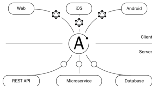
Figure 13.2: Apollo Server
