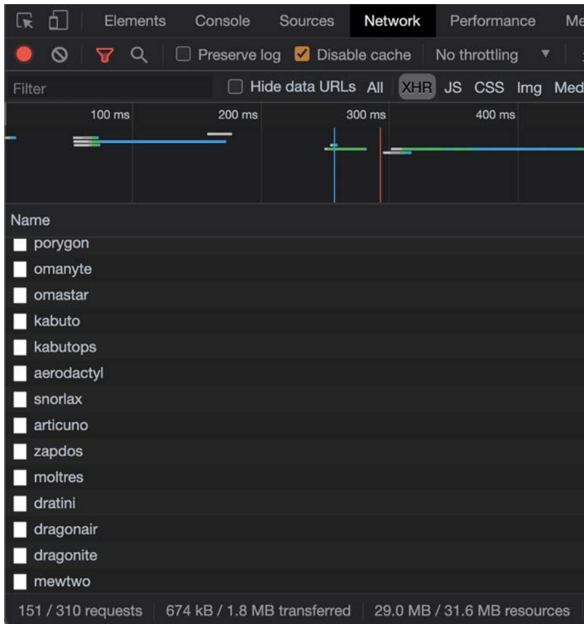
Figure 11.7: Requests
