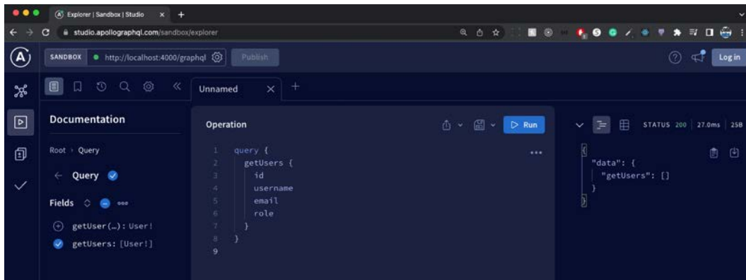
Figure 13.6: getUsers query
