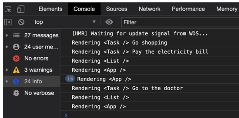
Figure 8.7: Improving performance
