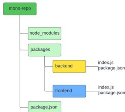
Figure 14.1: MultiRepo vs MonoRepo
