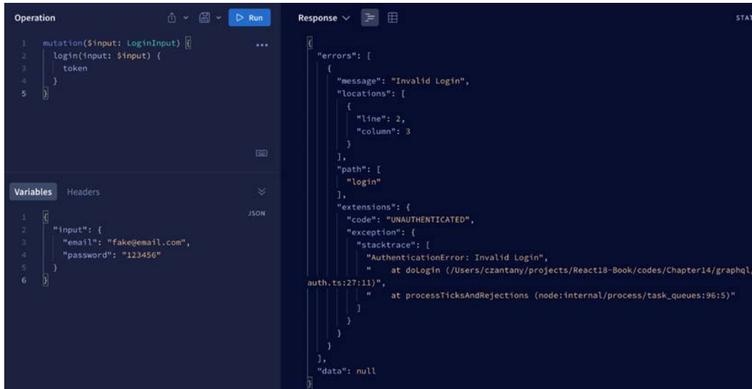
Figure 13.17: Invalid login after using non-existent login details
