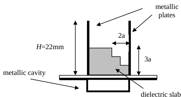
Fig. 10.25 Side view of staircase shaped image NRD antenna with no flared horn (from [38], reprinted with permission from IEE).
