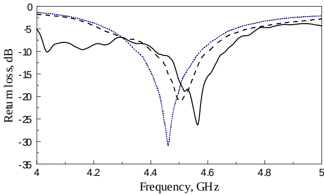
Fig. 1.32 Comparison of the measured return losses. ..... Single element, ----- 2×2 subarray, ——— 4×4 array.
