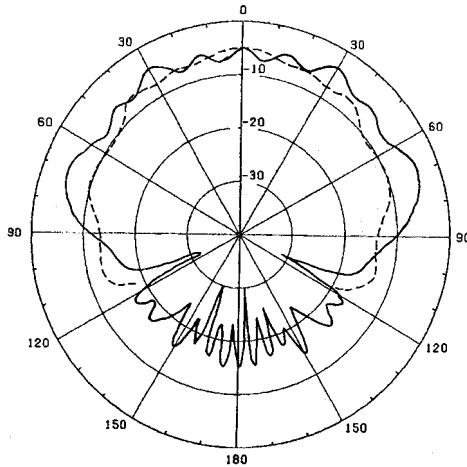
Fig. 4.29 Computed far field radiation patterns of a dielectric resonator with a=0.1706\lambda , a/h=1.67 , \rho_t/a=0.95 , \epsilon_r=8.9 , and a circular ground plane of radius 4\lambda (solid line) E-plane, (dashes) H-plane. (from [7] © 1989 IEEE Antenna and Propagation Magazine)
