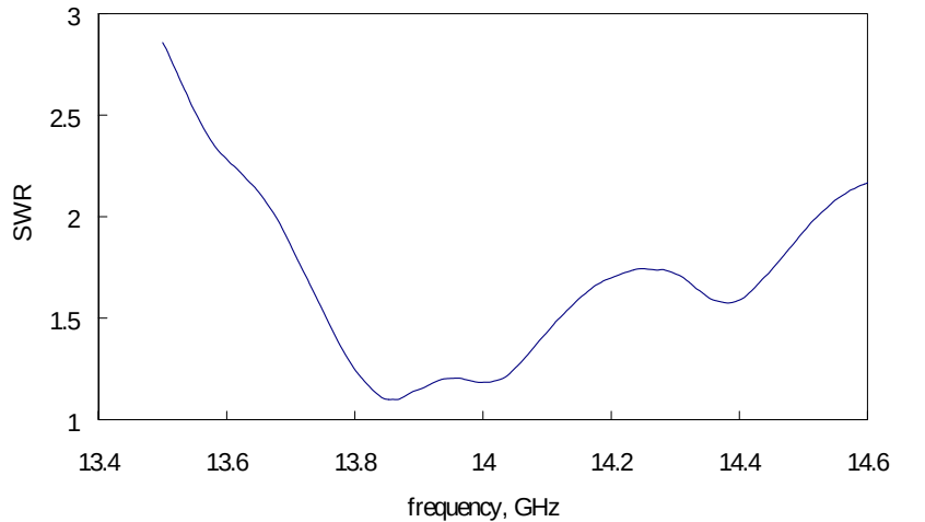
Fig. 10.12 Measured SWR of the antenna.
