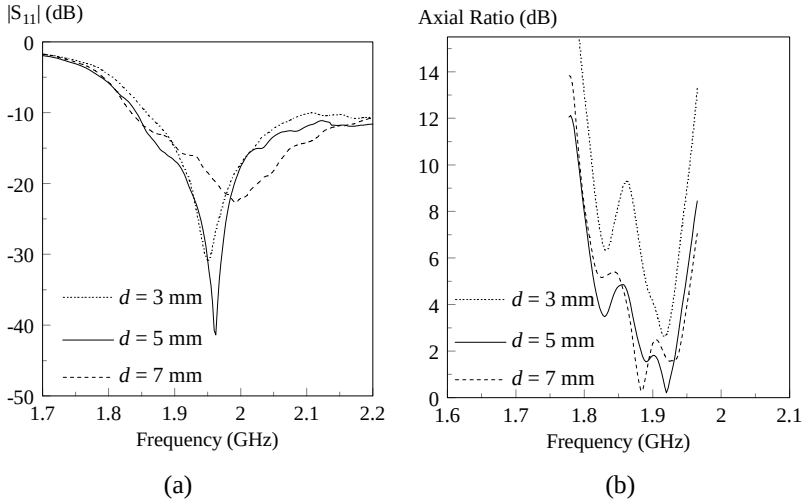
Fig. 1.26 Measured return loss and axial ratio against frequency for different stub depths. (a) Return loss; (b) Axial ratio. (From [92], reprinted with permission from IEEE)
