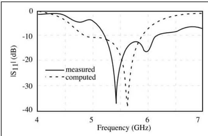
Figure 2.24 Computed and measured return losses of the DRA of Figure 2.22.
