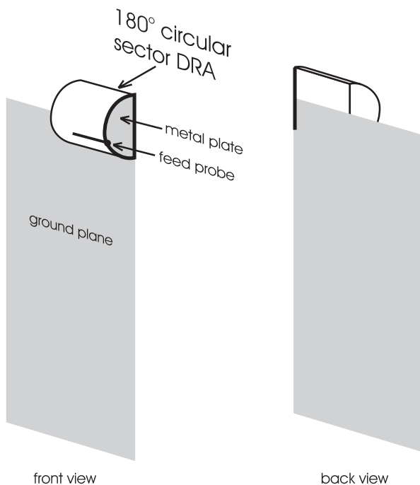
Figure 7.9: Proposed 180 degrees circular sector DRA design a=12\text{mm} , d=22\text{mm} mounted on a 100 \times 40\text{mm}^2 ground plane (from [5], © 1999 IEEE)
