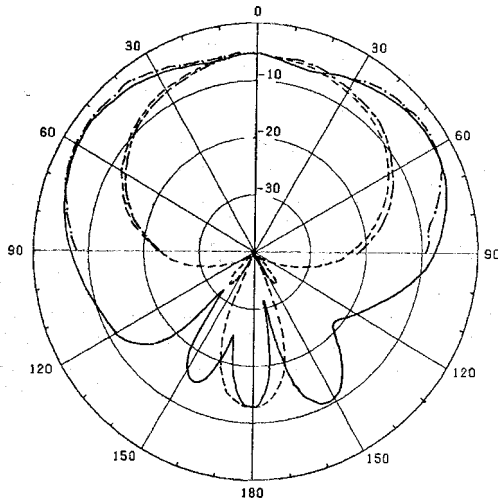
Fig. 4.28 Computed and measured far field radiation patterns of a dielectric resonator with a=0.1706\lambda , a/h=1.67 , \rho_t/a=0.95 , \epsilon_r=8.9 , and a circular ground plane of radius 1.297\lambda . (solid line) computed E-plane, (short dashes) computed H-plane, (dash dot) measured E-plane, and (long dashes) measured H-plane. (from [7] © 1989 IEEE Antenna and Propagation Magazine)
