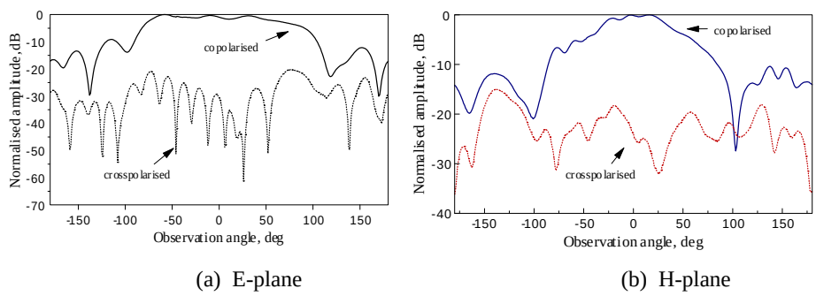
Fig. 1.33 Measured radiation patterns of the single element.
