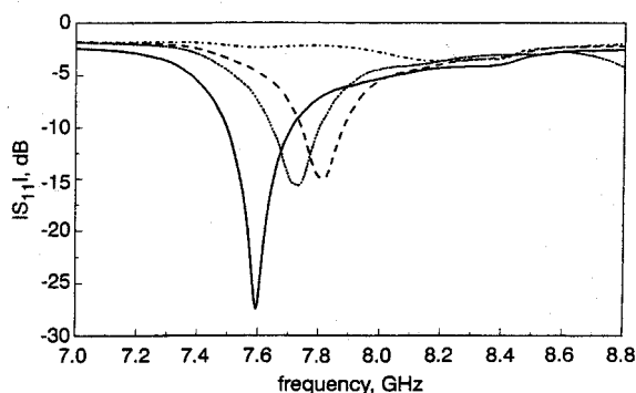
Fig. 6.22 Measured input reflection coefficient of the aperture-coupled triangular DR antenna for several offsets between the aperture and the resonator: — x'=0.99 mm, y'=-0.28 mm; ..... x'=-2.29 mm, y'=-1.03 mm - - - - x'=3.22 mm, y'=-0.42 mm; - . - . - x'=5.6 mm, y'=-0.98 mm (from [17], reprinted with permission from IEE)
