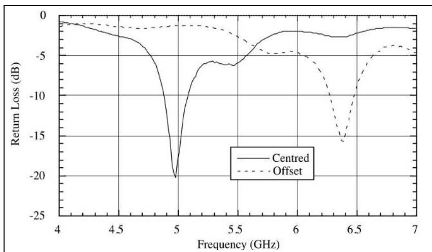
Figure 2.12 Measured return loss of aperture-fed DRA.
