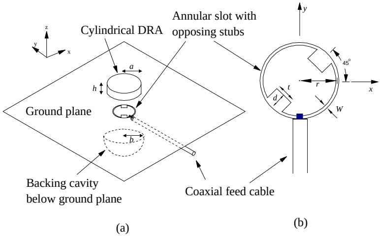
Fig. 1.24 The CP cylindrical DRA excited by the perturbed annular slot with a backing cavity. (a) Perspective view. (b) Perturbed annular slot with opposing stubs. (From [92], reprinted with permission from IEE)
