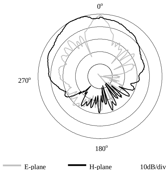
Fig. 10.14 Measured radiation pattern of the antenna.
