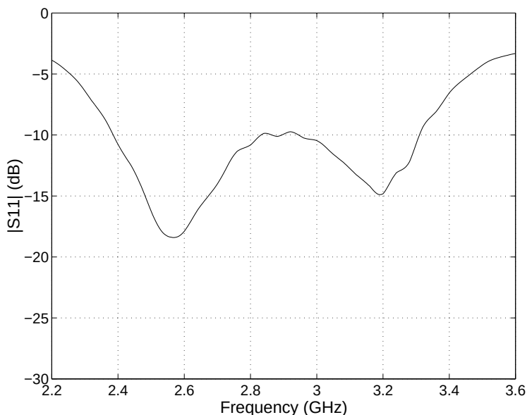
Figure 7.21: Measurement of the reflection coefficient, |S_{11}| , of the circularly polarised DRA. The DRA geometry is of \epsilon_r = 12 , \beta = 180 degrees, a = 18\text{mm} and d = 15\text{mm} (from [6], © 2000 IEEE)
