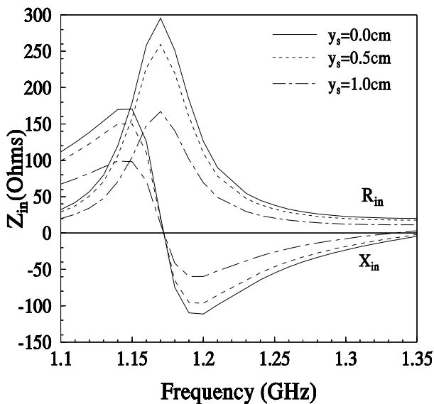
Fig. 4.43 Computed input impedances for the DRA excited by a slot/microstrip transmission line with a=2.75 cm, h=2.6 cm, \epsilon_r=12 , L_s = 4.0 cm, W_s=0.6 mm, \epsilon_s=2 , d=0.16 cm, w_f = 0.5 cm, and different microstrip line positions
