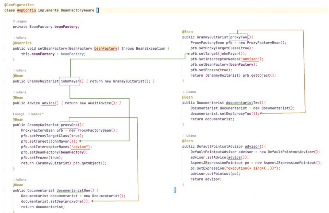
Figure 5-10. Declarative AOP configuration
