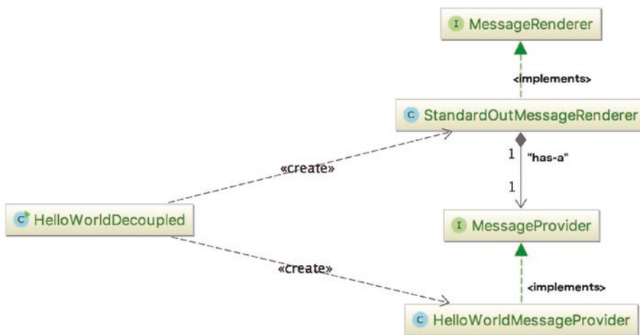
Figure 2-9. A little more decoupled Hello World application
