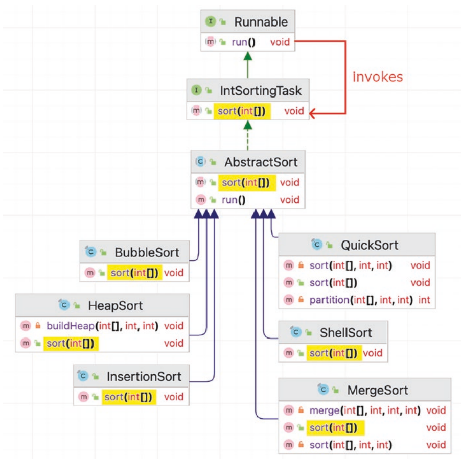
Figure 12-1. Hierarchy of classes modeling various sorting algorithms
