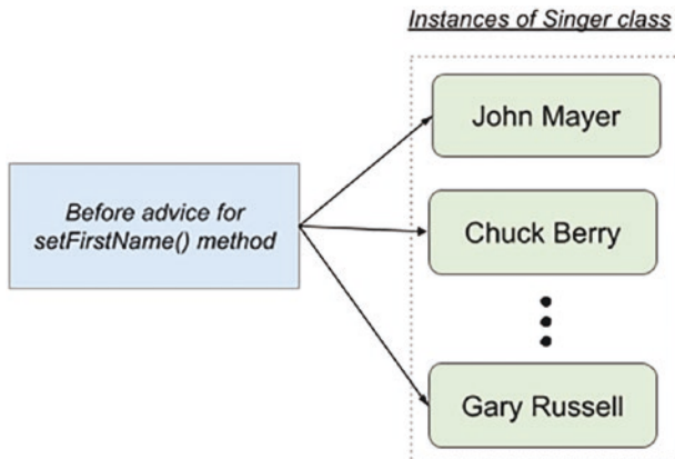
Figure 5-8. Per-class life cycle of advice
