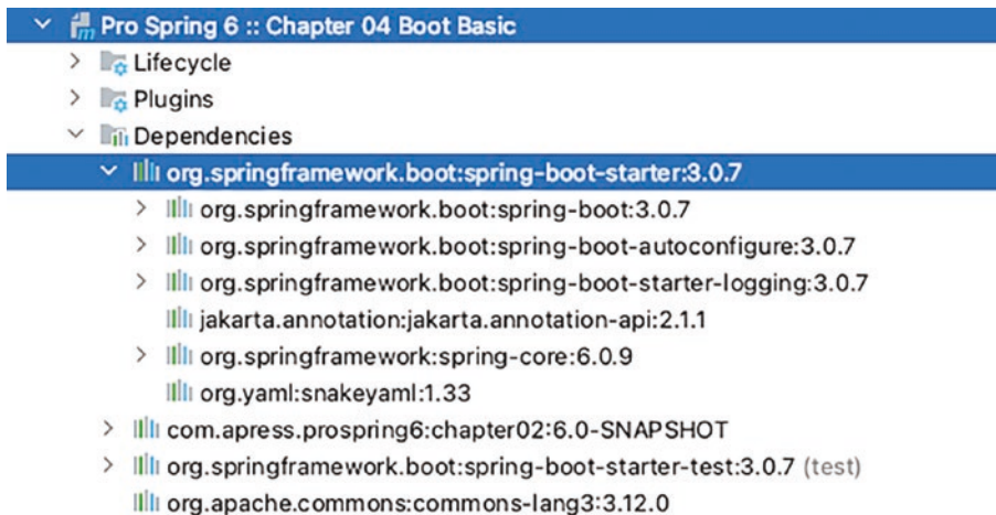
Figure 4-7. Spring Boot starter library and dependencies
