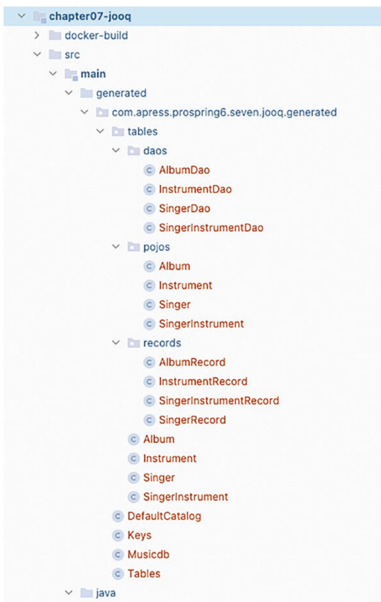
Figure 7-3. Classes generated by jOOQ
