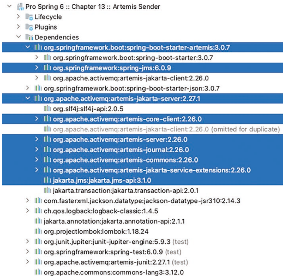
Figure 13-4. Spring Boot Artemis JMS project dependencies
