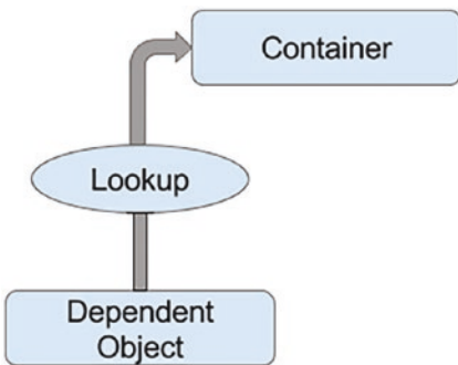
Figure 3-2. Contextualized dependency lookup
