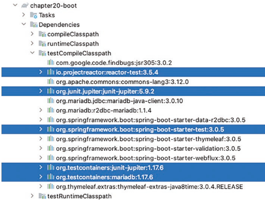
Figure 20-3. Project chapter20-boot test dependencies
