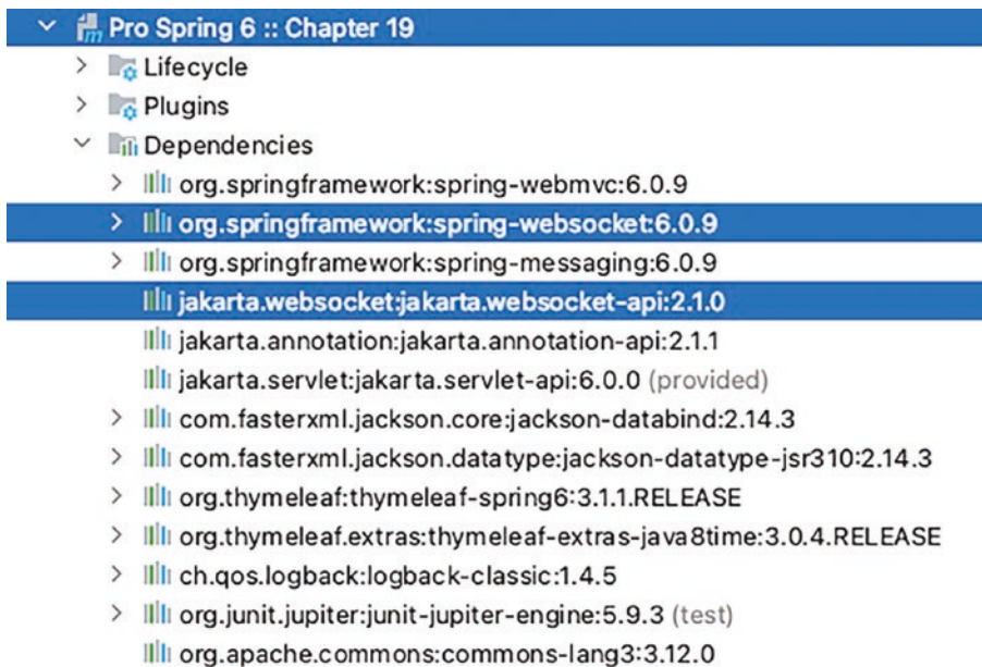
Figure 19-1. Project chapter19 dependencies
