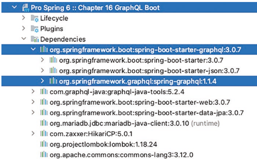
Figure 16-9. Dependencies for project chapter16-graphql-boot
