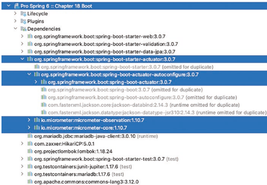
Figure 18-6. Project chapter18-boot dependencies
