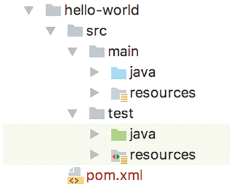
Figure 2-5. Maven typical project structure
