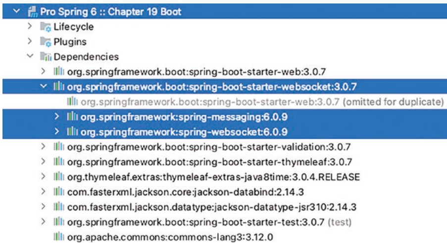
Figure 19-8. Project chapter19-boot dependencies
