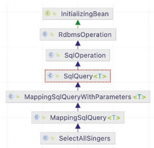
Figure 6-3. SelectAllSingers class hierarchy
