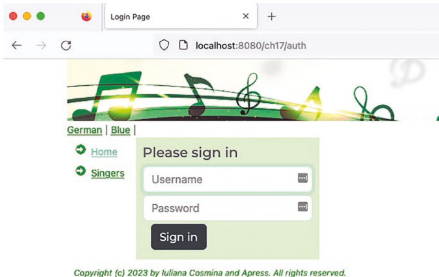
Figure 17-5. Custom login form configured with Spring Security
