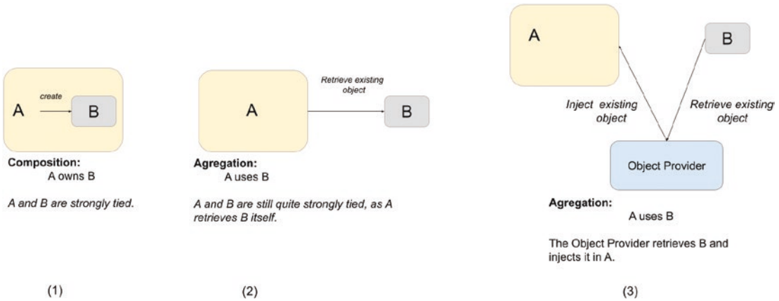
Figure 1-1. Object relationships and how they “meet”
