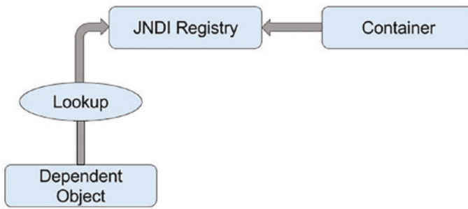
Figure 3-1. Dependency pull via JNDI lookup
