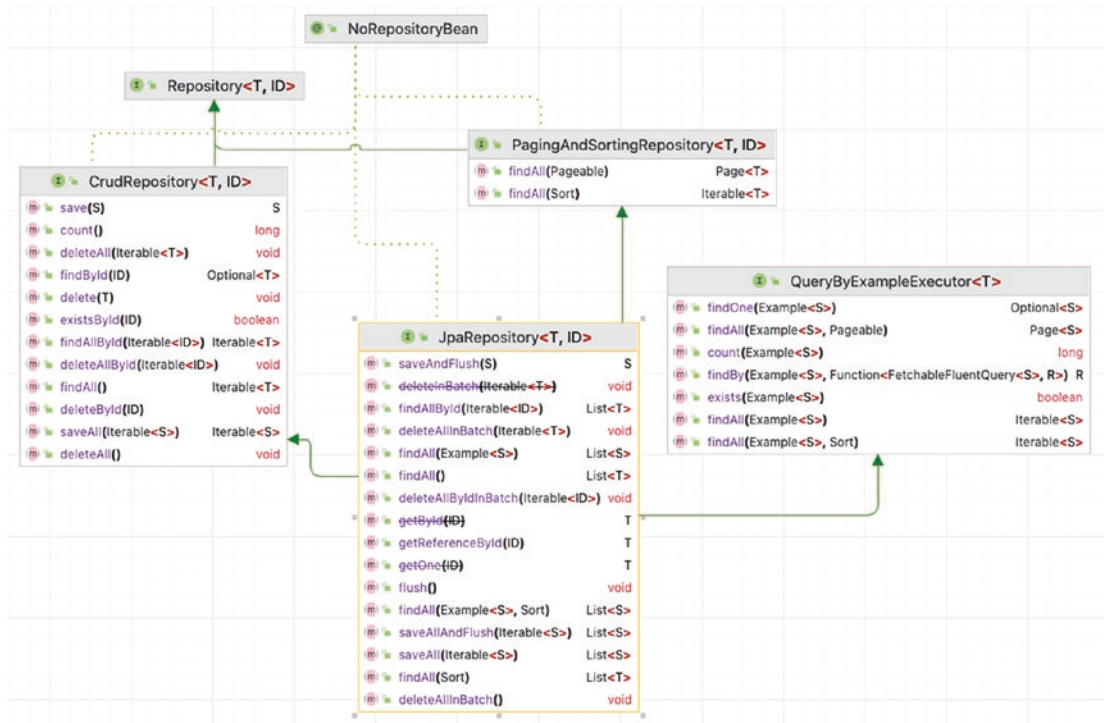
Figure 10-3. Spring Data JpaRepository<T, ID> hierarchy
