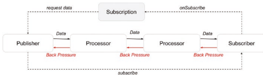
Figure 20-1. Reactive Streams specification abstract representation
