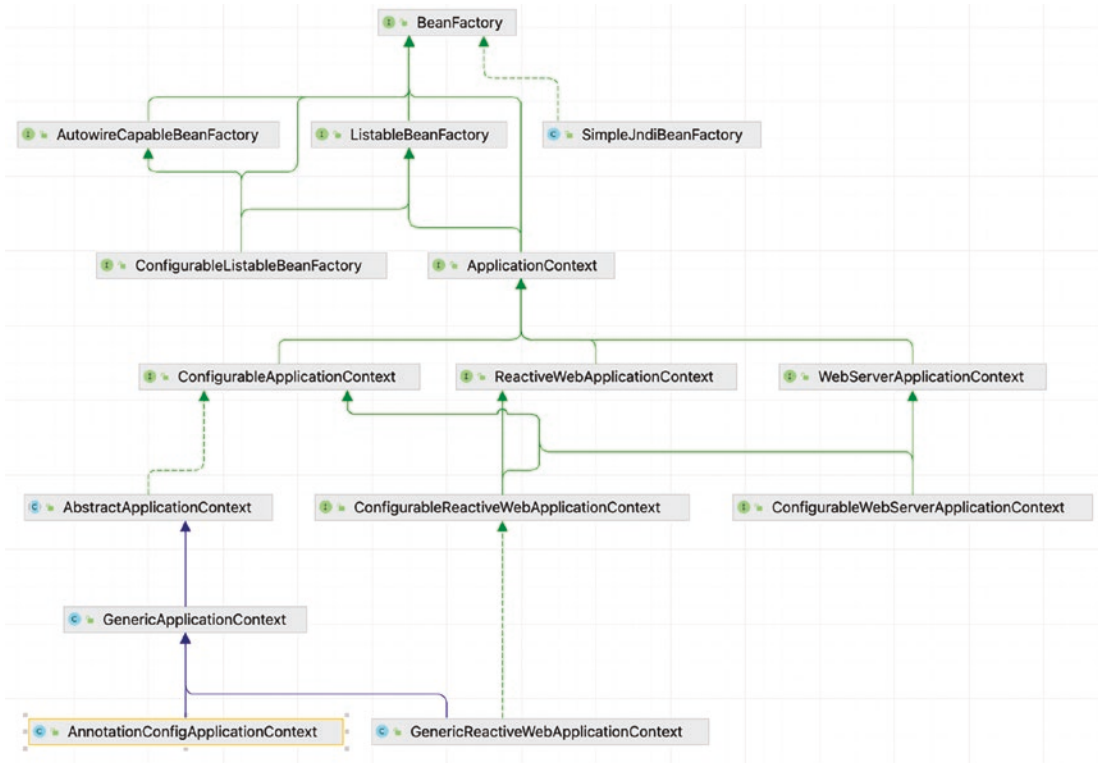
Figure 3-4. BeanFactory most common implementations
