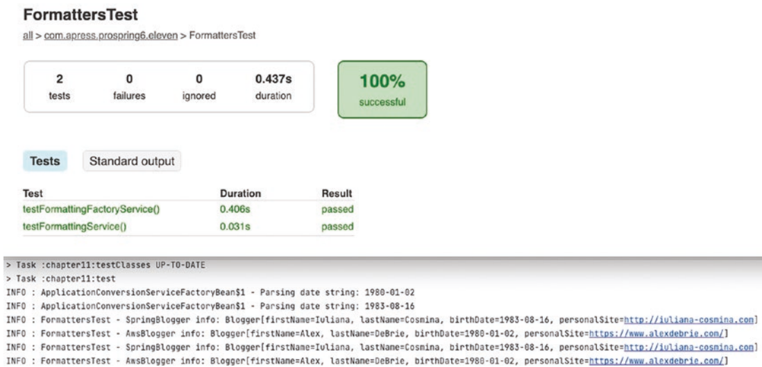
Figure 11-1. Gradle test result page and log showing the test methods under FormattersTest passing
