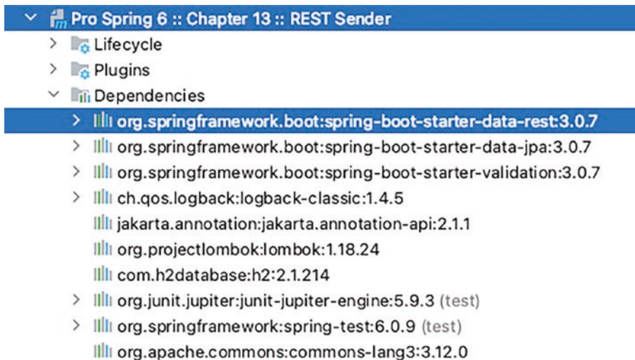
Figure 13-2. Project chapter13-sender-boot dependencies
