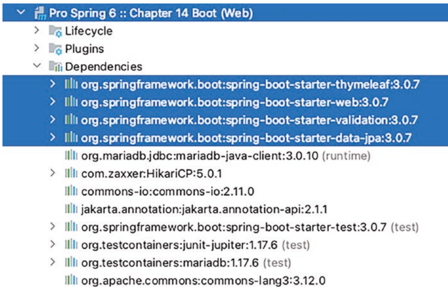
Figure 14-15. Spring Boot web application dependencies
