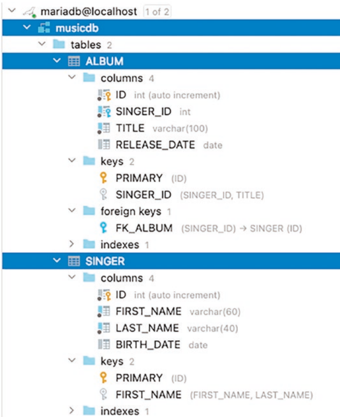
Figure 6-2. Contents of the musicdb schema
