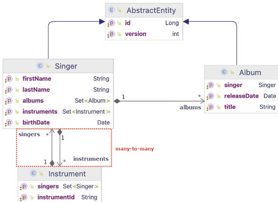
Figure 7-2. Class diagram for the sample data model
