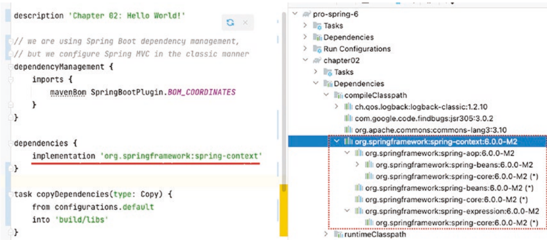
Figure 2-10. Gradle View showing spring-context and its dependencies
