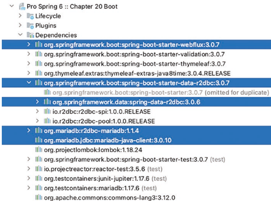
Figure 20-2. Project chapter20-boot dependencies
