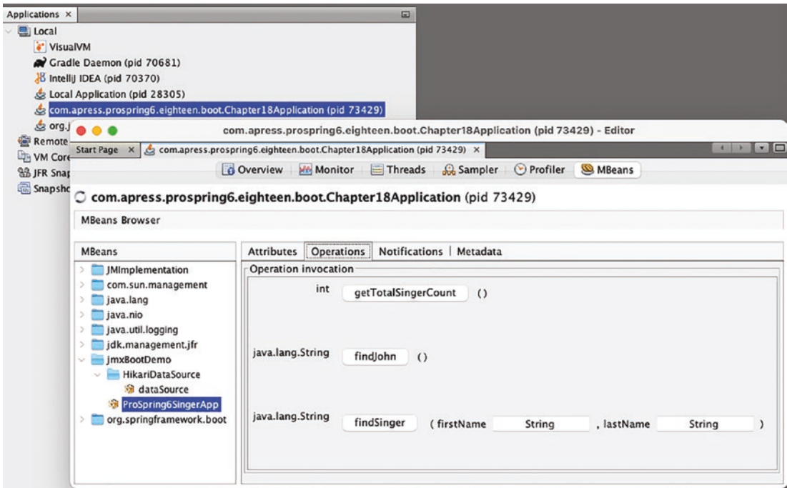
Figure 18-4. Operations for the ProSpring6SingerApp MBean declared in the chapter18-boot project
