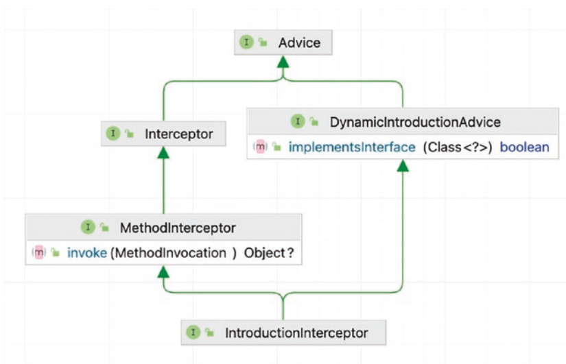
Figure 5-7. IntroductionInterceptor interface hierarchy
