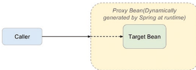
Figure 5-1. Spring AOP proxy in action
