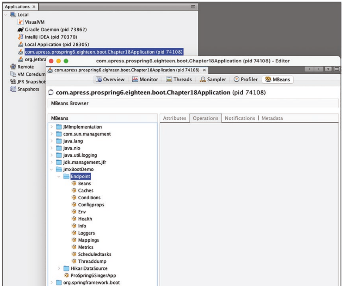
Figure 18-7. Spring Boot Actuator JMX endpoints shown in VisualVM
