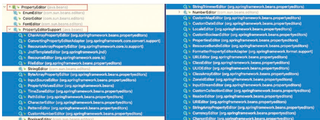
Figure 4-2. Spring PropertyEditor implementations
