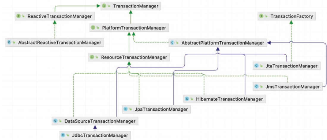
Figure 9-2. PlatformTransactionManager implementations
