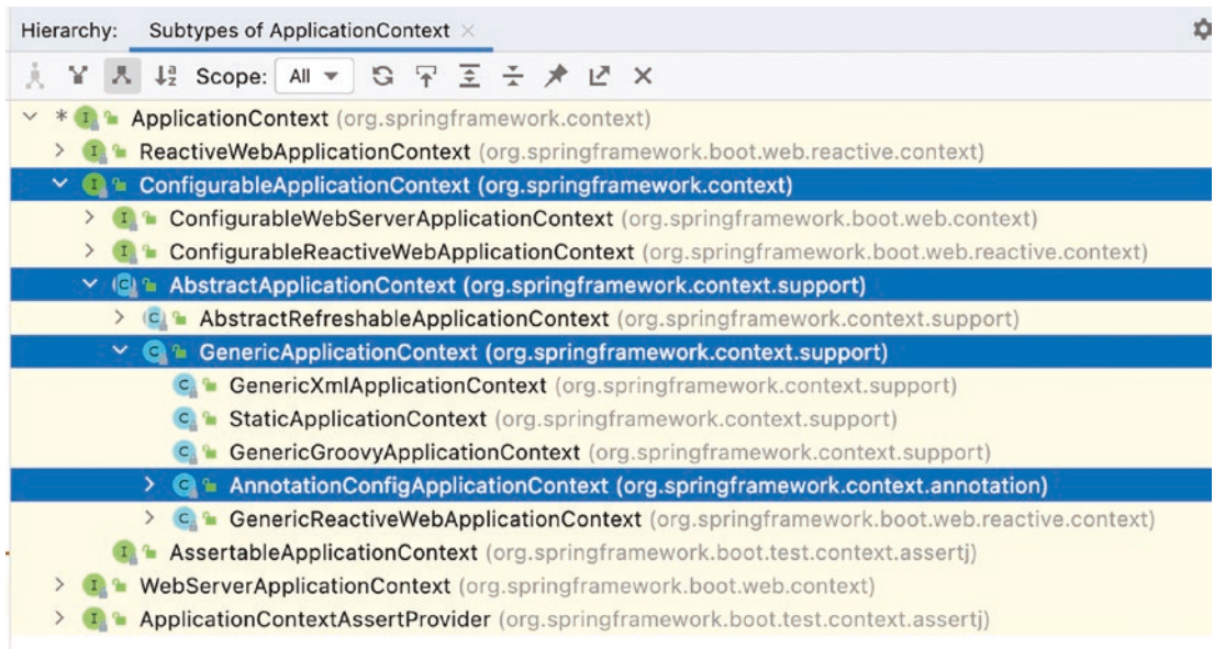
Figure 3-5. AnnotationConfigApplicationContext hierarchy
