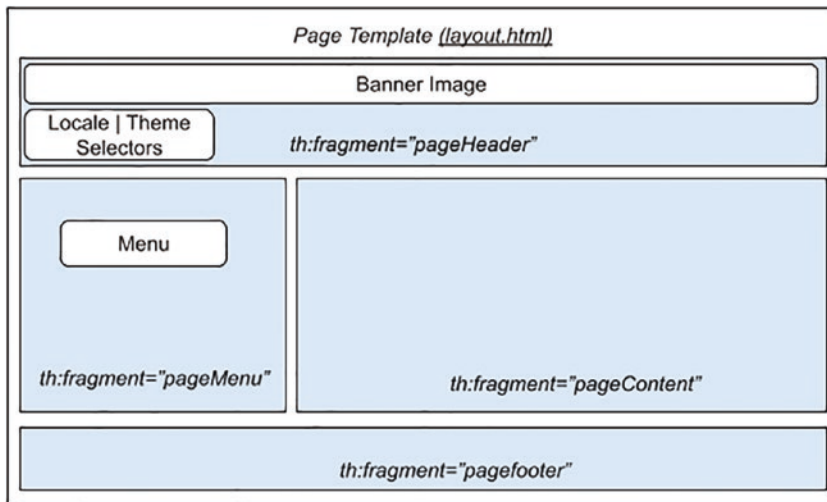
Figure 14-9. Thymeleaf template with fragments
