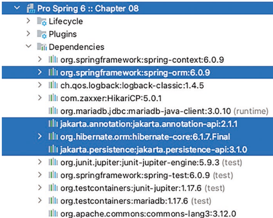
Figure 8-1. Spring with Hibernate JPA project dependencies
