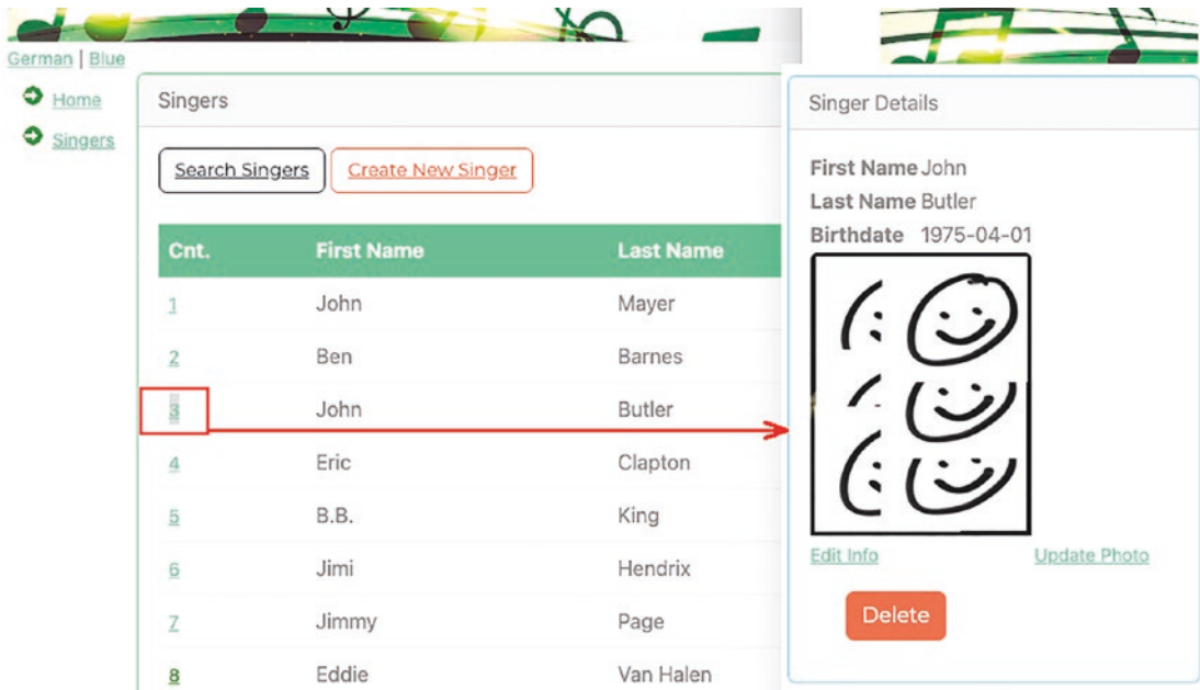
Figure 14-10. List and show views
