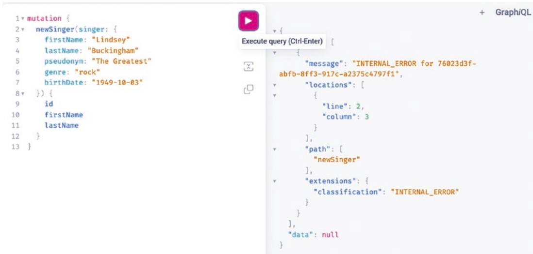
Figure 16-12. GraphQL web console showing an error when trying to execute the same mutation twice
