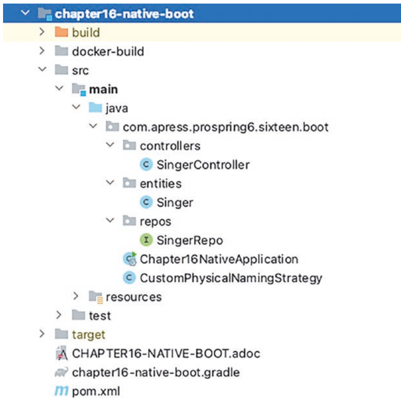
Figure 16-1. Project chapter16-native-boot structure
