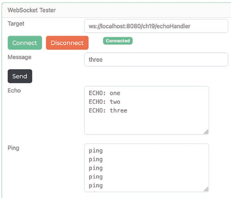
Figure 19-3. WebSocket client page
