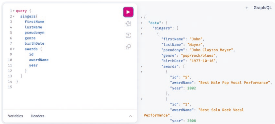
Figure 16-11. GraphQL web console with a nested query
