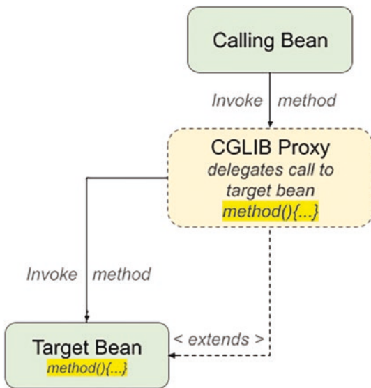
Figure 5-5. CGLIB proxy abstract schema
