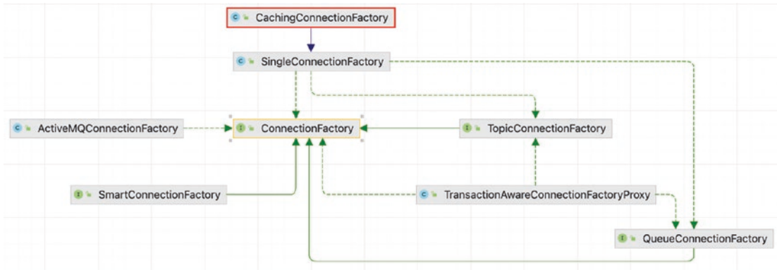
Figure 13-5. jakarta.jms.ConnectionFactory hierarchy
