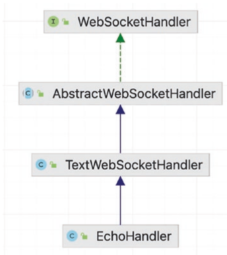
Figure 19-2. WebSocketHandler implementations
