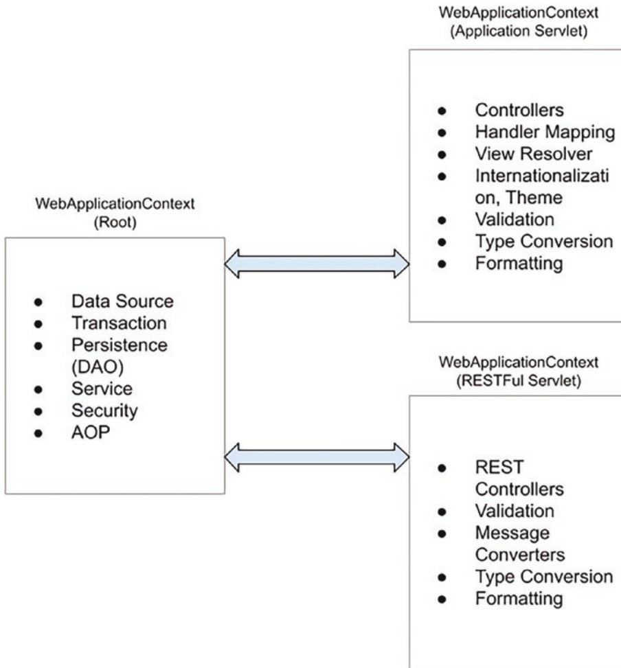
Figure 14-2. Spring MVC WebApplicationContext hierarchy
