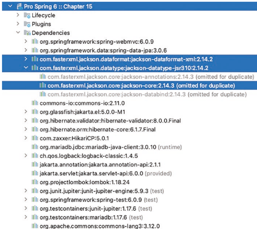
Figure 15-1. Project chapter15 dependencies
