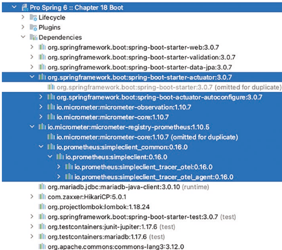
Figure 18-9. Spring Boot Actuator and Prometheus application dependencies
