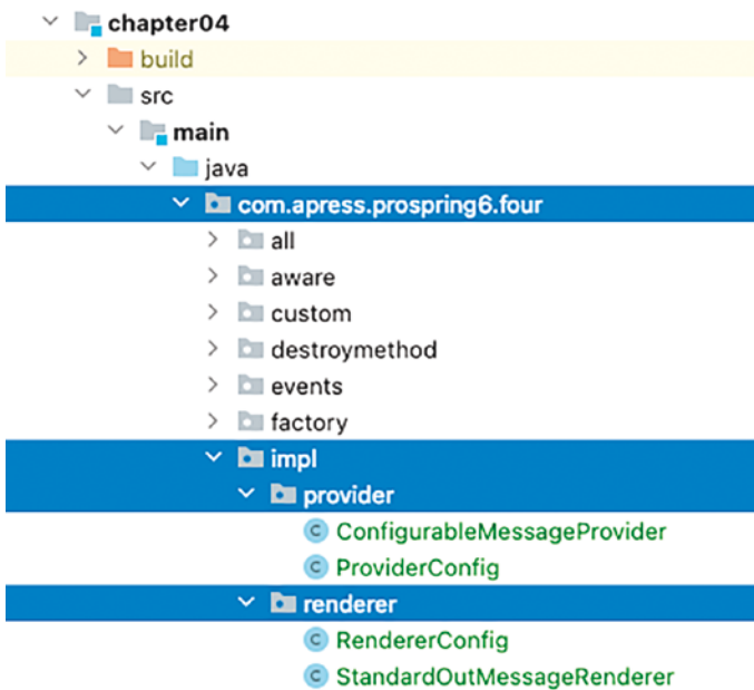
Figure 4-6. Organizing beans with their own configuration
