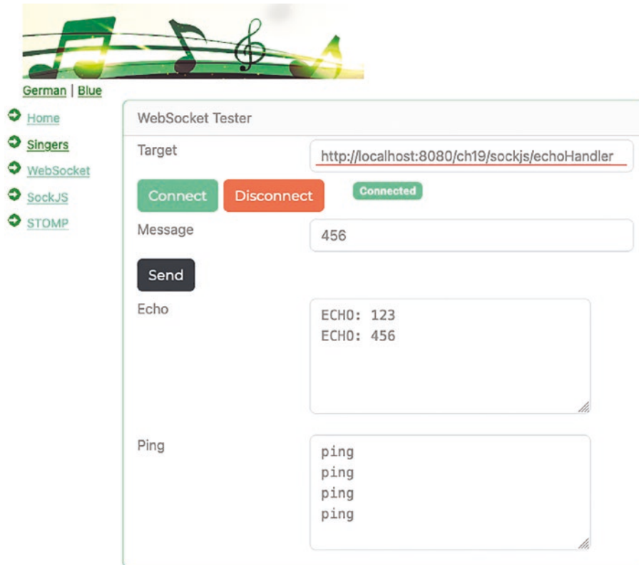
Figure 19-4. SocketJS application page, after establishing a connection
