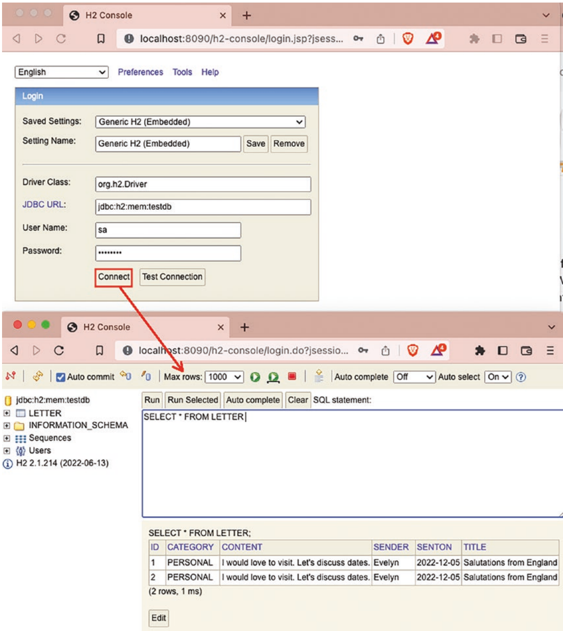
Figure 13-3. H2 Console login and dashboard
