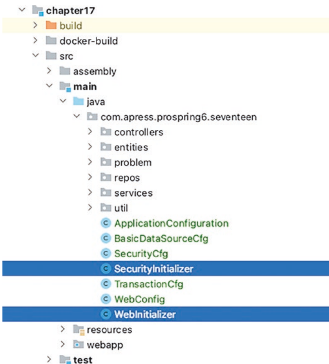
Figure 17-2. Project chapter17 configuration classes
