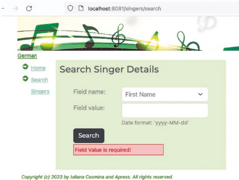
Figure 20-7. Search Singer page with a validation error message
