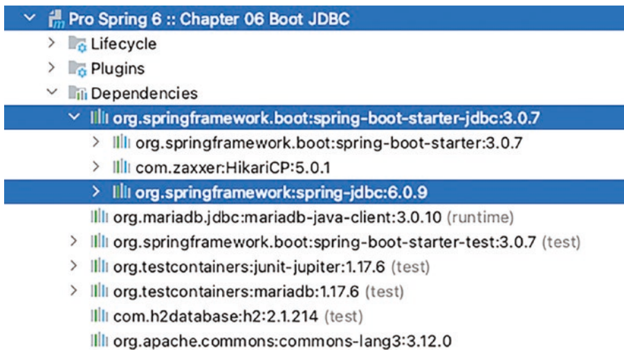
Figure 6-7. Spring Boot JDBC starter dependencies
