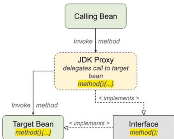
Figure 5-4. JDK proxy abstract schema
