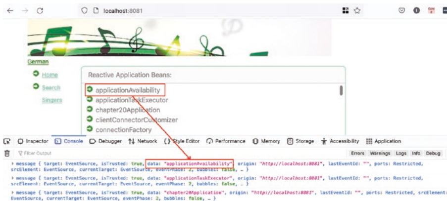
Figure 20-6. Server-sent events displayed in Firefox's developer console
