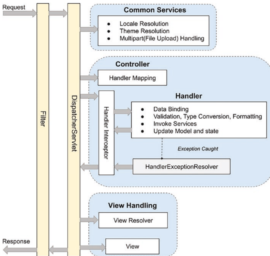
Figure 14-3. Spring MVC Request Handling Components
