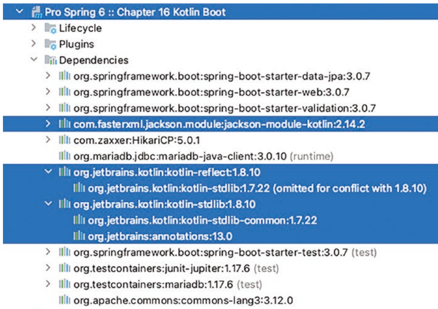
Figure 16-14. chapter16-kotlin-boot project dependencies
