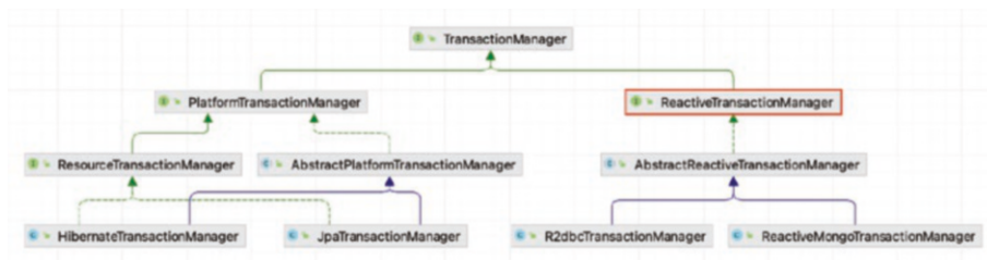
Figure 20-4. TransactionManger imperative and reactive hierarchy, side by side
