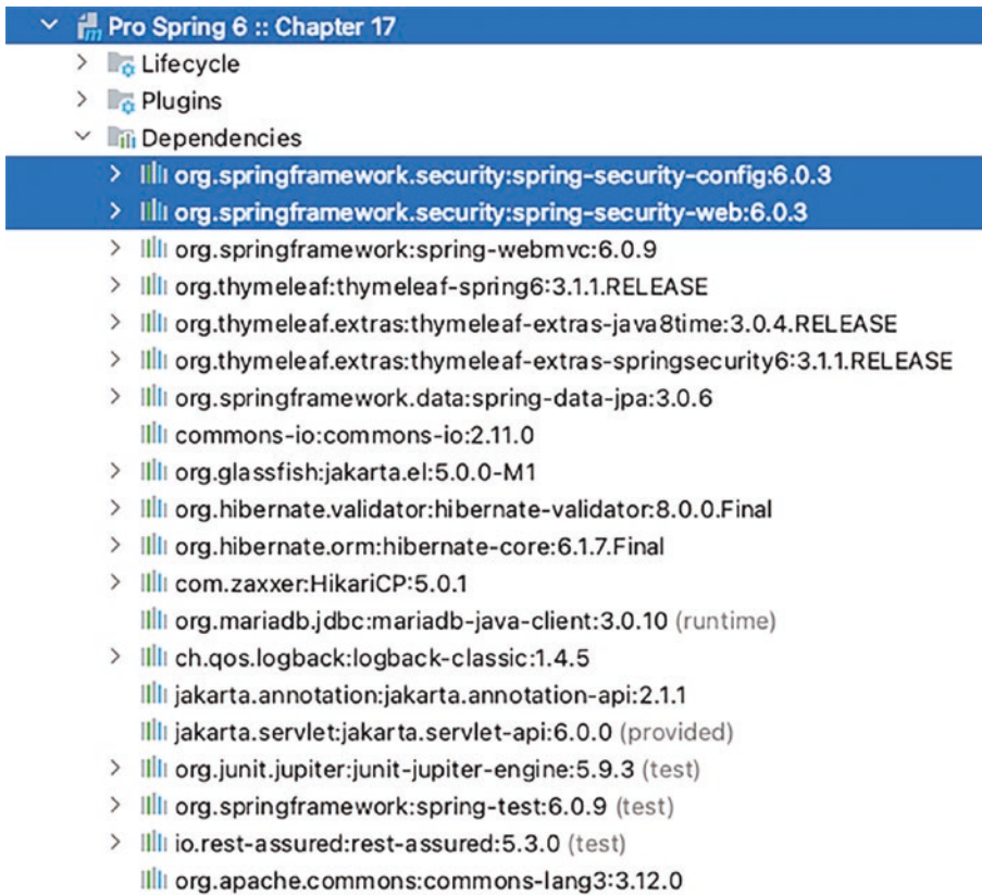
Figure 17-1. Project chapter17 dependencies
