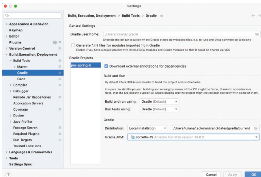
Figure A-8. IntelliJ IDEA JDK configuration pop-up for Gradle.
