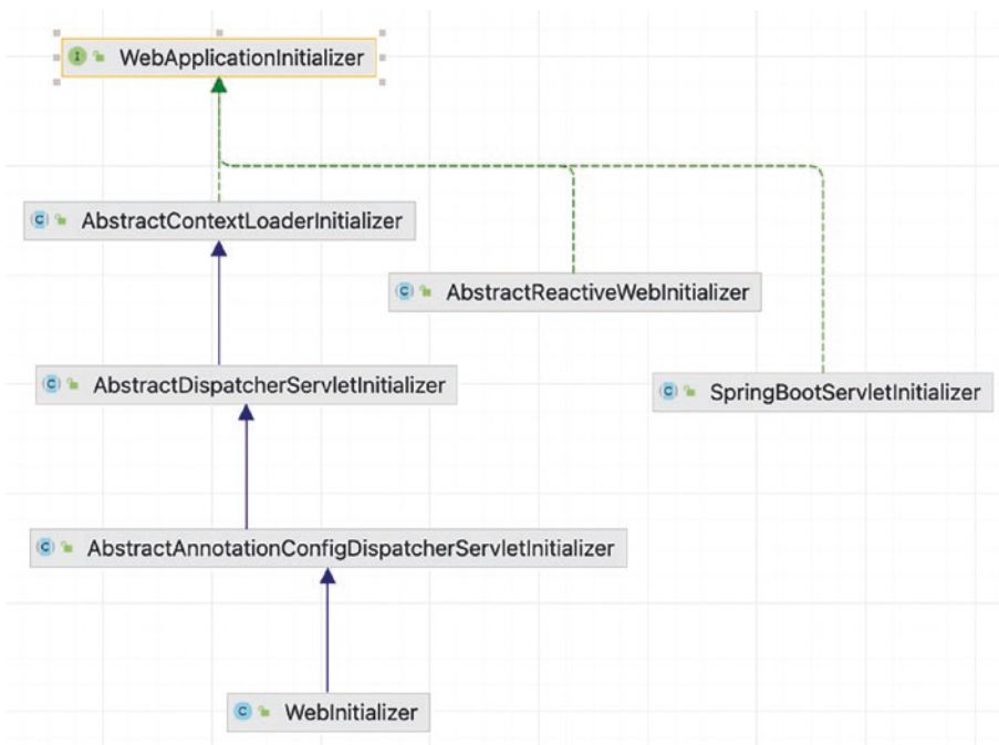
Figure 14-4. SpringWebApplicationInitializer implementations
