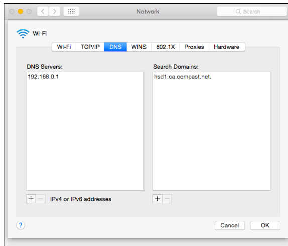
FIGURE 4-4: DNS settings.
