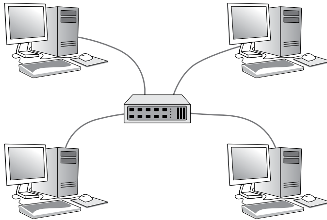
FIGURE 1-5: Star topology.
