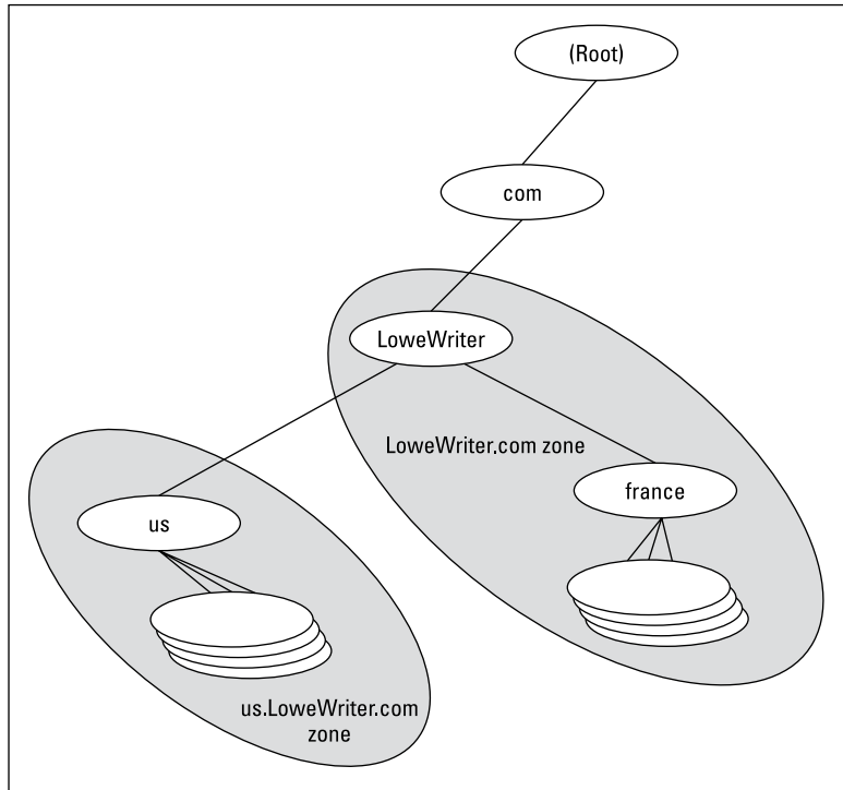
FIGURE 6-2: DNS zones.
