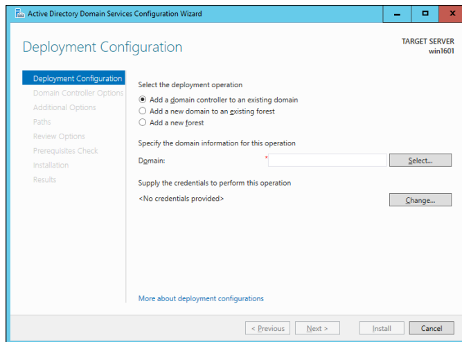
FIGURE 3-4: Creating a domain controller.
