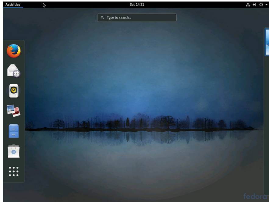
FIGURE 2-2: The desktop.
