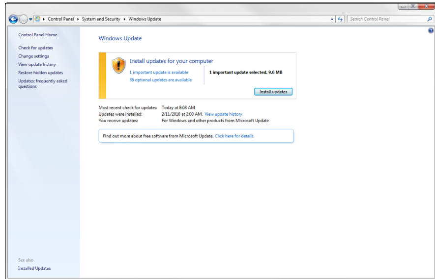
FIGURE 6-1: Windows Update.
