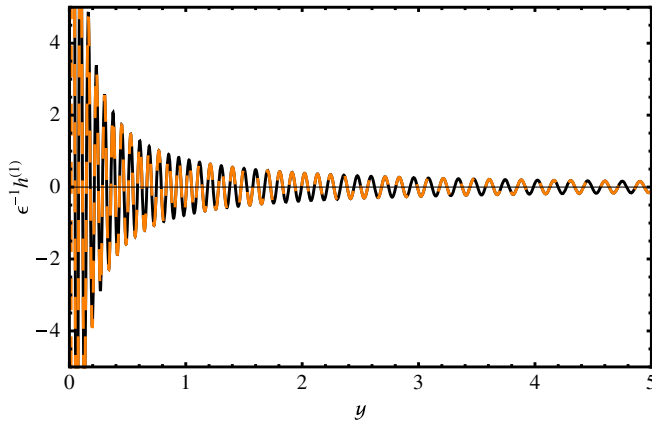
FIG. 3. The effect of collisionless matter on the time evolution of a mode with \kappa = 100 . We show the term of order \epsilon of the approximation to the mode function given in equation (93) (dashed orange) and the difference between the numerical solutions of the equation of motion with and without anisotropic stress (black).
