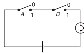
(a) Switching circuit for and-function
