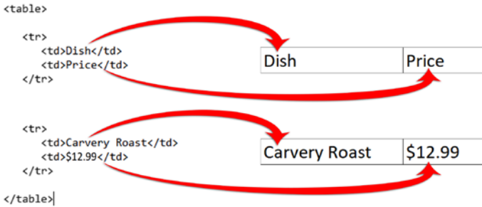
Figure 3-24. Creating a Table
