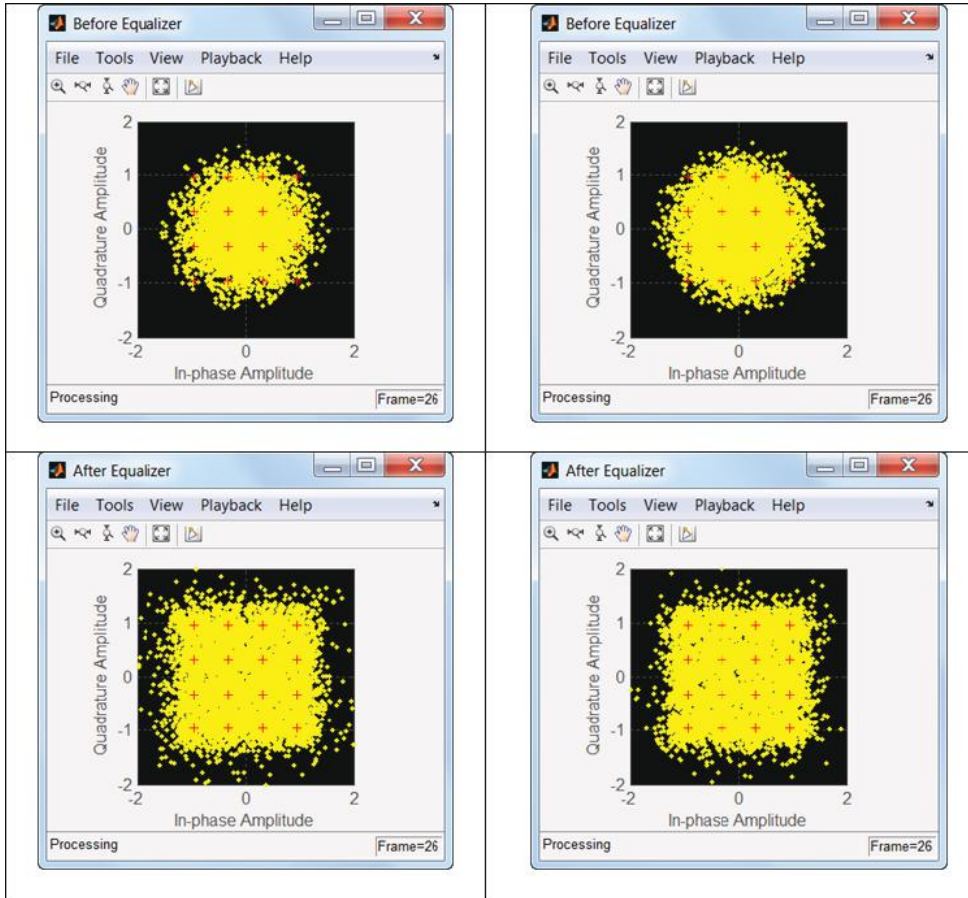
Figure 8.5 Constellation of received signals: before and after MIMO detection
