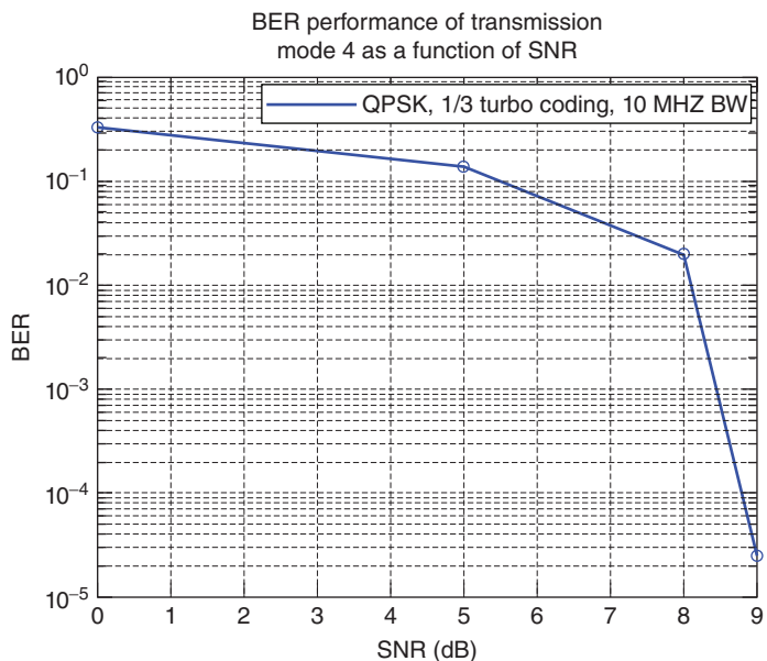
Figure 6.14 BER results: LTE mode 4 spatial-multiplexing single-codeword (2 × 2) MIMO channel
