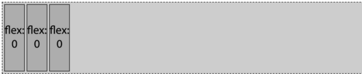
Flex container ↗
