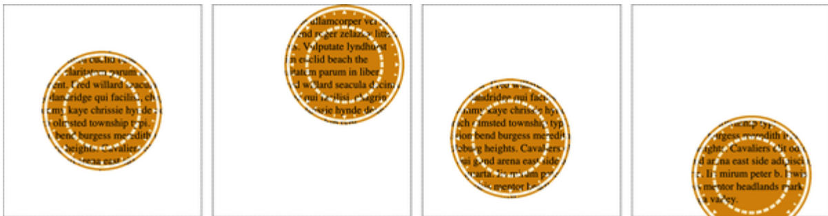
Figure 20-47. Positioning masks
