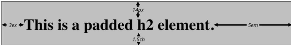
Figure 7-4. Mixed-value padding
