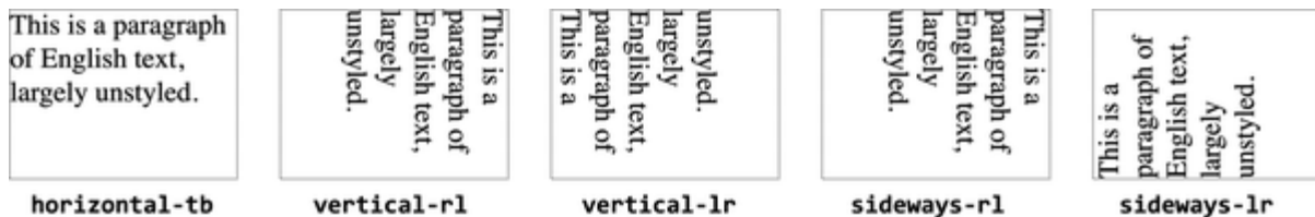
Figure 15-43. Writing modes
