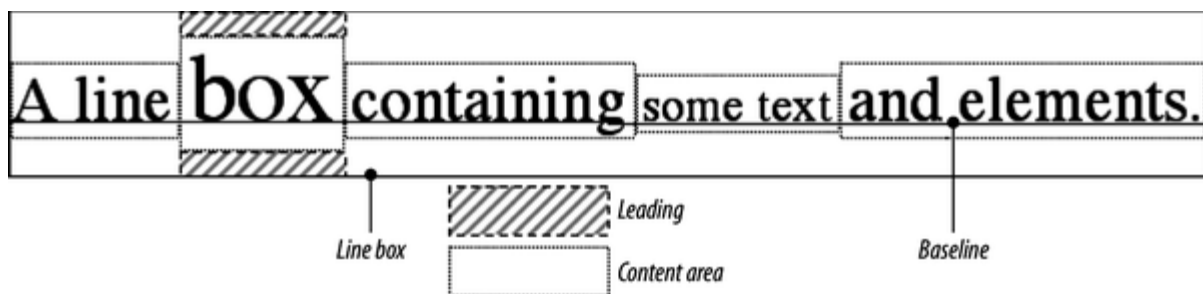
Figure 15-12. Line-box diagram
