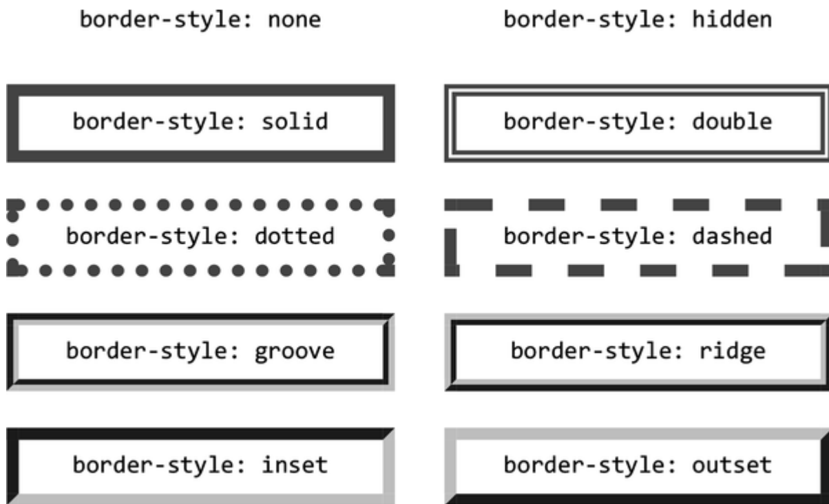
Figure 7-17. Border styles
