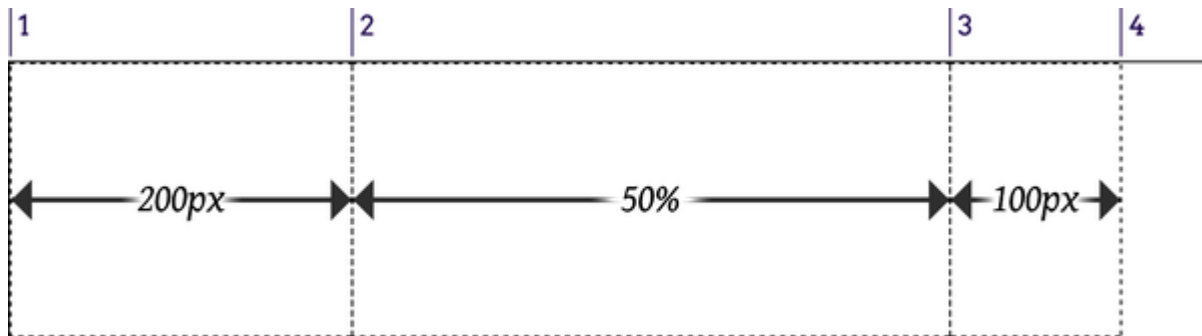
Figure 12-7. Grid-line placement
