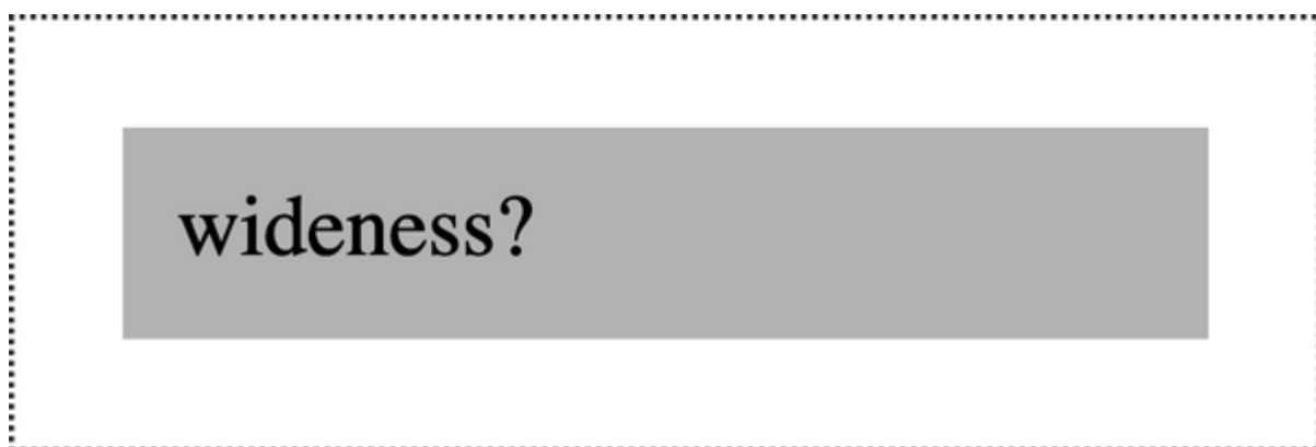
Figure 6-28. Subtractive padding
