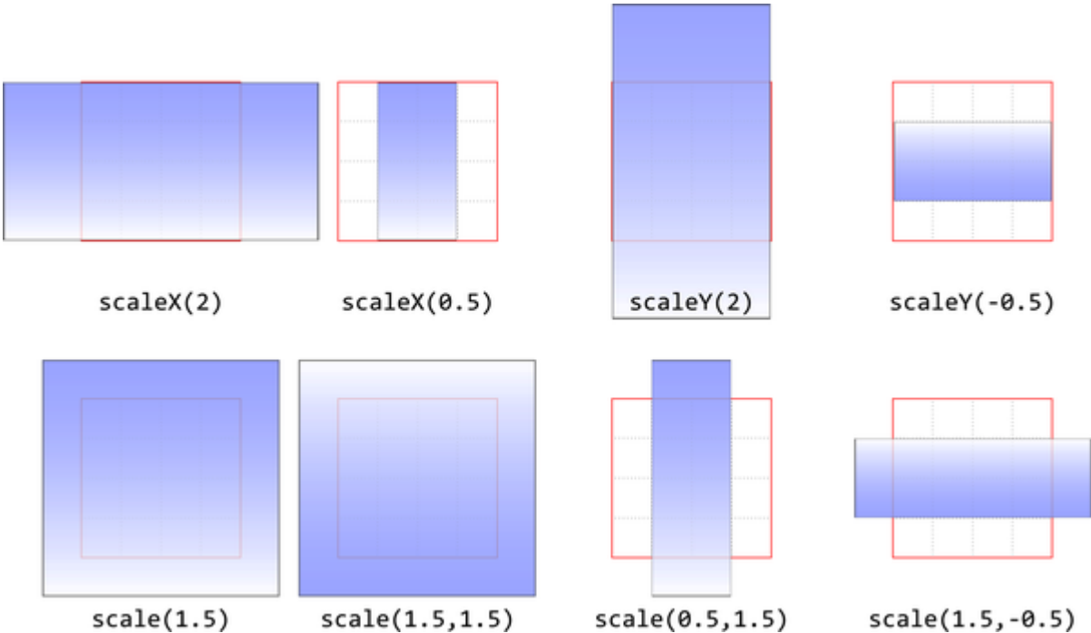
Figure 17-11. Scaled elements
