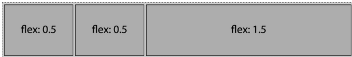
Flex container ↗
