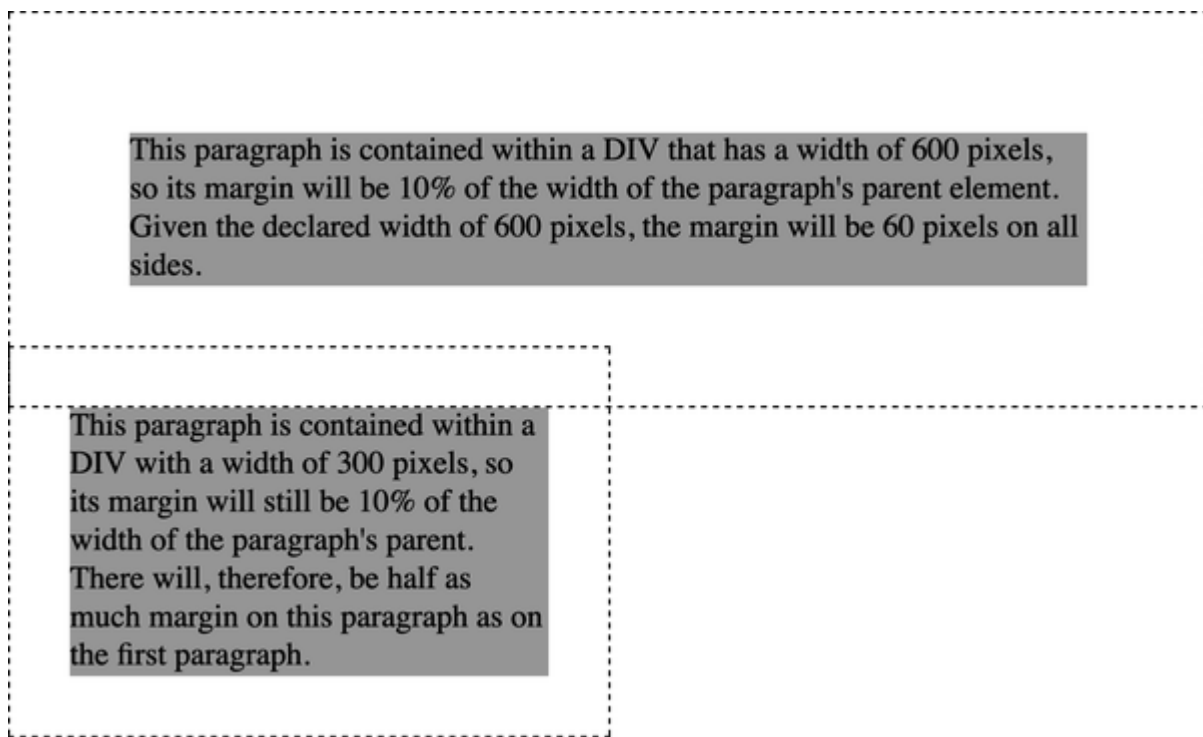
Figure 7-74. Collapsing margins
