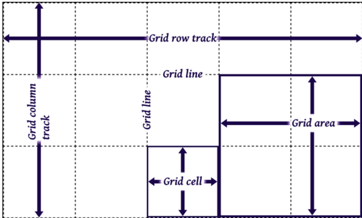
Figure 12-5. Grid components
