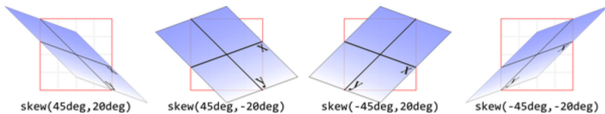
Figure 17-17. Skewed elements
