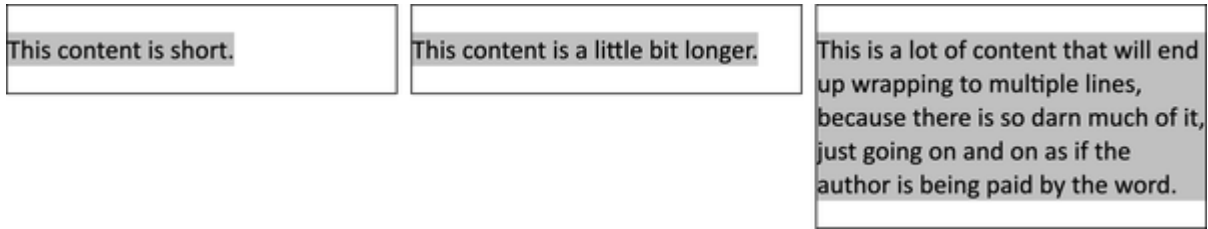
Figure 6-9. Fit-content sizing
