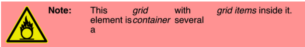
Figure 12-4. Grid items
