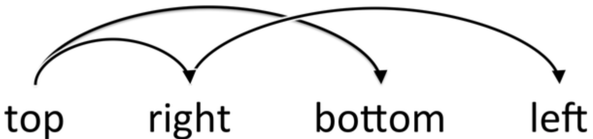
Figure 7-5. Value-replication pattern
