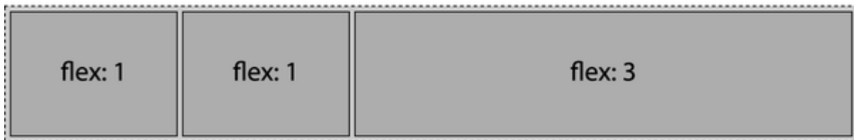
Flex container ↗
