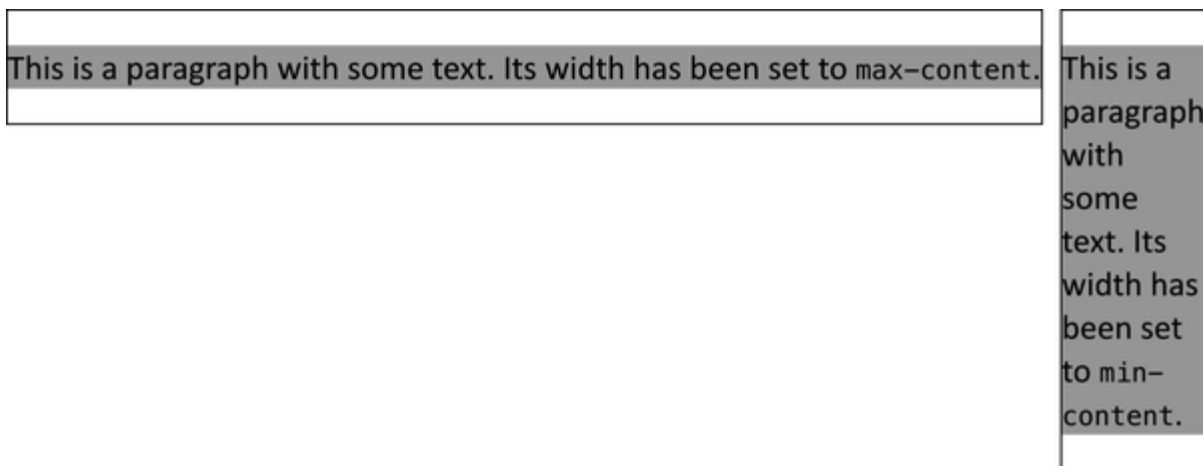
Figure 6-7. Content sizing
