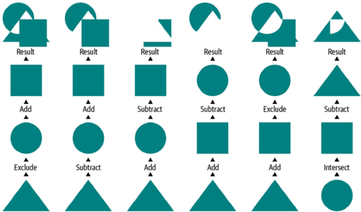
Figure 20-51. Compositing masks
