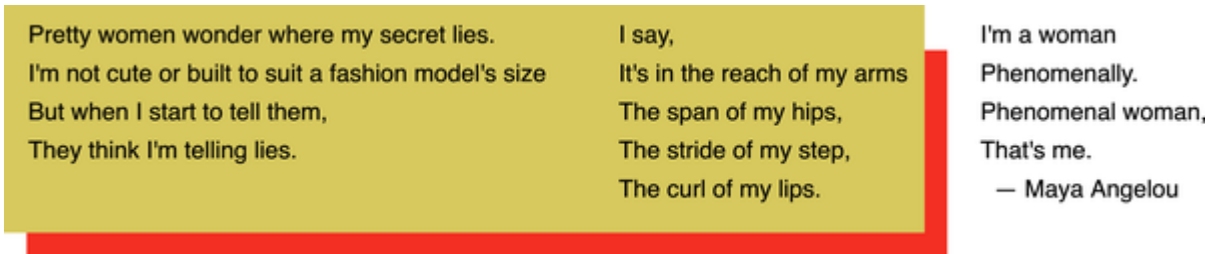
Figure 9-3. Solid-color gradients
