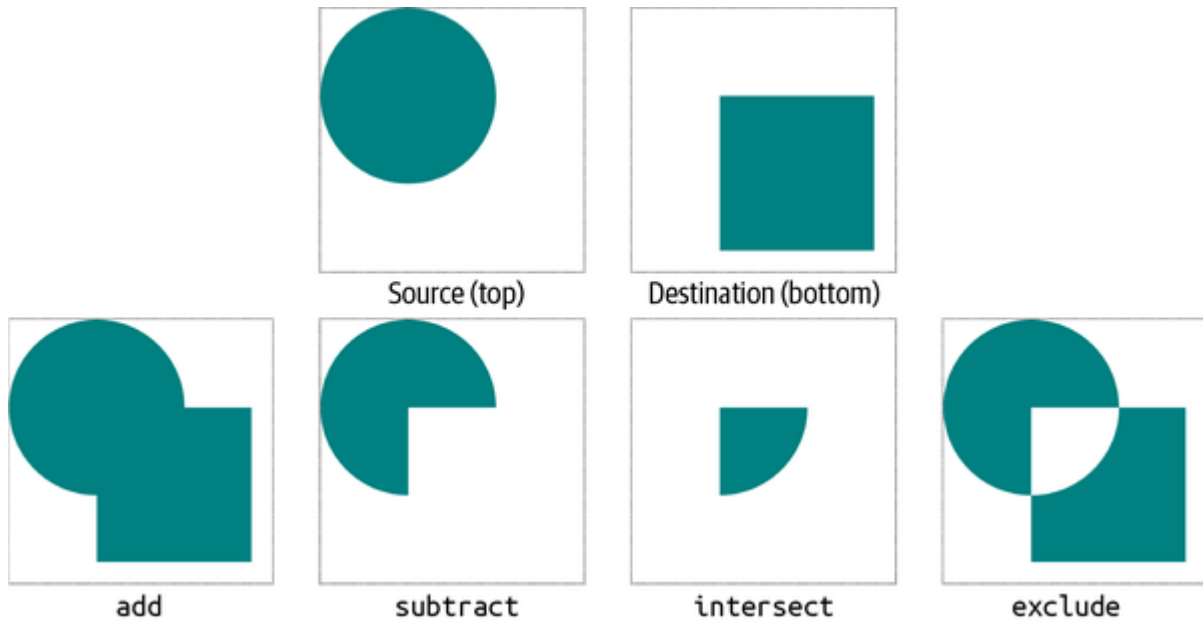
Figure 20-50. Compositing operations
