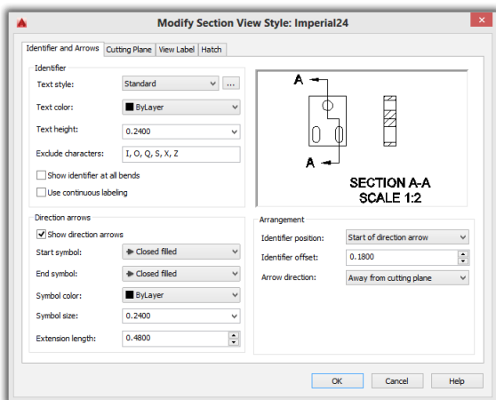
Left: AutoCAD's tabbed Modify Section View Style dialog box; right: BricsCAD's version in the Drawing Explorer
