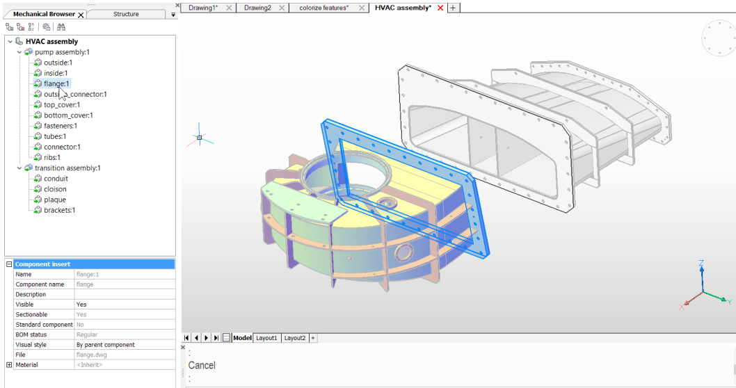
Assembly of sheet metal parts in BricsCAD
