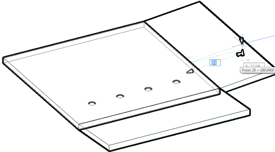
Two edges selected to bend
