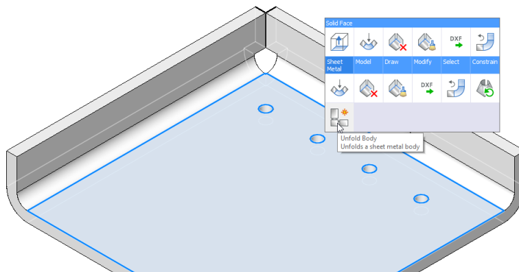
Accessing the smUnfold command
