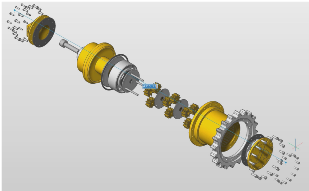
Exploding an assembly in BricsCAD Mechanical
