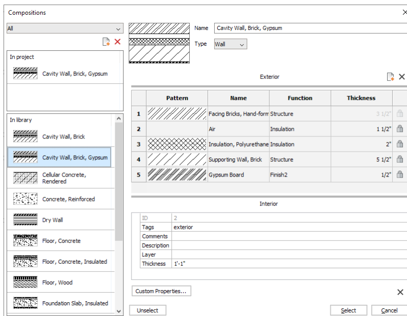
Selecting a composition for the walls
