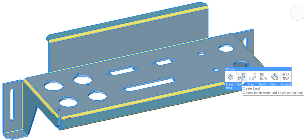
BricsCAD using color coding to indicate sheet metal elements
