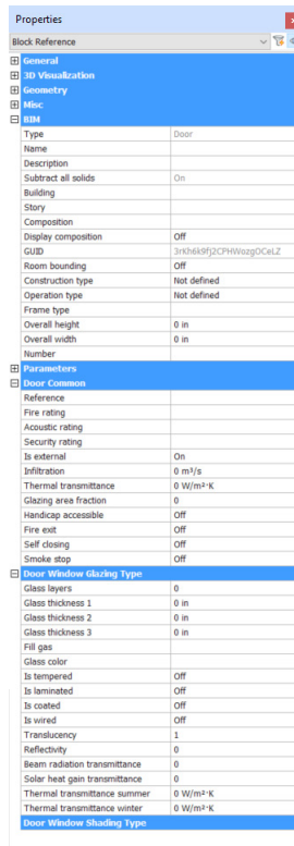
Properties panel showing IFC data for a door
