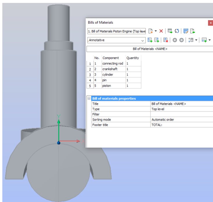
Bill of materials generated by BricsCAD automatically
