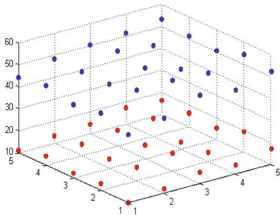
Fig. 5.3 The scatter diagram as behavior matrix
