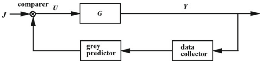
Fig. 11.10 Grey predictive control
