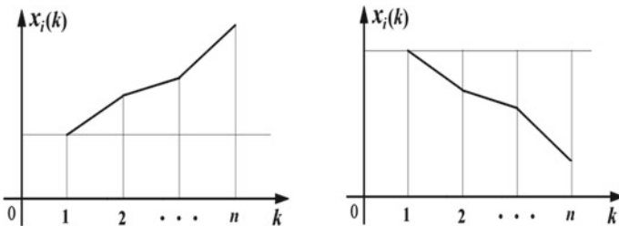
Fig. 5.6 Monotone sequence curves
