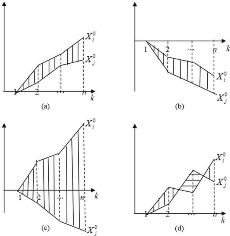
Fig. 5.8 Positional relationship of X_i^0 and X_j^0
