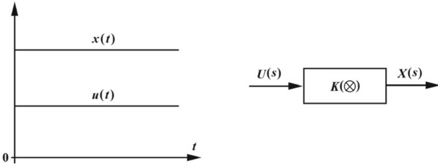
Fig. 11.4 The grey proportional link
