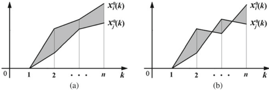
Fig. 5.2 A description of the relationship between X_i^0 and X_j^0
