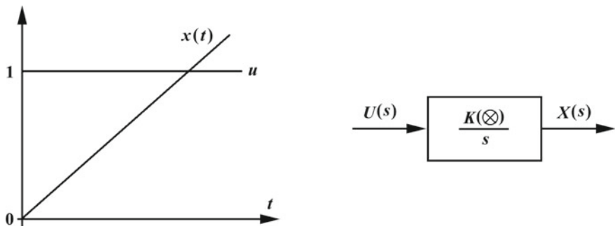
Fig. 11.6 The grey integral link
