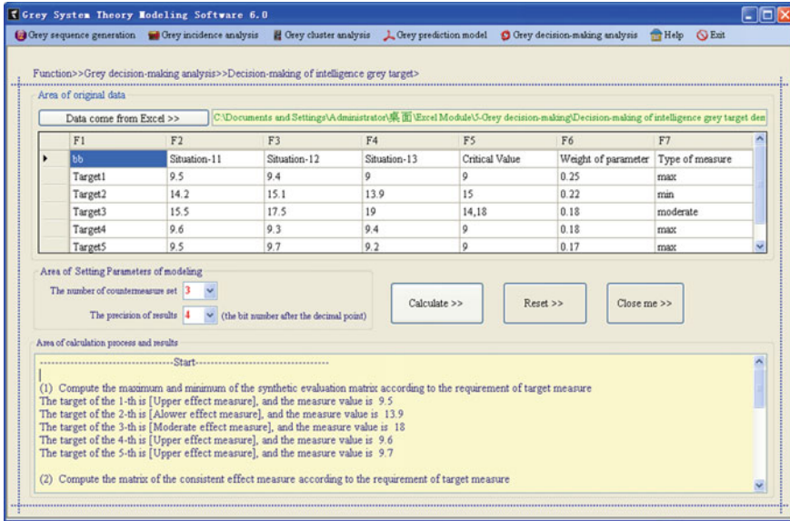
Fig. A.15 The entire operating page of multi-attribute grey target decision-making
