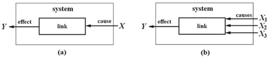
Fig. 9.3 Depicted causal relationships
