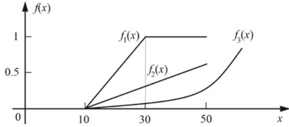
Fig. 3.1 Different types of possibility functions
