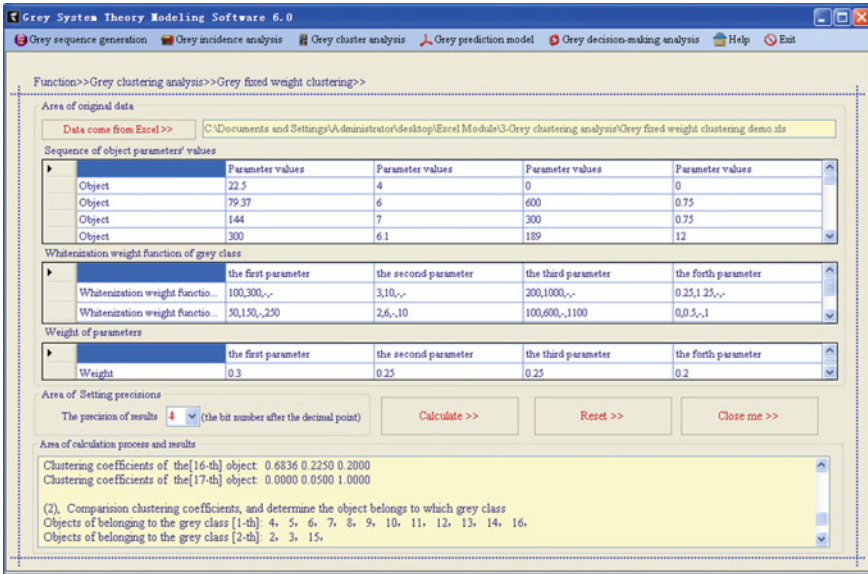
Fig. A.12 The operating interface of a grey clustering evaluation
