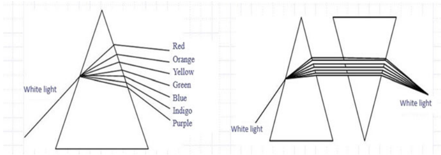
Fig. 12.2 Decomposition and synthesis of white light
