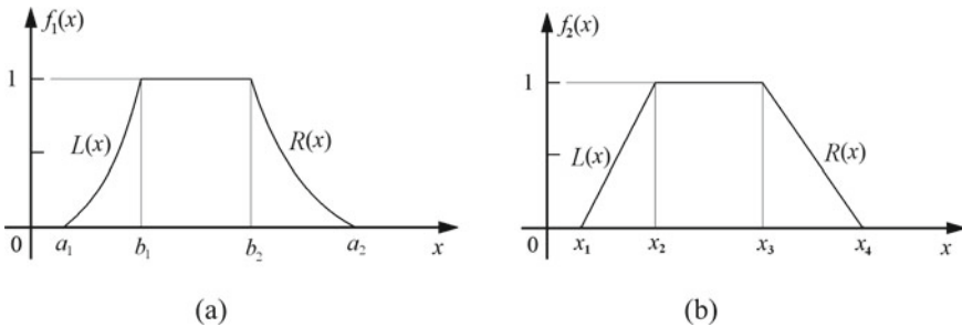
Fig. 3.2 Typical possibility function
