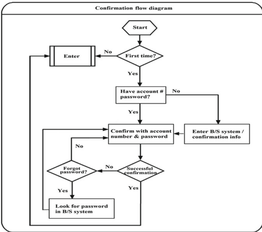
Fig. A.2 The confirmation flow chart
