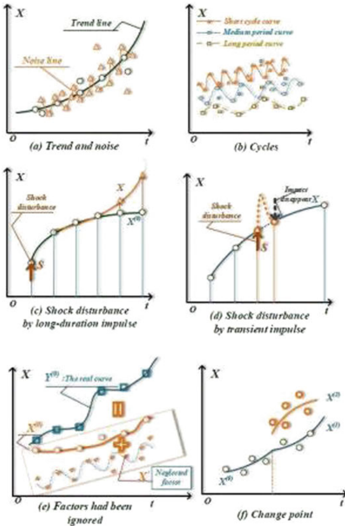
Fig. 12.1 Various factors of a data sequence
