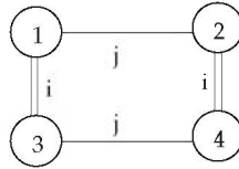
Figure 5. Within an i -face.
