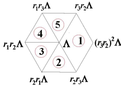
Figure 10. The vertices connected to the vertex \Lambda .
