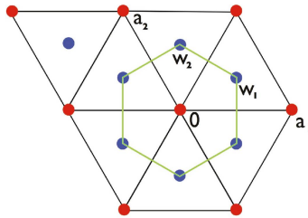
Figure 8. The generators a_1, a_2 of Q and the generators w_1, w_2 of P , showing how the cosets of Q in P split into the points of Q and the centroids (centers) of the up and down triangles. Around the point 0 \in Q we see the hexagonal tile centered on 0 with vertices in P \setminus Q .
