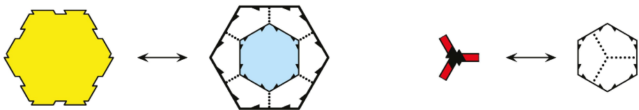
Figure 5. Rules for the mutual local derivation between (1 + \epsilon + \epsilon^2) -tilings and double hexagon tilings.
