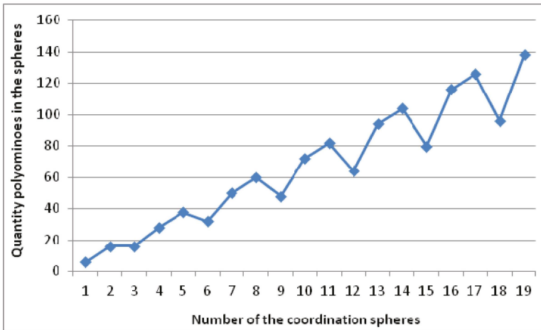
Figure 18. Coordination (magic) numbers of layer growth structure.
