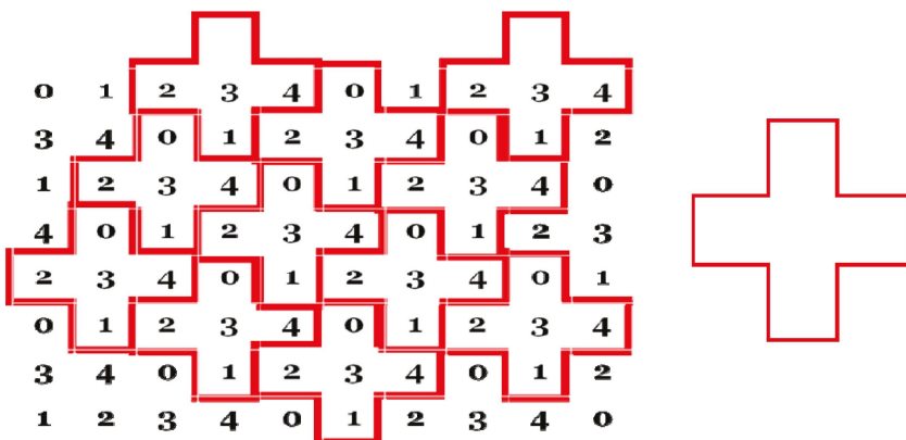
Figure 7. PS P51 2 . One of the cells, corresponding to the range of PS, is selected by vectors. The criterion of the space partition is tested by the polyomino shape—the “cross”. The center of the figure coincides with the “weight 3” of PS.
