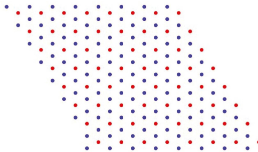
Figure 7. The figure shows the standard triangular lattice Q (the red points) and the larger lattice P (red and blue points) in which Q lies with index 3. The points of Q may be viewed as the vertices of a triangularization of the plane by equilateral triangles of side length 1. The blue points are the centres of these triangles. The color here has nothing to do with the coloring of the diagonals of the tiles—it only distinguishes the two cosets.
