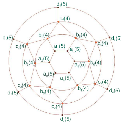
Figure 3. The graph of convex polytope S_6 .
