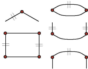
Figure 12. Five possible quotients of an edge quadrangle.
