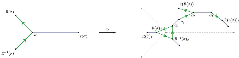
Figure 9. Chamfer Ch of an oriented map, local figure.
