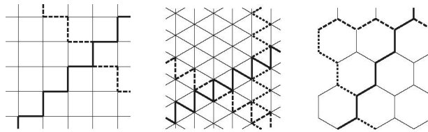
Figure 5. Petrie polygons of the planar polyhedra.
