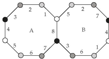
Figure 8. Faces and vertices in the map M'_{8,3} .
