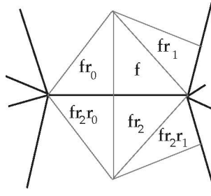
Figure 1. Flags in a map.
