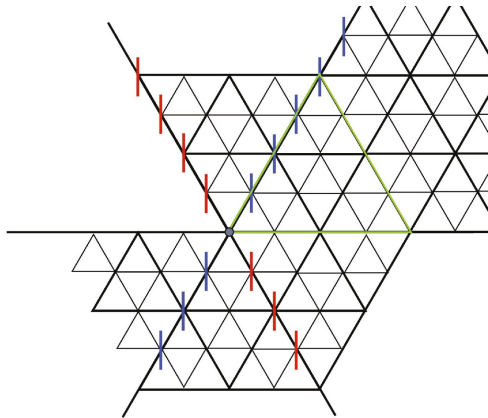
Figure 27. Vertical color lines start with a full blue diameter or full red diameter as shown. The green triangle indicates why the second blue line segment up from the origin is in fact blue. The vertical line is centered at the mid-point of an edge of a level 4 triangle and passes into one of the level 2 corner triangles of this level 4 triangle. The discussion on color shows that it must be blue. All the other blue line segments are explained in the same way. We cannot assign color at the origin itself since the origin is not the mid-point of any edge.
