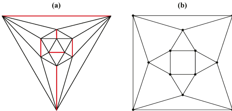
Figure 1. From (a) icosahedral graph to (b) cuboctahedral graph (removal of six red edges).
