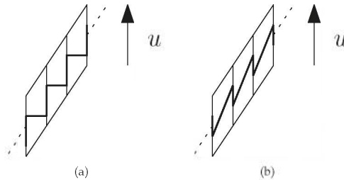
Figure 3. Unwrapped: An apeirobarrel winding up upstairs (a); and an apeirobarrel winding up downstairs (b). The staircases are highlighted.
