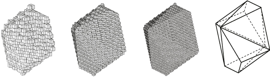
Figure 2. Formation of a grown polyhedron by tiling of the plane into polycubes. The number of layers n [15] is consistently indicated ( n = 5 ; n = 10 ; n = 15 ).
