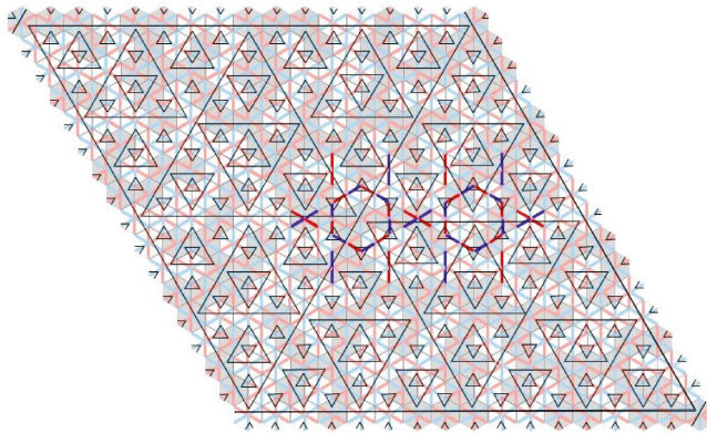
Figure 31. A figure showing that the pattern of the colored diameters of six surrounding tiles is same for every corner tile of a level 2 or higher triangle.
