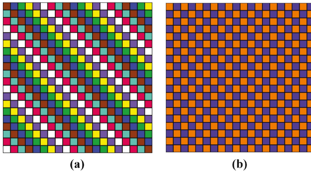
Figure 10. (a) PS 81_1 , operation (01234567); (b) PS 81_1 , operation (65470321).
