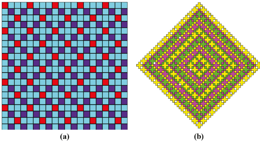
Figure 8. (a) An example of P42_2 space partition into the polyomino and (b) the form of layered structure growth.
