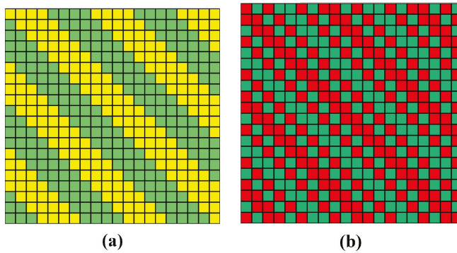
Figure 13. (a) PS 81_1 , operation (30127456); (b) PS 81_1 , operation (76541032).
