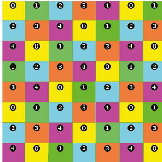
Figure 6. Definition of the packing space. PS P 51 3 .
