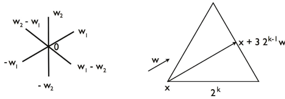
Figure 21. \Omega and a line through a vertex x in the direction w meeting the opposite edge at 3 \cdot 2^{k-1}w .
