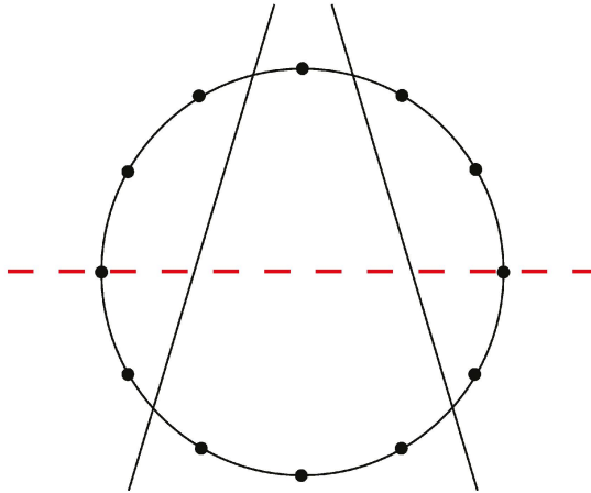
Figure 14. One of the two possible modes to section a circle with twelve evenly spaced vertices according to the criteria specified in the text.
