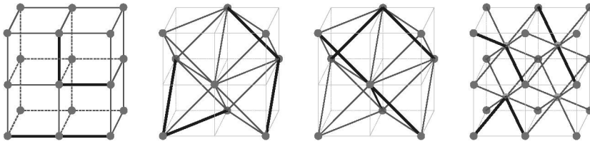
Figure 2. The angles formed by edges of the nets pcu, fcu and bcu.
