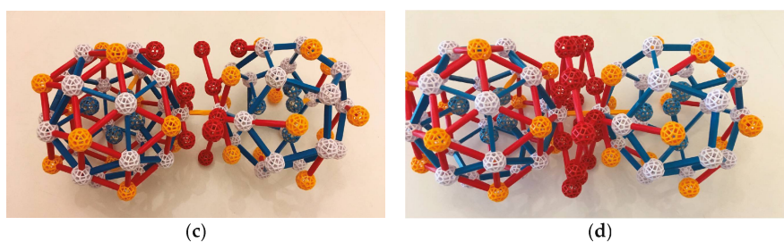
Figure 10. Development of a two-TDI cluster. (a) The initial bond between two TDIs. Only one of the five red bonds around each yellow Yb is shown for the right TDI; they are otherwise identical and have the same orientation; (b) Three red atoms from the icosidodecahedral shell have gelled into position on the right TDI at vertex V2; (c) Three red atoms have likewise gelled into position on V2, and a red bond and red ball have also been added to each of the three added in (b) to V2; (d) The entire OR complex has assembled around the yellow strut.
