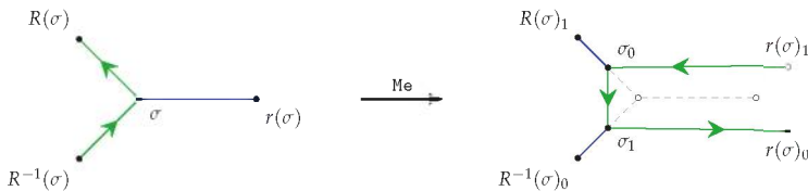
Figure 7. Medial Me of an oriented map, local figure.
