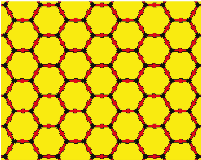
Figure 3. Patch of Penrose's (1 + \varepsilon + \varepsilon^2) -tiling.
