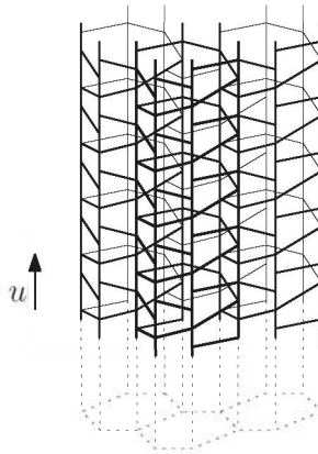
Figure 9. This patch with base (6^3) is not part of a barrel pseudotiling, as the face structure of the object does not correspond to an abstract 4-polytope.
