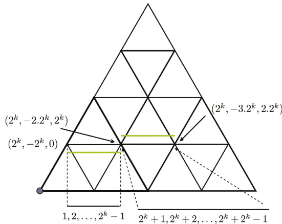
Figure 26. The horizontal line through the point (2^k, -2^k, 0) is seen as passing through midpoints of consecutive 2^{k+1} triangles. The corresponding edges along this line shift downwards and upwards alternately. The points (2^k, -2^k - m, m) with m = 1, 2, \dots, 2^k - 1 are on a shift-down edge. The next set for m = 2^k + 1, \dots, 2^k + 2^k - 1 are on a shift-up edge. The next set, m = 2.2^k + 1, \dots, 2.2^k + 2^k - 1 are on a shift-down edge, etc. The formula \lfloor \frac{x_3}{D(x_3 + x_2)} \rfloor = \lfloor m / (2^k) \rfloor accounts for this precisely, varying between 0 and 1 according to down and up.
