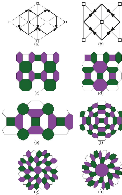
Figure 7. Decorated duals of the uniform base tilings (6^3) and (4.8^2) (a,b). The small boxes \square indicate \infty -colored vertices, and arrows indicate an increase in the function f^* . Patches of properly 3-colorable normal simple plane tilings, (c)–(e) periodic, (f)–(h) non-periodic.
