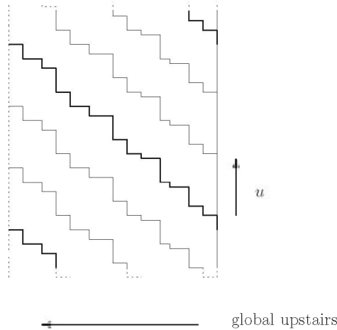
Figure 5. Staircase lines on unwrapped mantle of \infty -stack (schematic). Other edges have been omitted for clarity.
