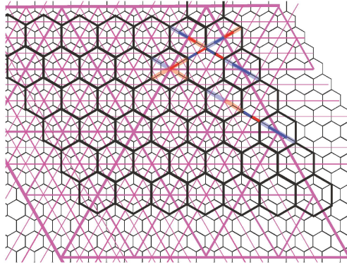
Figure 28. This shows how the scaled up hexagon inherits the colors of the smaller hexagons on which they are centered. The coloring is carried out by the same procedure that was used to color the original sized hexagons, though now the diameter sizes have doubled and only the lines of level at least 1 are used.
