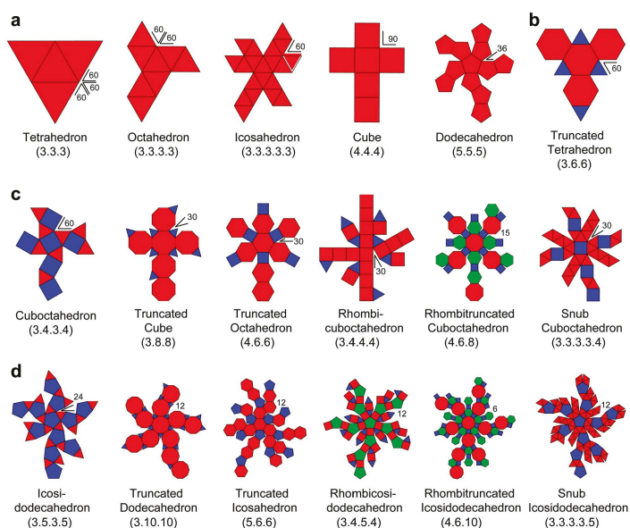
Figure 2. Platonic and Archimedean polyhedra and their angle deficits. Five Platonic polyhedra (a); one tetrahedral Archimedean polyhedron (b); six octahedral Archimedean polyhedra (c) and six icosahedral Archimedean polyhedra (d). Polyhedra with angle deficits of 60^\circ , 120^\circ and 180^\circ are compatible with decoration by a 6.6.6 tiling, the one with 90^\circ by a 4.4.4.4 tiling. However, a 6.6.6 tiling of the square faces in the cuboctahedron—with an angle deficit of 60^\circ —cannot knit across the boundaries of the squares.
