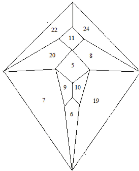
Figure 26. A zgyo-dodecahedral brain map of type II cadherins that conforms to the Shimoyama binding data and that reflects substantial agreement with the Hulpiau/van Roy cadherin map in Figure 25. CDH22 and CDH24 are assigned to the cerebellar lobes; CDH8 and CDH20 are assigned to the temporal lobes; CDH7 and CDH19 are assigned to the frontal lobes; CDH9 and CDH10 are assigned to the olfactory bulbs; CDH11 is assigned to the medulla/pons; CDH5 is assigned to the diencephalon; CDH6 is assigned to the corpus callosum (the back face has been assigned to cadherin-12 and corresponds to the cerebral cortex).
