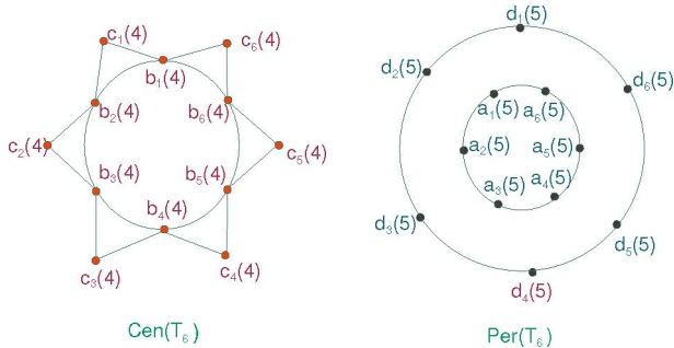
Figure 6. Centrality for T_6 .
