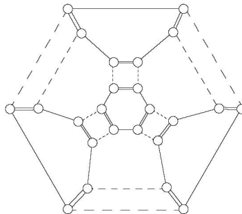
Figure 4. The tetrahedron as a 2-maniplex.
