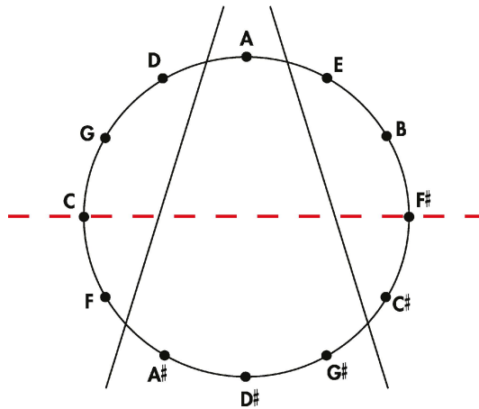
Figure 16. An installation of the tones of the Circle of Fifths onto the sectioned circle in Figure 14.
