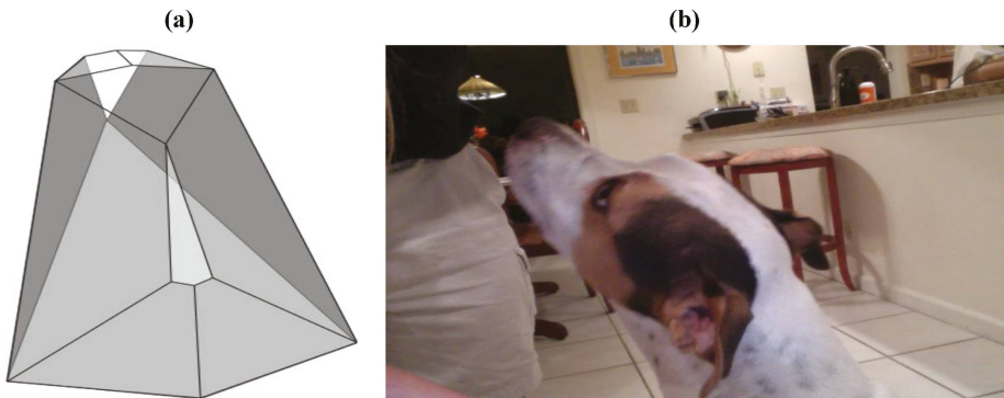
Figure 22. Similarity between the overall morphology of (a) the Figure 7 zygo-dodecahedron and (b) the head of a dolichocephalic dog.
