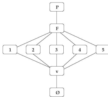
Figure 7. The poset of the map.
