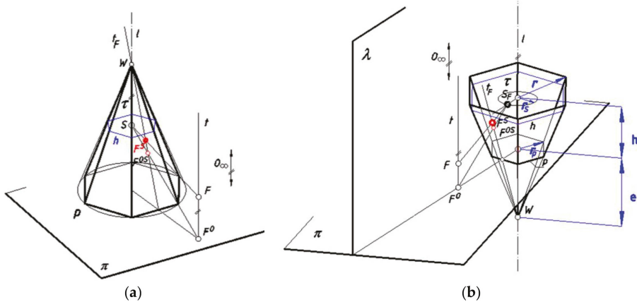
Figure 3. Representation of a point F on a pyramid surface: (a) of version A from a stationary center S ; and (b) of version B from a moving center S_\chi .
