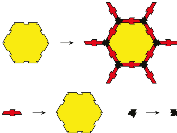
Figure 2. Inflation rule for Penrose's (1 + \varepsilon + \varepsilon^2) -tiling.
