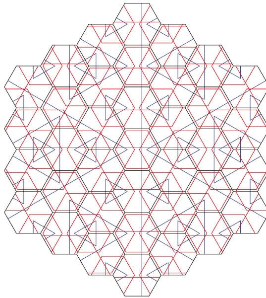
Figure 13. Patch of the (1 + \epsilon + \epsilon^2) -tiling in the variant with line decorations. In addition to the hierarchy of blue triangles from the half-hex tiling, there is now also a hierarchy of red hexagons. Hexagons of each size form a lattice periodic array, with lattices of different densities.
