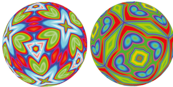
Figure 4. Two spherical patterns with [3,4] symmetries.
