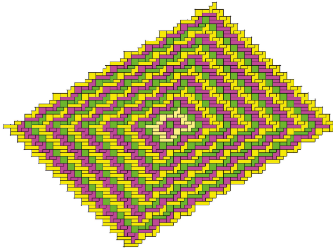
Figure 17. The shape of the growth of the partition PS P82_2 by element of g(8) of the permutation group of the Pauli matrices.
