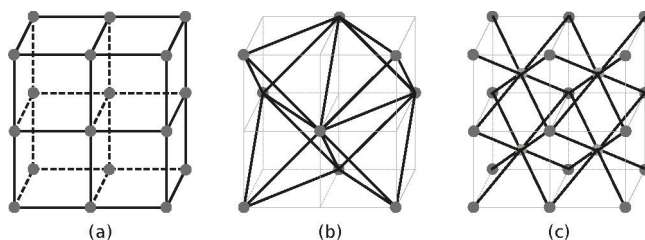
Figure 1. Nets pcu (a); fcu (b); and bcu (c).
