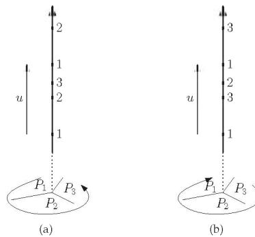
Figure 4. Determining upstairs orientations: (a) Counterclockwise; (b) clockwise.
