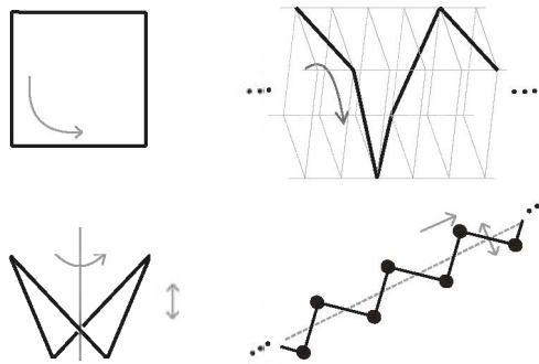
Figure 3. Abstract rotations of polygons.
