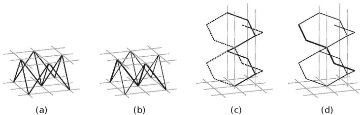
Figure 6. Blended polyhedra \{4, 4\}\#\{\} (a); \{\infty, 4\}_4\#\{\} (b); \{4, 4\}\#\{\infty\} (c) and \{\infty, 4\}_4\#\{\infty\} (d).
