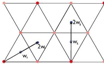
Figure 10. The figure shows how the centroids (indicated with solid blue dots) of the new side-length-2 triangles (indicated with solid red dots) are obtained as vectors from q_1 + 2P . The two 2Q -cosets of q_1 + 2P which are not q_1 + 2Q itself indicate the centroids of the new up and down triangles. Notice that the orientations of the new triangles, and hence the orientations associated with the new centroids, are opposite to the orientations associated with these points when they were viewed as centroids of the original triangulation. This explains why S_2^\downarrow \subset S_1^\uparrow and S_2^\uparrow \subset S_1^\downarrow .
