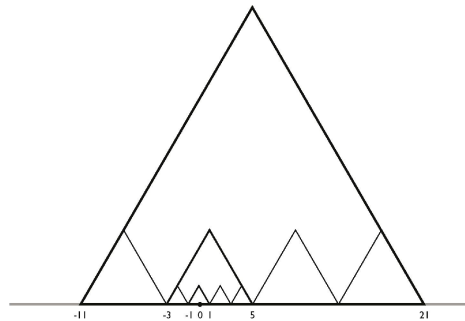
Figure 12. This shows a sketch of how a tiling with an infinite a -line (the horizontal line) can be constructed so that it is generic- w . Here \mathbf{q} = za_1 , where z is the 2-adic integer (1, 1, 5, 5, 21, 21, 85, 85, \dots) (the mod 2, 4, 8, 16, 32, 64, 128, 256, \dots values). Some triangles of edge lengths 2, 8, 32 are shown. There are triangles of arbitrary large side lengths on the horizontal line, but the triangulation does not admit a second infinite a -line and cannot admit an infinite w -line since \mathbf{q} is of the wrong form.
