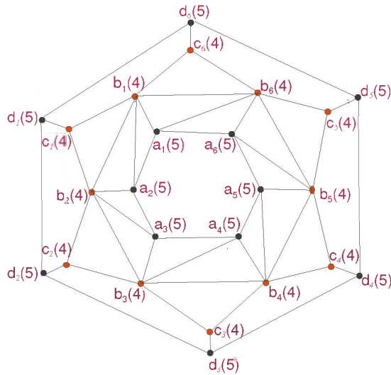
Figure 5. The graph of convex polytope T_6 .
