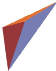
Figure 5. An irregular tetrahedron with scalene triangular faces.
