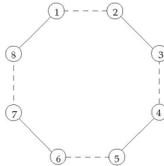
Figure 3. A 1-maniplex.
