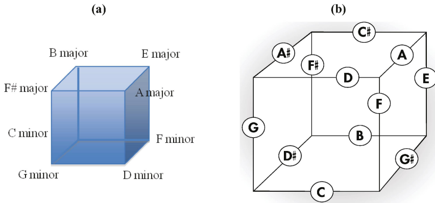
Figure 12. (a) The four major triads and four minor triads encoded at those eight of the fourteen vertices of the rhombic dodecahedron in Figure 10a that define a cube; (b) A version of the intonated rhombic dodecahedron in Figure 10a that features intonated cube edges.
