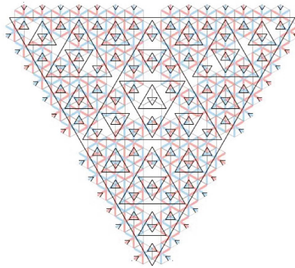
Figure 6. The iCw-L tilings. The triangulation is generic-a but not generic-w. Of course the partial tiling shown is perfectly consistent with generic tilings—in fact all Taylor–Socolar tilings contain this type of patch of tiles. However, if the pattern established in the picture is maintained at all scales, then indeed the result is a not a generic tiling since it fails generic-w.
