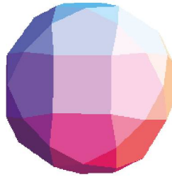
Figure 16. Chiral polyhedron consisting of equilateral triangles, squares and irregular pentagons.
