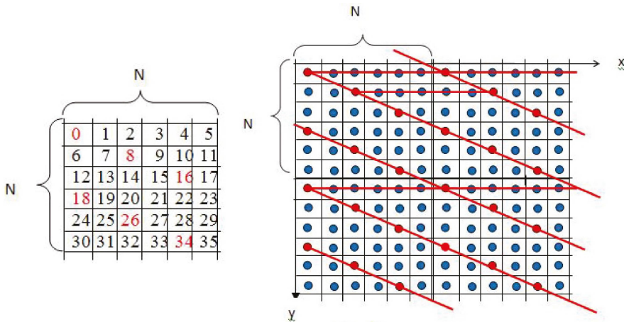
Figure 4. A series of parallel nodal lines.
