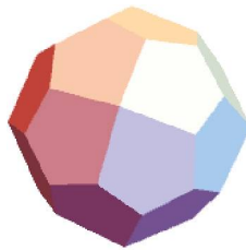
Figure 14. Dual of the snub cube (pentagonal icositrahedron) with its pentagonal face. If we substitute x = 1, y = 0 in (46) we obtain the Catalan solid tetrakis hexahedron (dual of the truncated octahedron).
