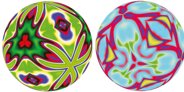
Figure 3. Two spherical patterns with [3,3] symmetries.
