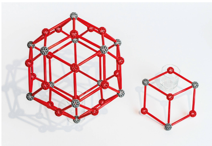
Figure 6. (Left): A rhombic triacontahedron viewed along a three-fold rotation axis; (Right): The six vertices ringing a vertex on the three-fold axis, together with that vertex, are seven of the eight vertices of an obtuse golden rhombohedron (OR).
