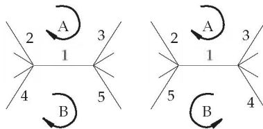
Figure 9. An edge in a map and its opposite.
