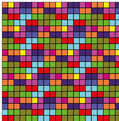
Figure 19. Tiling PS P841 by permutation operation g (13) (Table 12) of the Dirac matrices group.
