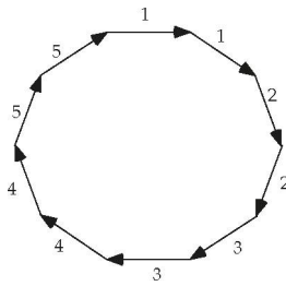
Figure 6. A map with one face.
