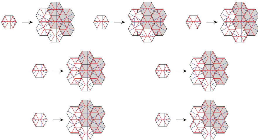
Figure 14. Inflation rules for (1 + \epsilon + \epsilon^2) -tiling in the variant with line decorations. If a hexagon is replaced by 7 hexagons, a pseudo inflation is obtained. Taking only the 4 shaded hexagons results in a standard inflation rule (for one sector).
