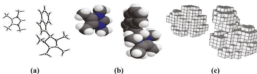
Figure 1. (a) The rod model of molecules; (b) geometrical (spherical) model; and (c) discrete model (policube).
