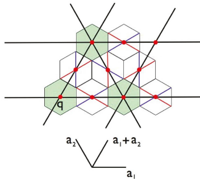
Figure 15. The figure shows some hexagonal tiles, each centered on a point of Q . The point q is assumed to be in the coset q_1 + 2Q and the gray hexagons are those in the picture whose centers are in this coset. The white hexagons are centered at points from all three of the remaining cosets of Q relative to 2Q . These are the midpoints of the edges of the level 1 triangles. Notice in each, the red and blue diagonals clockwise and counterclockwise of the direction of the black stripes. At the bottom we see the three vectors a_1, a_2, a_1 + a_2 . The centers of the white hexagons are, reading left to right and bottom to top, q_1 + a_1, q_1 + 3a_1; q_1 + a_1 + a_2, q_1 + 2a_1 + a_2, q_1 + 3a_1 + a_2; q_1 + 3a_1 + 2a_2 . The picture manifests the rule R2 and shows that elements of the same coset carry the same orientation of diameters. Note that from the rotational symmetry of the process and the fact that the hexagons centered on q_1 + a_1 and q_1 + 3a_1 have identically aligned diagonals, we can infer that this property is retained across each of the cosets q_1 + a_1 + 2Q, q_1 + a_2 + 2Q, q_1 + a_1 + a_2 + 2Q .
