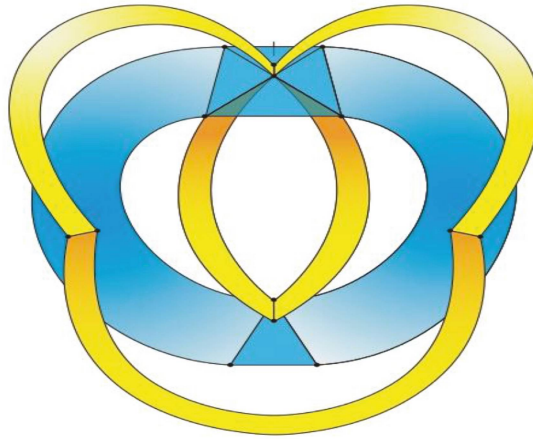
Figure 23. A non-convex version of the dodecahedron in Figure 7 is discernibly cephaloid such that the bottom yellow medial face corresponds to the mandible, the upper two yellow faces are assigned to the auricles, the two central yellow faces are attributed to the nasal bones, the lower blue medial triangle is ascribed to the maxilla, the two large central blue faces are assigned to the temporal bones, the top blue medial triangle corresponds to the occipital bone (the hash mark at the top of this face indicates the mid-line), the other blue medial triangle is ascribed to the frontal bone, and the remaining two blue triangles are ascribed to the parietal bones.
