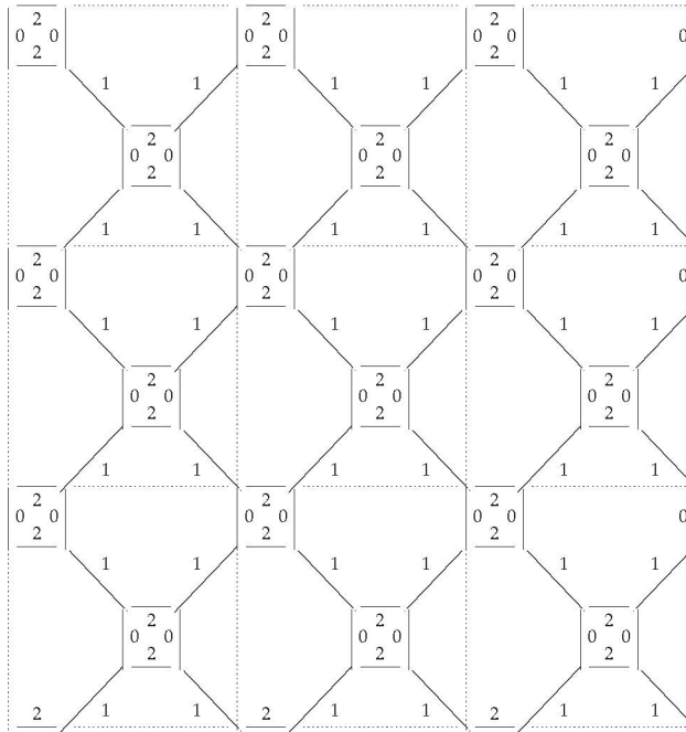
Figure 1. Local picture of the Cayley graph G .
