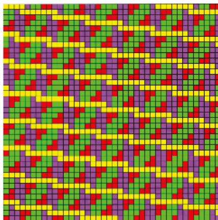
Figure 23. A discrete model of the structure layer [27] in PS P31_6 .
