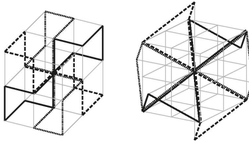
Figure 8. The polyhedra P(1,0) and Q(1,1) .
