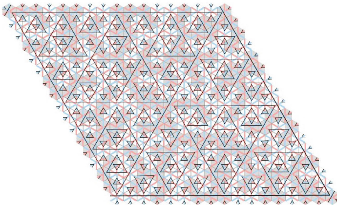
Figure 2. The figure shows a pattern of triangles emerging from the construction indicated in Section 2, manifesting the rule R1 . The underlying hexagonal tiling is indicated in light and dark shades, which indicate the parity of the hexagons. The underlying diagonal shading on the hexagons manifests the rules R2 .
