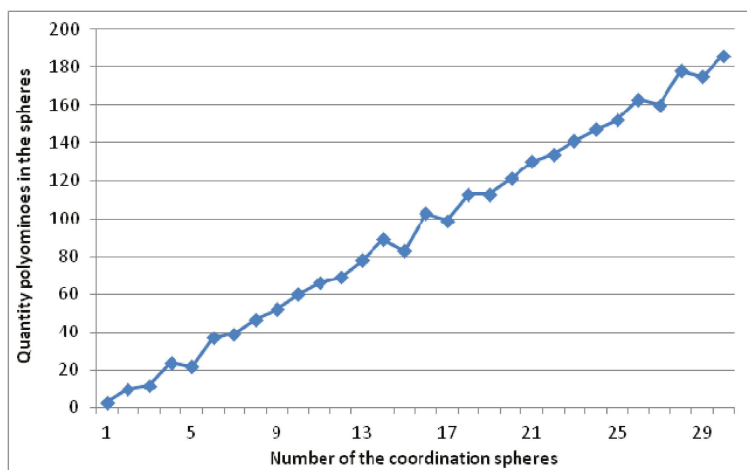
Figure 21. Coordination (magic) numbers of growth structure (Figure 19).
