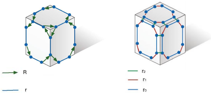
Figure 2. The cube may be considered as an oriented map determined by R and r , or as a map determined by r_0, r_1, r_2 .
