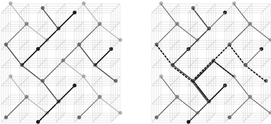
Figure 10. The polyhedron P_2(1,1) .
