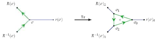
Figure 6. Truncated oriented map Tr, local figure.
