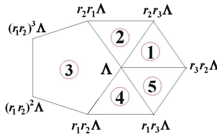
Figure 17. The vertices connected to the vertex \Lambda .
