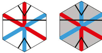
Figure 3. The two basic hexagonal tiles. One is a white tile and the other a light gray. These are colored with red and blue diameters. The rotational position of the tiles is immaterial. Note how the tiles are identical as far as the red diagonal and blue diagonal are concerned. The distinction is in which color of the red-blue diagonal cuts the black stripe.
