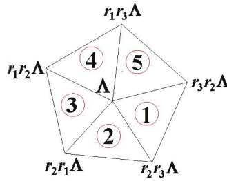
Figure 6. The vertices connected to the general vertex \Lambda (note that all vertices are not in the same plane).
