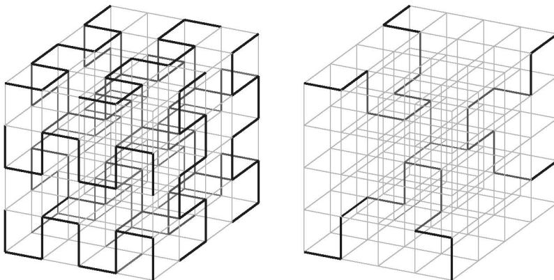
Figure 9. The polyhedron P_1(1,0) .
