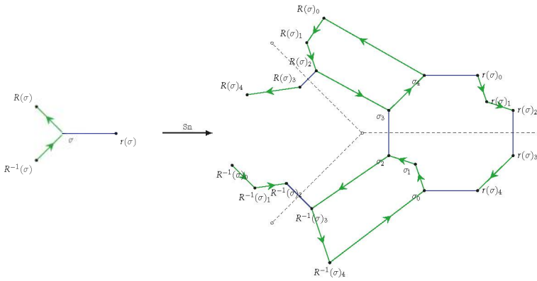
Figure 8. Snub S_n of an oriented map, local figure.
