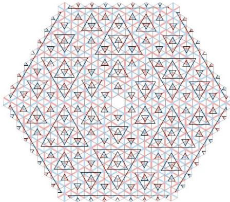
Figure 5. The (central part of a) central hexagon ( CHT ) tiling. Full (edge-shifted) triangles of levels 0, 1, 2 are shown. At the outside edges one can see the beginnings of triangles of level 3. The rays from the central hexagon in the six a -directions will have infinite a -lines in them. However the edge shifting rules cannot be applied to them because they are of infinite level—they are not composed of edges of finite triangles. In the end a full tiling is obtained by placing a fully decorated tile into the empty central hexagon. There are 12 ways to do this, and each way then determines the rest of the tiling completely. These tilings violate both forms of generic condition.
