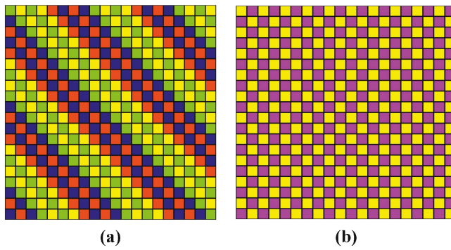
Figure 12. (a) PS 81_1 , operation (23016745); (b) PS 81_1 , operation (47652103).
