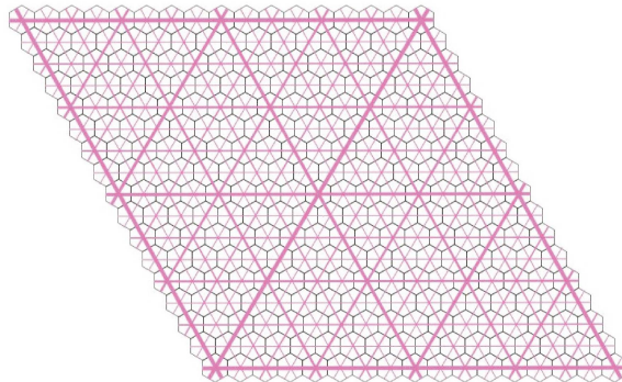
Figure 11. A partial triangulation of the plane overlaid on the basic lattice of hexagons which will make up the tiles. The levels of the triangles are indicated by increasing thickness. One can clearly see triangles of levels 0, 1, 2, 3, 4 and one can also see how triangle edges of level k ultimately become edges passing through the interior of triangles of level k + 1 . This will be used to make the shifting of edges later on.
