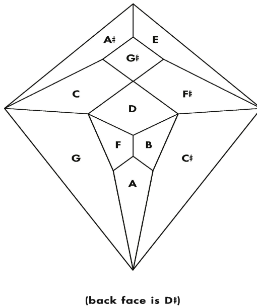
Figure 13. Schlegel diagram corresponding to the Figure 8a zygo-dodecahedron.
