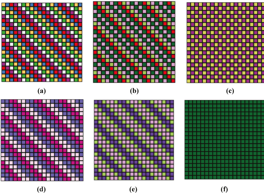
Figure 9. Colored PS P61 1 , obtained by partition of space by a subgroup of permutations of the 12th permutation order. (a) g(0); (b) g(1) = g(2) = g(5); (c) g(3) = g(4); (d) g(6); (e) g(7) = g(8) = g(11); (f) g(9) = g(10).
