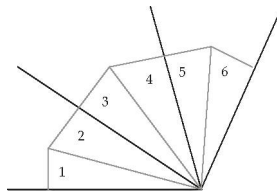
Figure 10. Facets and subfacets.
