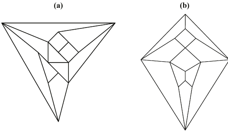
Figure 5. (a) The graph obtained from the tetrakis hexahedral graph after removal of the twelve red edges in Figure 4, can be redrawn as (b), the isomorphic graph.
