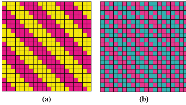
Figure 11. (a) PS 81_1 , operation (12305674); (b) PS 81_1 , operation (54763210).
