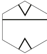
Figure 13. The basic hexagon with its markings arising from shrunk triangles.
