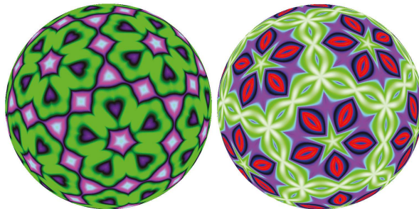
Figure 5. Two spherical patterns with [3,5] symmetries.
