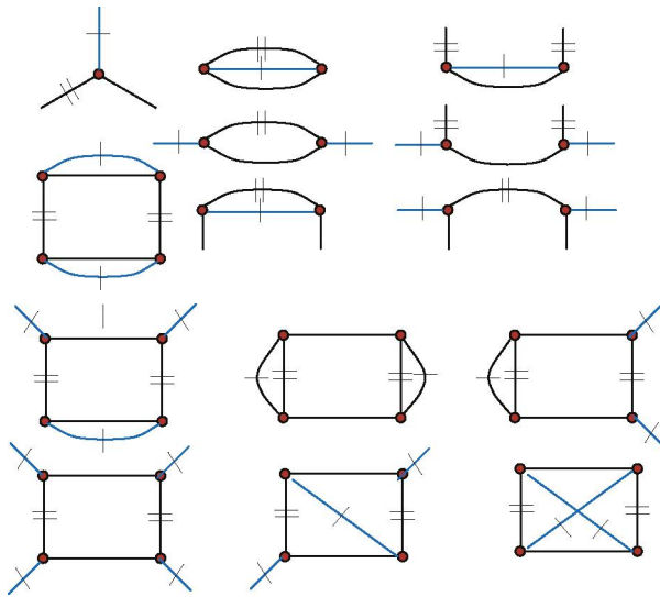
Figure 11. The 14 symmetry type graphs of edge-transitive maps.
