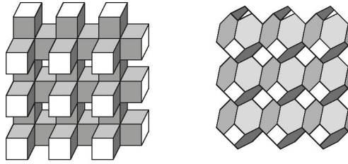
Figure 7. The polyhedra \{4,3|4\} and \{6,4|4\} . Squares and hexagons in the same shade of gray represent polygons in parallel planes
