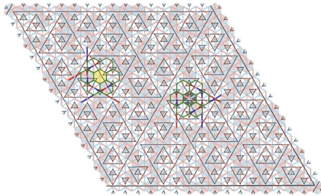
Figure 30. Examples are shown that demonstrate how we can see that around each hexagon centered on a level 1 vertex of q_1 + 2Q there are at least two different pairs of tiles with mismatched colors amongst its six surrounding tiles. The two cases correspond to a level 1 vertex at the mid-point of a level 2 triangle and a level 1 vertex a non-midpoint of a higher level triangle. As explained in the text, one pair is found in a uniform way in both cases. The other pair is found by one method in the first case and another method in the other.
