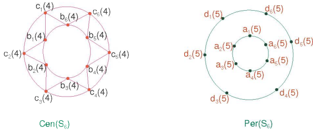
Figure 4. Centrality for S_6 .
