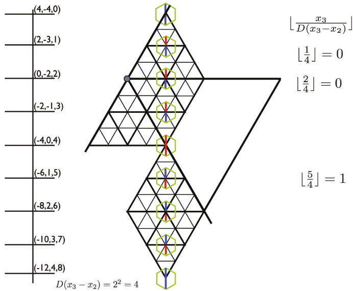
Figure 19. In the figure the small circle indicates (0, 0) . A vertical color line is shown, which meets the a_3 axis in the point p = (4, -4, 0) . The points on this axis are all of the form (u, -u, 0) , u \in \mathbb{Z} . In the CHT tiling set-up, D(u) indicates that the point is a vertex of a level \log_2 D(u) triangle, in this case D(4) = 4 , so we are on a level 2 triangle ( 2^2 = 4 ). We already saw that the color starts with a full blue diagonal at (4, -4, 0) . Moving down the line to the next point decreases x_1 by 2 and increases x_2, x_3 by 1. We note that x_3 - x_2 remains constant, and D(x_3 - x_2) = 4 . At the second step we cross, at right-angles into another triangle of level 2, and the color proceeds without interruption. At the 4th step we are at a vertex that is the midpoint of the side of a triangle of level 3 and looking up our vertical line we can see that it is passing into a corner triangle of level 4—namely where we just came from, and we see a forced full red diagonal. In the first three steps the diameters are all red-blue (top to bottom), whereas after the red-red diagonal the next three steps are blue-red diameters, so there is a switch that affects parity. We can ignore the points with full diameters (they get sorted out in a different w-direction). We note that \lfloor \frac{x_3}{D(x_3-x_2)} \rfloor maintains the value 0 on steps 1, 2, 3 and maintains the value 1 on steps 5, 6, 7, showing that the formula notices the change of diameters correctly. If we continue \lfloor \frac{x_3}{D(x_3-x_2)} \rfloor = 2 on the next three step sequence, but modulo 2 this is the same as 0.
