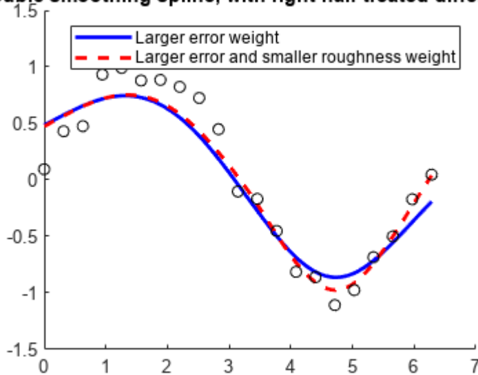
Cubic smoothing spline, with right half treated differently
