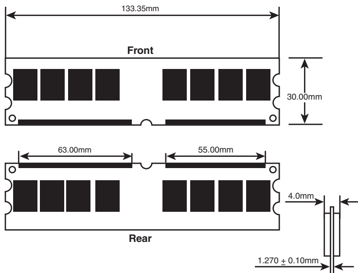
Figure 6.7 A typical 240-pin DDR2 DIMM.
