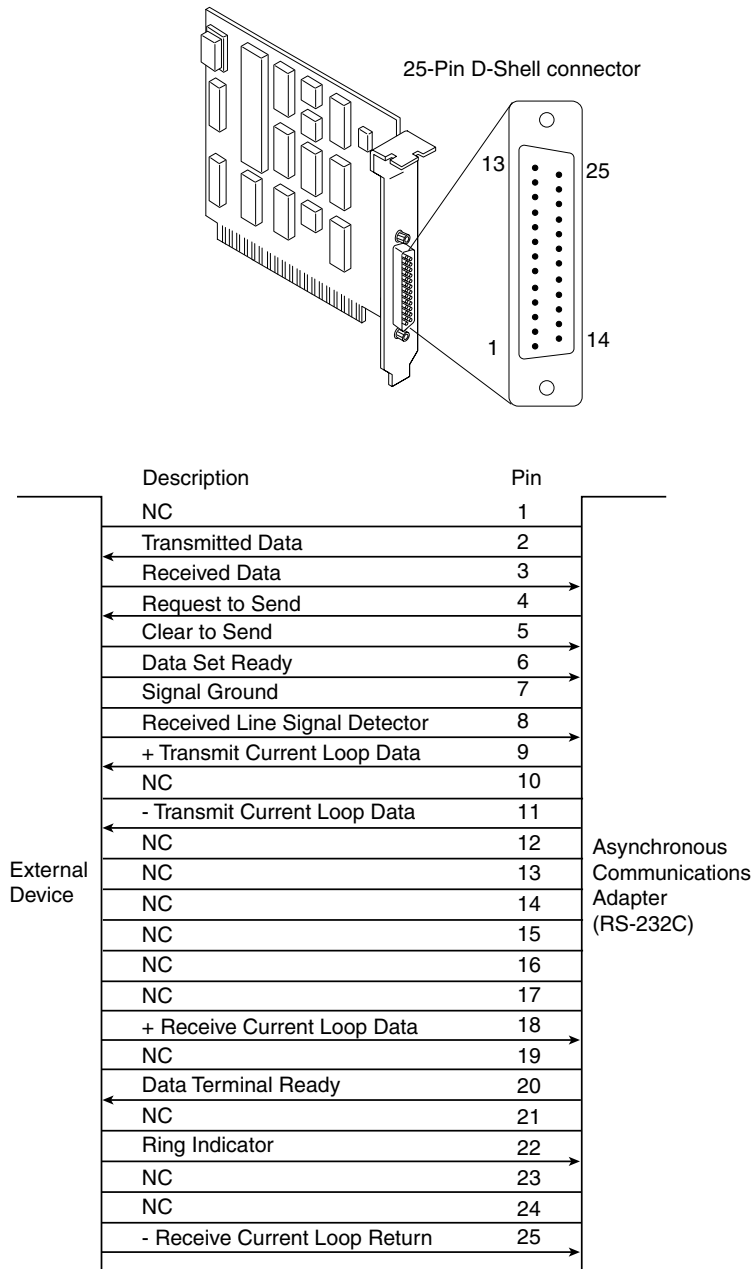
Figure 14.24 Standard 25-pin serial port connector specifications.
