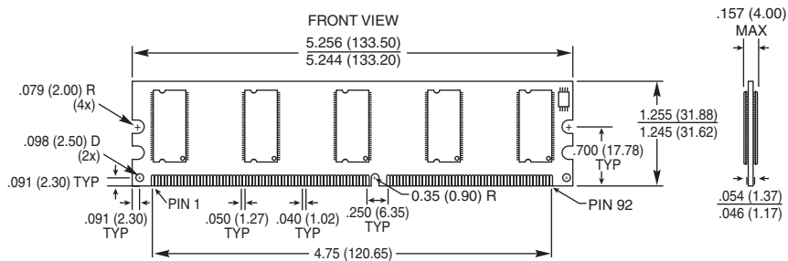
Figure 6.6 A typical 184-pin DDR DIMM.
