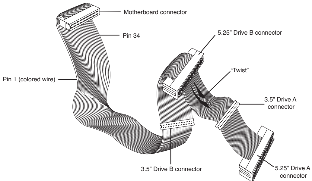
Figure 10.7 Universal five-connector floppy interface cable.
