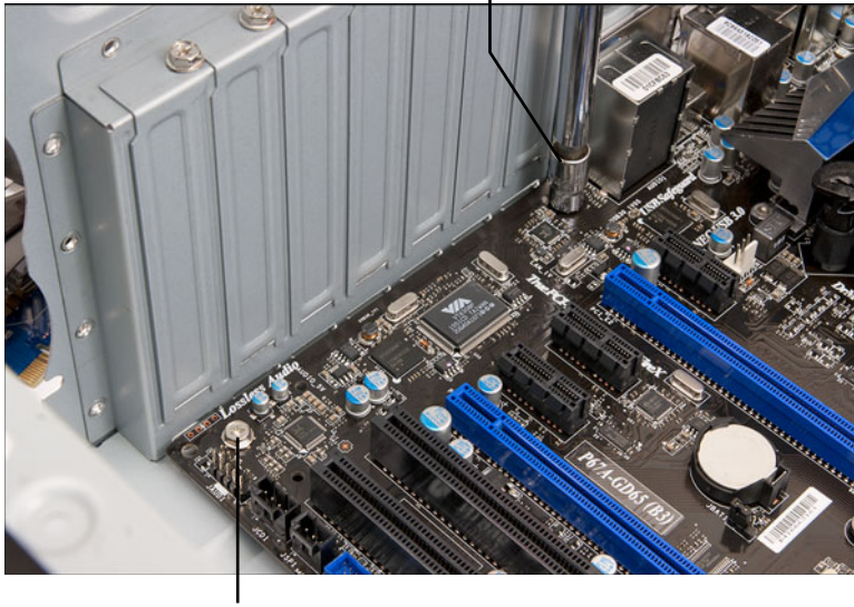
Figure 19.20 Installing the screws that hold the motherboard to the chassis.
