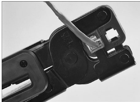
Figure 17.13 Firmly squeeze the crimping tool to attach the connector to the cable.
