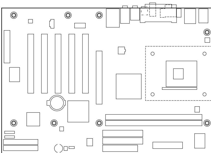
Figure 19.16 Mounting screw holes in a typical ATX motherboard. The highlighted circles mark the screw holes for mounting the motherboard to the case.
