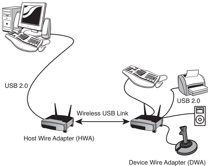
Figure 14.14 Using a HWA and DWA to wirelessly connect traditional wired USB devices to a system.
