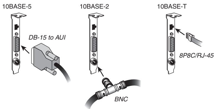
Figure 17.5 An Ethernet network card with Thick Ethernet (DB-15), Thin Ethernet (RG-58 with T-connector), and UTP (8P8C/RJ-45) connectors.
