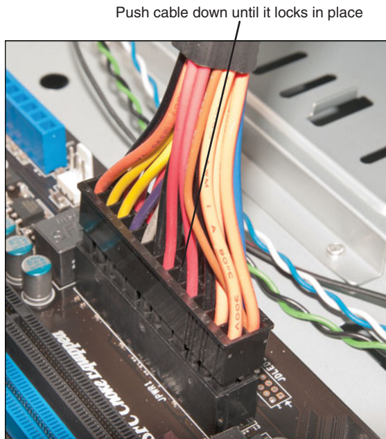
Figure 19.24 Attaching a 24-pin ATX motherboard power connector.
