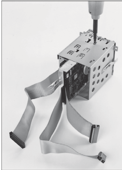
Figure 19.28 A hard disk drive mounted in a removable drive cage.
