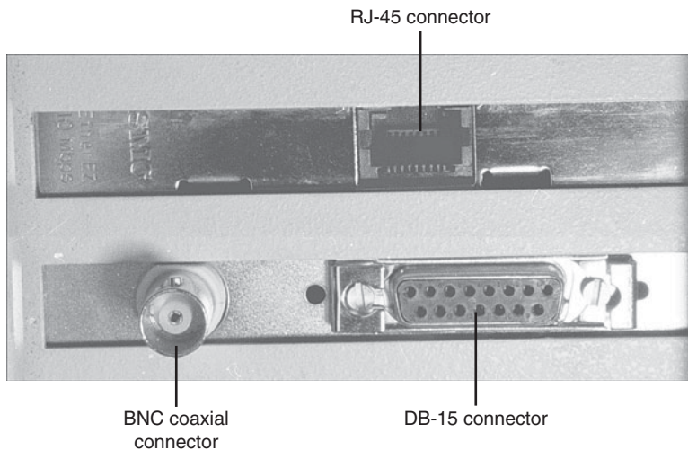
Figure 17.4 Three Ethernet connectors on two NICs: Modern 8P8C (RJ-45) connector (top center), Obsolete DB-15 connector (bottom right), and Obsolete BNC connector (bottom left).
