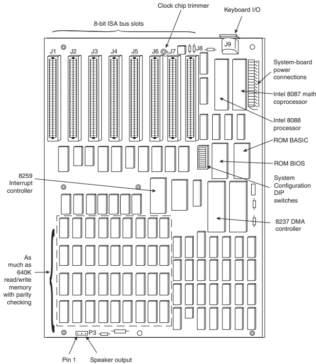
Figure 4.2 IBM PC-XT motherboard (circa 1983).
