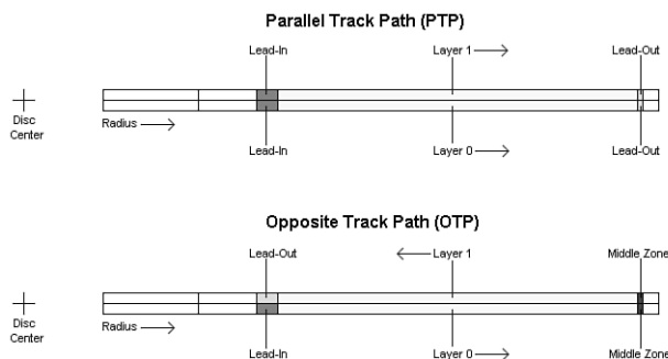
Figure 11.12 PTP versus OTP.
