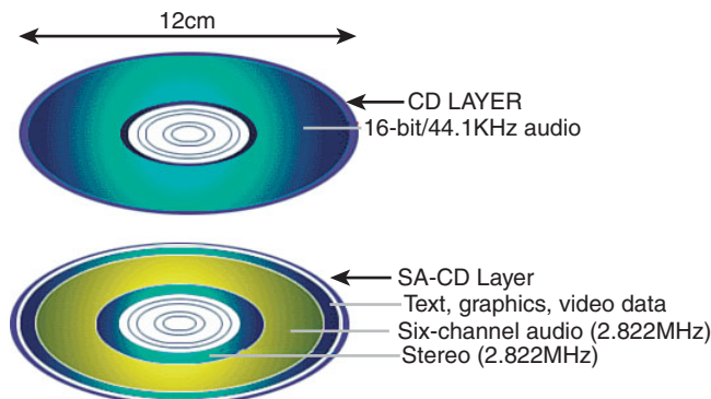
Figure 11.16 The structure of a hybrid SA-CD disc.
