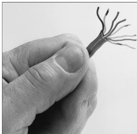
Figure 17.11 Arrange the wire pairs for insertion into the 8P8C (RJ-45) connector according to your chosen scheme (EIA 568B, for instance).
