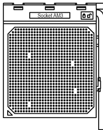
Figure 3.17 Socket AM3. The arrow (triangle) at the lower left indicates pin 1.
