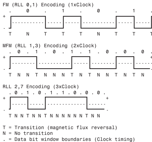
Figure 8.10 ASCII character X write waveforms using FM, MFM, and RLL 2,7 encoding.
