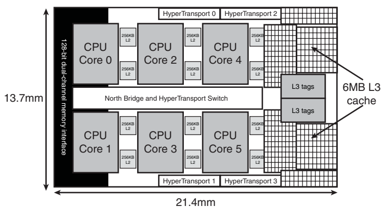
Phenom IIx6 core diagram
