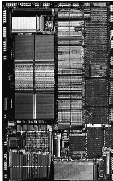
Figure 3.20 486 processor die. Photograph used by permission of Intel Corporation
