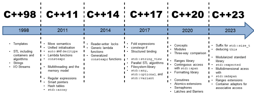
C++ timeline
