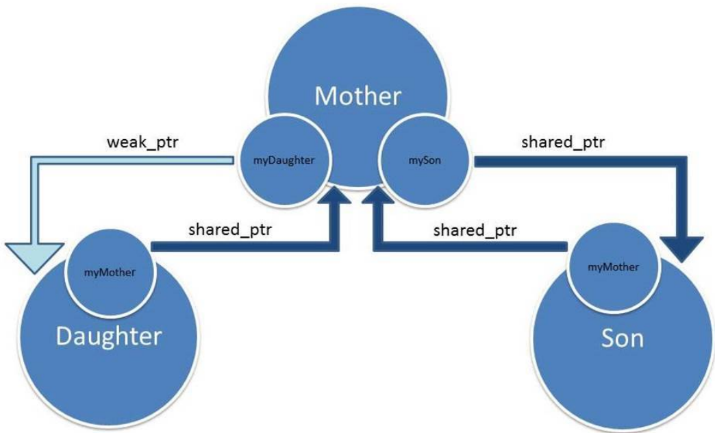
Cyclic references
