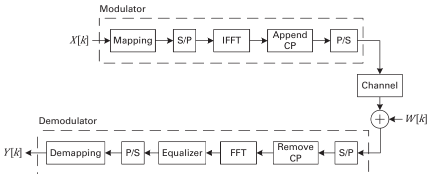
Figure 7.4 Discrete representation of an OFDM system.
