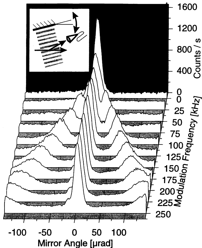
Figure 5: Diffracted atoms as a function of their incidence angle at the amplitude modulated standing light wave (see inset), at different modulation frequencies. The detection slit is located such that only diffracted atoms are registered. The top graph of the series shows the result for an unmodulated light crystal and only one peak at the static Bragg angle is observed. The next curves show the same experiment, but with intensity modulation frequencies in the range from 25\text{kHz} to 250\text{kHz} in steps of 25\text{kHz} . In contrast to the static case two pronounced side peaks appear in each curve. They are located symmetrically around the central Bragg angle. Their angular separation from the central peak increases linearly with the modulation frequency. The deBroglie wave frequency of the atoms in the new Bragg peaks is shifted by \pm the modulation frequency.
