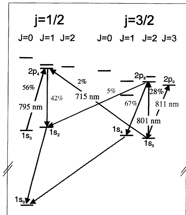
Figure 1: Figure showing the level scheme of metastable Ar, including the branching ratios of the various open decay channels. In our experiments we used the 1s_5 metastable state and there the closed transition ( 1s_5 \rightarrow 2p_9 ) at 811 nm ( J = 2 \rightarrow J = 3 ) and the open transition ( 1s_5 \rightarrow 2p_8 ) at 801 nm ( J = 2 \rightarrow J = 2 ).
