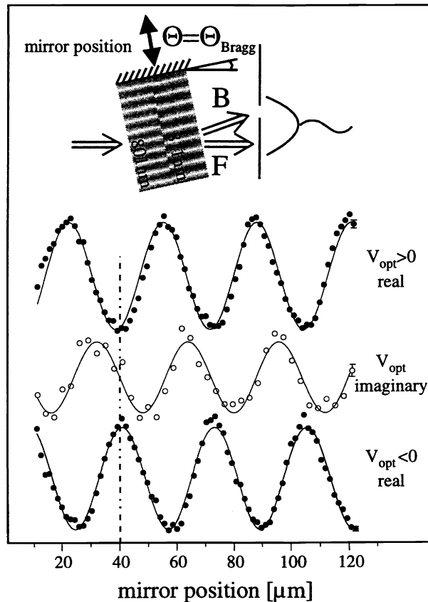
Figure 4: Measurement of the standing atomic wave fields in the light crystal. The anomalously transmitted wave field (middle trace) has its maxima at the nodes of the standing light field. If the 801 nm standing wave is detuned far off resonance, the standing atomic wave is shifted by \pi/2 to the left for blue detuning (positive potential) and to the right for red detuning (negative potential).
