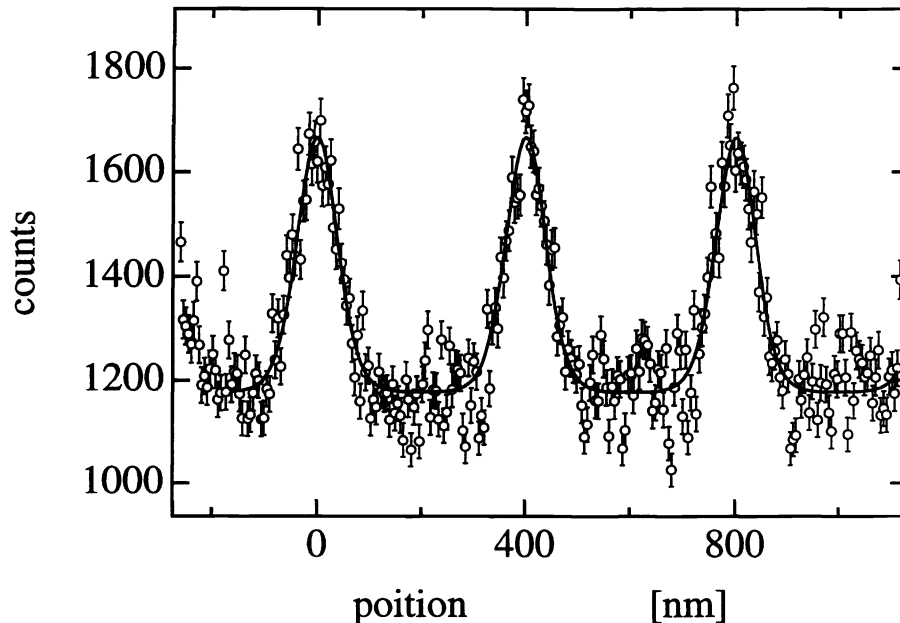
Figure 2: Total transmission through two on resonant light gratings as a function of their relative transversal position. The line is a fit with an exponential attenuation law as given in the text.
