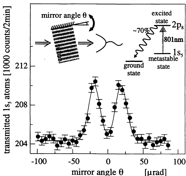
Figure 3: Total intensity of the metastable Ar^* beam after transmission through a standing light wave tuned exactly on resonance to an open transition (see insert) as a function of incidence angle. The transmission increases anomalously for Bragg incidence from either side relative to the planes of the standing light field. The solid line is a fit curve with two Gaussian curves.
