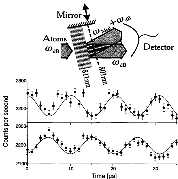
Figure 6: A thin stationary absorptive grating ( 801\text{nm} focused standing light wave) probes the travelling atomic interference pattern behind the modulated ( 100\text{kHz} ) 811\text{nm} light crystal. The total atomic transmission is detected as a function of time showing the interference between matter waves of different frequencies. A relative phase shift of \pi between the two light waves is introduced by shifting the common retro-reflection mirror by 16.4\ \mu\text{m} . This results in a corresponding \pi -phase shift of the atomic transmission oscillations between upper and lower data graphs.
