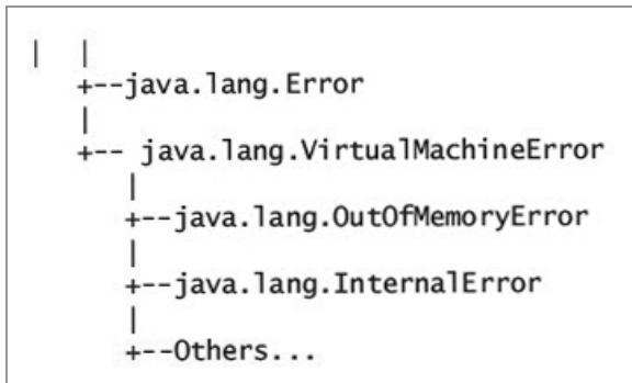
Figure 12-1 The Exception and Error class inheritance hierarchy
