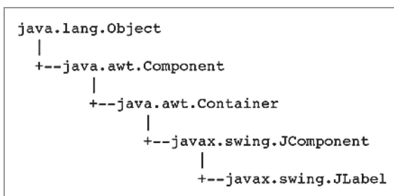
Figure 14-7 The JLabel class inheritance hierarchy
