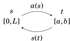
Figure 1.9.1 t = \alpha(s)
