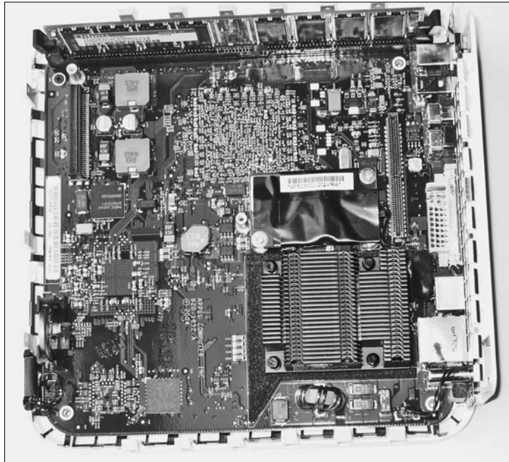
Figure 6-2: Plug the mezzanine board into the connector at the upper left.
