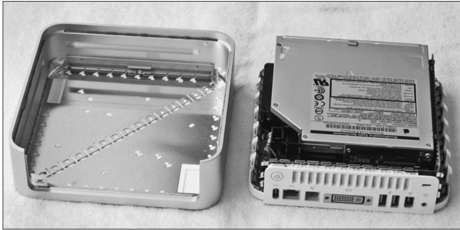
Figure 4-6: Lift the Mac mini body out of the outer casing and set it on its bottom.
