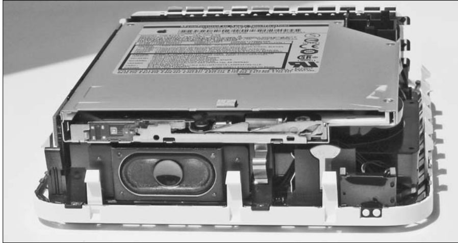
Figure 4-3: Three plastic tabs hold the front of the Mac mini together.
