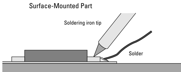
Figure 16-4: You can hold down a small surface- mounted part with the iron.
