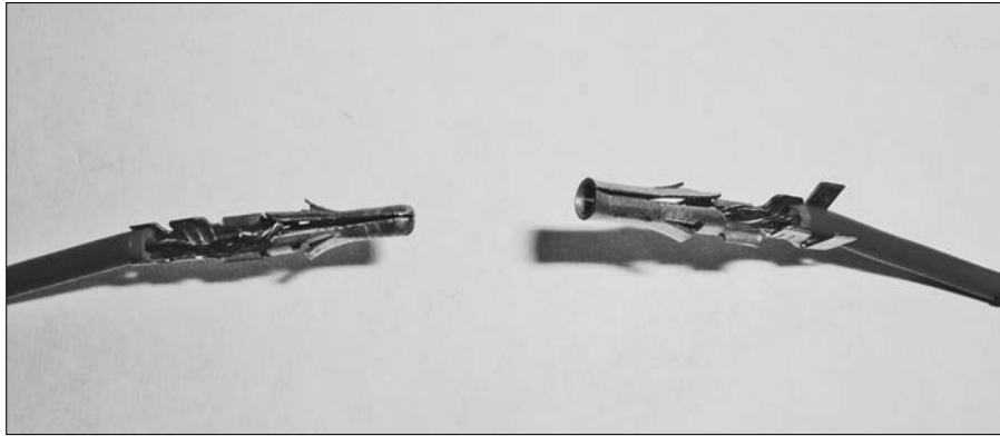
Figure 13-11: Male and female pins ready for crimping.
