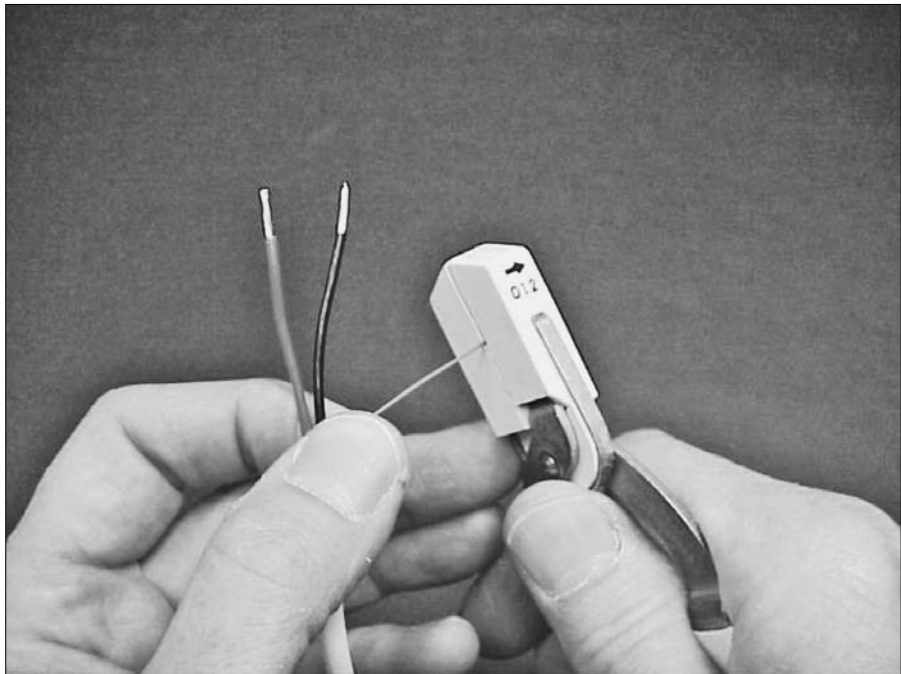
Figure 13-9: Stripping the wires.
