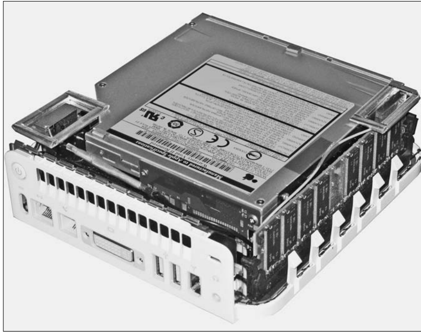
Figure 6-5: The installed antennas look like this.
