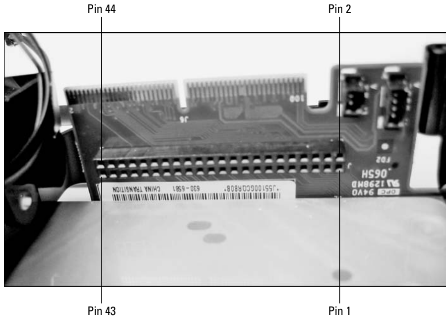
Figure 19-6: Pinouts for the 44-pin connector in the Mac mini.
