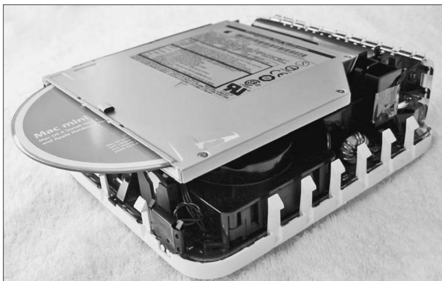
Figure 8-4: The optical drive sits on top.
