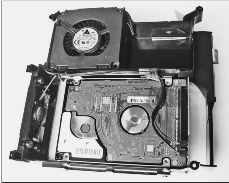
Figure 7-6: You can see the hard drive and fan with the internal frame flipped over.
