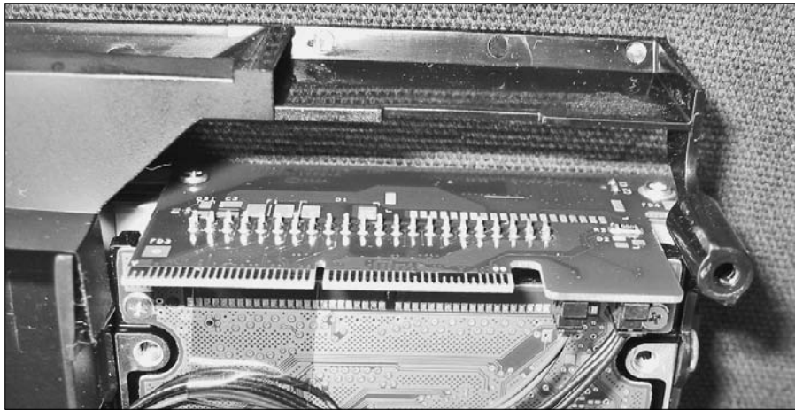
Figure 5-2: The interconnect board connects the DVD and hard drives to the motherboard.
