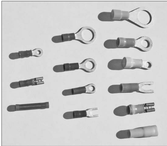
Figure 12-2: Assorted crimp-on wire terminals.
