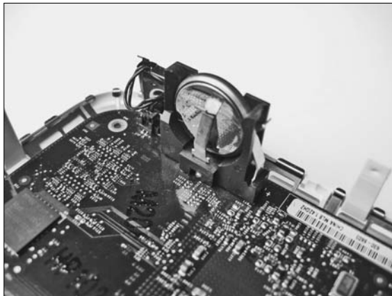
Figure 20-2: The LED cable is to the left of the battery.
