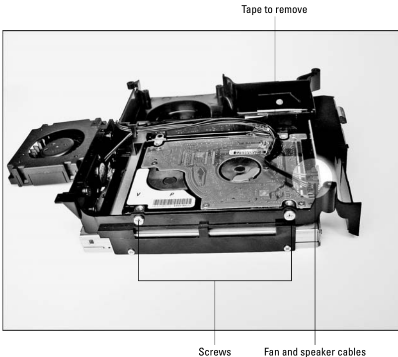
Figure 7-7: Remove the fan and place it to the side.
