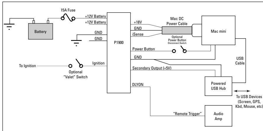
Figure 13-4: Wiring diagram for a Mac mini car installation using a DC-to-DC power converter.
