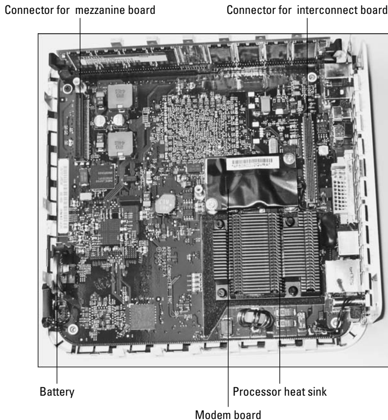
Figure 5-3: The motherboard sits in the bottom housing.
