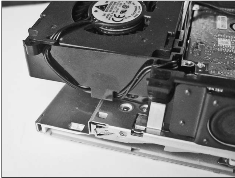
Figure 7-11: It may take a few attempts to route the fan cable properly as you replace the fan.
