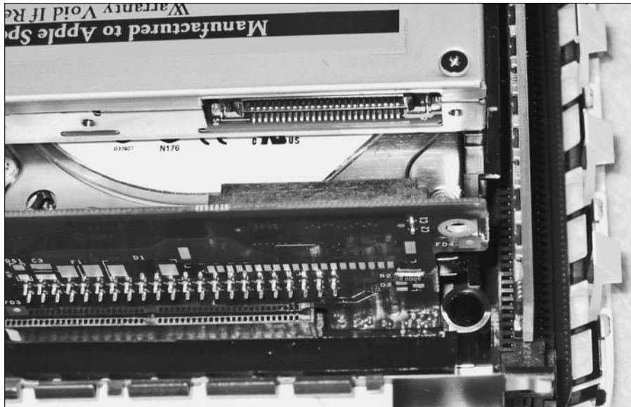
Figure 8-8: Slide the drive forward; note the connector.
