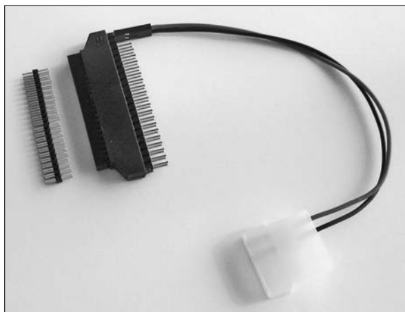
Figure 19-4: Beware: This converter adapter and a gender changer don't work.
