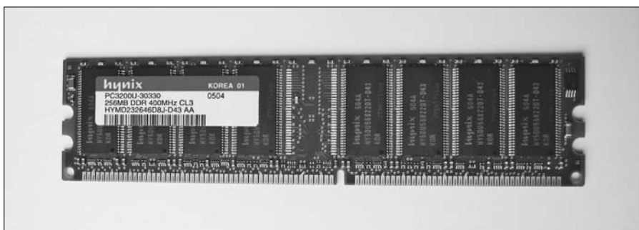
Figure 7-3: A RAM module has two sets of fingers of different sizes.
