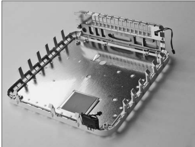
Figure 20-7: The bottom housing, with port holes in the back panel and the thermal pad at the front.
