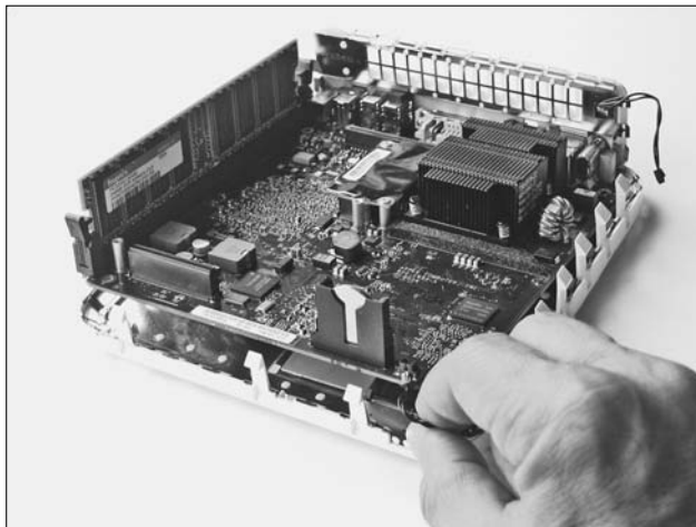
Figure 20-8: Pull the black LED panel back slightly while you lower the mother- board.
