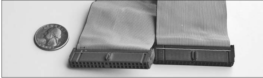
Figure 19-3: A standard 40-pin IDE connector for a 3.5- inch hard drive.
