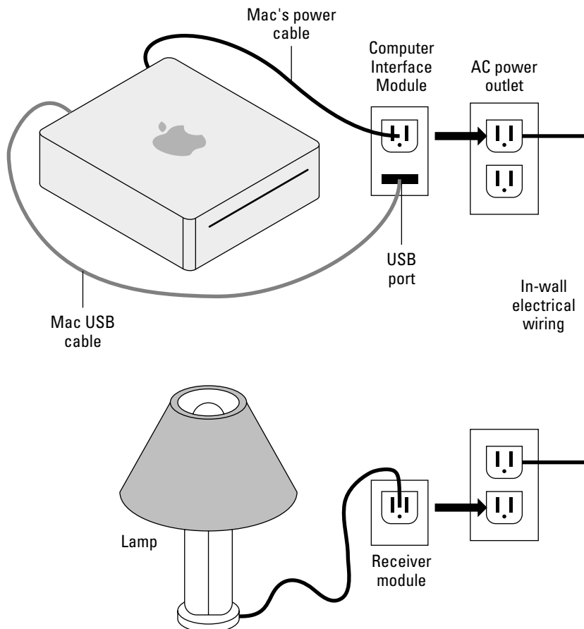
Figure 10-6: A basic X10 setup.
