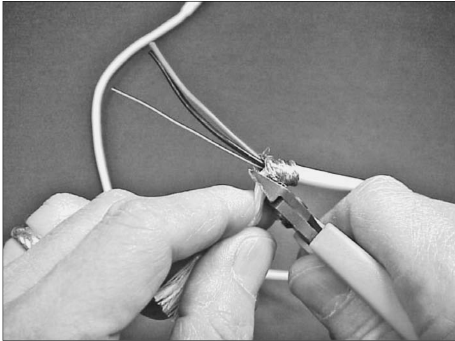
Figure 13-8: Carefully cut the fluff, avoiding the wires.
