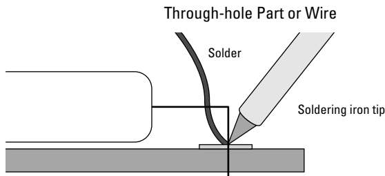
Figure 16-3: Heat both surfaces with the iron, and apply solder to the surfaces.
