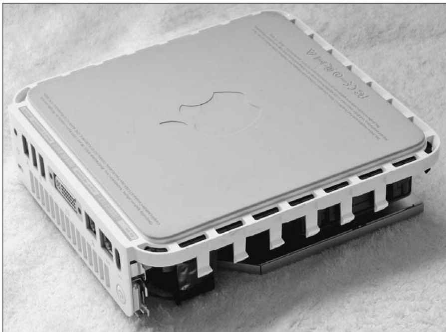
Figure 4-2: You open the Mac mini by pressing the white tabs inward.
