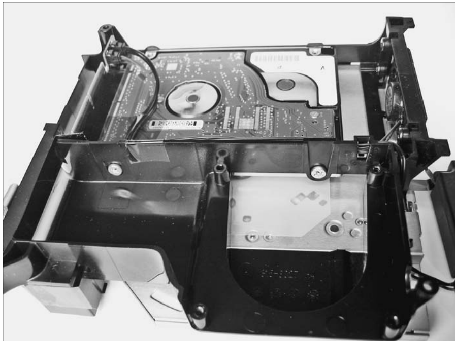
Figure 7-8: Remove the two screws (center) in the black frame.
