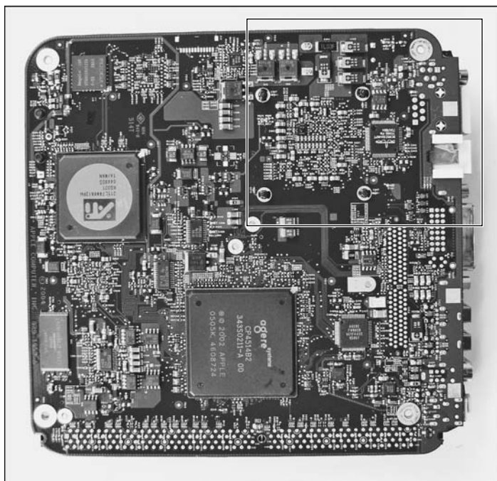
Figure 20-3: The bottom side of the motherboard.
