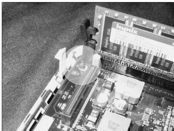
Figure 20-10: The motherboard screw.
