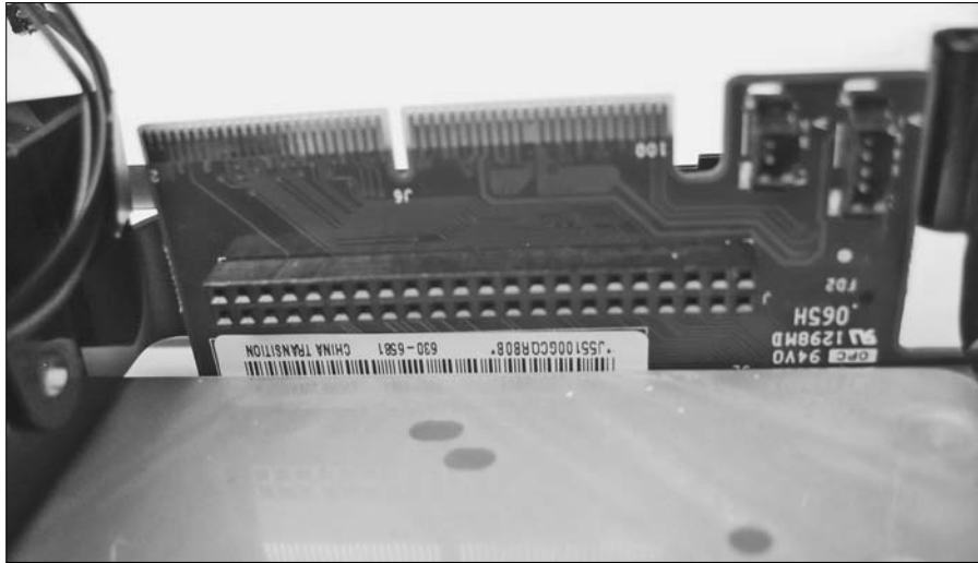
Figure 7-10: The hard drive connector and the fan and speaker connectors.
