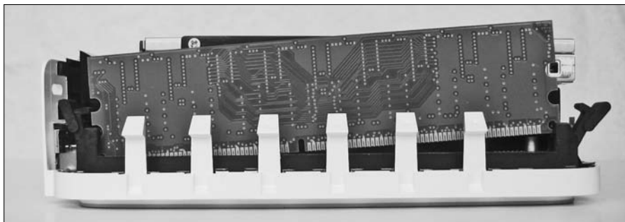
Figure 7-2: Begin removing the RAM module by pulling up on the right side.
