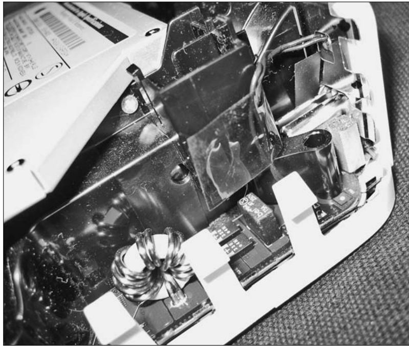
Figure 5-6: Peel back this bit of tape to detach this small cable from the internal frame.
