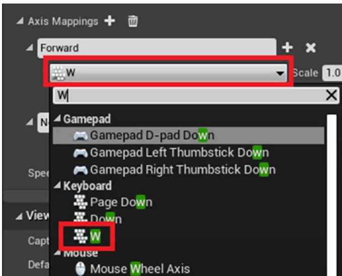
Figure 12-13. Adding a key binding
