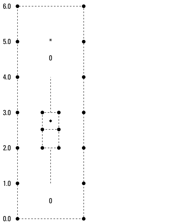
Figure 19-8: Mean 2.75 A box and Median 2.50 whisker 75th percentile 3.00 plot. 25th percentile 2.00 Standard deviation 0.50
