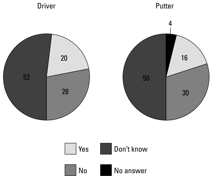
Figure 19-1: Black-and-white pie charts.
