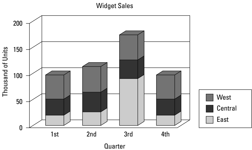
Figure 19-4: A stacked bar chart with mis- leading 3-D effects.
