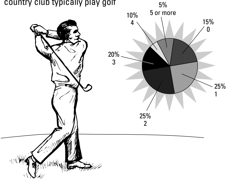
Figure 19-2: A pie chart with attention-getting graphics.
