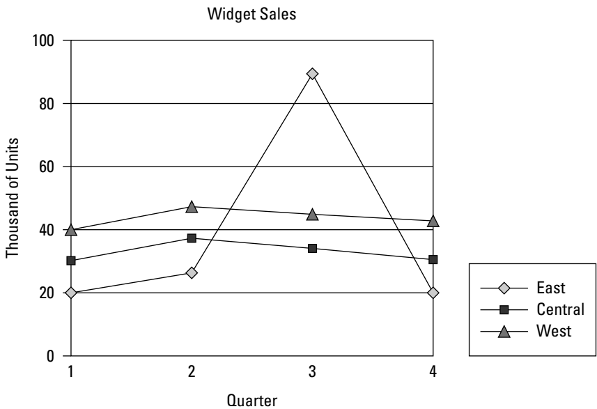
Figure 19-5: A multi-line graph.
