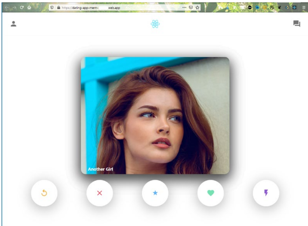
Figure 2-1. Finished app
