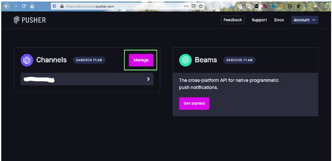
Figure 4-16. Pusher dashboard
