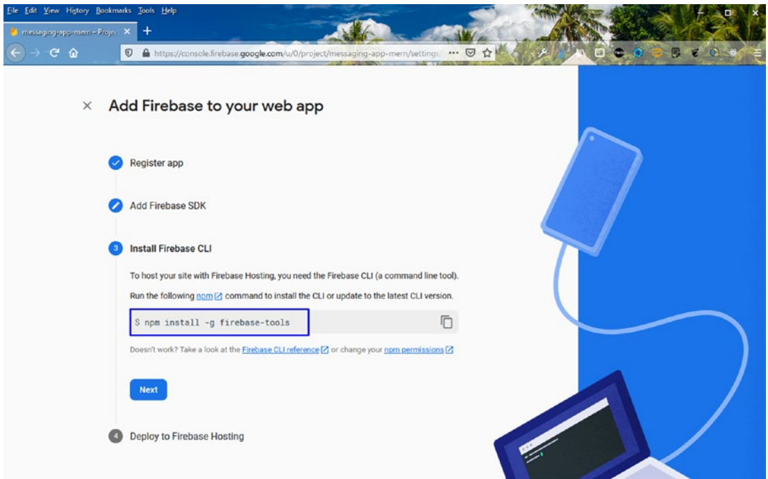
Figure 4-29. Global install
