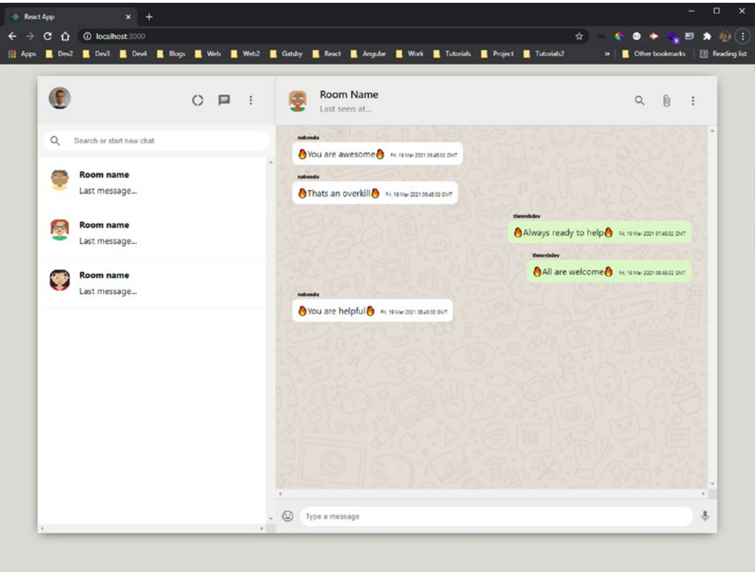
Figure 4-23. New messages
