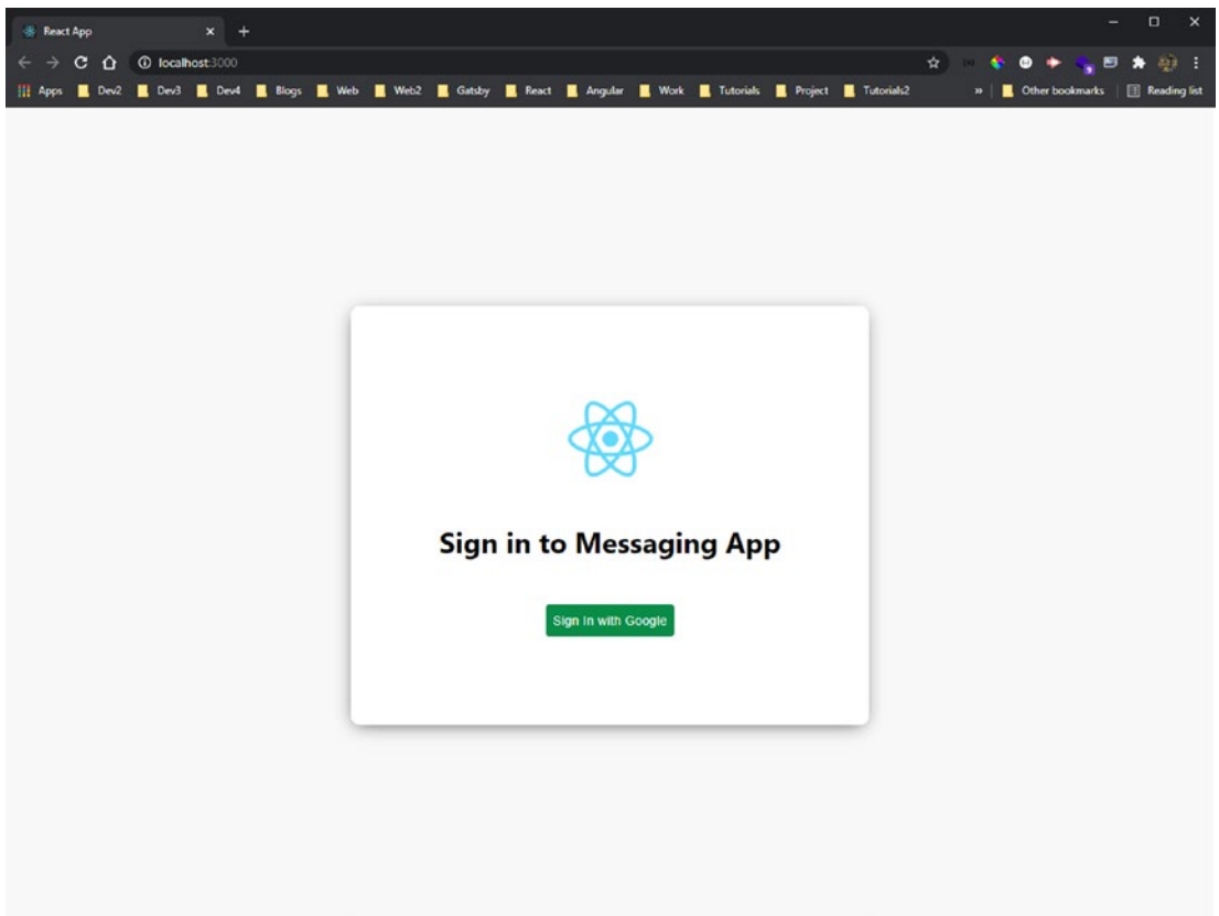
Figure 4-32. Login screen
