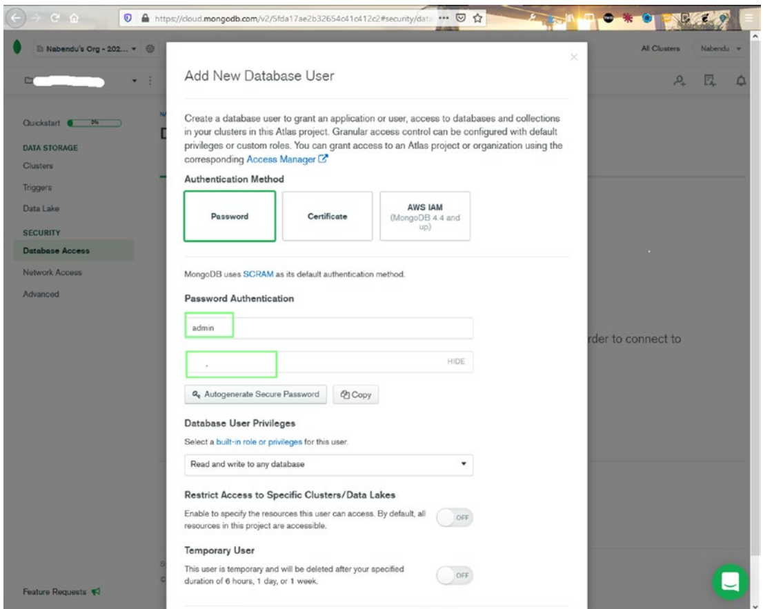
Figure 1-14. Add user
