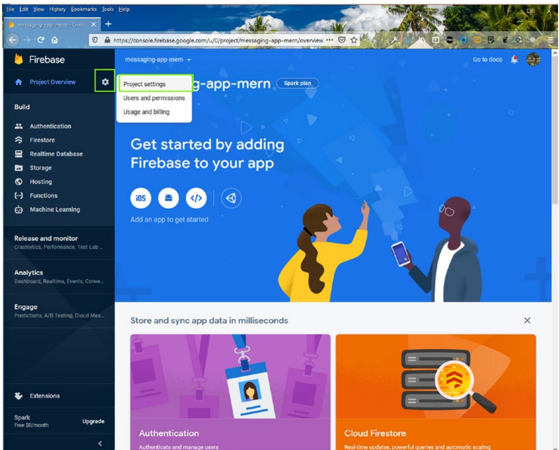
Figure 4-25. Additional settings
