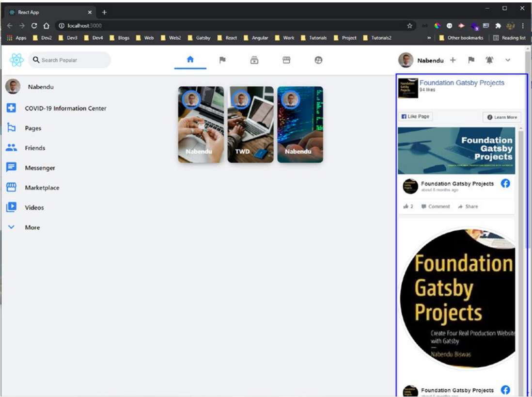
Figure 6-8. Widget shown
