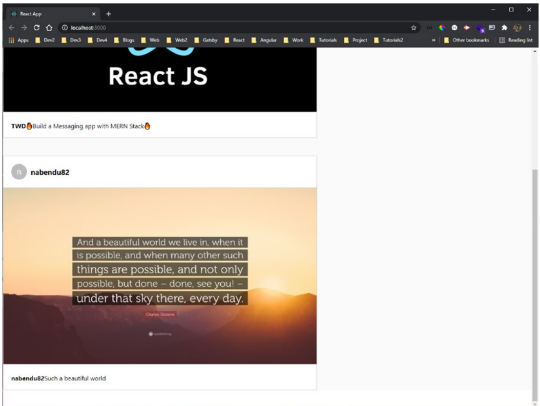
Figure 5-6. Everything dynamic
