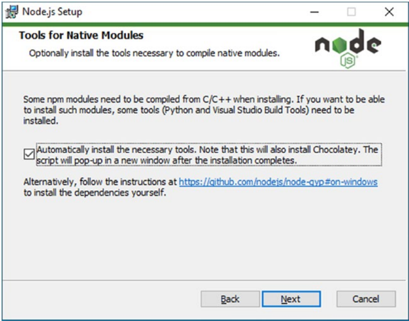
Figure 1-36. Dependencies
