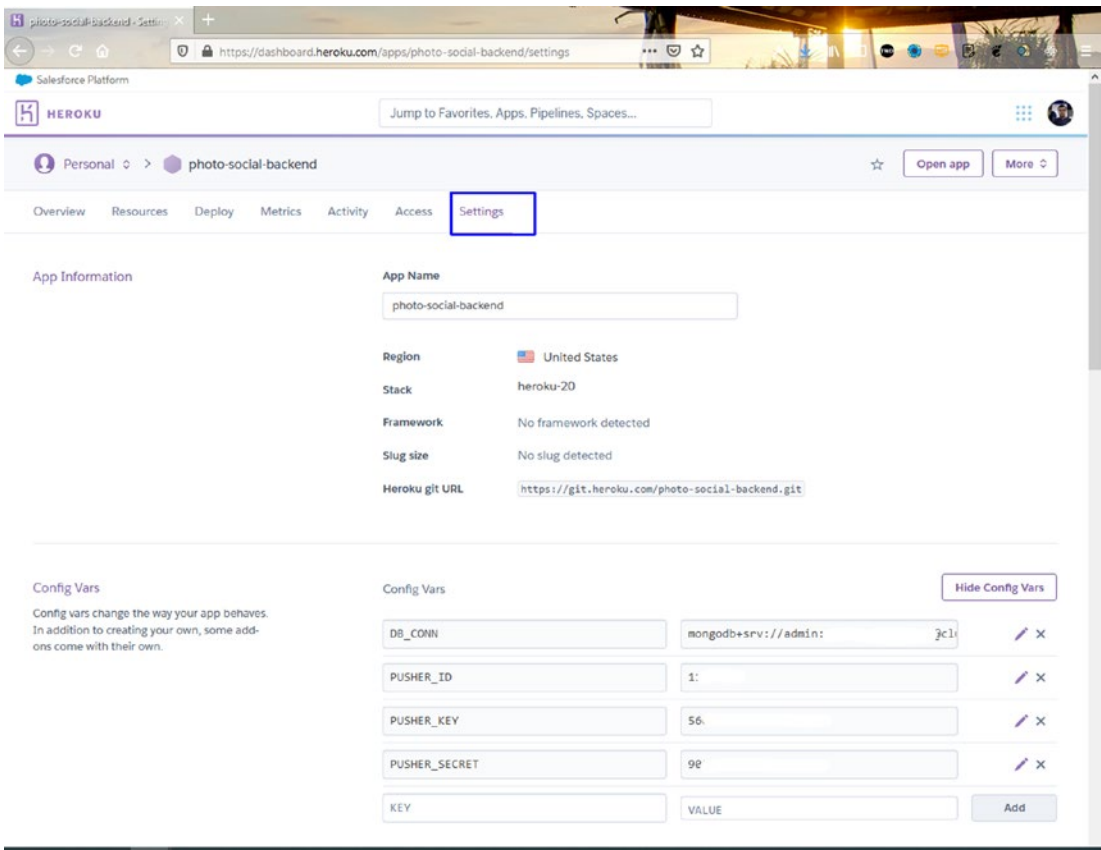
Figure 5-26. Environment variables in Heroku
