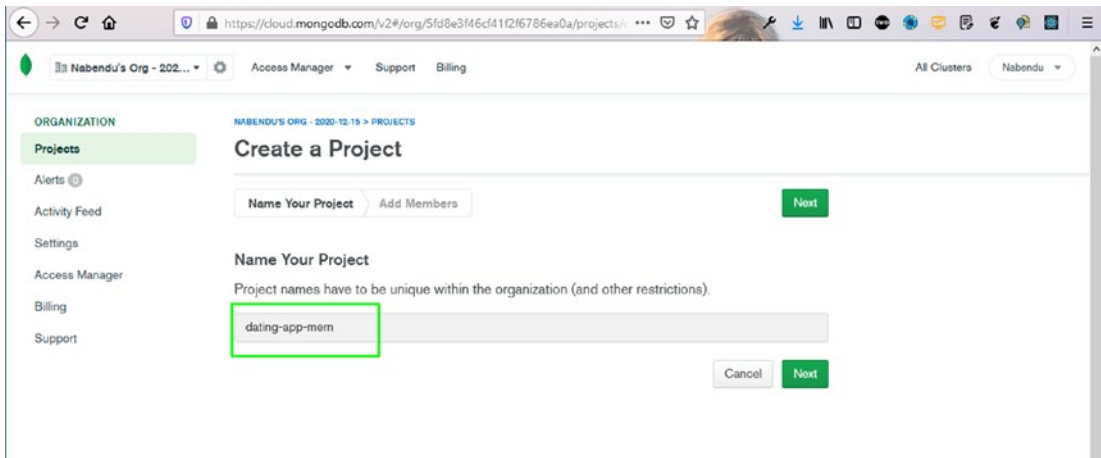
Figure 1-7. Project name
