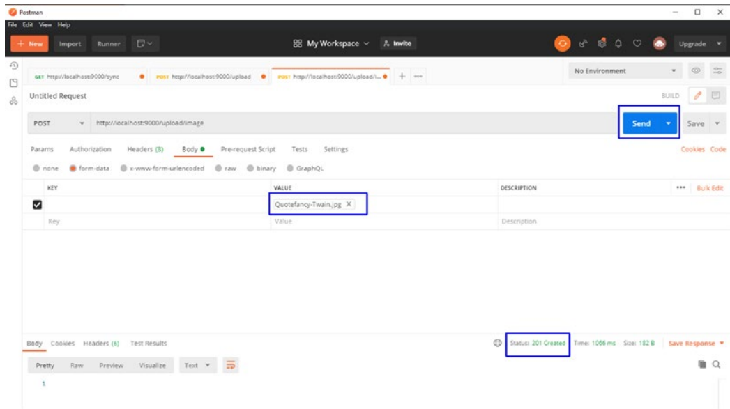
Figure 6-18. Post image
