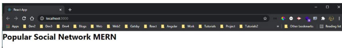
Figure 6-2. Initial app
