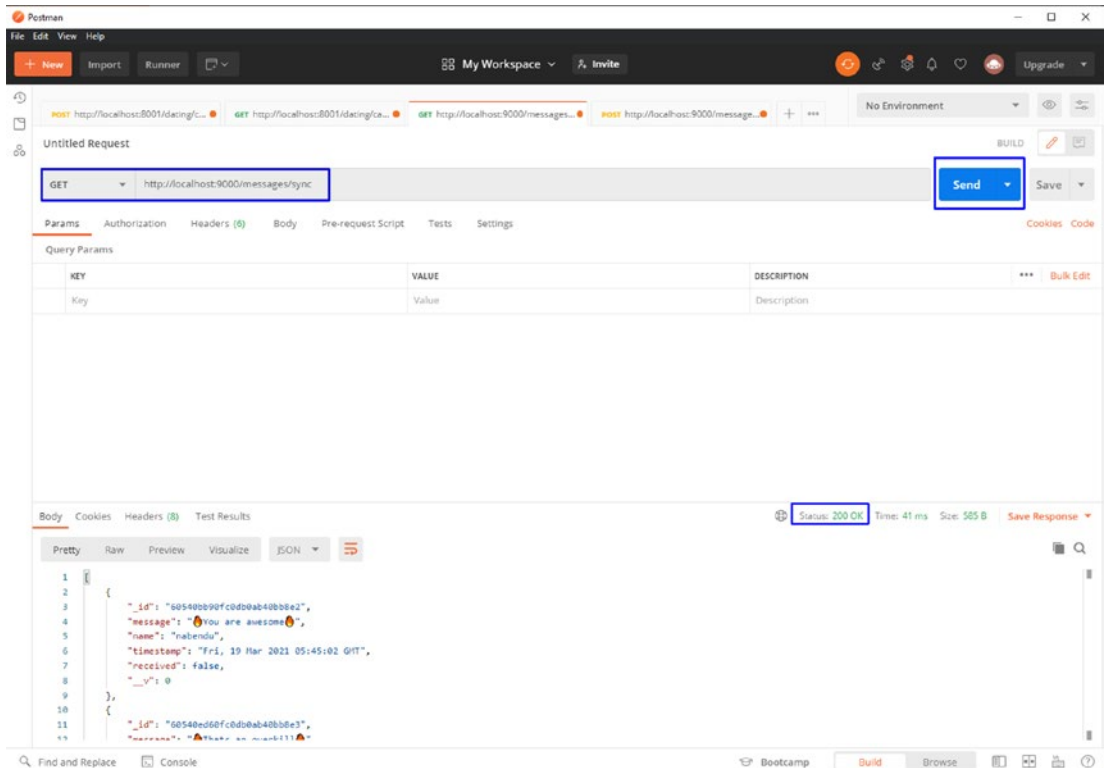
Figure 4-14. GET request
