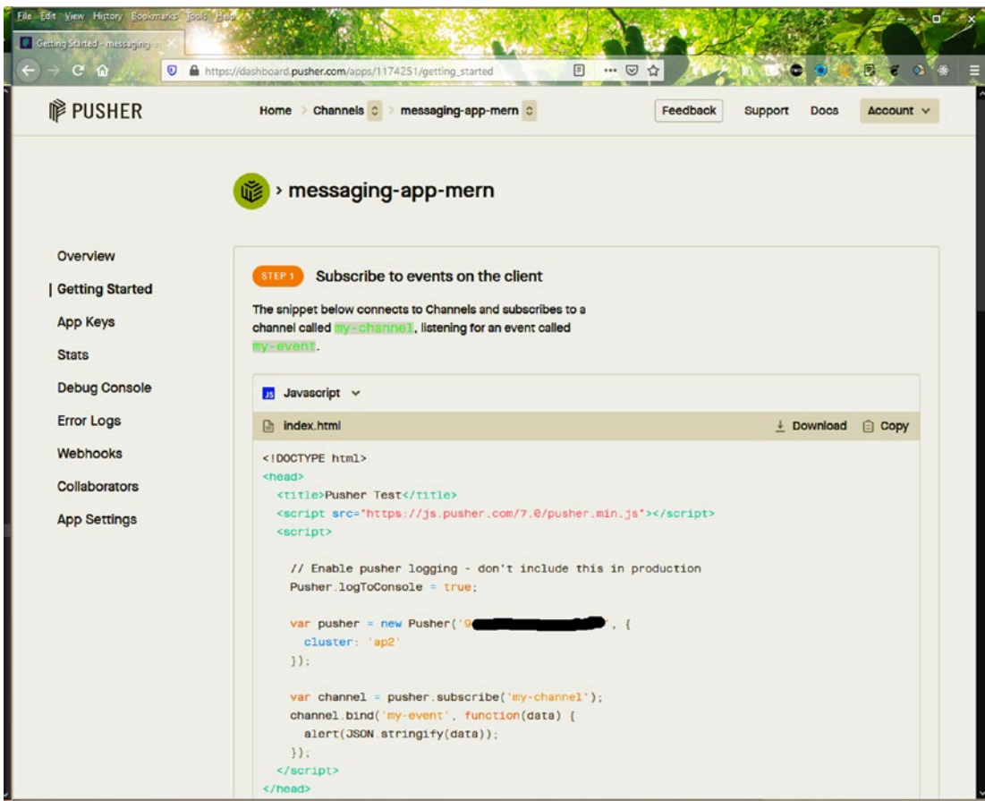
Figure 4-19. Back-end code
