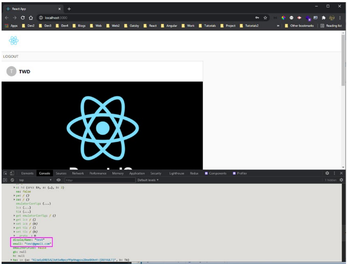
Figure 5-12. User sign-up
