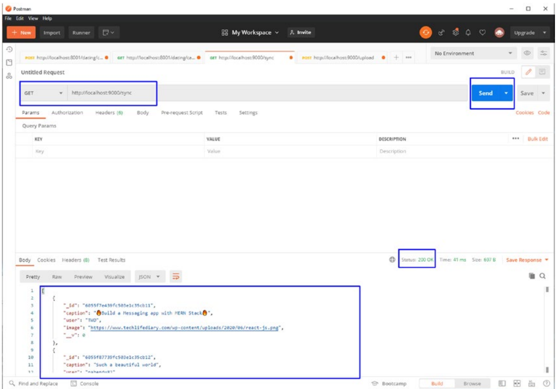
Figure 5-19. Postman GET
