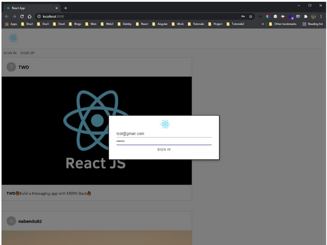
Figure 5-13. Sign-in popup
