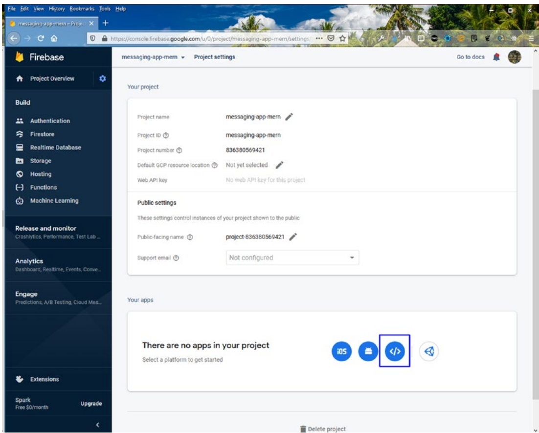
Figure 4-26. Web icon
