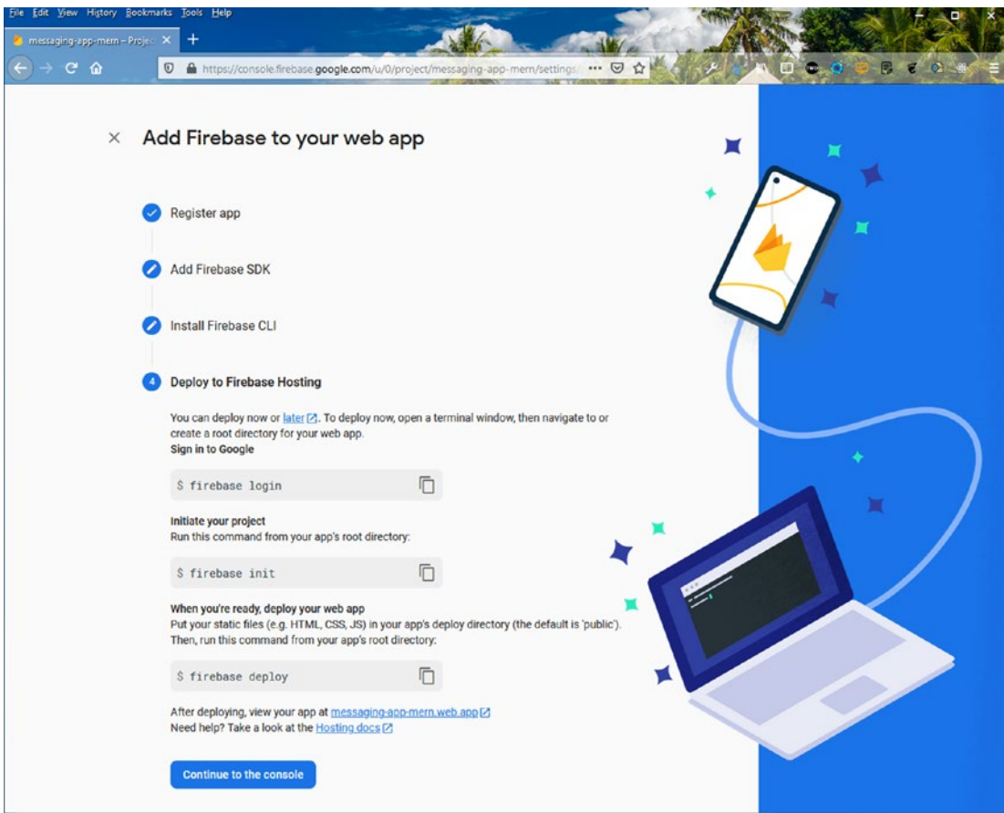
Figure 4-30. Continue
