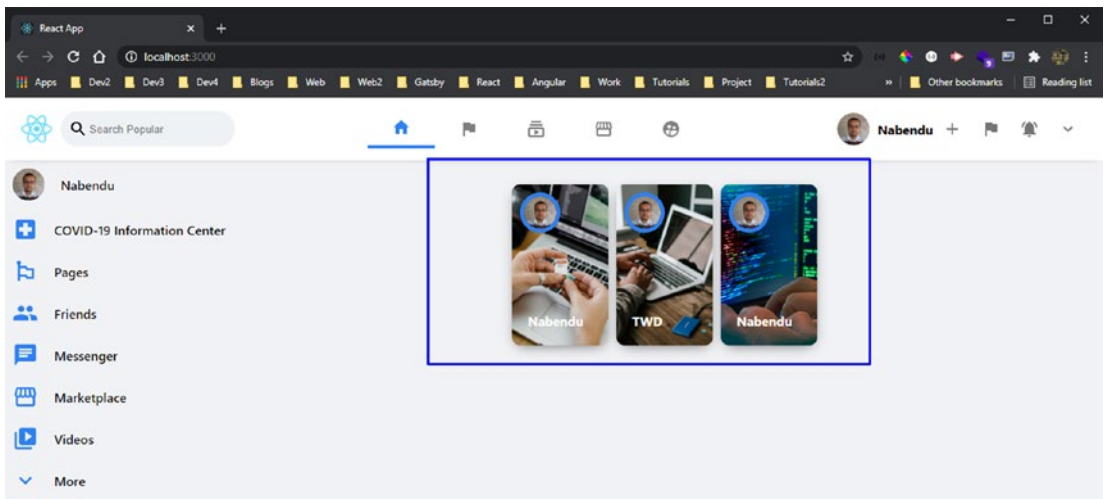
Figure 6-5. Nice image
