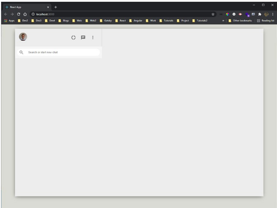
Figure 4-5. Search bar
