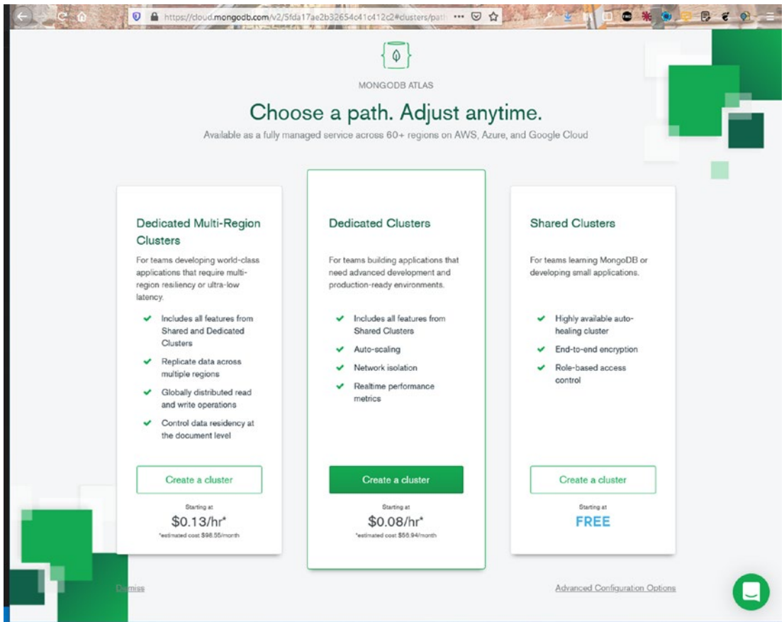
Figure 1-10. Free tier
