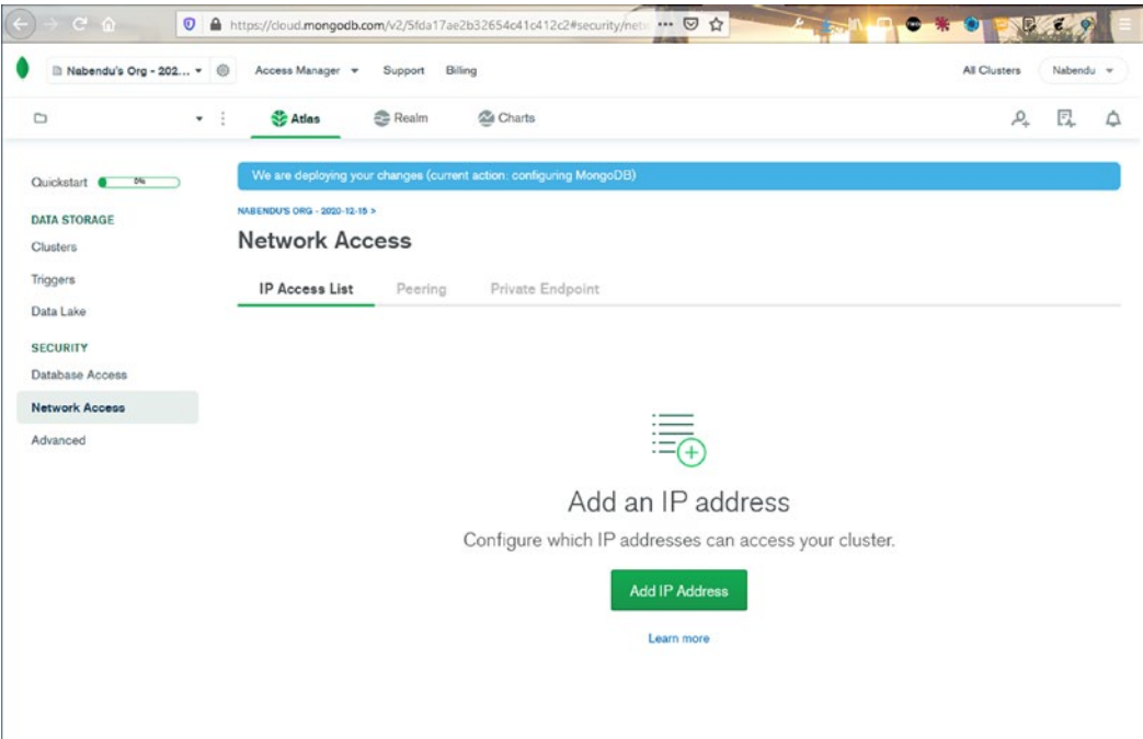
Figure 1-15. Network access
