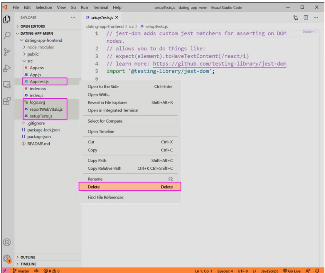
Figure 2-2. Delete files
