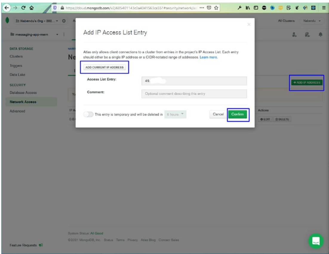
Figure 5-20. Add current IP
