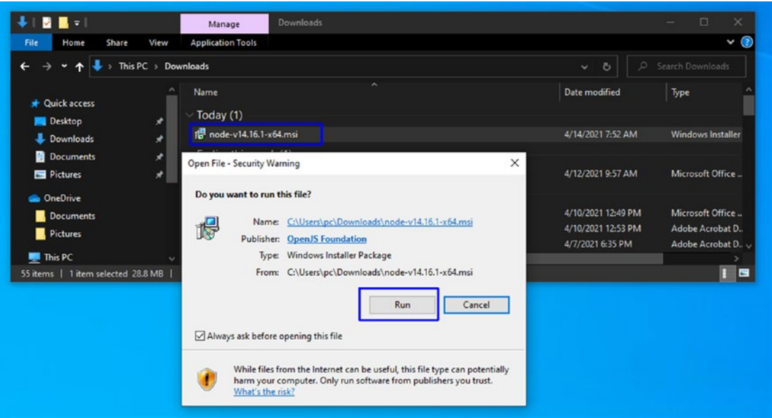
Figure 1-31. Run button
