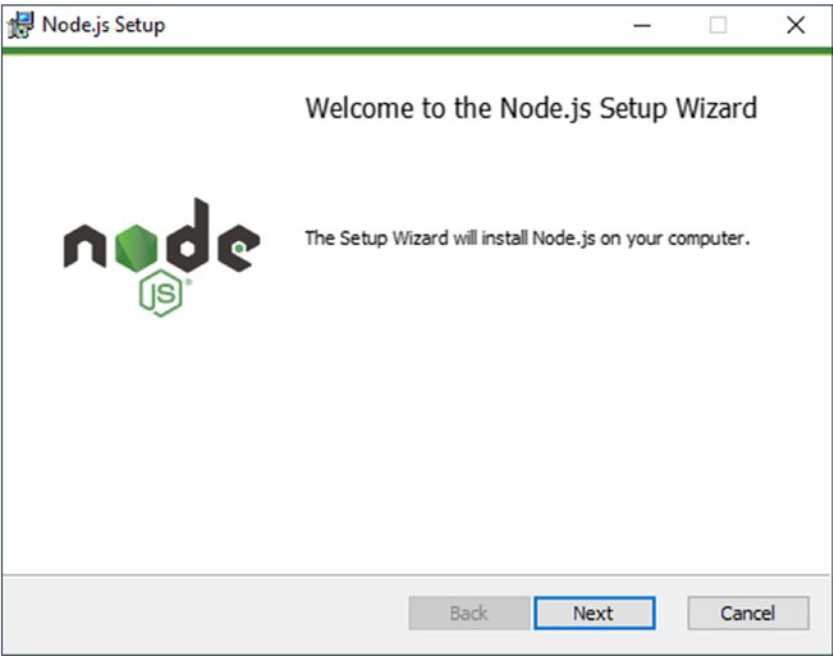
Figure 1-32. Node.js welcome
