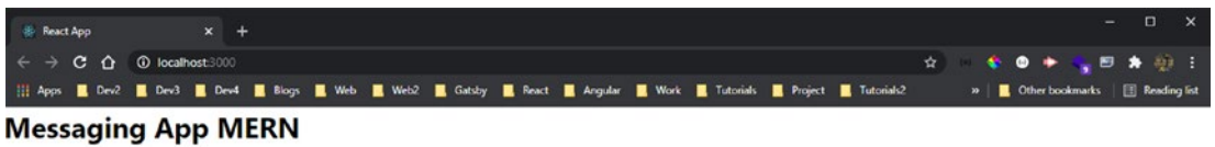
Figure 4-2. Initial app
