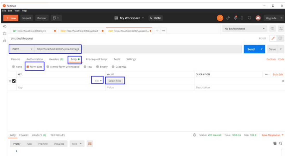
Figure 6-17. POST request
