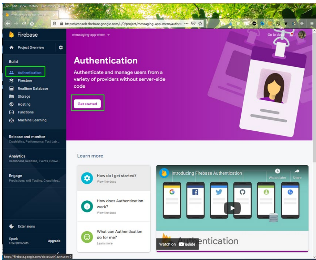
Figure 4-33. Get started
