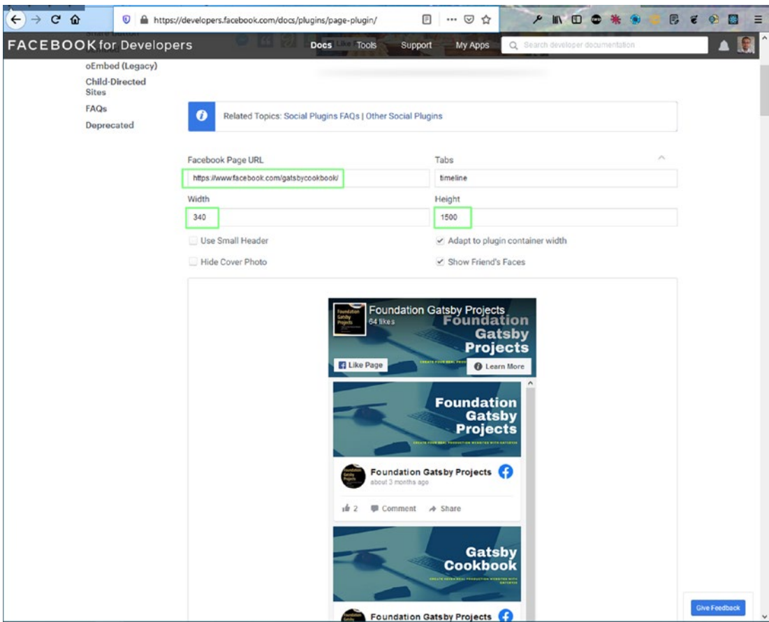
Figure 6-6. Adding widget
