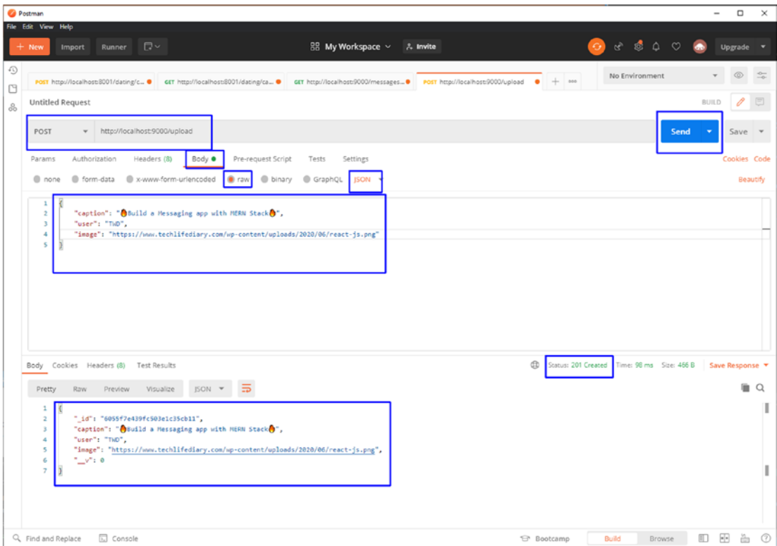
Figure 5-18. Postman POST
