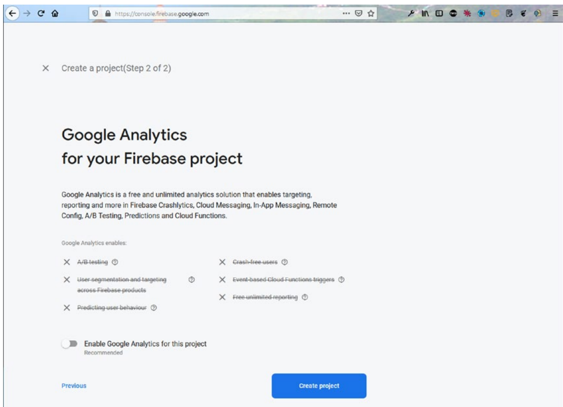
Figure 1-4. Create project
