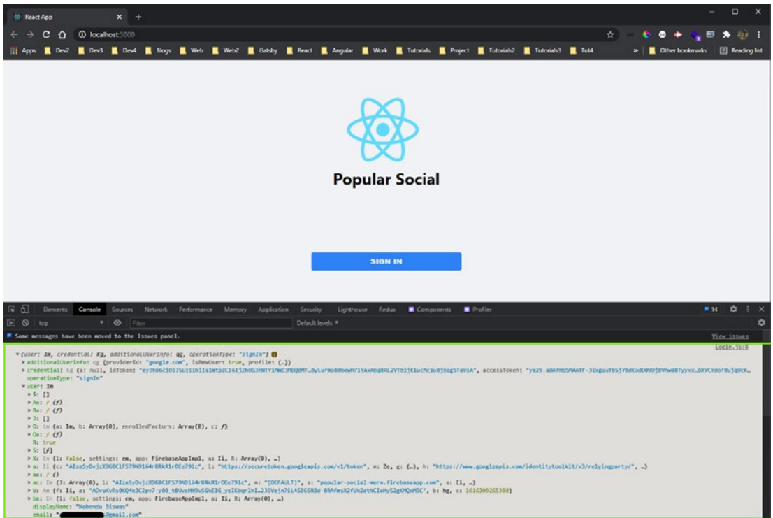
Figure 6-12. Login details
