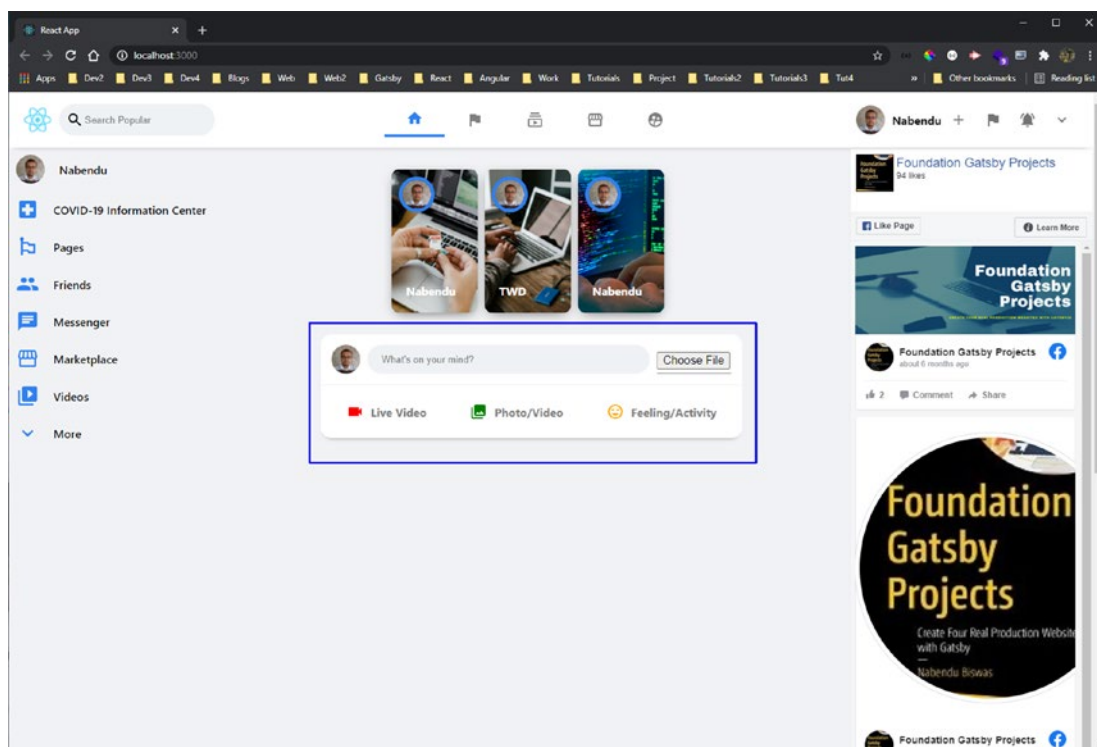
Figure 6-9. Messenger component
