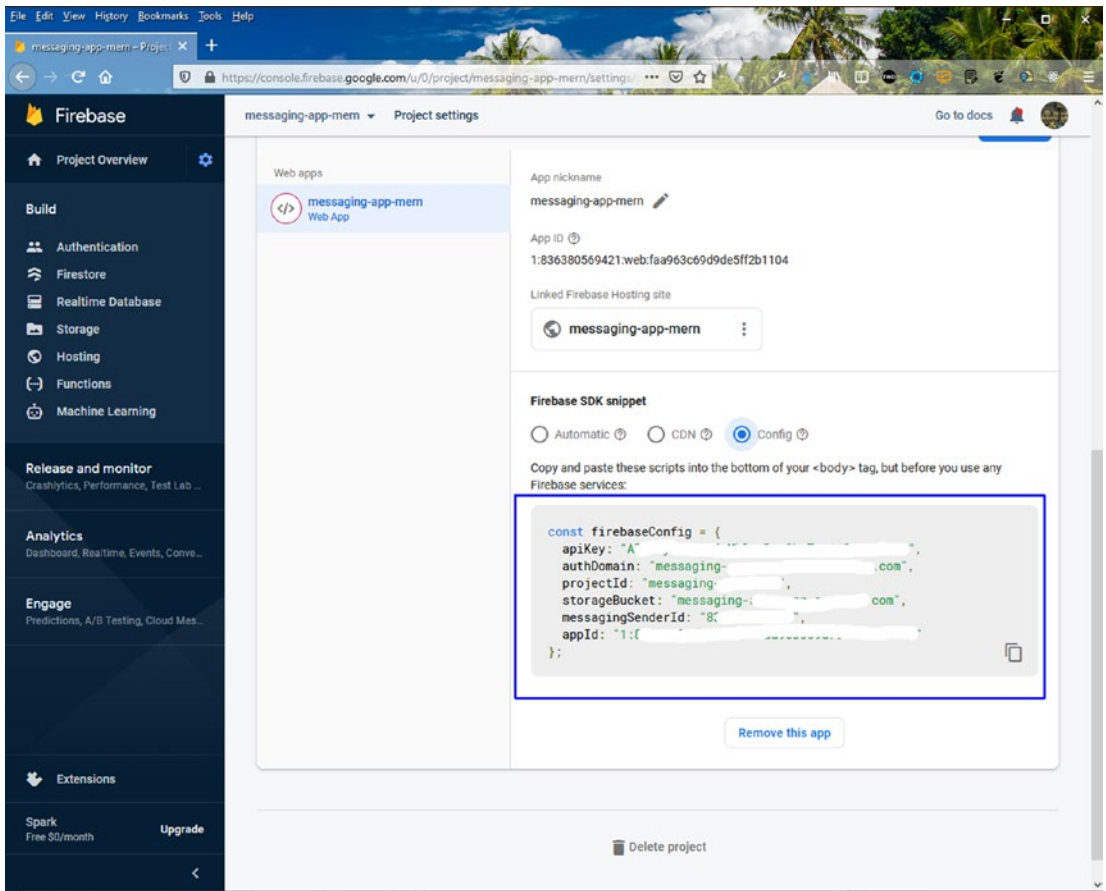
Figure 4-31. Config details
