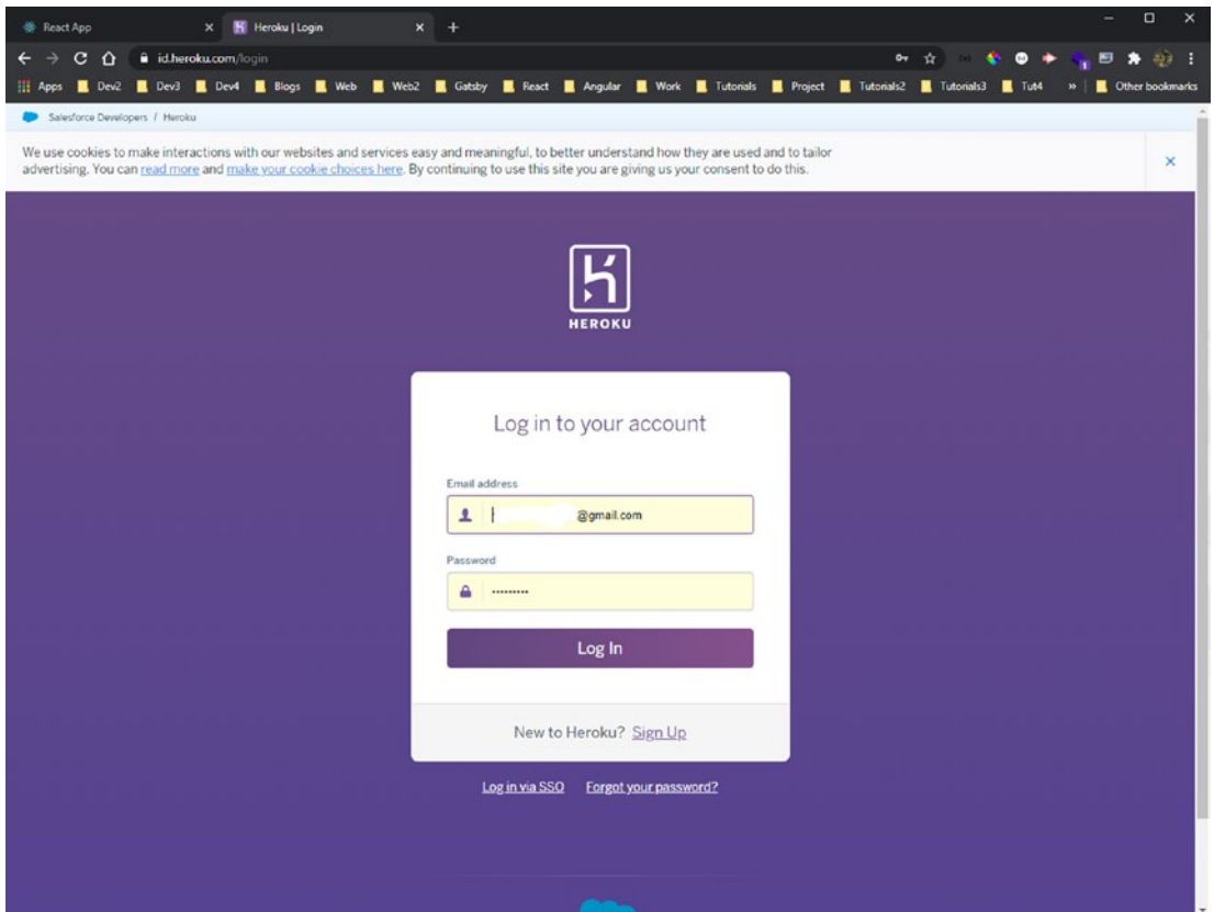
Figure 1-23. Login credentials
