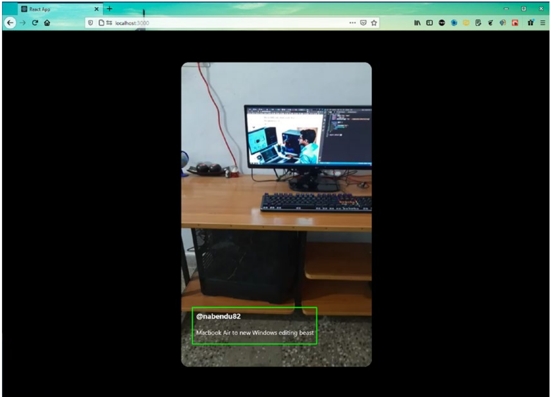
Figure 3-5. Initial footer
