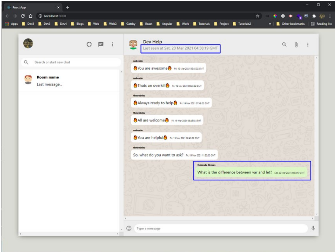
Figure 4-39. Time updates
