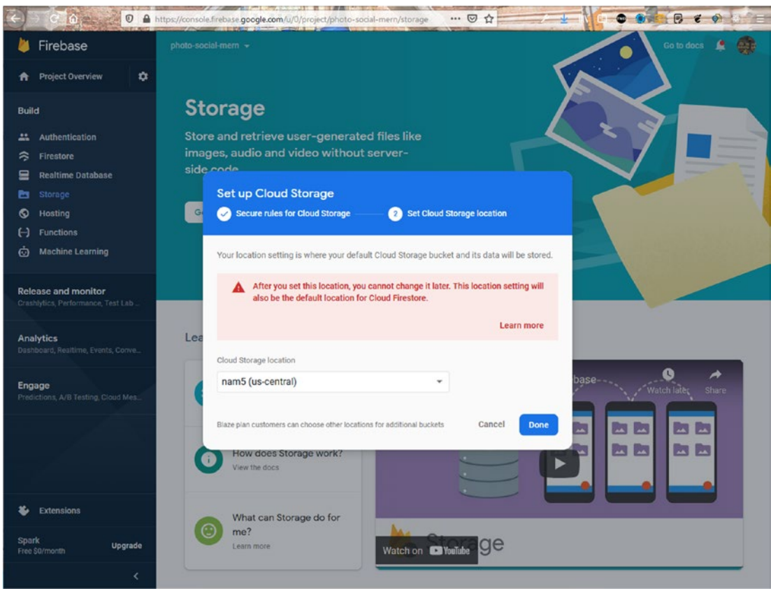
Figure 5-22. Cloud storage
