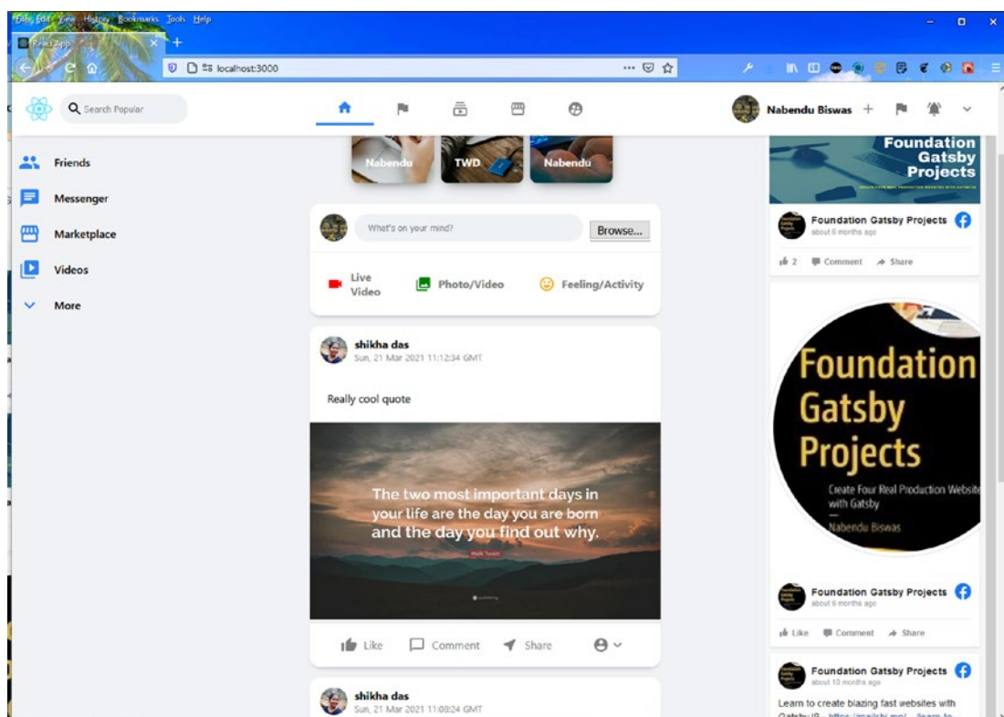
Figure 6-21. Problem
