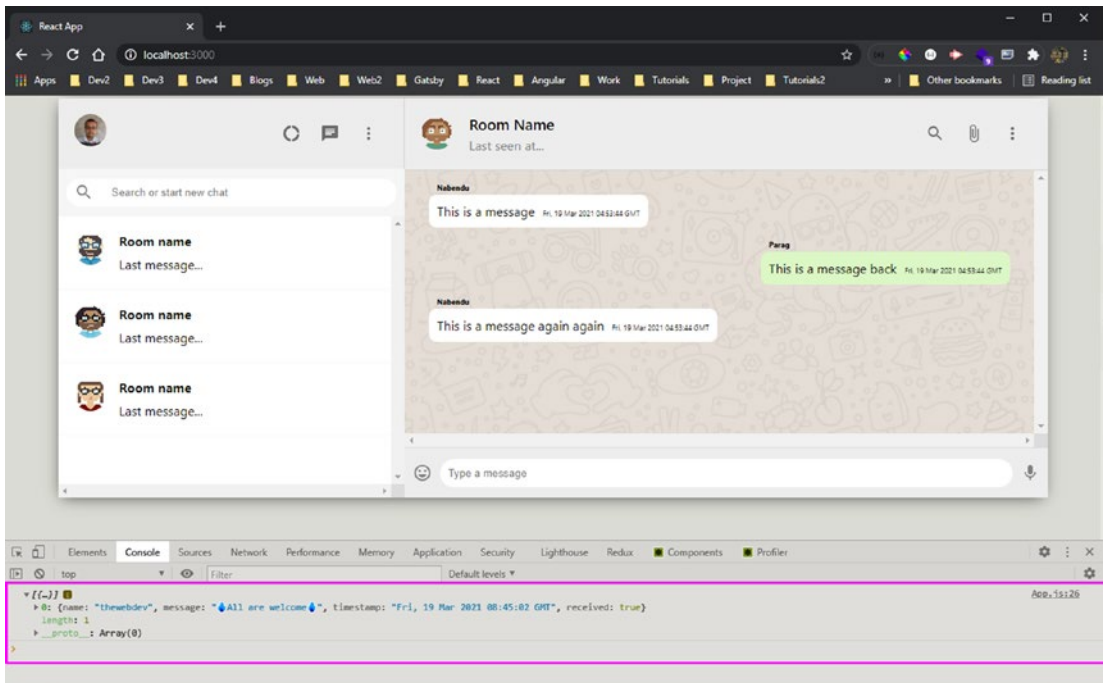
Figure 4-22. Console log
