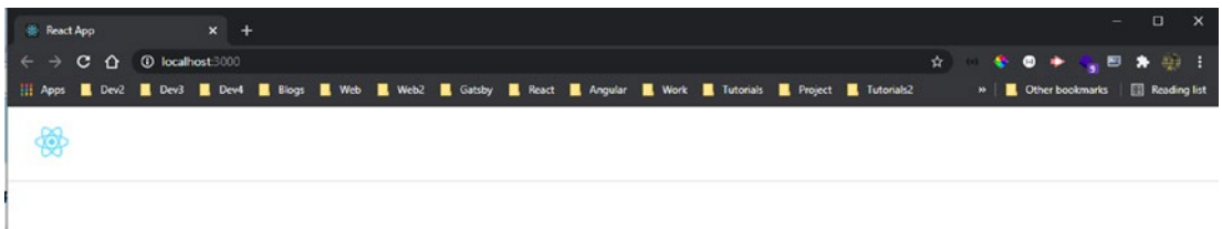
Figure 5-4. Perfect logo
