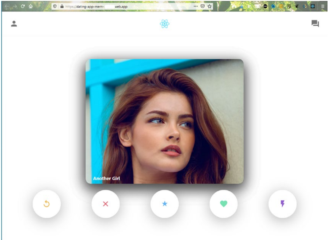
Figure 2-15. Deployed app
