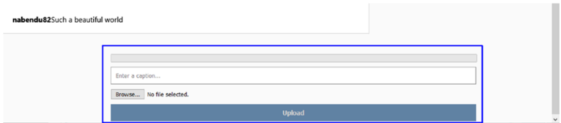
Figure 5-14. Image upload
