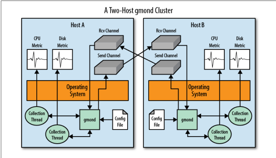
Figure 1-2. gmond architecture
