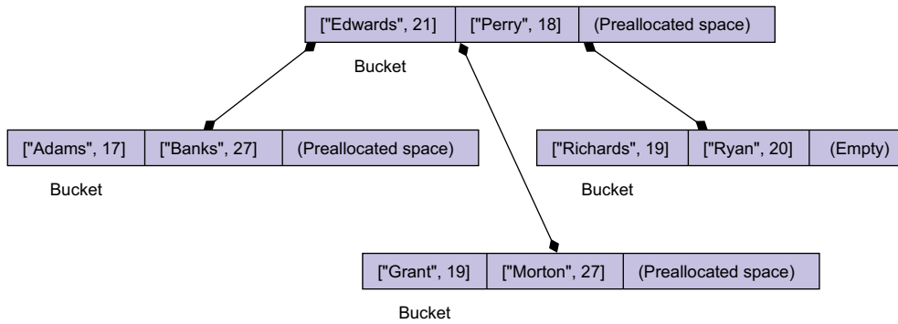
Figure 8.5 Sample B-tree structure
