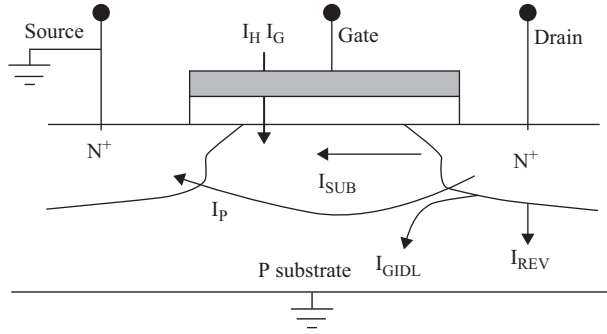
Figure 5.4 Leakage current components in NMOS transistor (Source: N. Ekekwe, 2006, p.853 [19])
