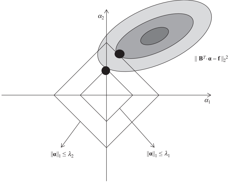
Figure 1.2 L_1 -norm regularization \|\alpha\|_1 \leq \lambda results in a sparse solution (i.e., \alpha_1 = 0 ), if \lambda is sufficiently small (i.e., \lambda = \lambda_1 )
