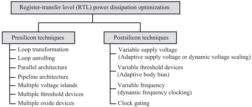
Figure 9.4 Various techniques for RTL power optimization
