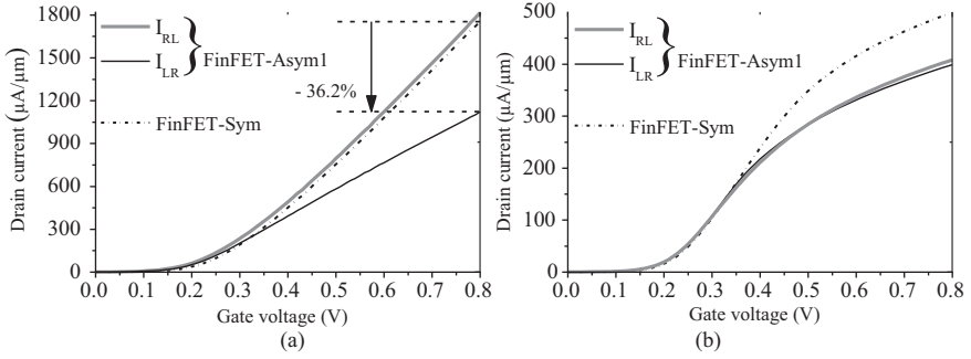
Figure 4.9 Comparison of drain currents that are produced by asymmetrical n -type tied-gate FinFET-Asym1 and symmetrical n -type tied-gate FinFET-Sym. (a) Saturation region drain current. V_{drain} = 0.8 V . V_{source} = 0 V . (b) Linear region drain current. V_{drain} = 50 mV . V_{source} = 0 V . T = 25^\circ C
