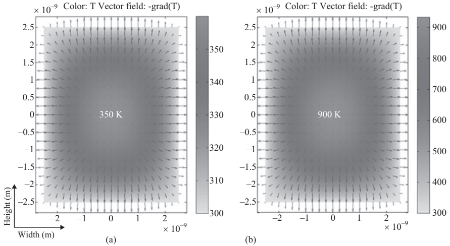
Figure 6.9 Cross-sectional temperature distributions and heat flow vector (arrow) for (a) 10 mA, D = 1 nm, L = 1 \mu m, (b) 10 mA, D = 4 nm, L = 1 \mu m. In case of (b) central shell temperature is above melting point (873 K), therefore breakdown will occur
