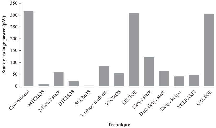
Figure 5.20 Standby power dissipation for NAND3 at 65 nm technology node
