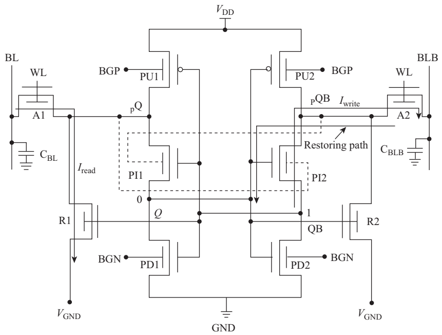
Figure 3.26 Hybrid 10T SRAM cell with selective back-gate biasing
