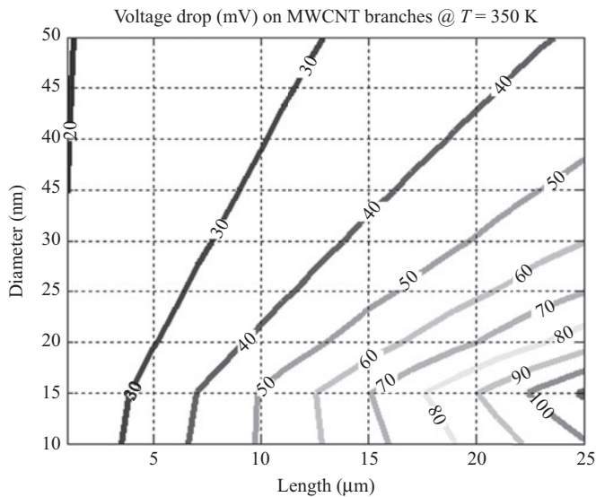
Figure 7.13 Voltage drop for MWCNT interconnects with different lengths and diameters for T = 350 K
