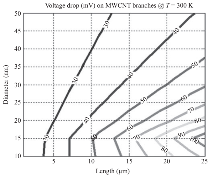
Figure 7.12 Voltage drop for MWCNT interconnects with different lengths and diameter for T = 300 K
