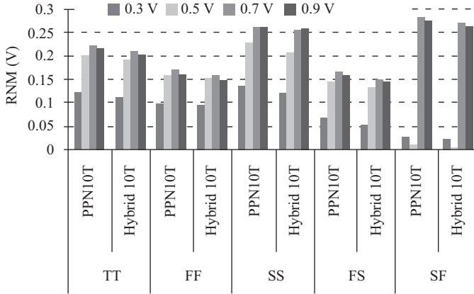
Figure 3.18 RNM at different process corners (PCs) for IG-FinFET-based SRAM cells (Source: Yadav, 2015, p. 12 [36])
