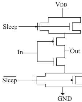
Figure 5.16 Dual sleepy stack (Source: M. S. Islam, 2010, p.90 [59])
