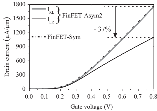
Figure 4.15 Comparison of saturation region drain currents that are produced by n -type FinFET-Asym2 and FinFET-Sym for various gate voltages. V_{drain} = 0.8\text{ V} . V_{source} = 0\text{ V} . T = 25^\circ\text{C}
