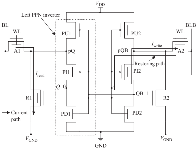
Figure 3.11 IG-FinFET-based PPN 10T SRAM cell (Source: Yadav, 2015, p. 4 [36])
