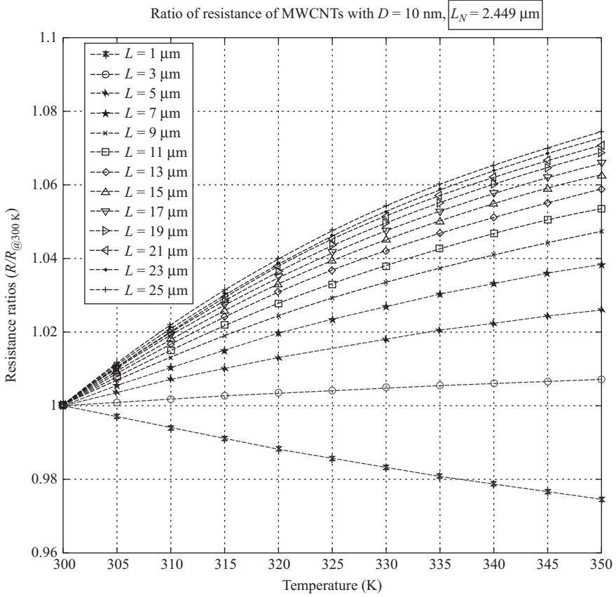
Figure 7.10 Resistance ratio for MWCNTs with D = 10 nm for various lengths. Note that L_N = 2.449 \mu\text{m}
