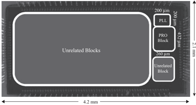
Figure 2.25 Showing the chip micrograph with the RRO block and PLL [37].
