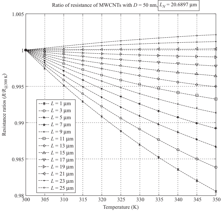
Figure 7.11 Resistance ratio for MWCNTs with D = 50 nm for various lengths. Note that L_N = 20.6897 \mu\text{m}
