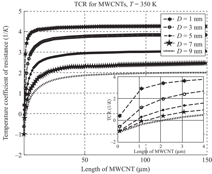
Figure 7.6 TCR for MWCNTs for longer lengths (i.e. up to 150 \mu\text{m} ) and outer diameters (i.e. 1\text{--}10 nm). The inset shows the TCR for shorter lengths MWCNTs
