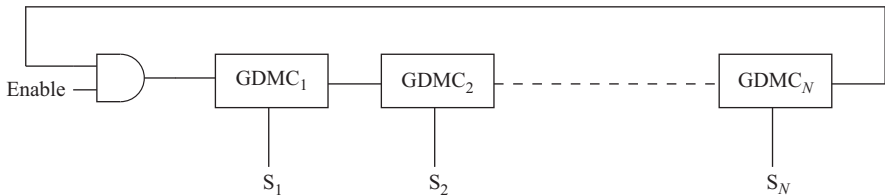
Figure 2.6 RO based on GDMC [28]. © 2009 IEEE
