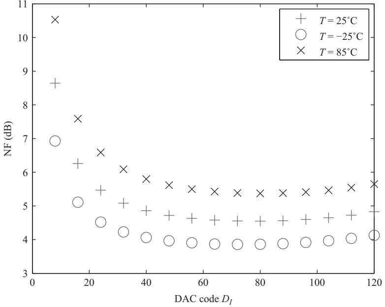
Figure 1.13 Simulated 60 GHz NF vs. current DAC code D_I at T = 25^\circ\text{C} , T = -25^\circ\text{C} , and T = 85^\circ\text{C}
