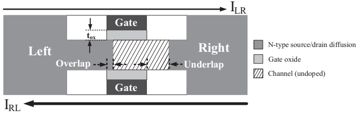
Figure 4.6 Cross-sectional view (along the gate length) of an asymmetrical n-type tied-gate FinFET-Asym1
