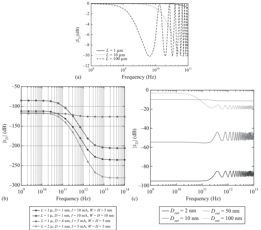
Figure 6.12 Scattering parameter S_{12} of various interconnects (a) SWCNT, (b) SWCNT bundle based and (c) MWCNT
