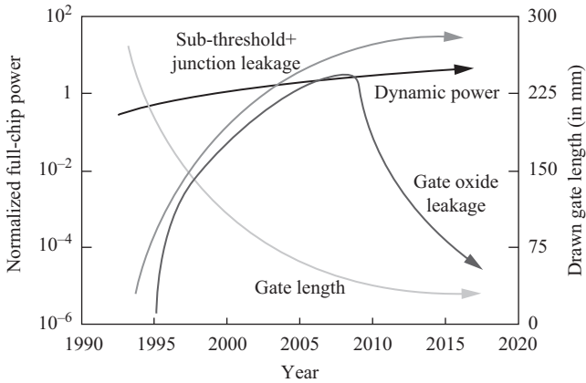
Figure 5.5 Power dissipation and physical gate length trends (Source: Z. Abbas, 2014, p.180 [28])
