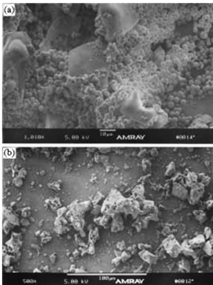
FIGURE 3.4 SEM micrographs of calcined mesoporous silica stirred for: (a) 0.5; and (b) 16 h.
