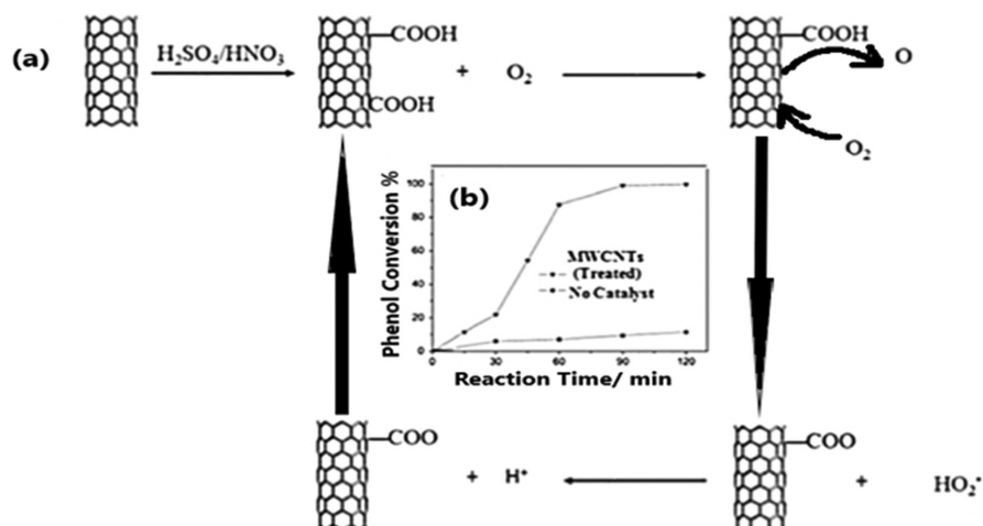
FIGURE 10.6 (a) Mechanism of producing the radical ( \text{HO}_2^\bullet ) in CWAO for phenol breakdown by \text{H}_2\text{SO}_4/\text{HNO}_3 treated MWCNTs; (b) efficiency of phenol removal.
