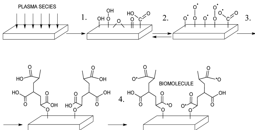
SCHEME 11.2 Multistep approach of biomolecules binding: (1) Plasma treatment, (2) Generation radicals, (3) AA radical graft polymerization, (4) Antibacterial deposition.
