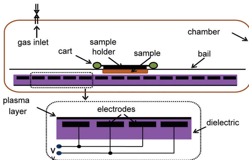
SCHEME 11.1 Scheme of device for DSBD plasma treatment.
