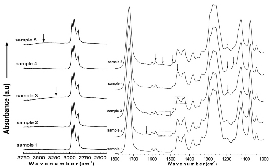
FIGURE 11.2 FTIR spectra of PVC samples 1–5 with different range of wavenumbers.
