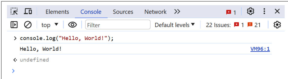
Figure 3-2. JavaScript example
