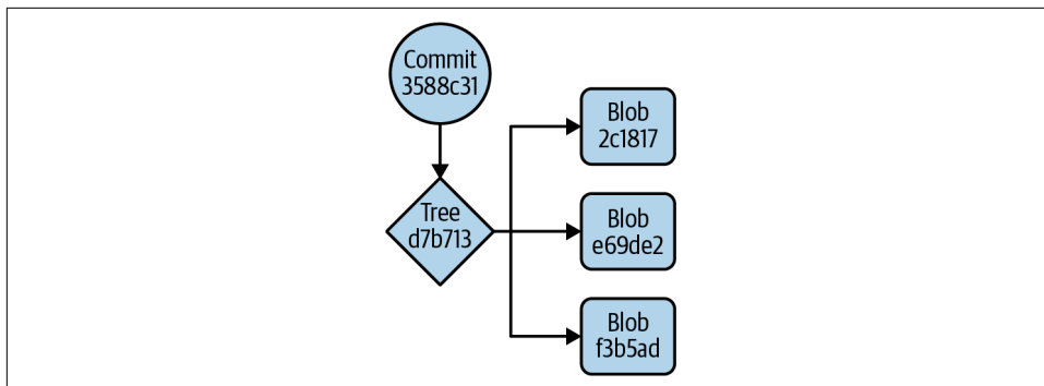
Figure 11-1. Objects in a Git repository
