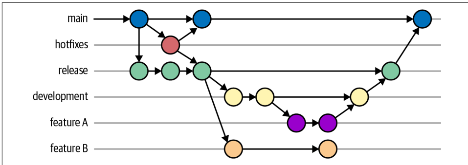
Figure 11-8. Multiple branches in a development cycle
