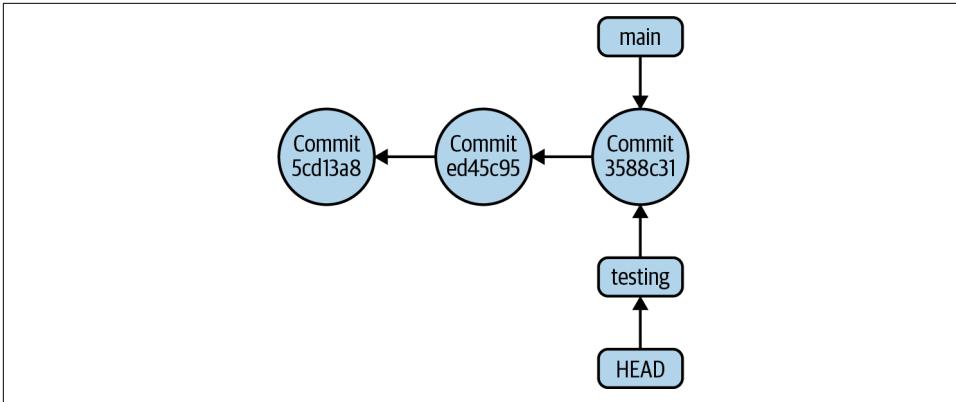
Figure 11-6. HEAD pointing to a checked-out branch
