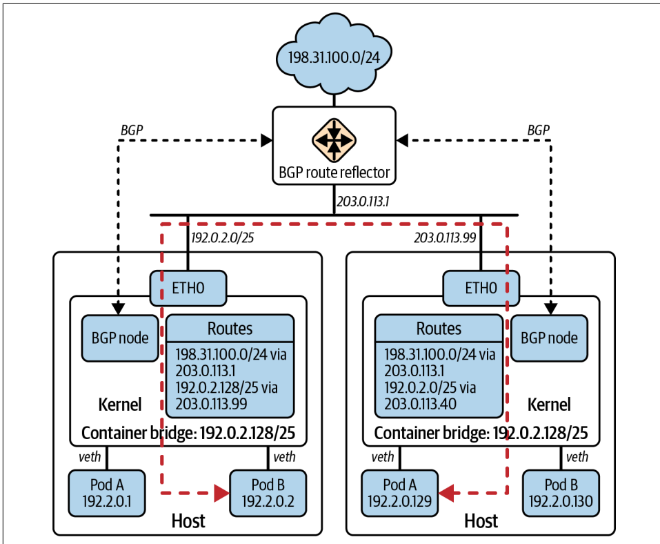
Figure 4-4. Kubernetes networking with BGP
