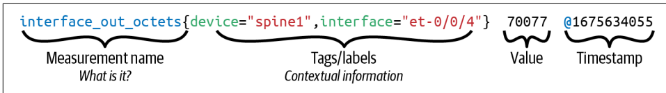
Figure 14-7. Prometheus metric format
