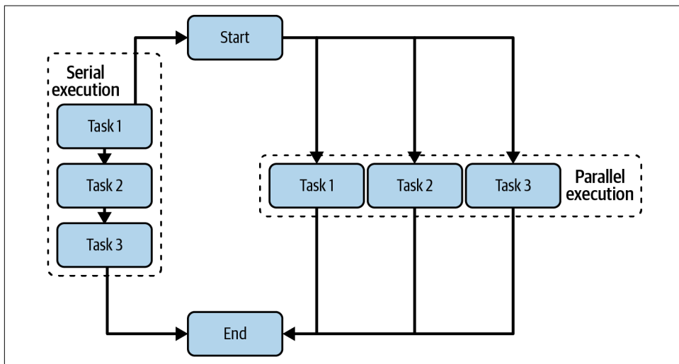
Figure 6-1. Serial versus parallel execution
