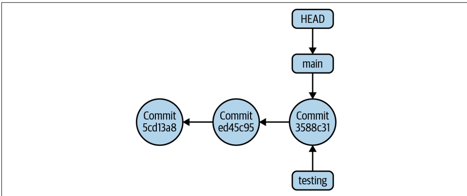
Figure 11-5. New branch created in a Git repository
