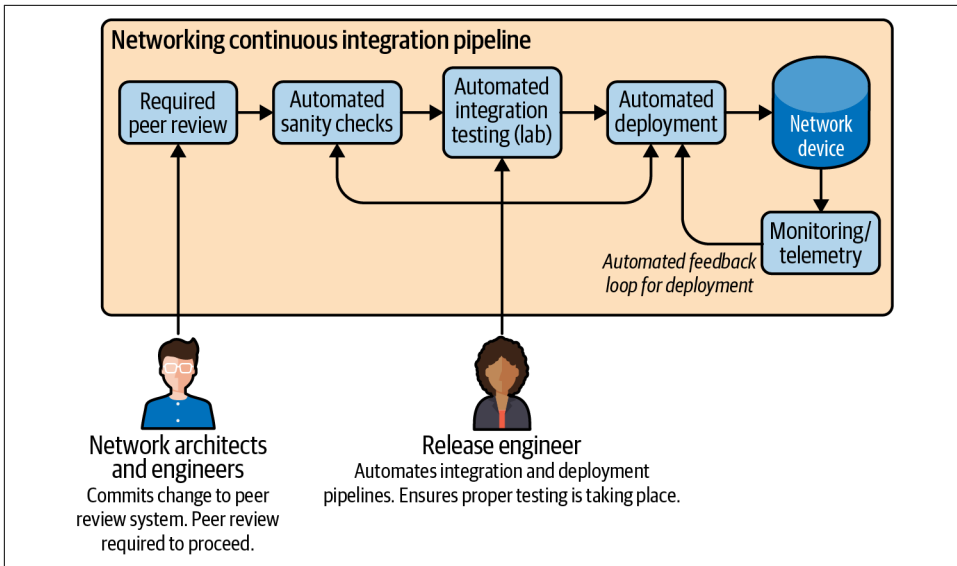
Figure 13-2. Automated change with continuous integration
