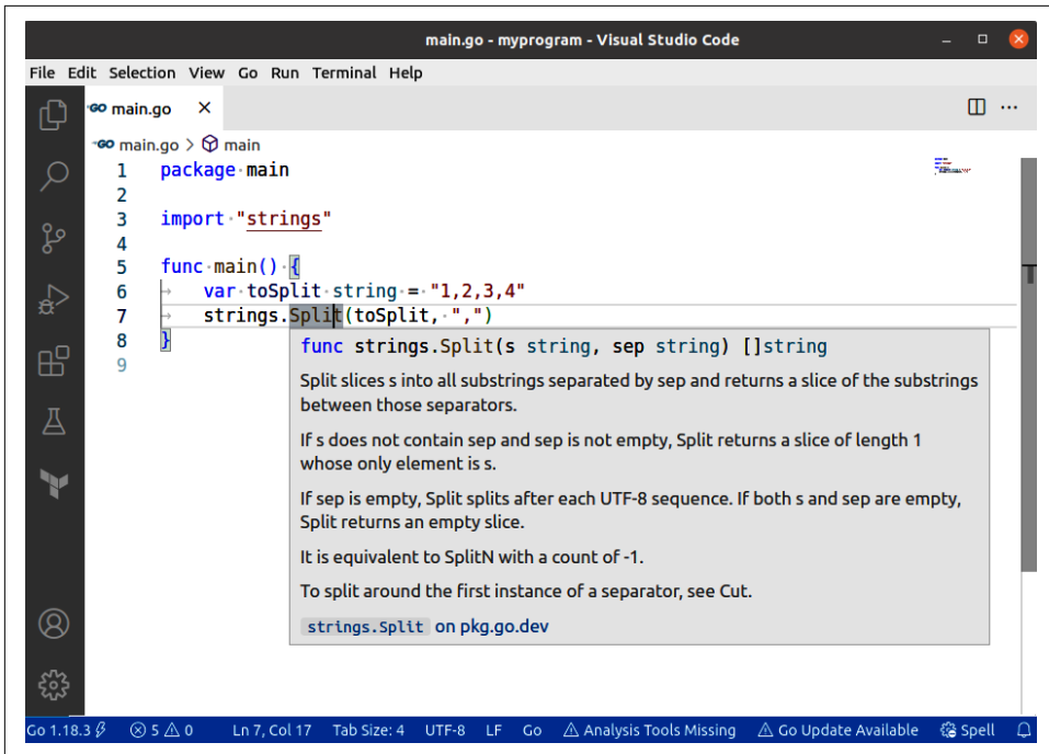
Figure 5-7. Viewing code documentation in a text editor
