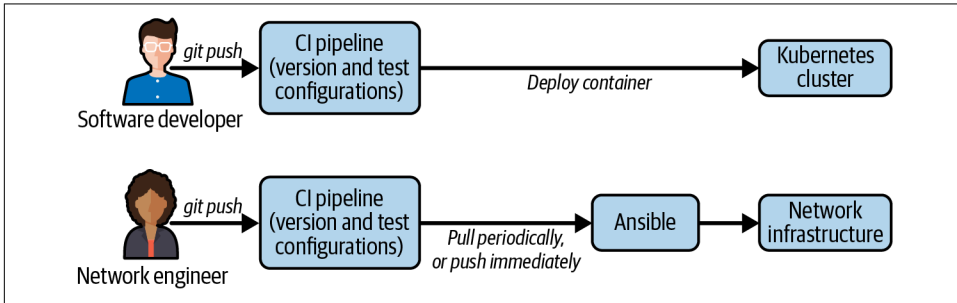
Figure 13-16. A comparison of development and networking CI pipelines
