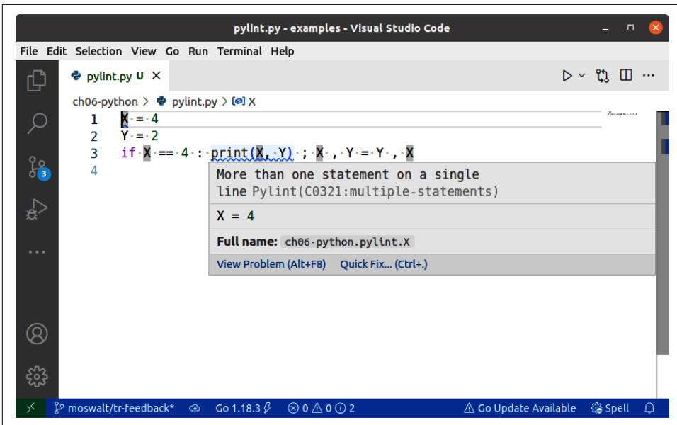
Figure 5-5. Using a text editor for linting
