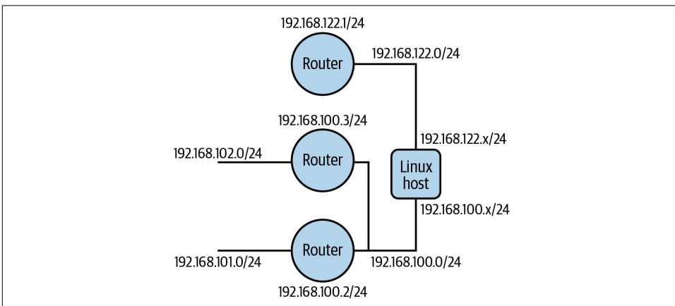
Figure 3-7. Final network topology
