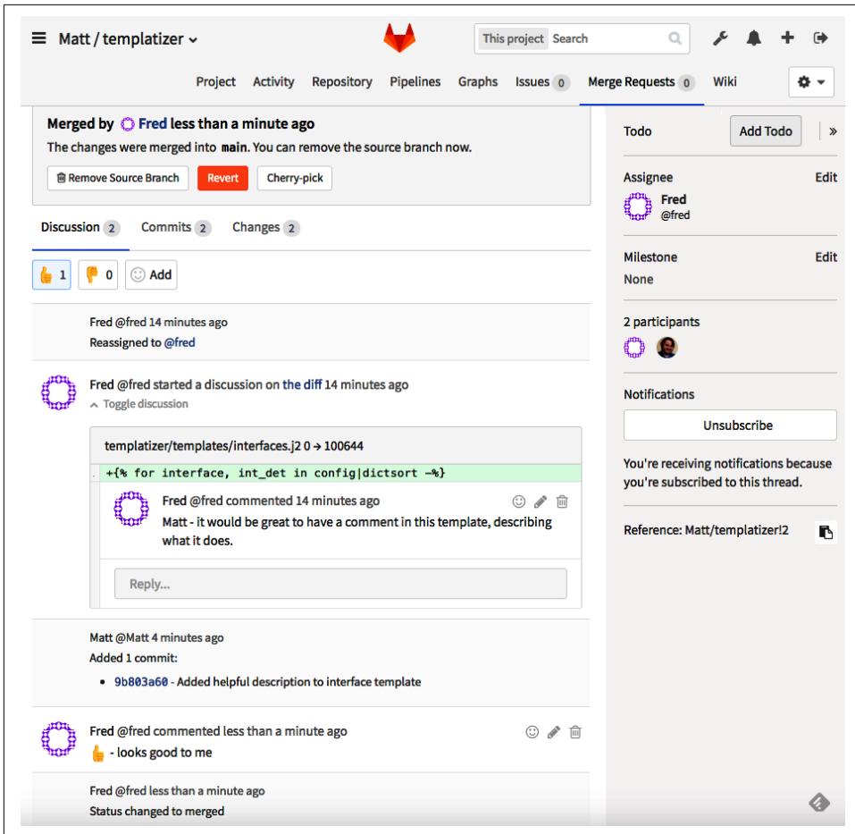
Figure 13-10. Change accepted and merged
