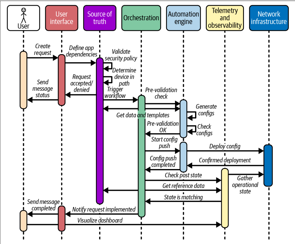
Figure 14-14. Automated workflow in a sequence diagram
