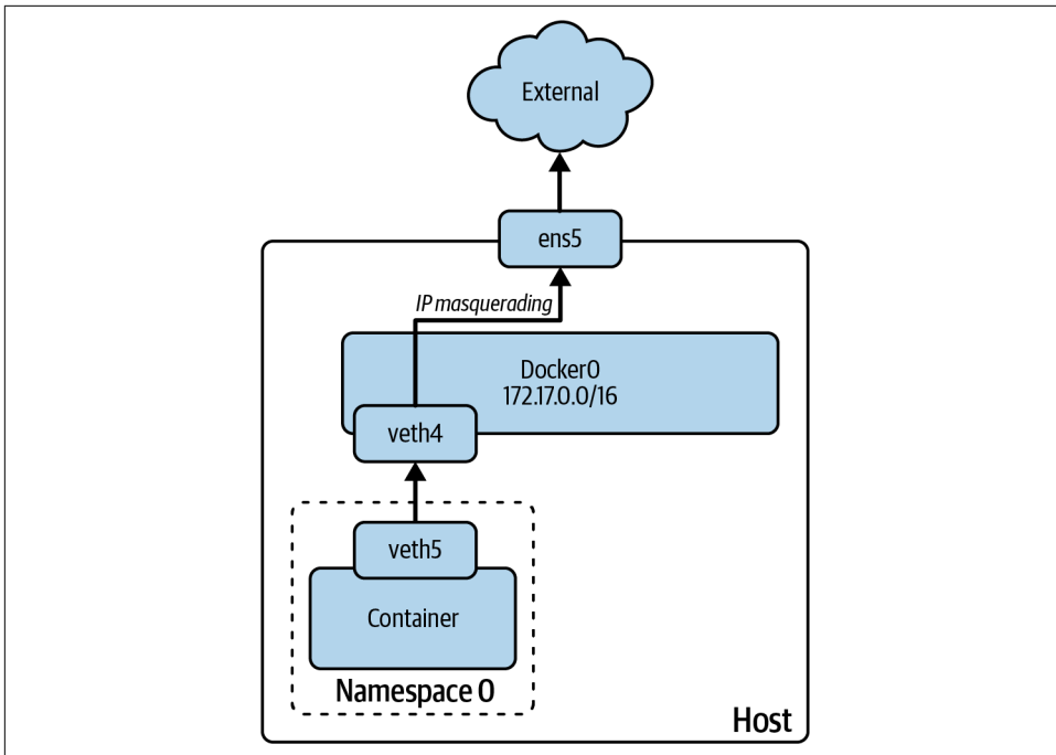
Figure 4-3. Container networking summary
