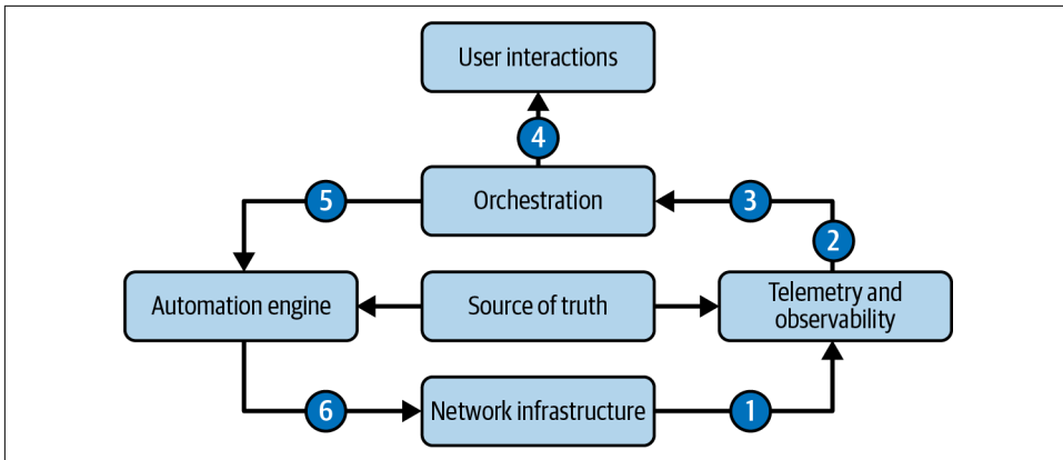
Figure 14-12. Event-driven automation
