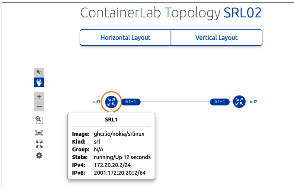
Figure 5-11. Containerlab graph
