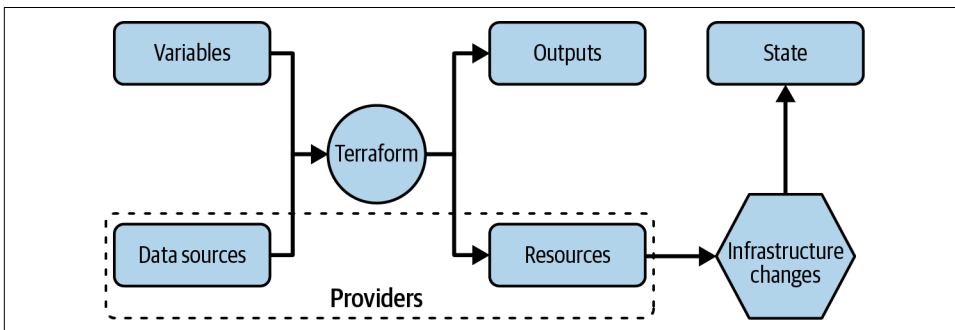
Figure 12-3. Terraform components
