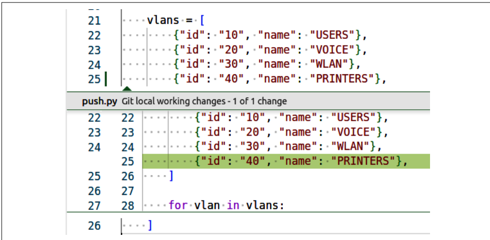
Figure 5-3. Integrating Git
