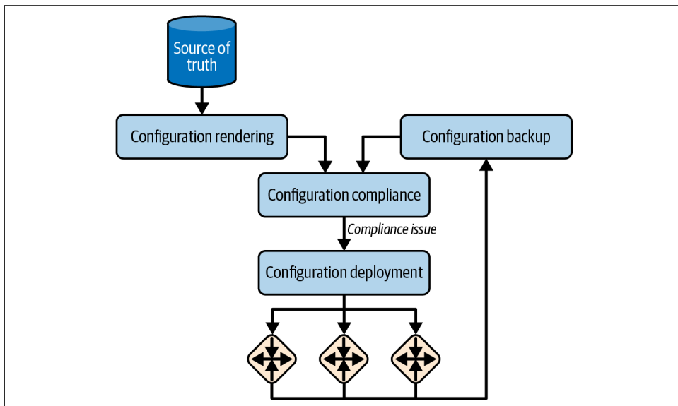
Figure 14-6. Configuration management
