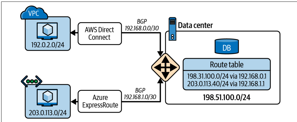
Figure 4-2. Hybrid network topology
