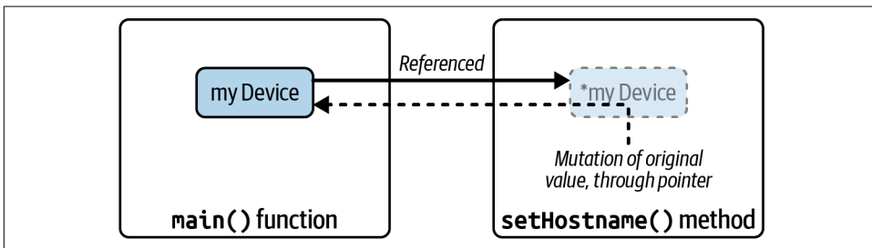
Figure 7-2. Mutating a pointer receiver
