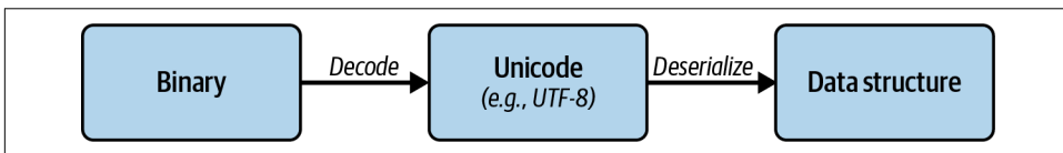
Figure 8-1. Decoding and deserializing text-based data formats
