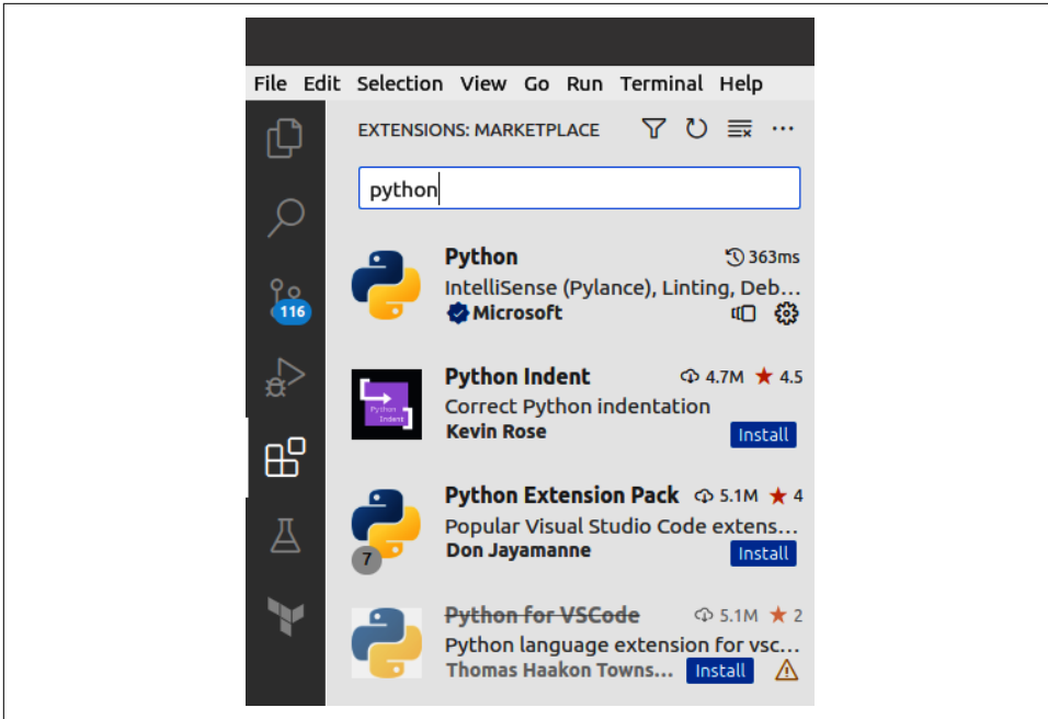
Figure 5-2. Customizing text-editor options via plug-ins
