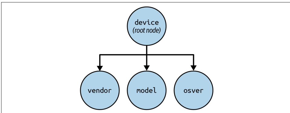
Figure 8-3. Visualization of an XML tree structure
