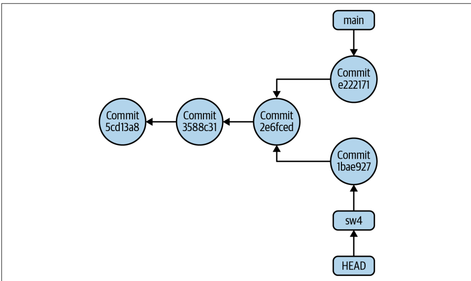
Figure 11-9. Divergent branches requiring a merge commit
