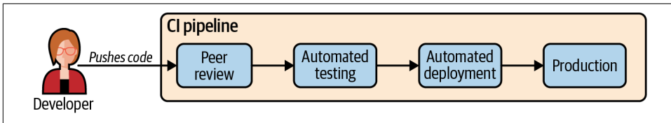
Figure 13-4. Deploying software to a CI pipeline
