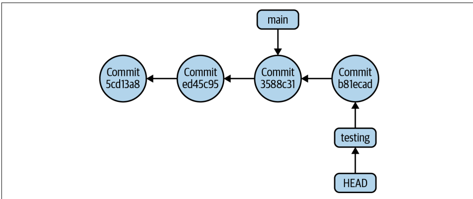
Figure 11-7. Adding a commit to a branch
