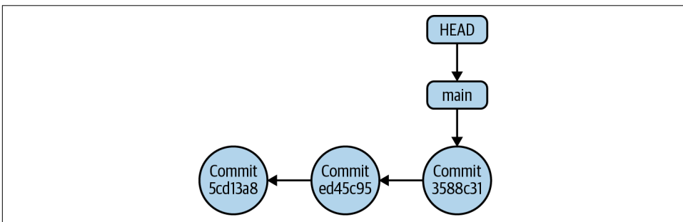
Figure 11-4. HEAD pointing to the latest commit in the default branch
