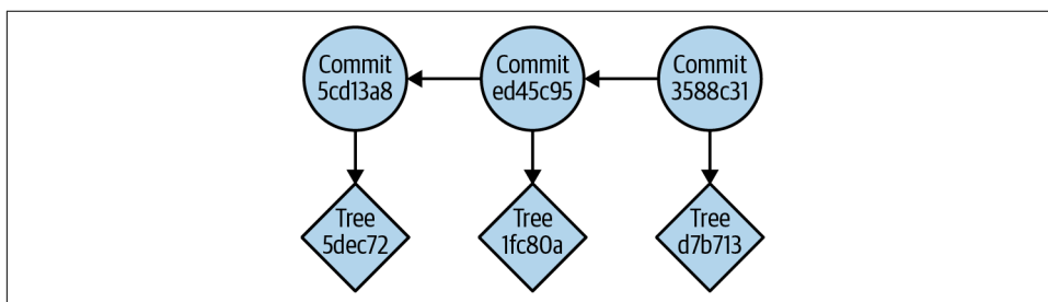
Figure 11-2. A chain of commits in a Git repository
