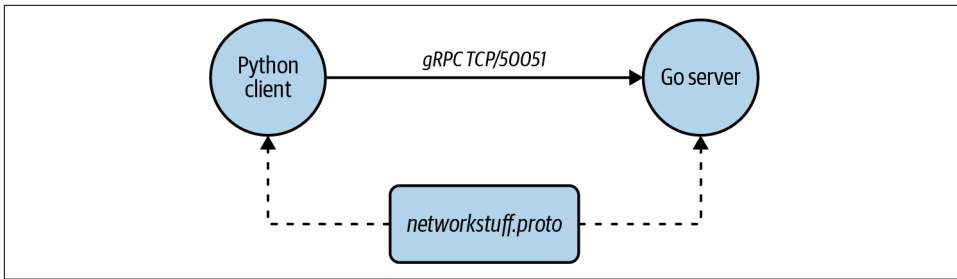
Figure 10-3. gRPC communication
