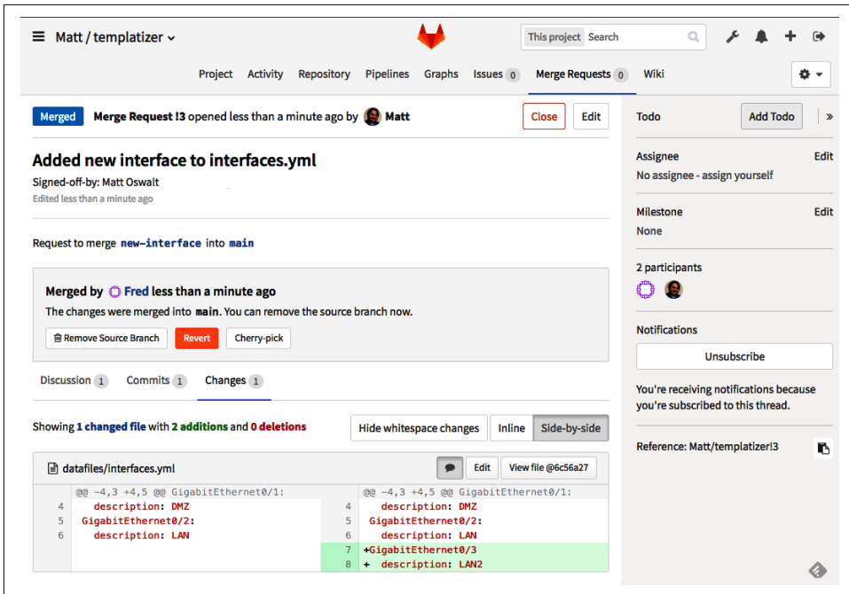
Figure 13-11. Minor change to YAML
