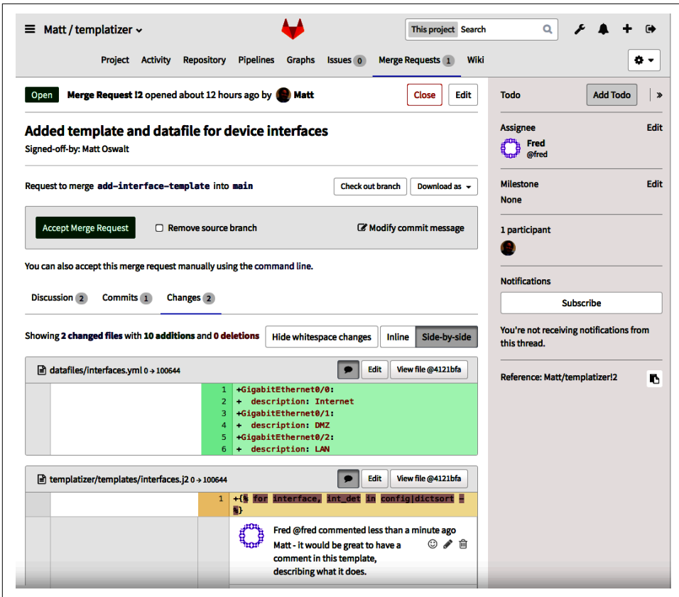
Figure 13-9. Fred providing comments to the merge request
