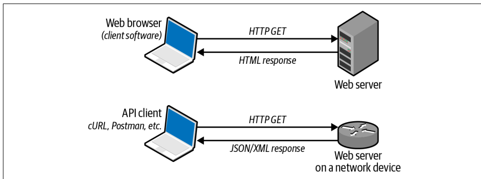
Figure 10-1. Understanding REST by looking at HTTP GET responses
