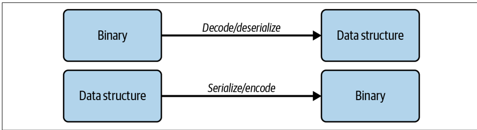
Figure 8-4. Decoding/deserialization and serialization/encoding binary data formats
