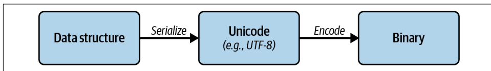
Figure 8-2. Serializing and encoding of text-based data formats
