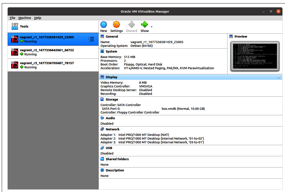
Figure 5-10. VirtualBox
