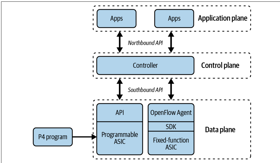
Figure 1-3. Programmable ASICs
