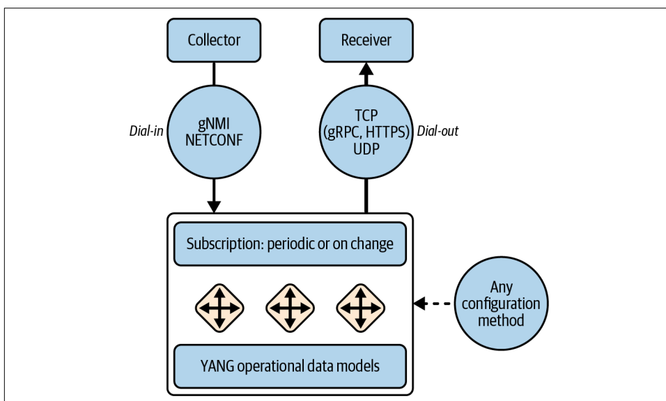
Figure 10-4. Model-driven telemetry
