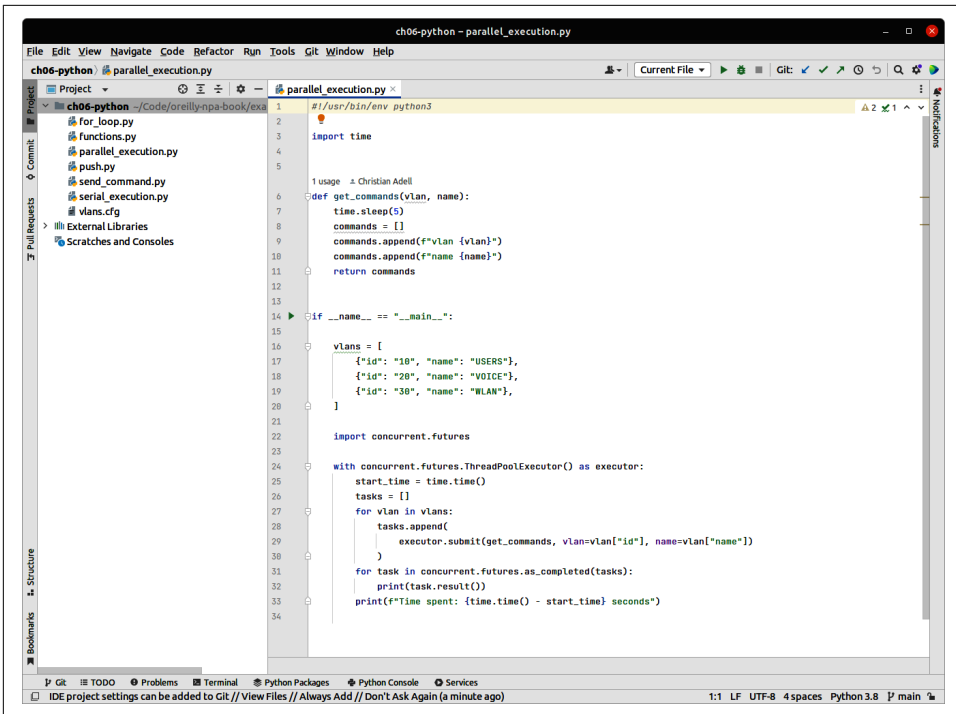
Figure 5-9. PyCharm
