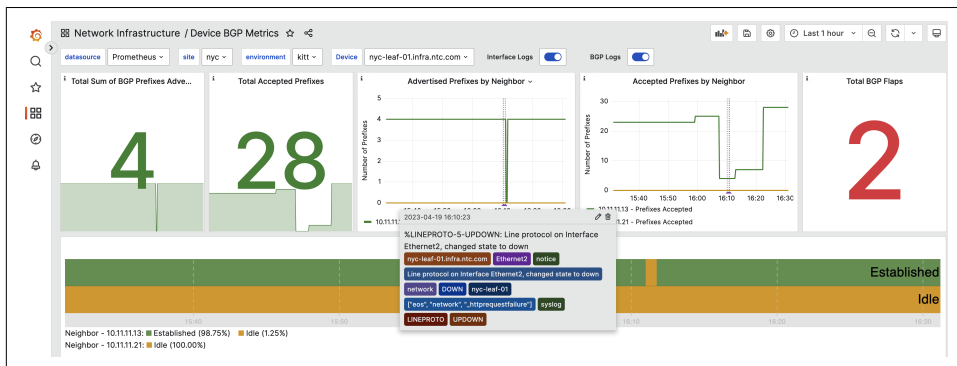
Figure 14-10. Network dashboard
