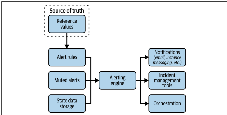
Figure 14-11. Alerting engine
