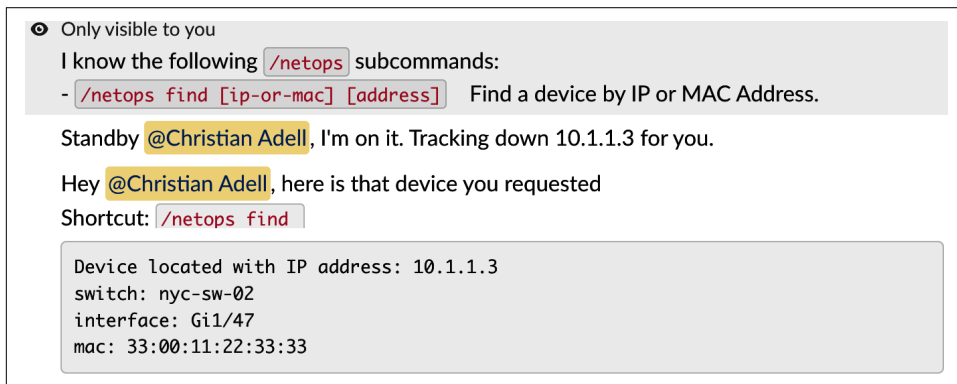
Figure 14-3. ChatOps example
