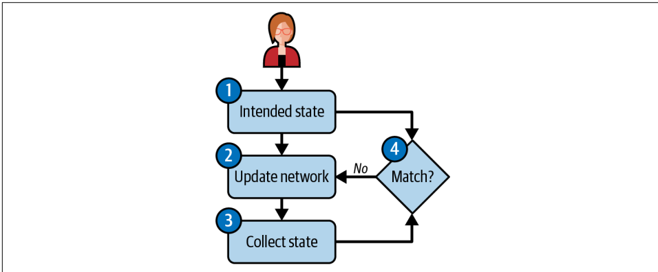
Figure 1-4. Intent-based automation
