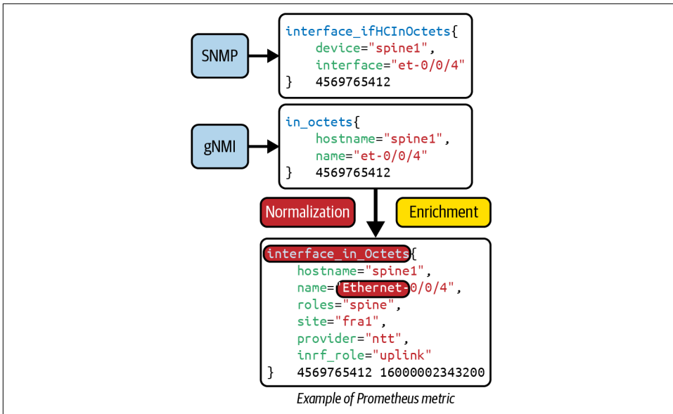
Figure 14-9. Normalization and enrichment
