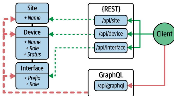
Figure 14-5. REST versus GraphQL APIs
