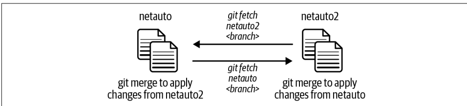
Figure 11-11. Using git fetch and git merge between repositories
