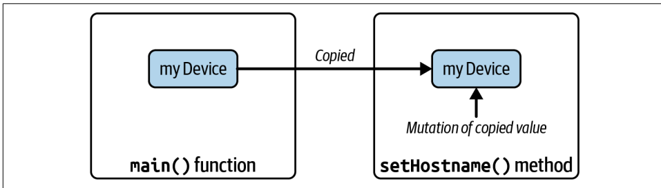
Figure 7-1. Mutating a value receiver
