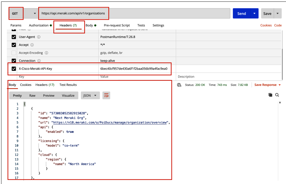
Figure 10-2. Postman GET request
