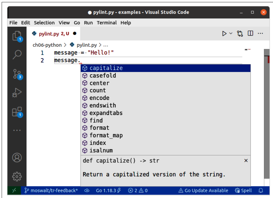
Figure 5-6. A text editor with autocompletion
