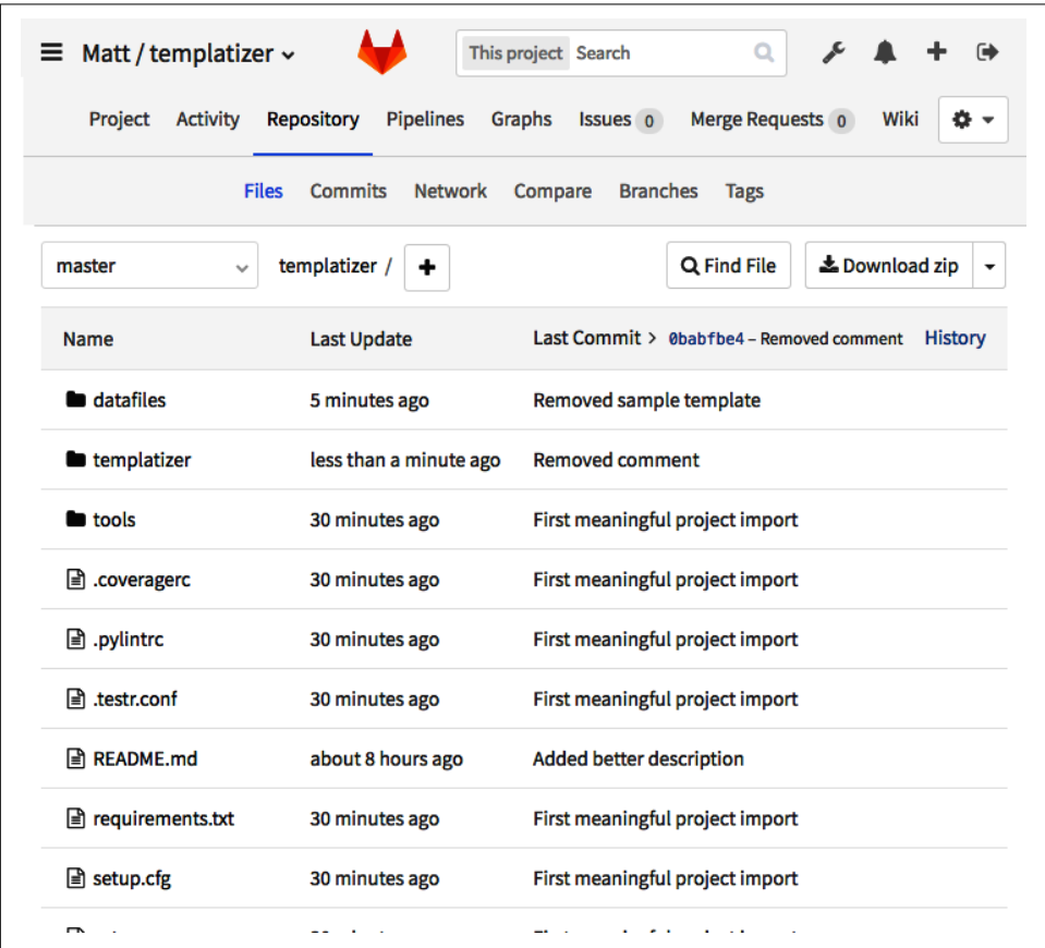
Figure 13-7. Templatizer project
