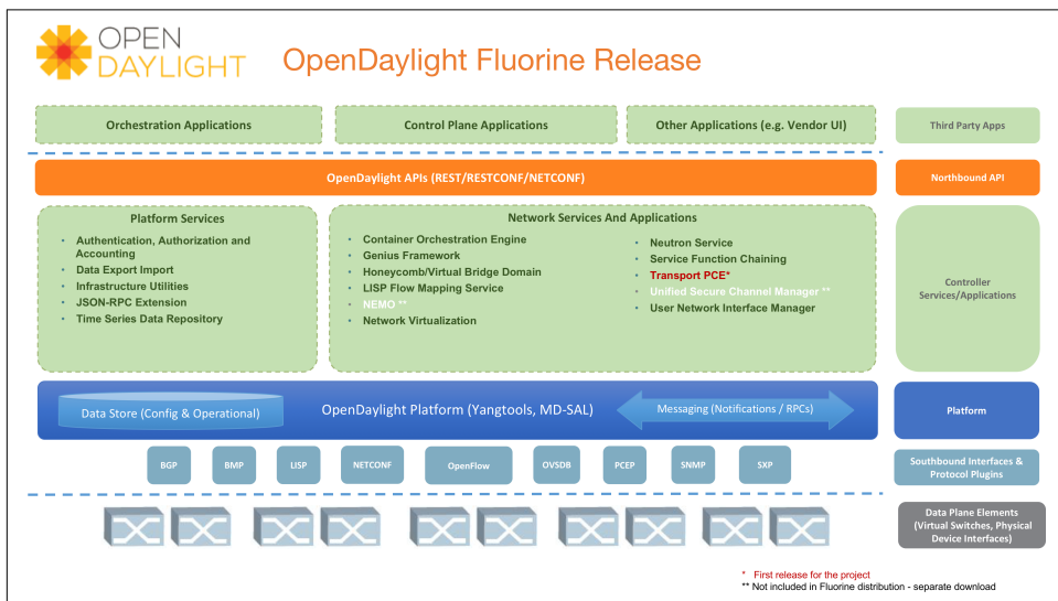
Figure 1-6. OpenDaylight architecture
