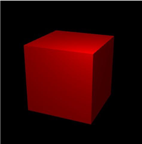
Figure 8.20 PointLightedCube_perFragment
