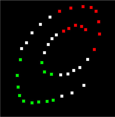
Figure 2.29 ColoredPoints
