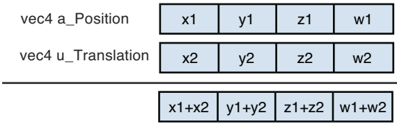
Figure 3.20 Addition of vec4 variables
