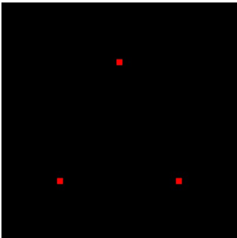
Figure 3.2 MultiPoint
