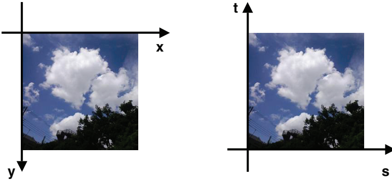
Image coordinate system
