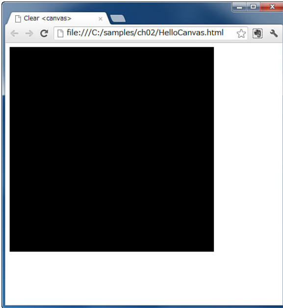
Figure 2.6 HelloCanvas
