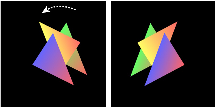
Figure 7.8 LookAtTrianglesWithKeys
