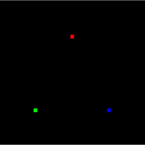
Figure 5.5 MultiAttributeColor
