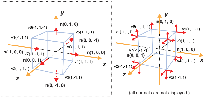
Figure 8.9 Normals of the surfaces of a cube
