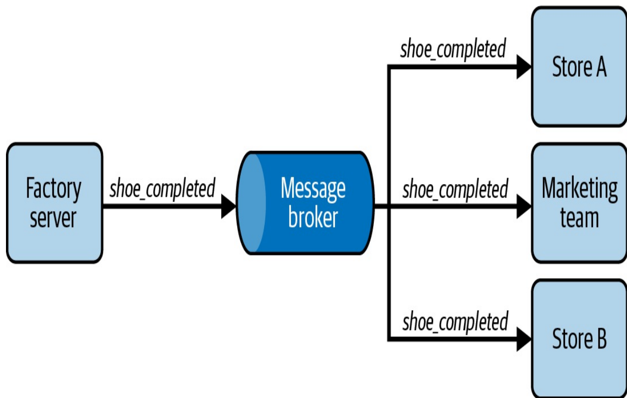
Figure 1-1. Sending/receiving shoe_completed event message
