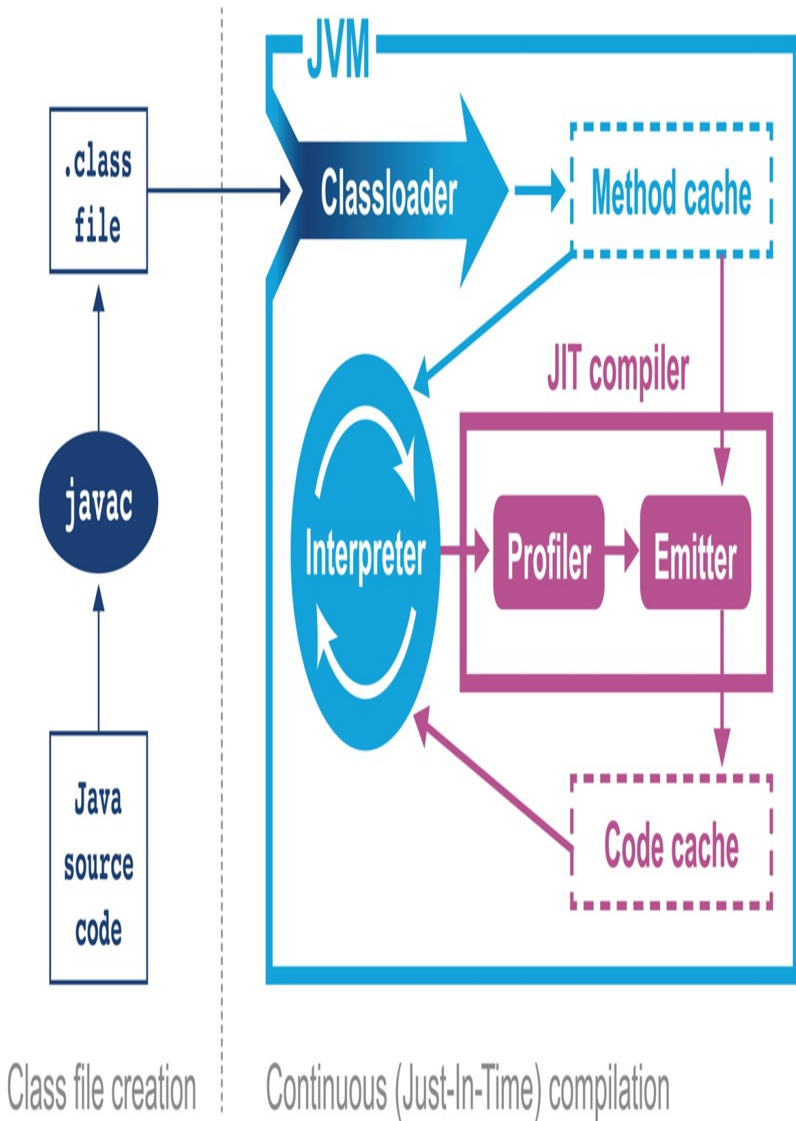
Figure 3-3. The HotSpot JVM
